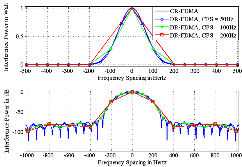
Figure 3.13: CR-FDMA and DR-FDMA, Interference vs frequency difference \delta_f , BW = 12 kHz
