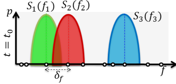
Figure 3.4: Continuous Random - FDMA scheme
