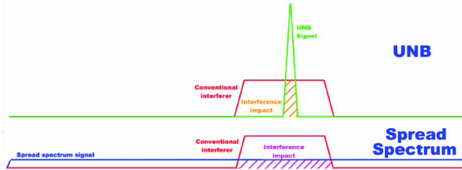
Figure 2.2: Noise vs UNB and spread spectrum signals.
