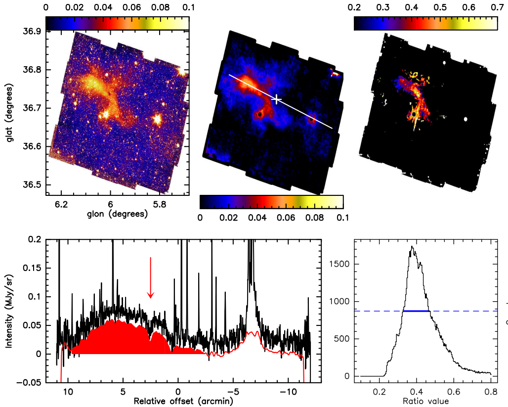
Fig. 3. Top: from left to right, L183 original image in galactic coordinates from the HCS survey (IRAC 1, 3.6 \mu\text{m} ), point sources and background-subtracted image showing the 3.6 \mu\text{m} coreshine intensity (with a Gaussian smoothing), and coreshine ratio (4.5/3.6) image. The white line shows the position of the cut presented below, the white cross indicates the zero-position reference. Bottom left: the profile through the cut for the source data (black) and through the cleaned and smoothed image (red); the 3.6 \mu\text{m} coreshine zone is highlighted by the red shading. The intensities are given in \text{MJy sr}^{-1} . The cut has been chosen to fit both a region with strong coreshine intensity ( \sim 50 \text{ kJy sr}^{-1} here) and to show the internal depression, which traces self-absorption, \sim 2.5 \text{ arcmin} from the zero reference, marked by the red arrow on the profile. Bottom right: the coreshine ratio histogram. The blue line displays the FWHM of the histogram.
