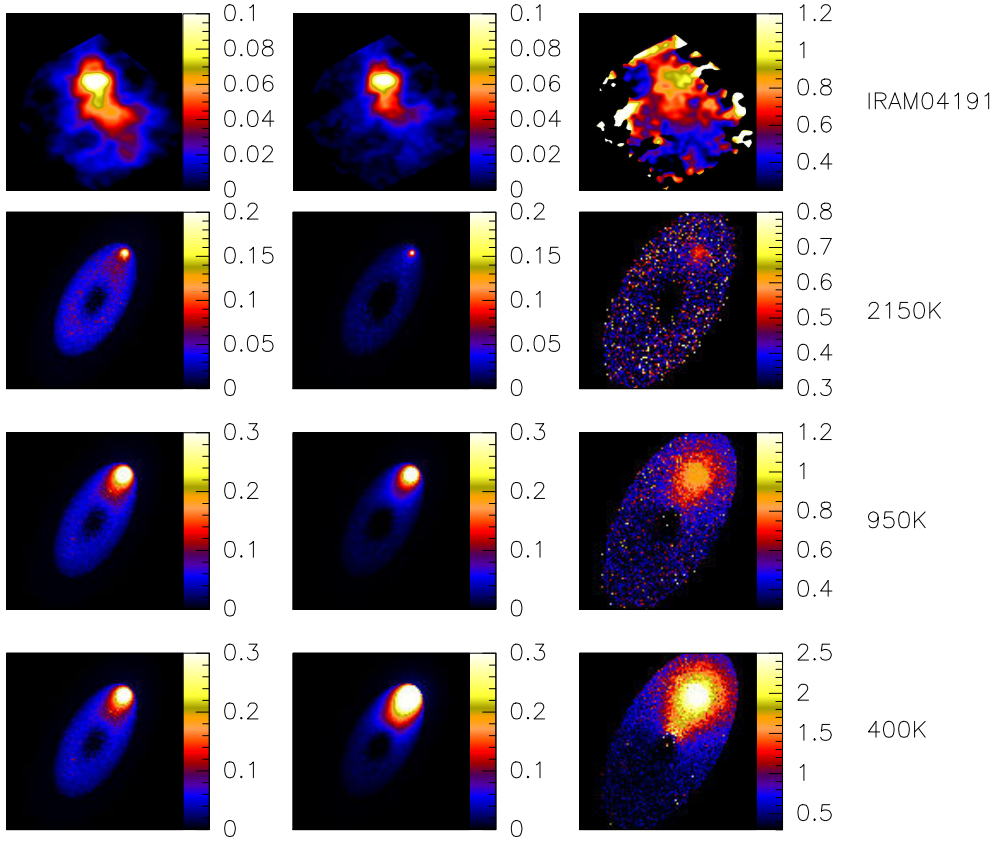
Fig. 16. From left to right: IRAC 1 (3.6 μm), IRAC2 (4.5 μm), core-shine ratio. First row: analysis of IRAM04191 Spitzer observations. Next rows: modeling in the dense case ( M_{\text{high}} ) for the three internal sources. Color scales are given in MJy sr -1 .
