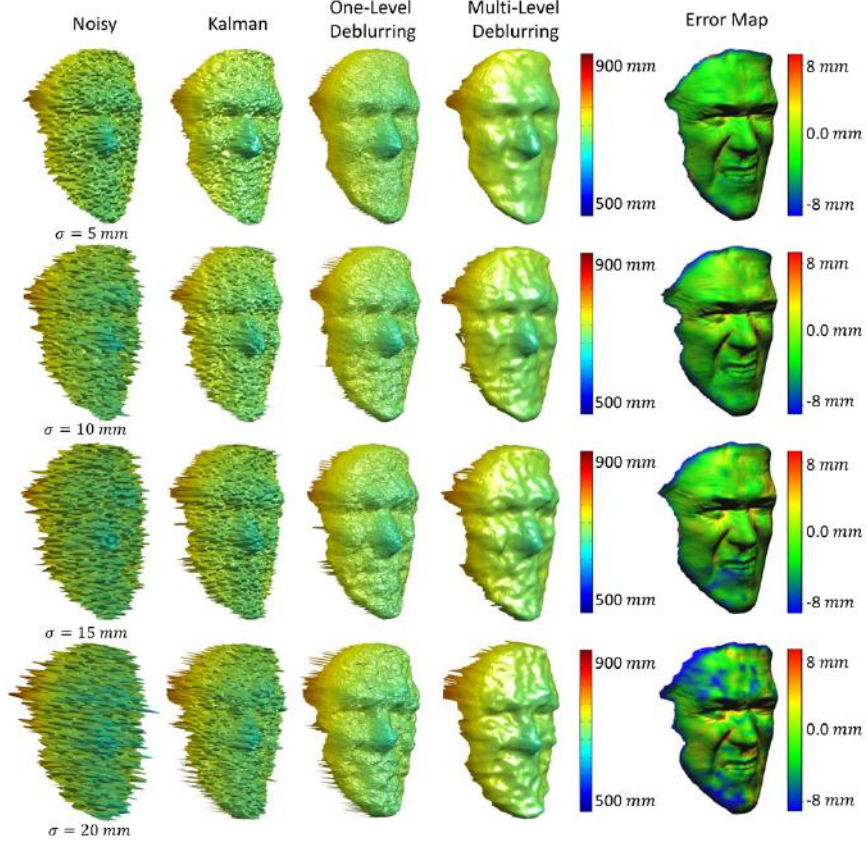
Figure 5.7: 3D plotting of (starting from left column): 1) LR noisy depth frames, 2) super-resolved depth frames with r = 4 using Kalman filter, 3) super-resolved depth frame with r = 4 using the proposed method with one-level deblurring step with [L = 1, K = 25] 4) super-resolved depth frame with r = 4 using the proposed method with the proposed multi-level deblurring step with [L = 5, K = 25] , 5) Error map of comparing the obtained results in forth column with the 3D ground truth.
