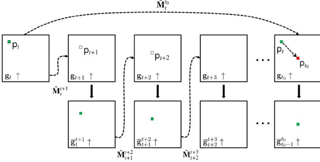
Figure 4.1: UP-SR Cumulative Motion Estimation: All intermediate registered upsampled depth frames are used to register the pixel p_t in frame g_t \uparrow to its corresponding pixel at the position p_{t_0} from the reference frame g_{t_0} \uparrow where g_t \uparrow and g_{t_0} \uparrow are non-consecutive upsampled frames.
