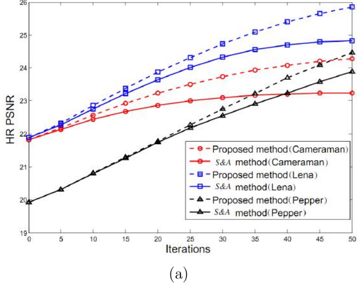
Figure 3.5: PSNR per iteration of the proposed selective optimization in eS\&A against S\&A [7] using 11 ( 96 \times 96 ) LR images with SNR = 25dB and SR scale factor r = 5 .
