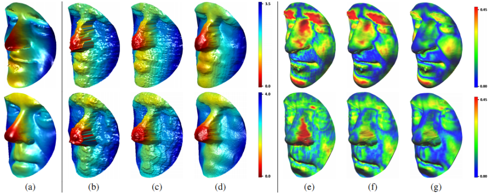
Figure 7.5: 3D face reconstruction results. (a) 3D laser scan ground truth. (b) One of the LR 3D faces. (c) Results of the superfaces algorithm. (d) Results of the proposed SurfUP-SR algorithm. (e) 3D error map corresponding to the 3D LR face. (f) 3D error map corresponding to the superfaces results. (g) 3D error map corresponding to the proposed SurfUP-SR .
