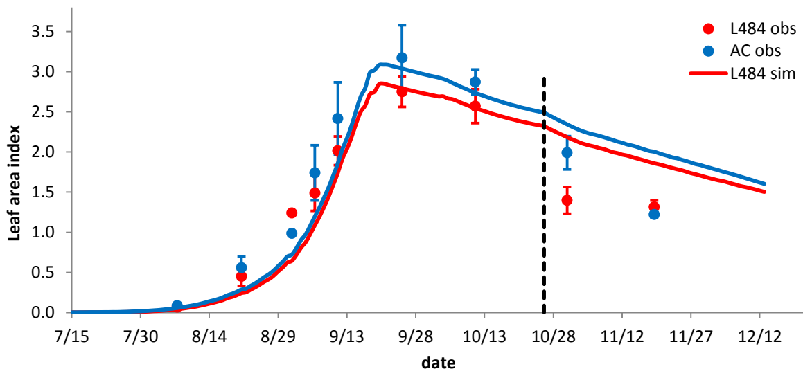
Figure 27. Calibration of leaf area index for cultivars L484 and AC in eraly planting of Sanguéré 2013.
