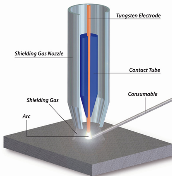
Figure 1.1: GTAW Process [9]
