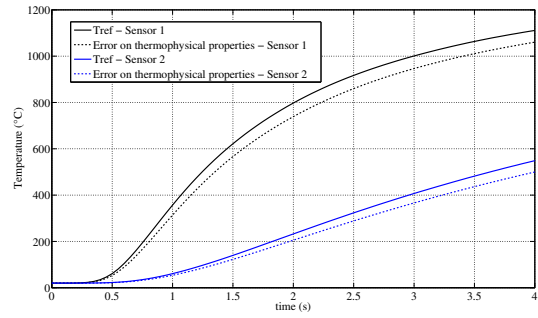
(b) Reference temperatures (with no noise) and new input temperatures with errors on the thermo-physical properties.
