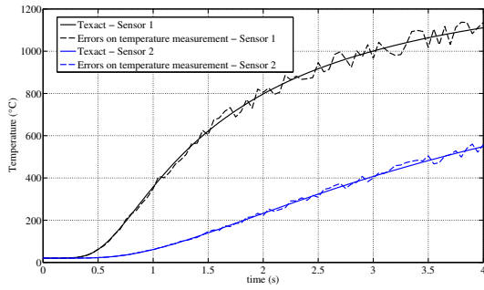
(a) Reference temperatures (with no noise) and new input temperatures including noise measurement.
