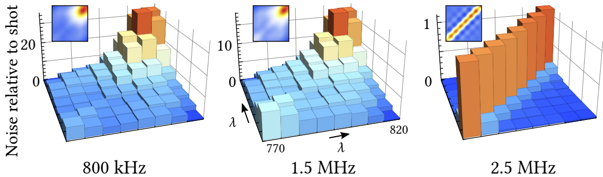
Figure 7.4: Covariance matrix representation of the fluctuations in amplitude only of the laser source described in 3.1.1.
