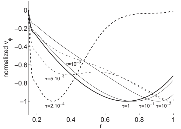
Figure 11. Radial profiles taken at various times of the azimuthal velocity in the equatorial plane of the star for E = 10^{-5} , B = 10^2 , \epsilon = 10^{-7} , \lambda = 10^{-4} , and Ro = 10^{-5} . Profiles are scaled as in Fig. 10. The dimensionless time \tau is specified for each curve. Dashed lines are profiles for baroclinically dominated dynamics while solid lines are for spin-up dominated dynamics. The dashed bold curve shows the initial profile and the solid bold curve shows the last profile.
