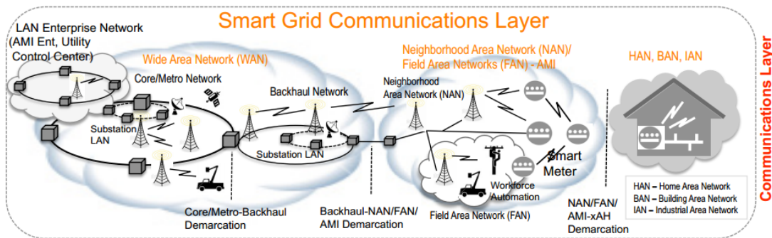
Figure 2.2: Smart Grid from communications Point of View. (source: IEEE )
