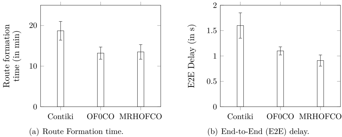
Figure 7.4: Route formation time and E2E delay in a large-scale narrowband PLC network with RPL under different objective functions – vanilla Contiki (with ETX/MRHOF), OF0 based on CO, and MRHOF based on CO. The bars provide the average values over 30 independent simulations, whereas the whiskers indicate the 95% confidence interval.
