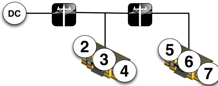
(b) Urban topology – high-density area. Nodes 2-3-4 can communicate directly with all others, while Nodes 5-6-7 need to go through at least one intermediary to reach the DC.
