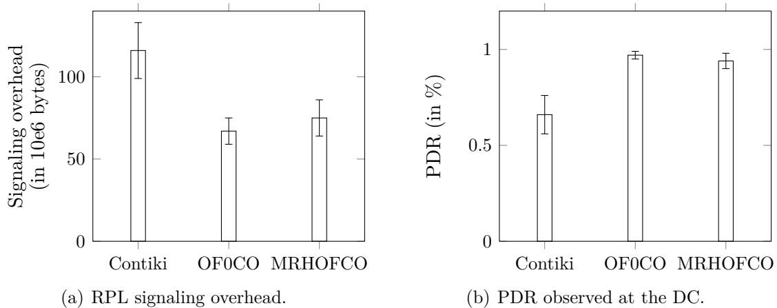
Figure 7.5: Average values and 95% confidence interval for signaling overhead and PDR with RPL different metrics – vanilla Contiki (with MRHOF), OF0 based on CO, and MRHOF based on CO.
