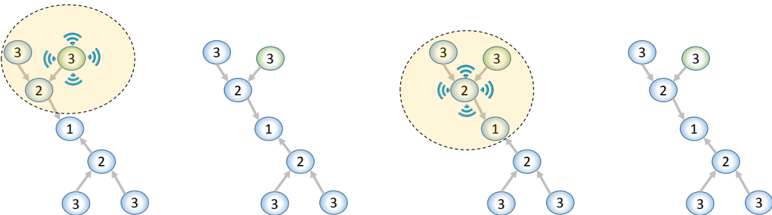
Figure 3.6: Downward Route Construction for Non-Storing Mode (Green Circle represents the Node sending the first DAO - Light Yellow Circle represents DAO transmission coverage area - Light grey arrow represents Upward Routes - Number inside the circle represents the rank of a node).
