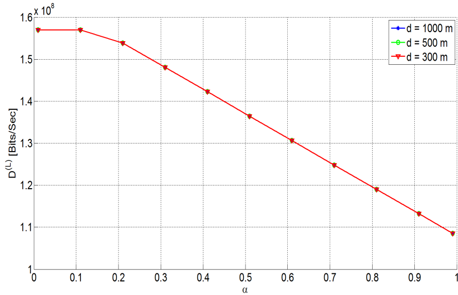
Figure 5.5 – LTE received data rate in [Bits/sec]
