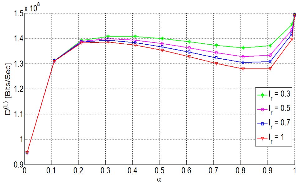
Figure 5.8 – LTE data rate w.r.t. \alpha labeled on interference-cancellation coefficient and d = 1000 m.
