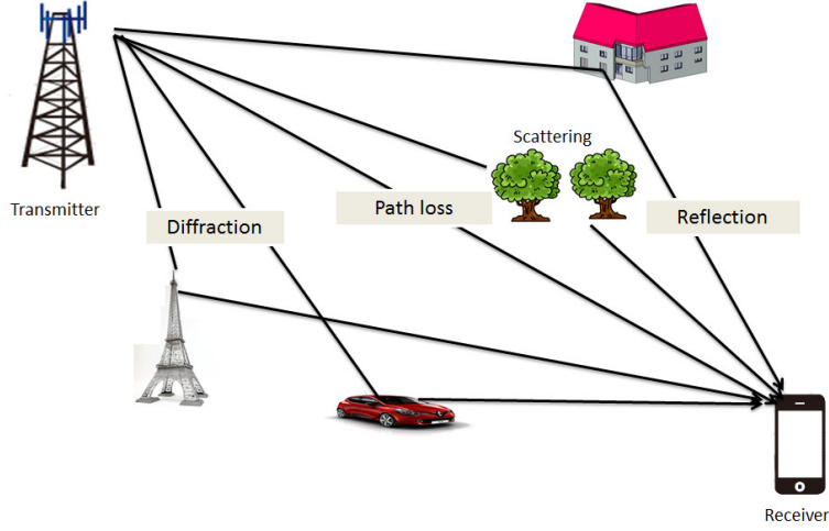
Figure 1.2 – Multipath channel
