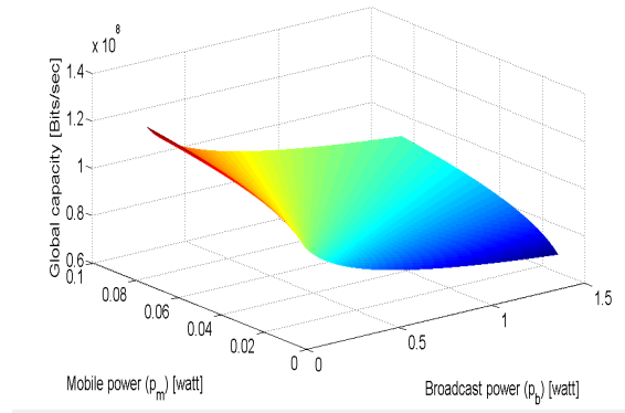
(c) Global data rate
