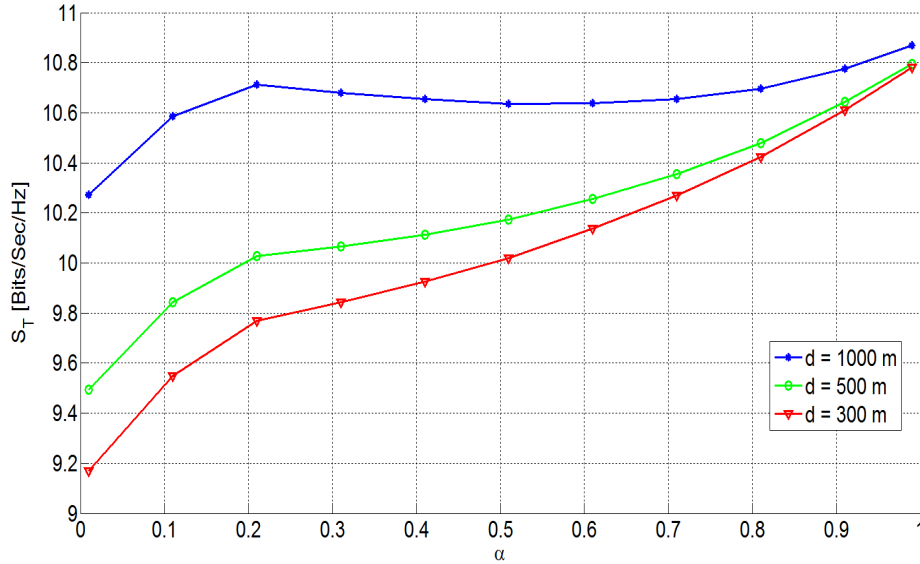
Figure 5.7 – Total spectral efficiency w.r.t. \alpha and labeled on d .
