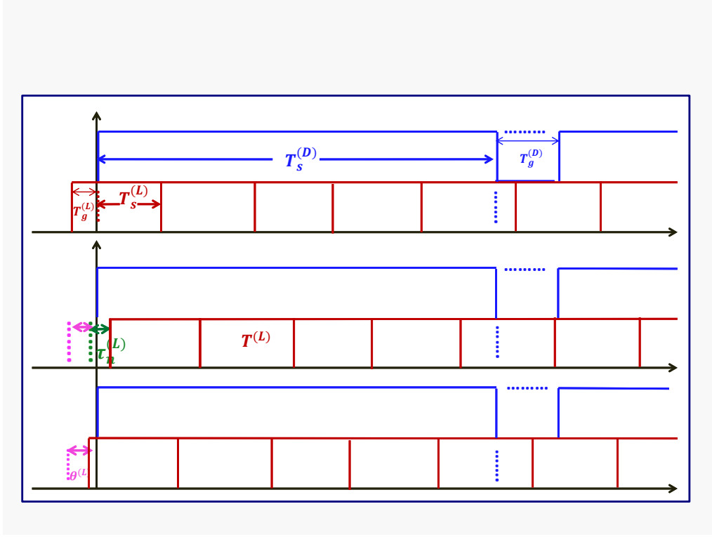
Figure 5.4 – Interfering LTE symbols over DVB symbol
