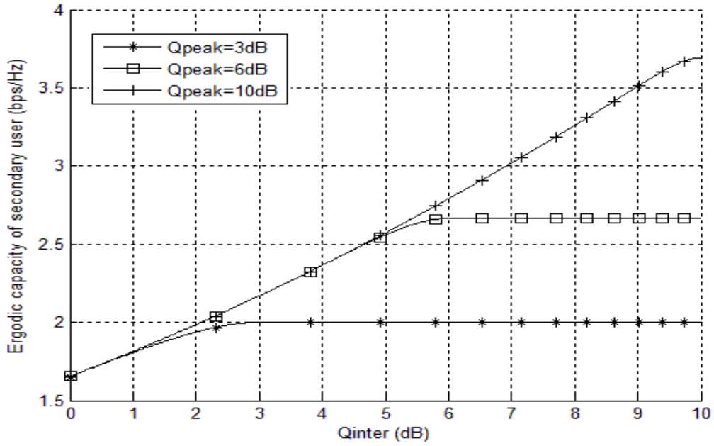
Figure 2.7 – Ergodic capacity versus Q_{inter} for different Q_{peak} values.
