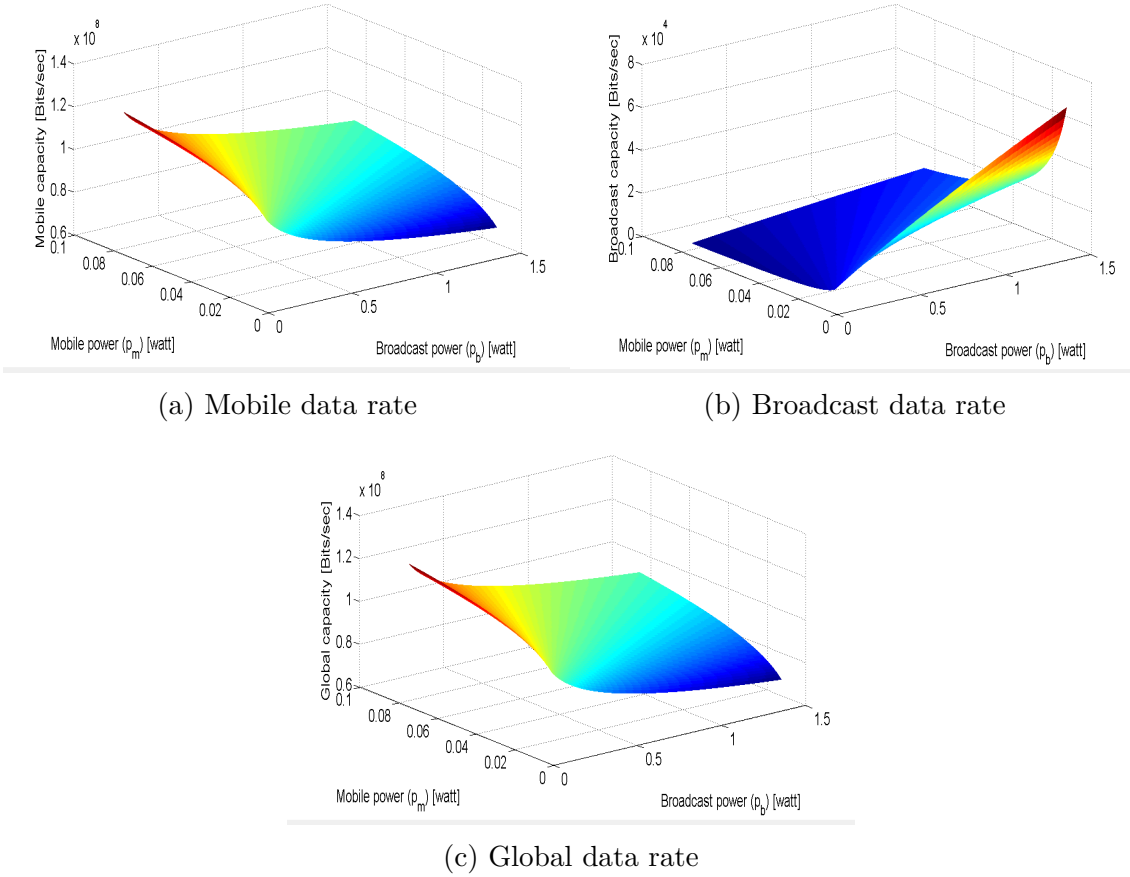
Figure 3.6 – Data rate variation in (bits/sec) according to p_b and p_m , B_m = 10 MHz, DVB mode 8K, d = 100 m.
