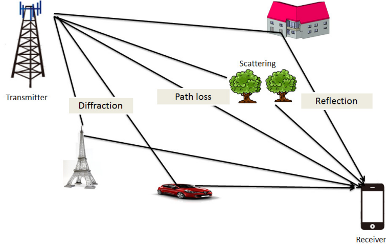
Figure 1.2 – Multipath channel
