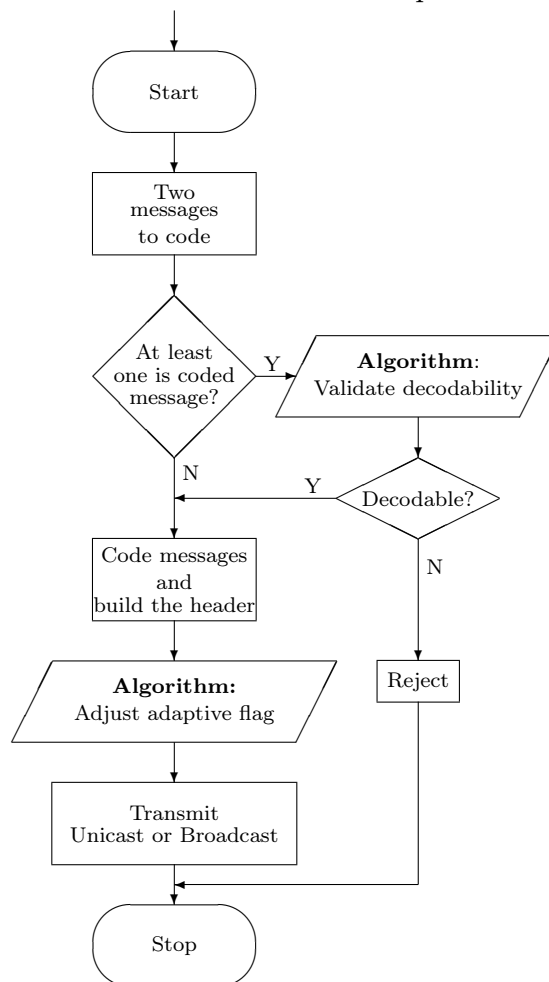
Figure 2.9: Coding and Forwarding Process (CFP)
