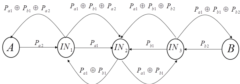
Figure 4.1: NC technique
