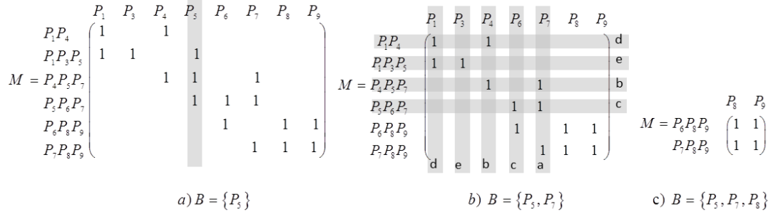
Figure 5.9: BCSD example
