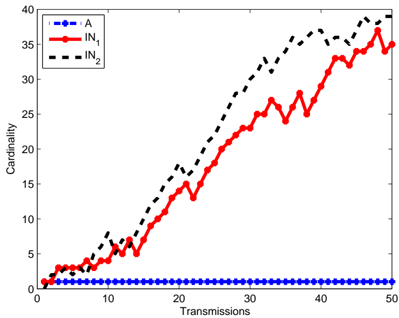
Figure 2.14: Cardinality of coded message at different nodes without synchronization
