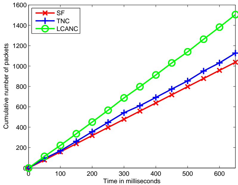
Figure 2.6: Cumulative number of packets transmitted
