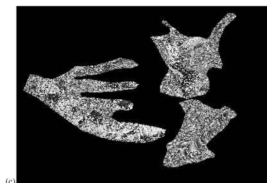
Fig. 3. Wrapped phase difference between interferograms on the Tour, Trient, and Saleina glaciers with the new DEM. (a) \Delta\Phi_{\text{April-March}} . (b) \Delta\Phi_{\text{April-December}} . (c) \Delta\Phi_{\text{April-October}} .
