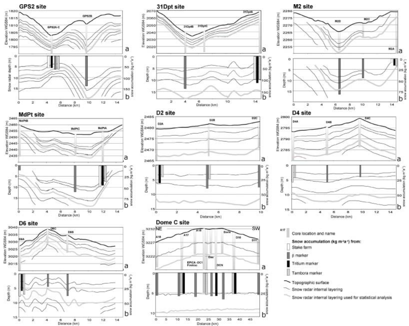
Fig. 2. (a) Core location and elevation of GPR selected horizons and surface profiles; (b) depth profile of GPR selected horizons and snow accumulation from firm cores using different methods.
