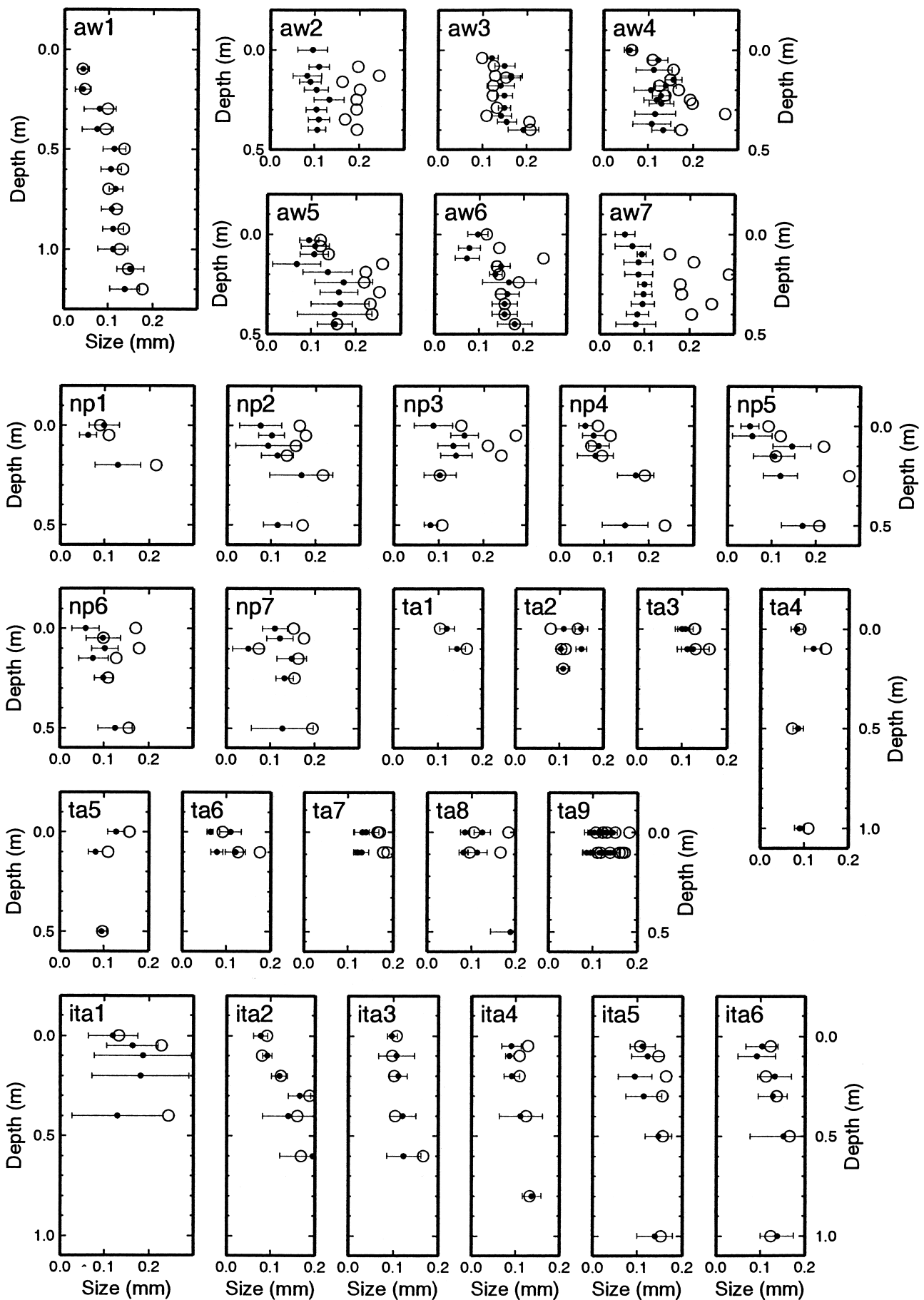
Fig. 6. Mean convex radius of snow grains vs depth along several traverses (Table 2; Fig. 1). Technique 1 is used for all the samples. The dots (●) are for radii corresponding to the end-points of the skeleton, and circles (○) are for nodal points.
