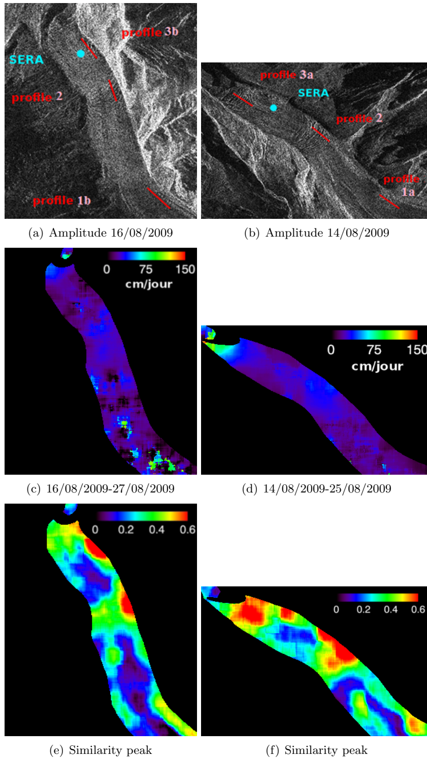
FIGURE 6.3.2 – Amplitude image of Argentiere Glacier in ascending passes (figure 6.2(a)) and descending (figure 6.2(b)); 2-D displacement fields, arising from amplitude correlation (figures 6.2(c) and 6.2(d)) and their similarity peak (figures 6.2(e) and 6.2(f)).
