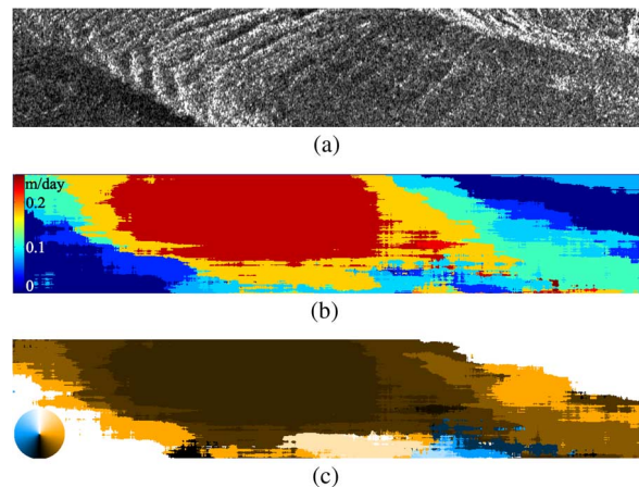
Fig. 5. Displacement estimation over a crevasse field of the Argentière glacier, dual-pol TSX data, 2009-01-06/2009-02-08. (a) Master texture estimated using SIRV model. (b) Displacement field in LOS. (c) Orientation map.
