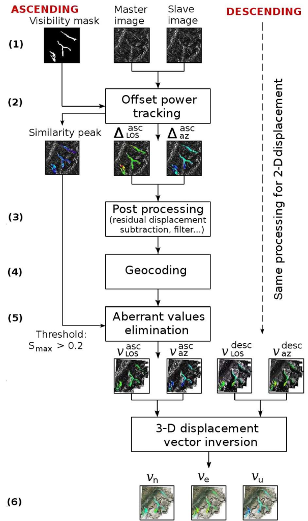
Fig. 3. Steps of SAR offset power tracking analysis, from SAR images to 3-D displacement results.
