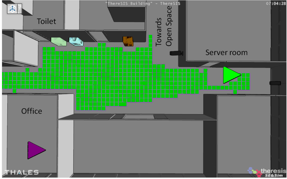
Figure 5.22: 3D representation of the office building environment. The green squares represent areas under sensory coverage. The purple and green triangles are used to model the activities associated with the office room and the server room respectively.
