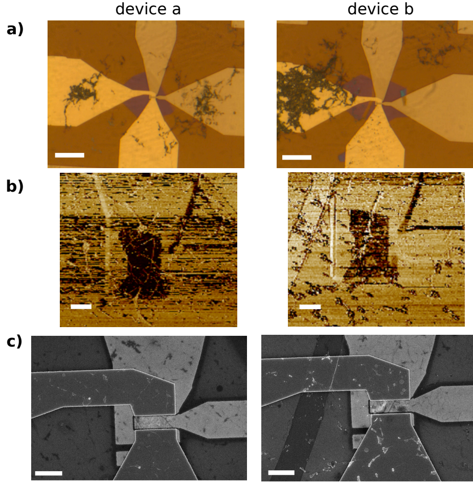
FIGURE 4.20: (a) optical pictures of devices GoBN3-4x2 and GoBN3-1x2. One can notice the remains of folded CVD graphene outside the BN flake. White scale bar: 10\ \mu\text{m} . (b) AFM images (phase mode) of the two devices before contact deposition. One can notice the presence of a few graphene wrinkles. White scale bar: 1\ \mu\text{m} . (c) SEM images of the devices. The channel of device 4x2 appears much cleaner than the one of 1x2. White scale bar: 1\ \mu\text{m} . Device dimensions: L = 500\ \text{nm} , W = 1.5\ \mu\text{m} and t_{BN}^{4\times 2} = 15\ \text{nm} , t_{BN}^{1\times 2} = 12\ \text{nm} .
