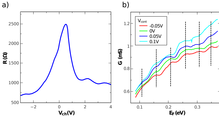
FIGURE 4.15: Device GoBN2 measured at 6 K. (a) Resistance as a function of the channel gate voltage for V_{cont} = 0 . Fabry P erot oscillations observed on the n-side. (b) Conductance as a function of the channel Fermi energy for V_{cont} = -0.05 \rightarrow 0.1 V from bottom to top. Several oscillations are identified by the vertical dotted lines (maxima of the red curve). A period of 50 meV is observed, that corresponds to a 40 nm cavity.
