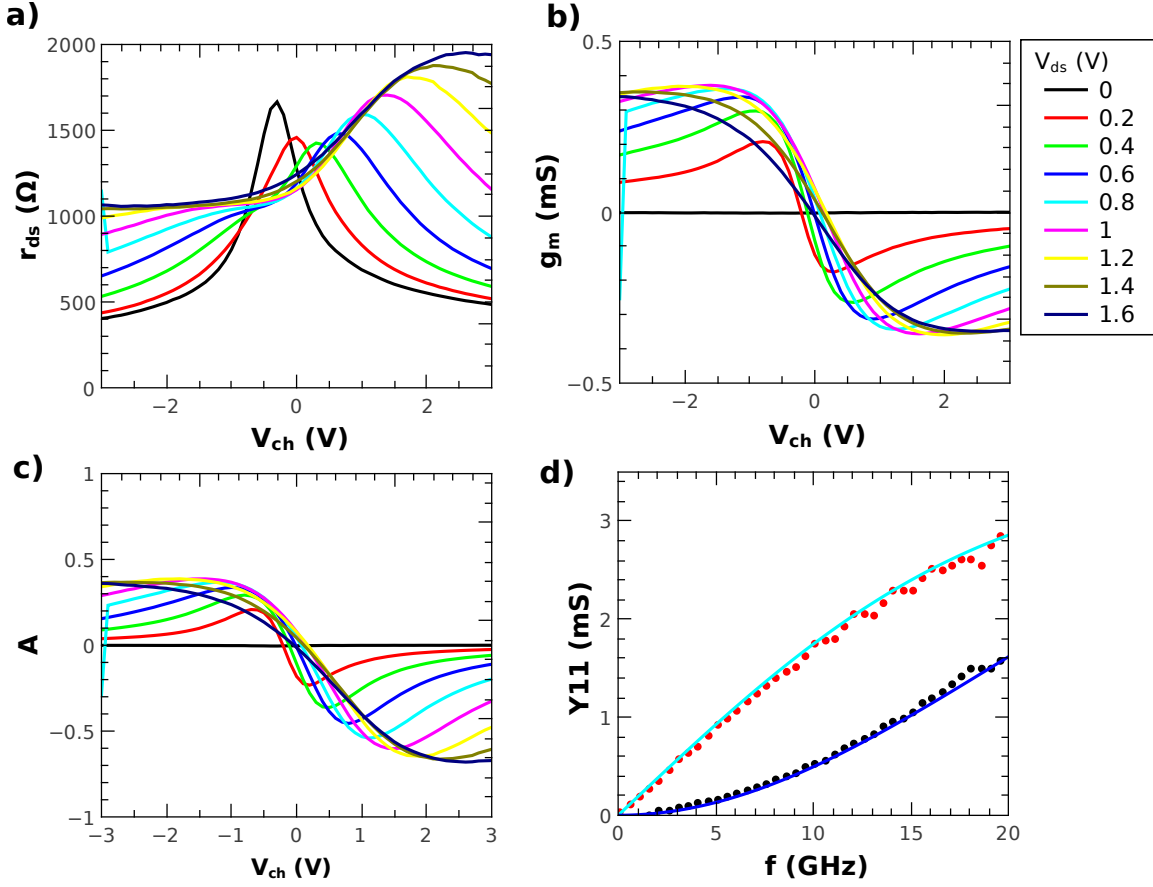
FIGURE 6.4: Quantities extracted from Fig. 6.3. (a) Small signal resistance (b) transconductance and (c) voltage gain as a function of the gate voltage, for bias voltages V_{ds} = 0 \rightarrow 1.6 V . (d) Y_{11} spectra real (blue line) and imaginary (red line) parts fitted with Eq. 6.8 (solid lines). The fit gives R_G = 150 \Omega and C'_{gs} + C_{gs}^0 + C_{gd} + C_{gd}^0 = 30 fF
