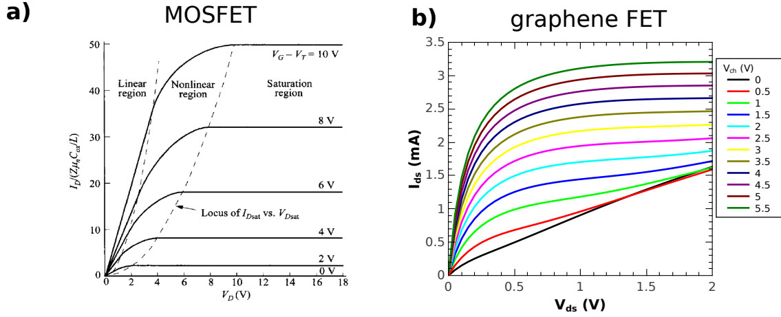
FIGURE 5.13: (a) Typical I-V curves of a MOSFET from [71]. (b) Simulated I-V curves of a graphene transistor ( L = 500 \text{ nm} , W = 1.5 \text{ }\mu\text{m} ). The simulation parameters are identical to those of Figs. 5.11 and 5.12 except that the mobility \mu = 15 \cdot 10^3 \text{ cm}^2/\text{V/s} and V_{ds} = 0 - 2 \text{ V} have been pushed further in that simulation. The current saturation is as good for the graphene transistor as for the MOSFET. The I-V curves of the graphene transistor show ideal properties for a FET: there is a fast increase of the current, thanks to the high mobility, and a saturation thanks to the scattering by the remote phonons of hBN
