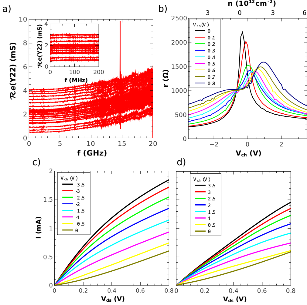
FIGURE 5.5: High bias measurement on sample GoBN3-4x2 ( L = 0.5 \mu\text{m} , W = 1.5 \mu\text{m} , t_{\text{hBN}} = 15 \text{ nm} ) at T = 8 \text{ K} . (a) VNA measurement of the small signal channel conductance \Re(Y_{22}) = g_{\text{ds}}(f) as a function of frequency in the range 70 \text{ kHz} \rightarrow 200 \text{ MHz} (inset) and up to 20 \text{ GHz} (main panel). (b) Differential resistance r extracted from panel (a) by averaging \Re(Y_{22})^{-1} over the flat frequency range 70 \text{ kHz} \rightarrow 3 \text{ GHz} , as a function of gate voltage V_{\text{ch}} for various biases V_{\text{ds}} . (c) I-V characteristics for V_{\text{ch}} < 0 . (d) I-V characteristics for V_{\text{ch}} > 0 . We observe a trend toward saturation at high densities, and a slight change of curvature near the Dirac point.
