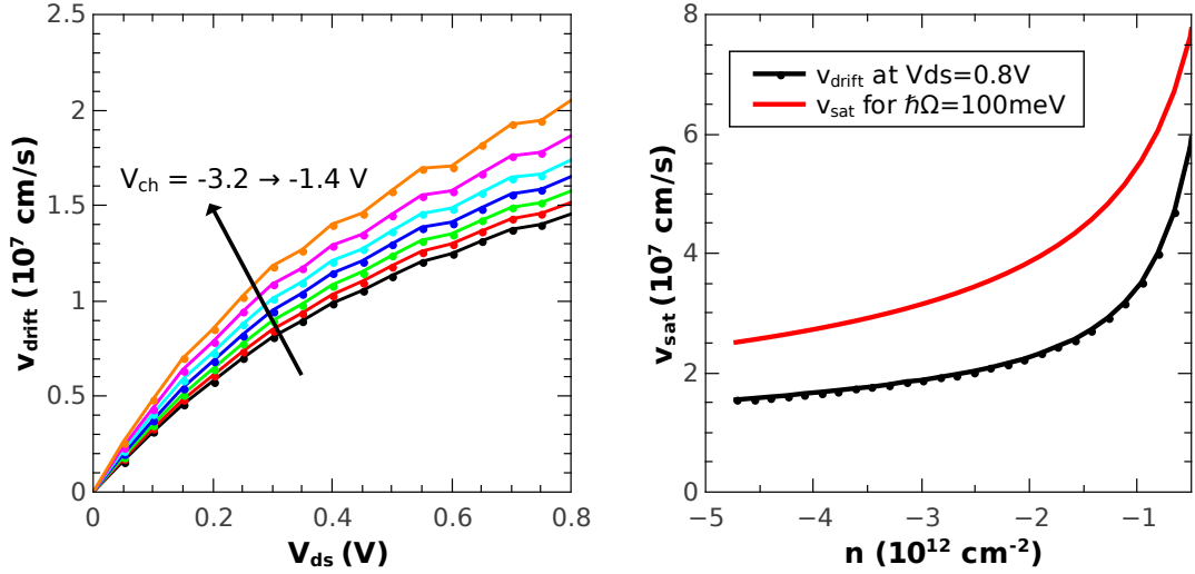
FIGURE 5.8: Left panel: Data of Fig. 5.7 replotted in terms of drift velocity v_d = I/(neW) (without fit). Right panel: Maximum measured drift velocity at V_{ds} = 0.8 V compared to the saturation velocity one would expect for a full saturation by hBN remote phonon scattering (Eq. (5.7)), as a function of the carrier density n . The low density region is not plotted as (5.7) is no longer valid for |n| < 0.4 \times 10^{12} \text{cm}^{-2}
