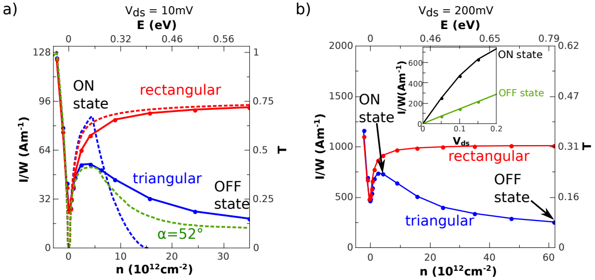
FIGURE 3.14: Influence of the barrier doping n on the current density I/W (and corresponding total transmission T ) for (a) V_{ds} = 10 \text{ mV} and (b) V_{ds} = 200 \text{ mV} . Solid lines (resp. dotted lines) correspond to NEGF simulations (resp. scattering calculations), red lines (resp. blue lines) correspond to the rectangular (resp. triangular) device. In panel (a) the scattering calculation for the rectangular device with sharp junctions (red dotted line) is in good agreement with NEGF. The scattering calculation for the triangular device with a smooth junction d = 10 \text{ nm} and opening angle \alpha = 52^\circ (green dotted line) is a way to take into account diffraction effects and compares well with NEGF simulations (blue solid line). Panel (b) inset: I/V_{ds} characteristics of the triangular transistor in the ON state n = 2 \times 10^{12} \text{ cm}^{-2} (black line) and in the OFF state n = 6 \times 10^{13} \text{ cm}^{-2} (green line).
