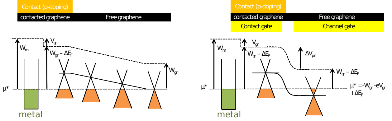
FIGURE 4.2: Graphene doping profile at the metal-graphene interface. Left : Long screening length in the absence of gating (100 nm according to [76]). Right : The contact gate controls the contact doping thanks to the absence of vertical screening and the channel gate sets the channel doping. The p-n junction length between contact and channel areas is controlled by the gate geometry.
