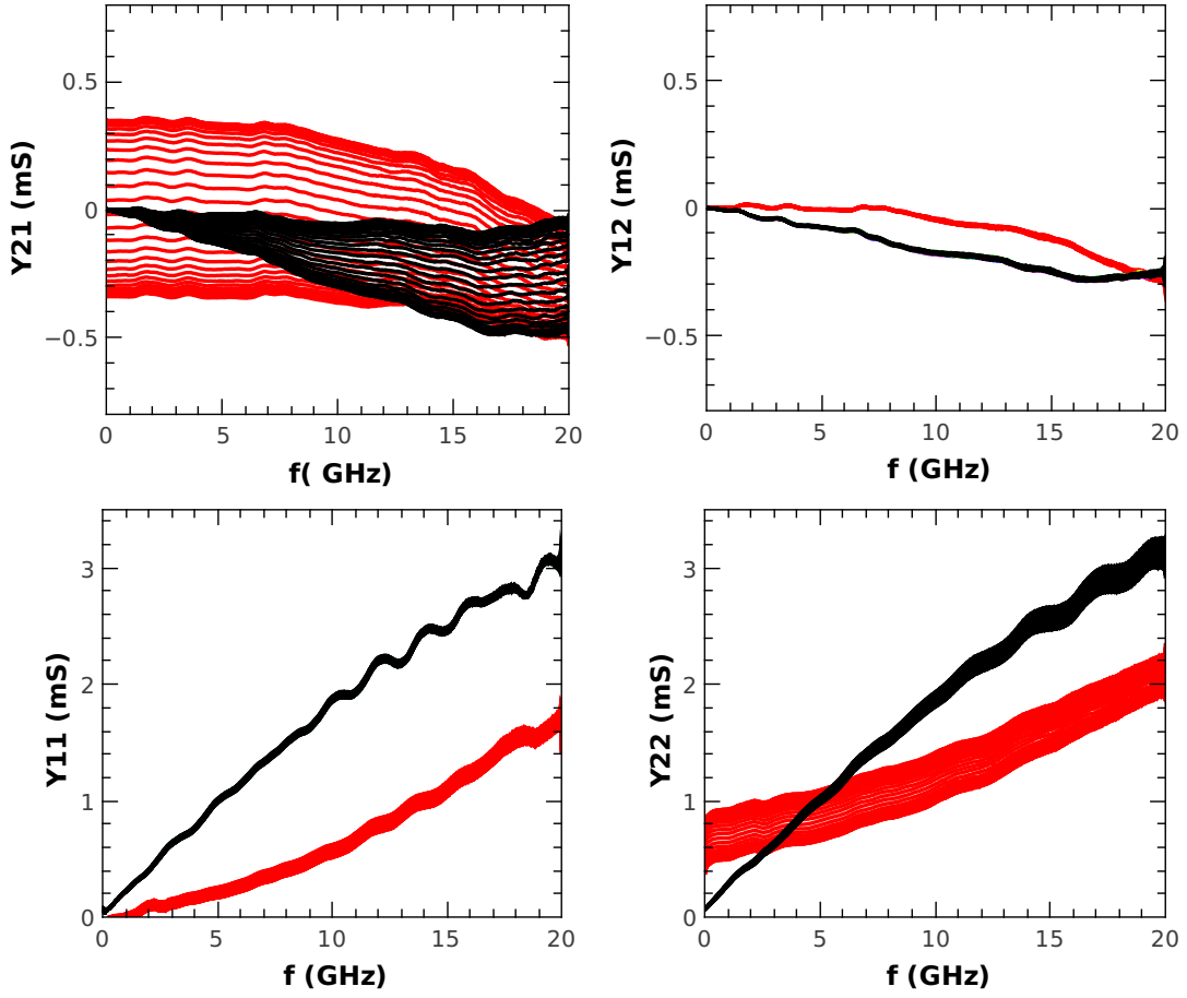
FIGURE 6.3: VNA measurement of the complex admittance parameters. The spectrum are the de-embedded Y-parameters ( Y - Y_{open} ), supposedly intrinsic, for various gate voltages. The red lines stand for the Y real parts and the black lines for the Y imaginary parts. The \Re(Y_{21}) spectra reflect the variation of the transconductance, \Re(Y_{22}) reflects the channel conductance. The \Im(Y_{21}) spectrum is linear and its slope corresponds to the gate capacitance. The slope of \Im(Y_{11}) and \Im(Y_{22}) is higher suggesting a remaining contribution of the parasitic capacitance.
