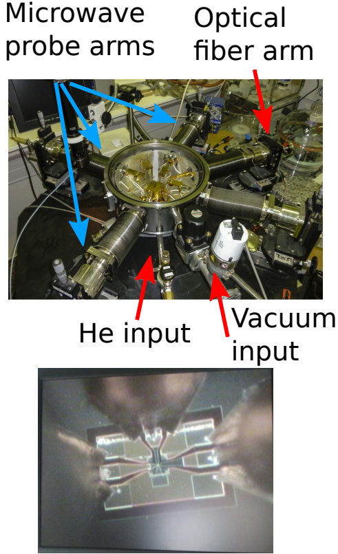
FIGURE 2.9: Top left: picture of the Janis probe station with the vacuum chamber open. Bottom left: picture of the device being measured. One can see the 3 RF probes on the CPW. Right: RF and DC measurement setup.
