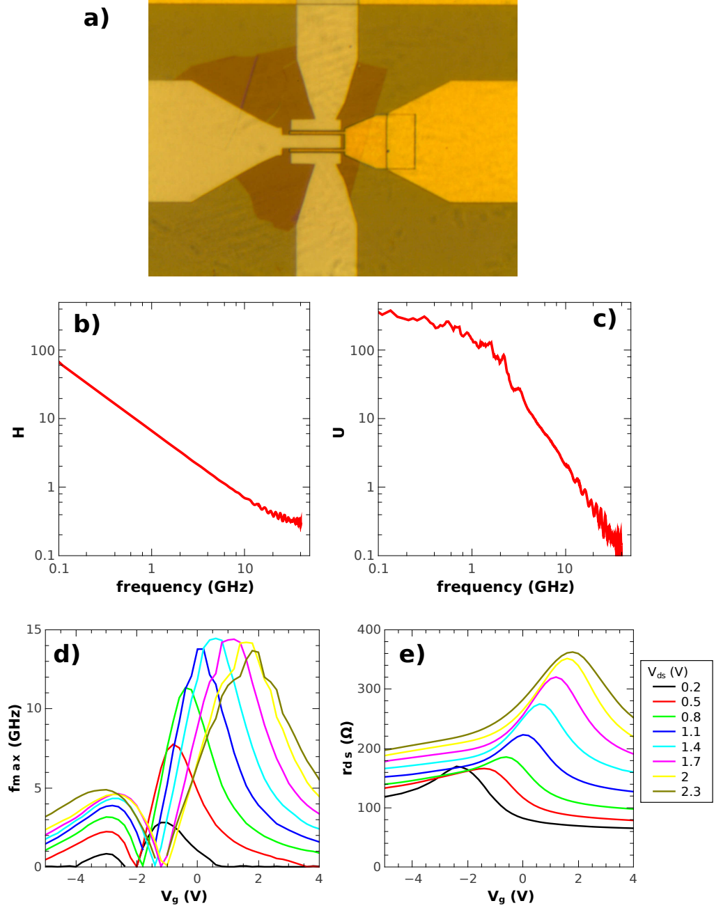
FIGURE 6.7: (a) Optimized graphene RF transistor with thick ( 200\text{ nm} ) Au double gates ( W = 10\text{ }\mu\text{m} , L = 300\text{ nm} ) fabricated by M. Boukhicha. (b) Current and (c) Mason gains at V_g = 1\text{ V} and V_{ds} = 1.5\text{ V} without de-embedding. We obtain f_t \approx 7\text{ GHz} and f_{max} \approx 14\text{ GHz} (d) f_{max} and (e) r_{ds} as a function of the gate voltage for V_{ds} = 0 \rightarrow 2.3\text{ V} . The device is driven on the low contact resistance side and with positive V_{ds} to take advantage of the pinch-off effect ( V_g = 1\text{ V} , V_{ds} = 1.5\text{ V} ).
