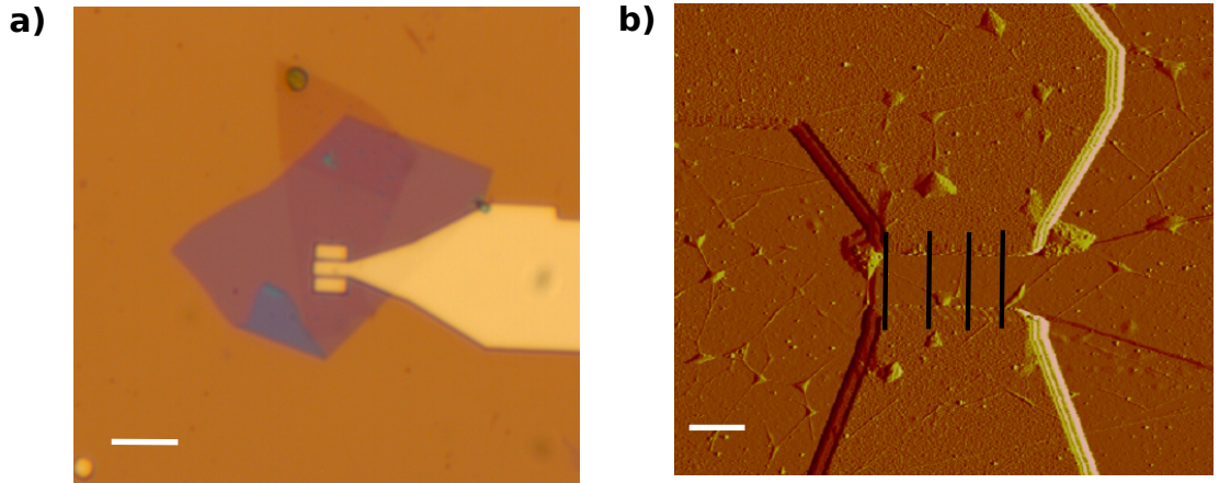
FIGURE B.1: (a) Optical image before the contact deposition and channel etching. The white scale bar is 5\,\mu\text{m} . (b) AFM scan of the contacted device. The black lines indicate the position of the channels etching. The white scale bar is 1\,\mu\text{m} .
