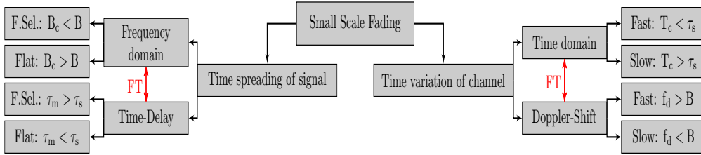
Figure 1.2: Fading channel classification
