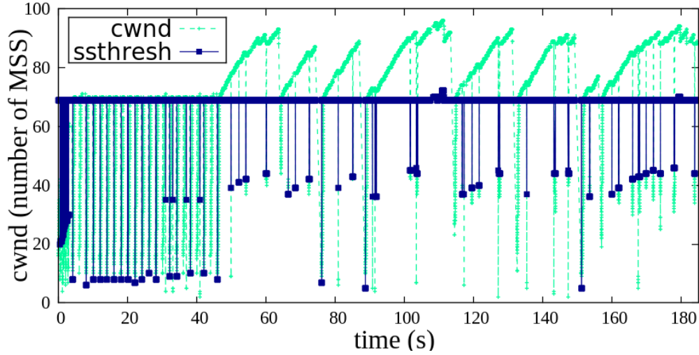
Figure 5.1 – Cwnd variation of {NewReno HTBM} ( IS = 5.48\% , IF = 35.68\% , V = 180s , fr_{\widehat{OFF}} = 0.2 , CNG = 43.33 )
