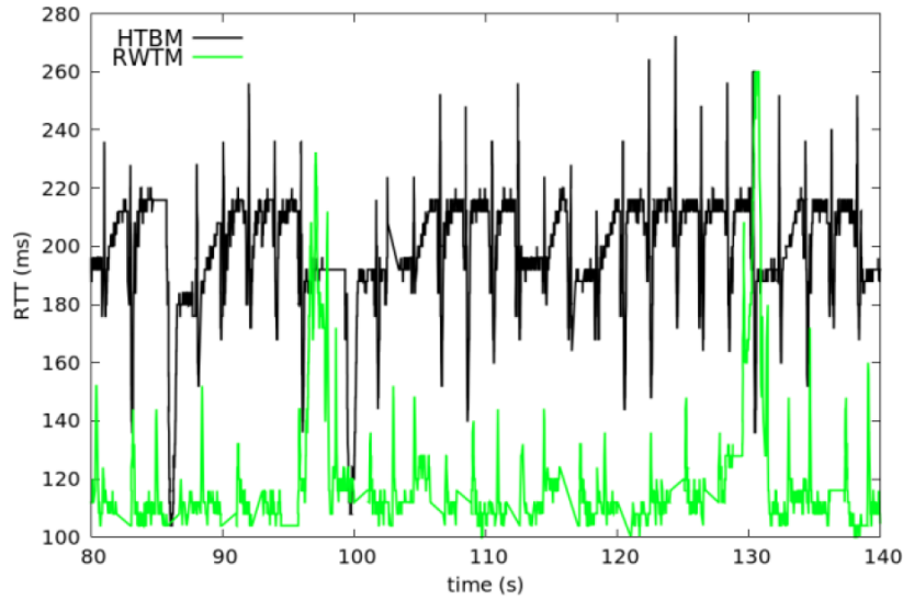
Figure 4.5 – RTT_{1-S} variation
