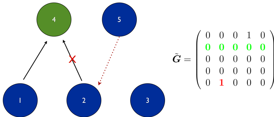
Figure 5.4: Row-wise relaxation: newly predictive covariate cannot be regressed anymore.
