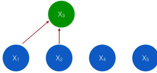
Figure 4.1: The bipartite graph associated to the running example. \mathbf{X}_r is green and \mathbf{X}_f is blue.
