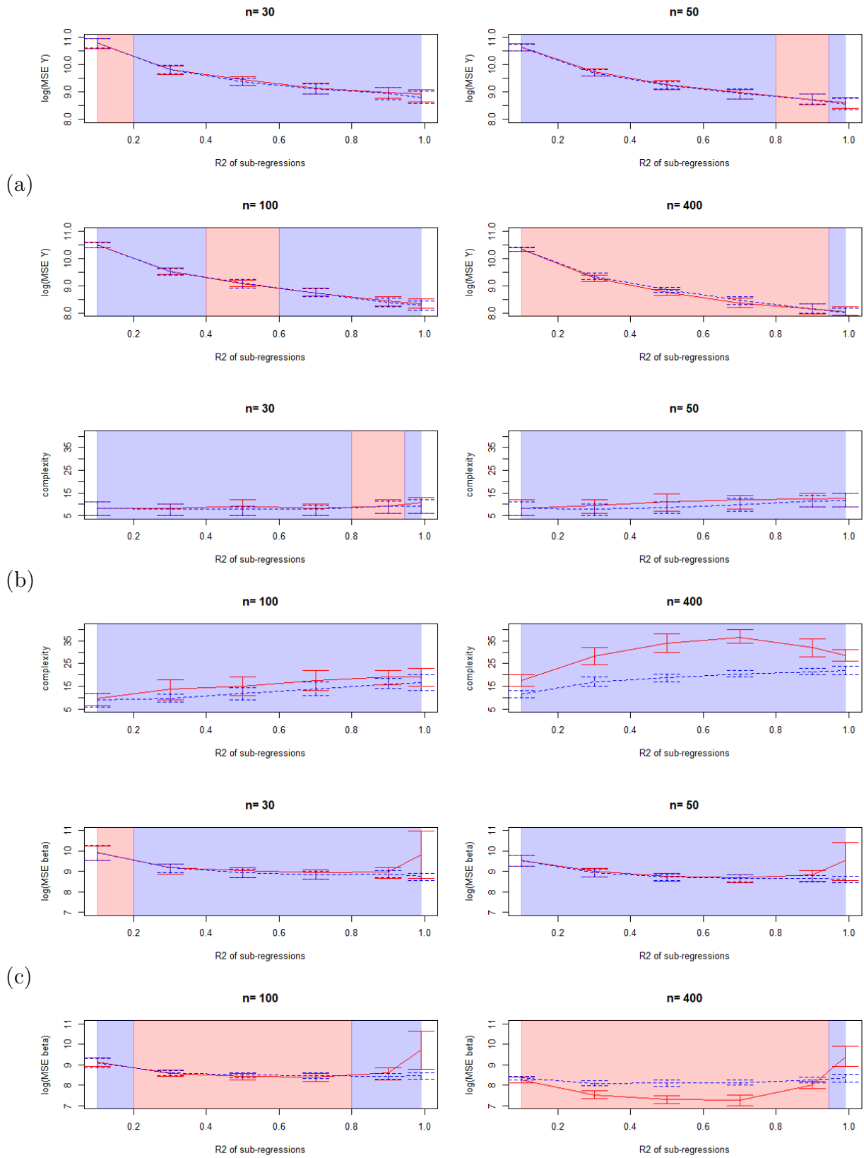
Figure 6.7: Comparison of the MSE on \hat{Y} (a), complexities (b) and MSE on \hat{\beta} (c), red=classical (complete) model, blue=marginal model
