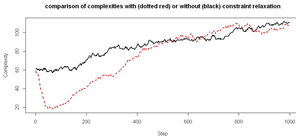
Figure 5.10: Comparison of complexity evolution with or without constraint relaxation.
