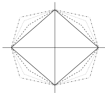
Figure 3.14: Geometric view of the Penalty for OSCAR
