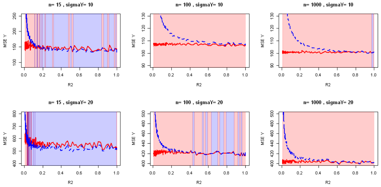
Figure 4.9: Evolution of observed Mean Squared error on \hat{\mathbf{Y}}_{stepwise} with the strength of the correlations for various sample sizes and strength of regression. d = 5 covariates.
