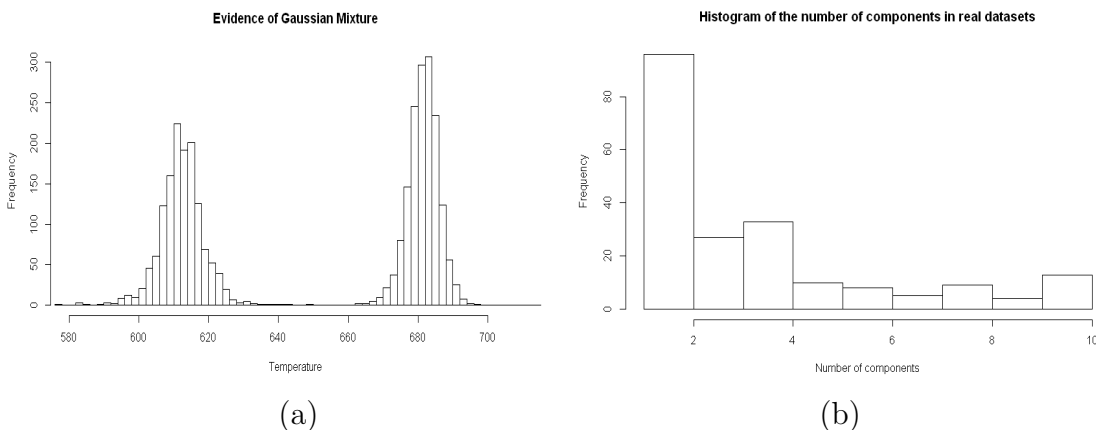
Figure 7.2: Quality case study: (a) Example of a non-Gaussian real variable easily modeled by a Gaussian mixture, (b) distribution of the number of components found for each covariate.
