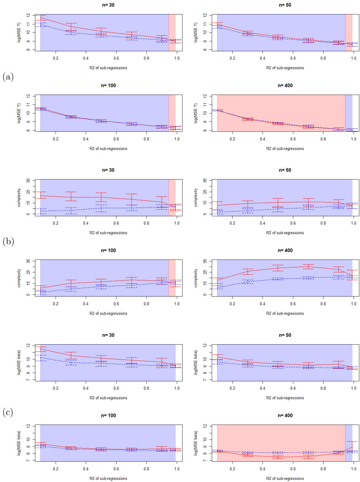
Figure 4.15: Comparison of the MSE on \hat{Y} (a), complexities (b) and MSE on \hat{\beta} (c), plain red=classical (complete) model, dashed blue=marginal model
