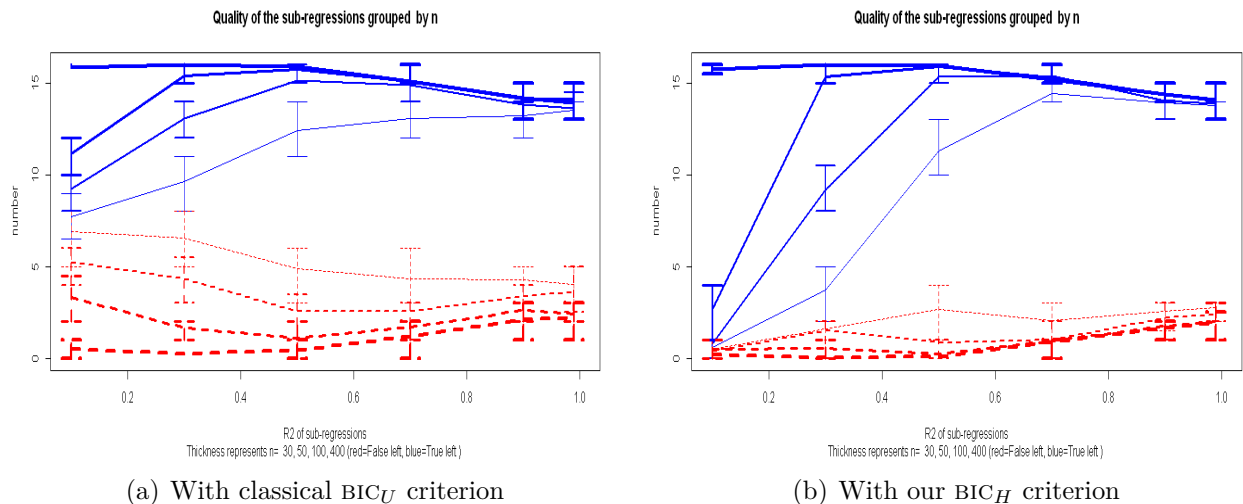
Figure 6.1: Quality of the sub-regressions found by the MCMC. True left (plain blue) and Wrong left (dotted red) for n varying in (30, 50, 100, 400), the thicker the greater n .
