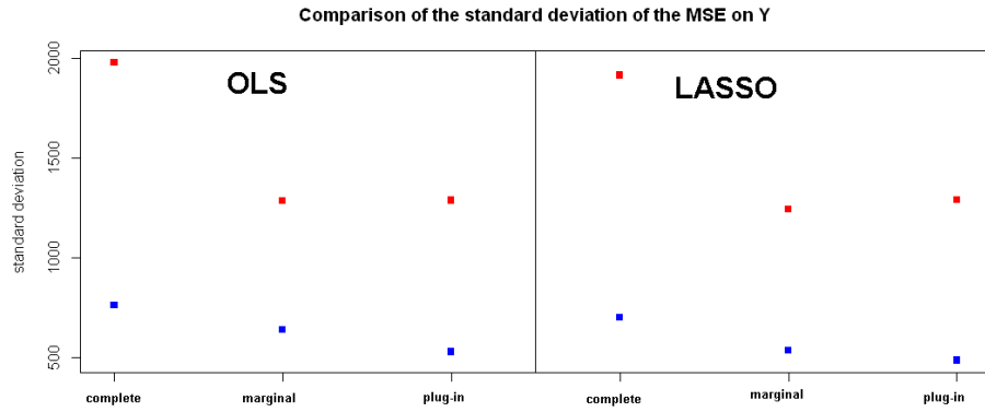
Figure 9.5: our Stochastic EM (blue) provides more robust results than imputation by the mean (red) but the variances are still too wide.
