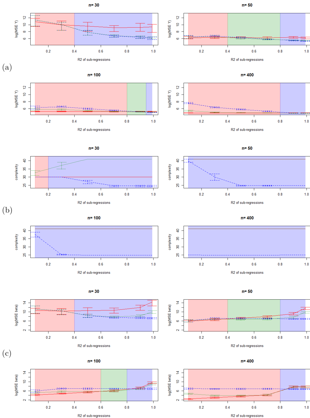
Figure 8.12: Comparison of the MSE on \hat{Y} (a), complexities (b) and MSE on \hat{\beta} (c), plain red=classical (complete) model, dashed blue=marginal model, dotted green=plug-in model.
