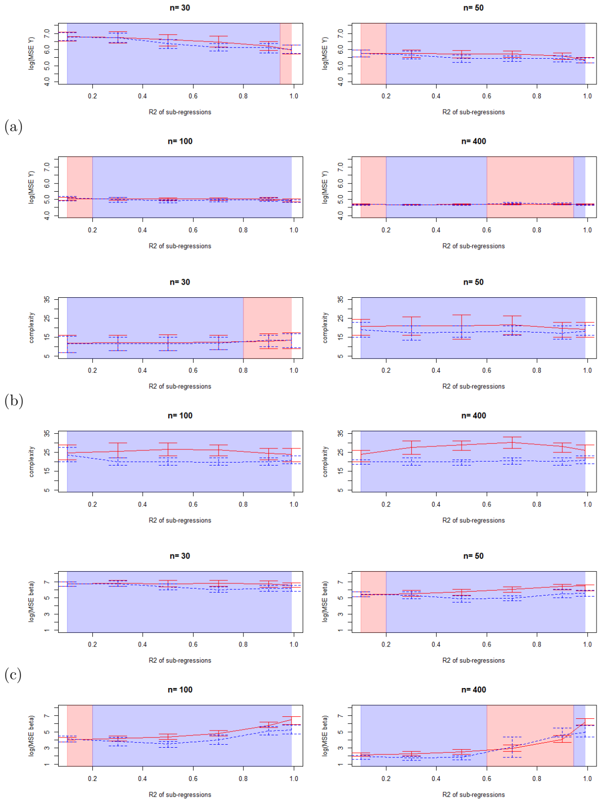
Figure 6.13: Comparison of the MSE on \hat{Y} (a), complexities (b) and MSE on \hat{\beta} (c), red=classical (complete) model, blue=marginal model
