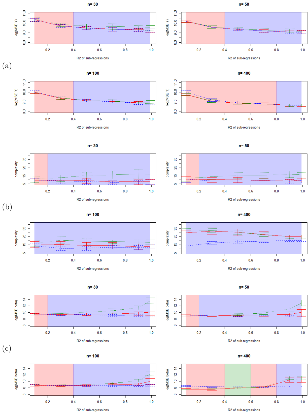
Figure 8.4: Comparison of the MSE on \hat{Y} (a), complexities (b) and MSE on \hat{\beta} (c), plain red=classical (complete) model, dashed blue=marginal model, dotted green=plug-in model.
