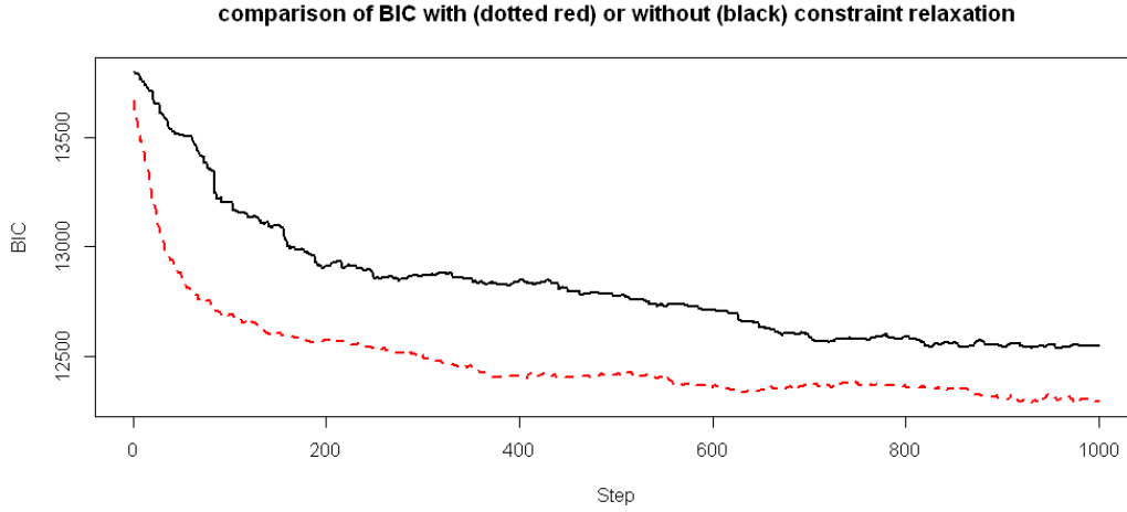
Figure 5.11: Comparison of BIC evolution with or without constraint relaxation.
