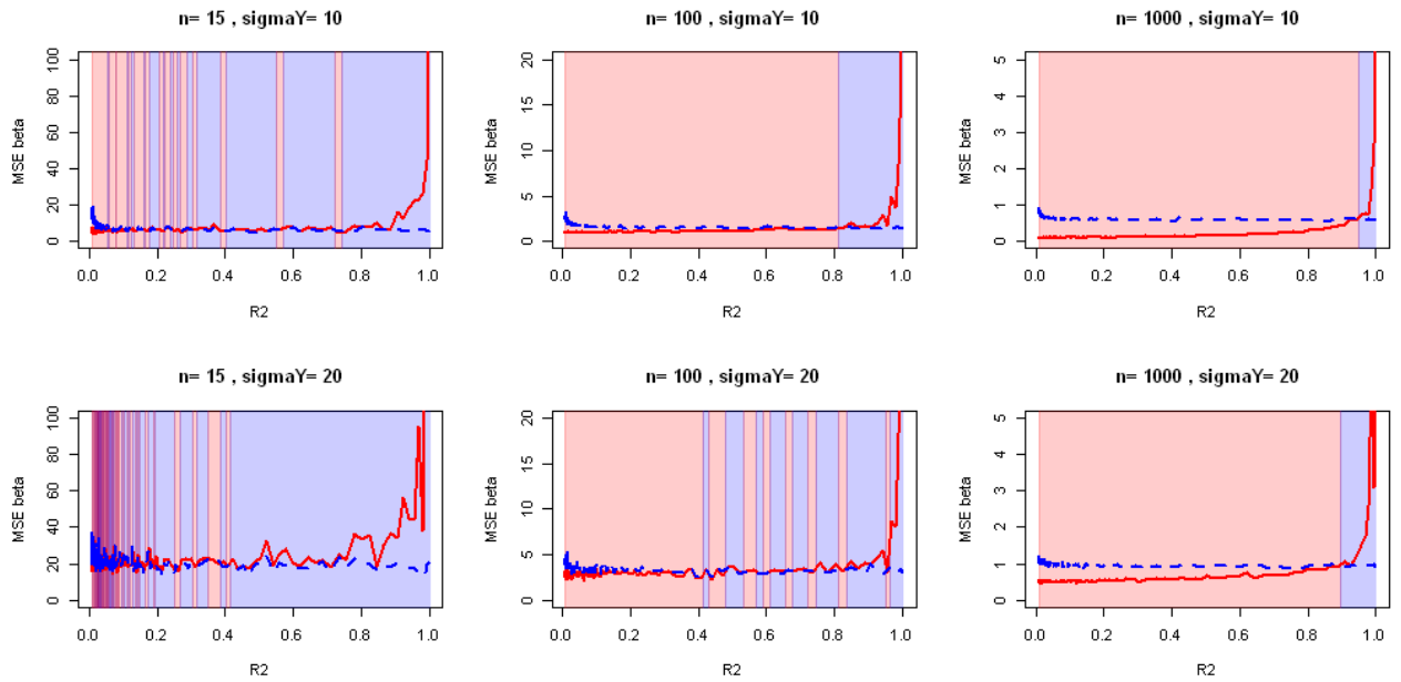
Figure 4.4: Observed MSE on \hat{\beta} of LASSO with LAR on both \mathbf{X} (red) and CorReg's marginal \mathbf{X}^{I_f} (blue) for varying R^2 of the sub-regression, n and \sigma_Y . d = 5 covariates.
