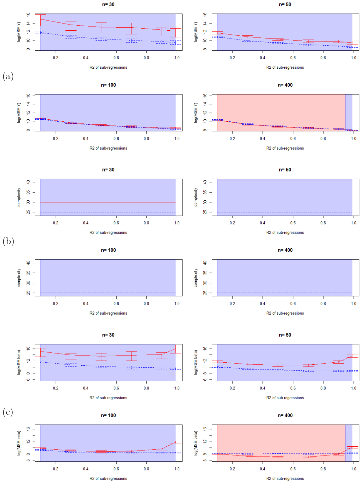
Figure 4.12: Comparison of the MSE on \hat{Y} (a), complexities (b) and MSE on \hat{\beta} (c), plain red=classical (complete) model, dashed blue=marginal model
