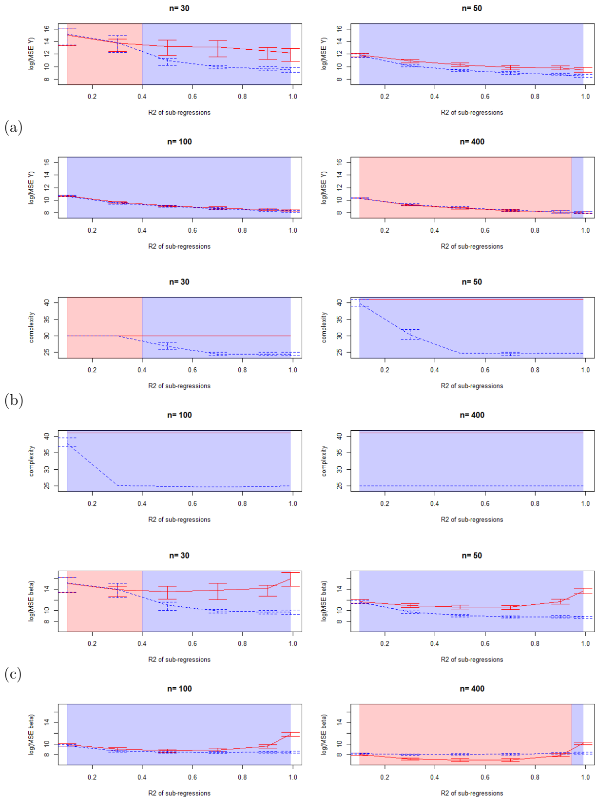
Figure 6.5: Comparison of the MSE on \hat{Y} (a), complexities (b) and MSE on \hat{\beta} (c), red=classical (complete) model, blue=marginal model
