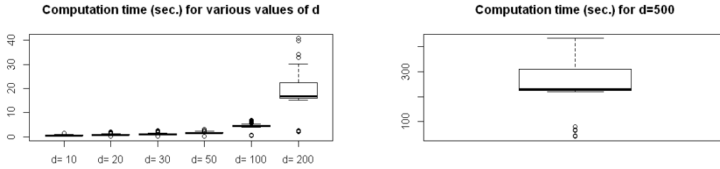
Figure 6.3: Evolution of the mean time for 10 times 1 000 steps of the MCMC, 40 candidates each time (constraint relaxation). d_r = 0.4 \times d sub-regressions, n = 30 .
