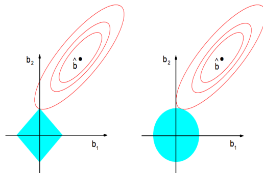
Figure 3.8: Geometric view of the Penalty for the LASSO (left) compared to ridge regression (right) as shown in the book from Hastie [Hastie et al., 2009]
