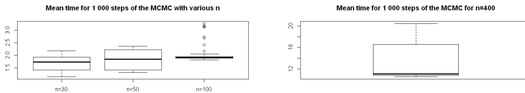
Figure 6.2: Evolution of the mean time for 10 times 1 000 steps of the MCMC, 39 candidates each time (constraint relaxation). d = 40 covariates with d_r = 16 sub-regressions
