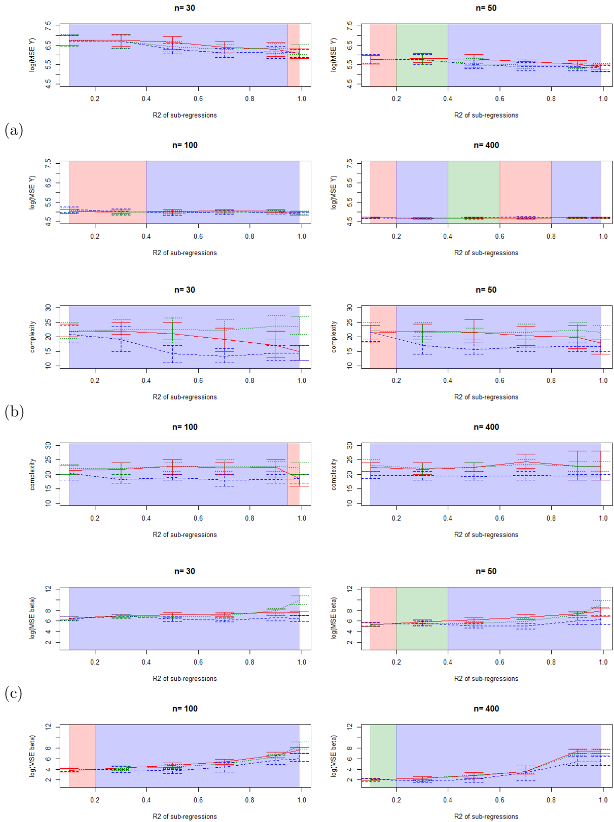
Figure 8.10: Comparison of the MSE on \hat{Y} (a), complexities (b) and MSE on \hat{\beta} (c), plain red=classical (complete) model, dashed blue=marginal model, dotted green=plug-in model.
