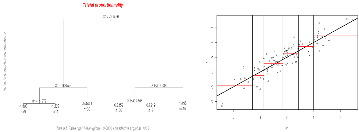
(a) Tree found for the trivial case
