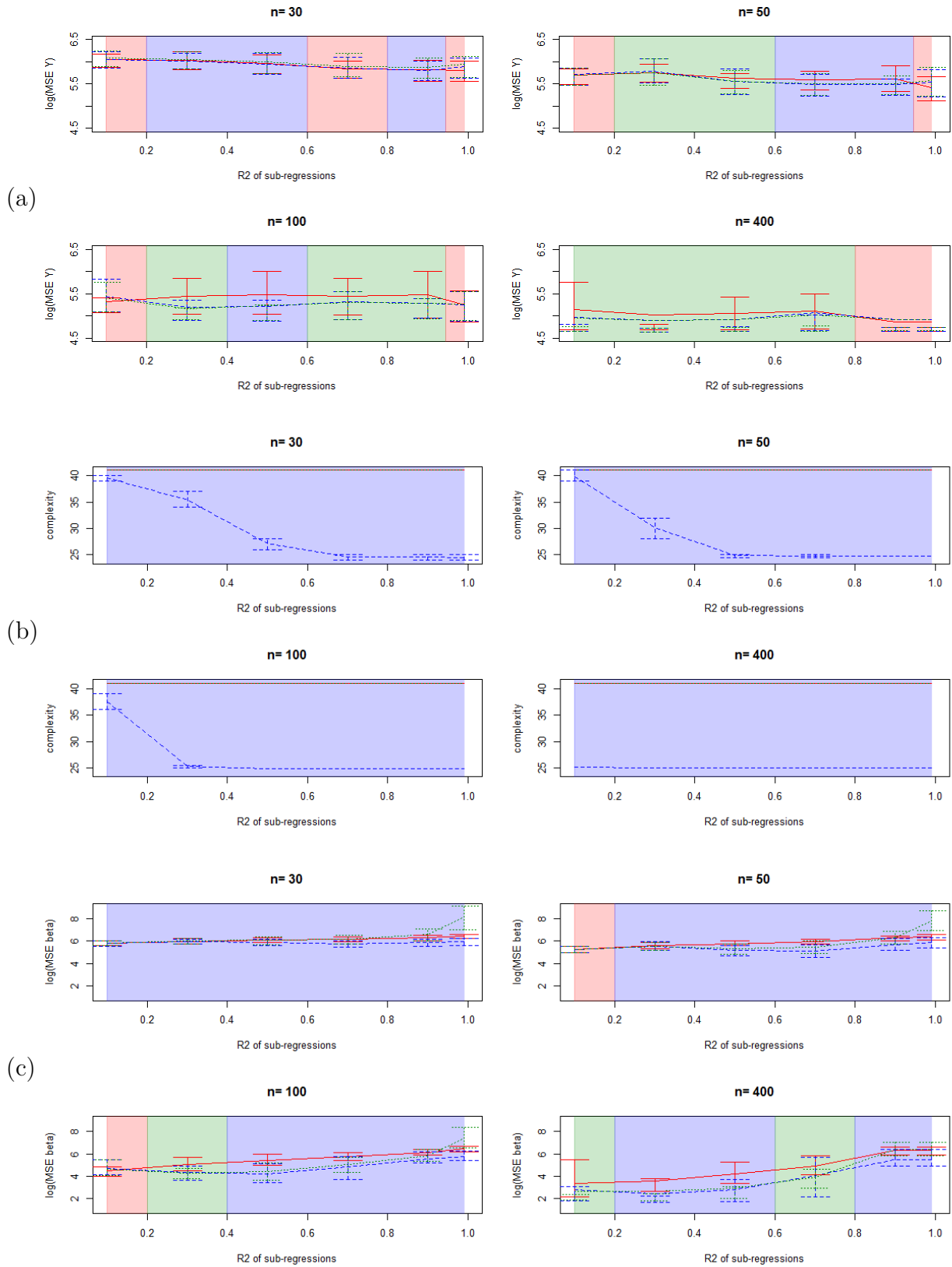
Figure 8.11: Comparison of the MSE on \hat{Y} (a), complexities (b) and MSE on \hat{\beta} (c), plain red=classical (complete) model, dashed blue=marginal model, dotted green=plug-in model.
