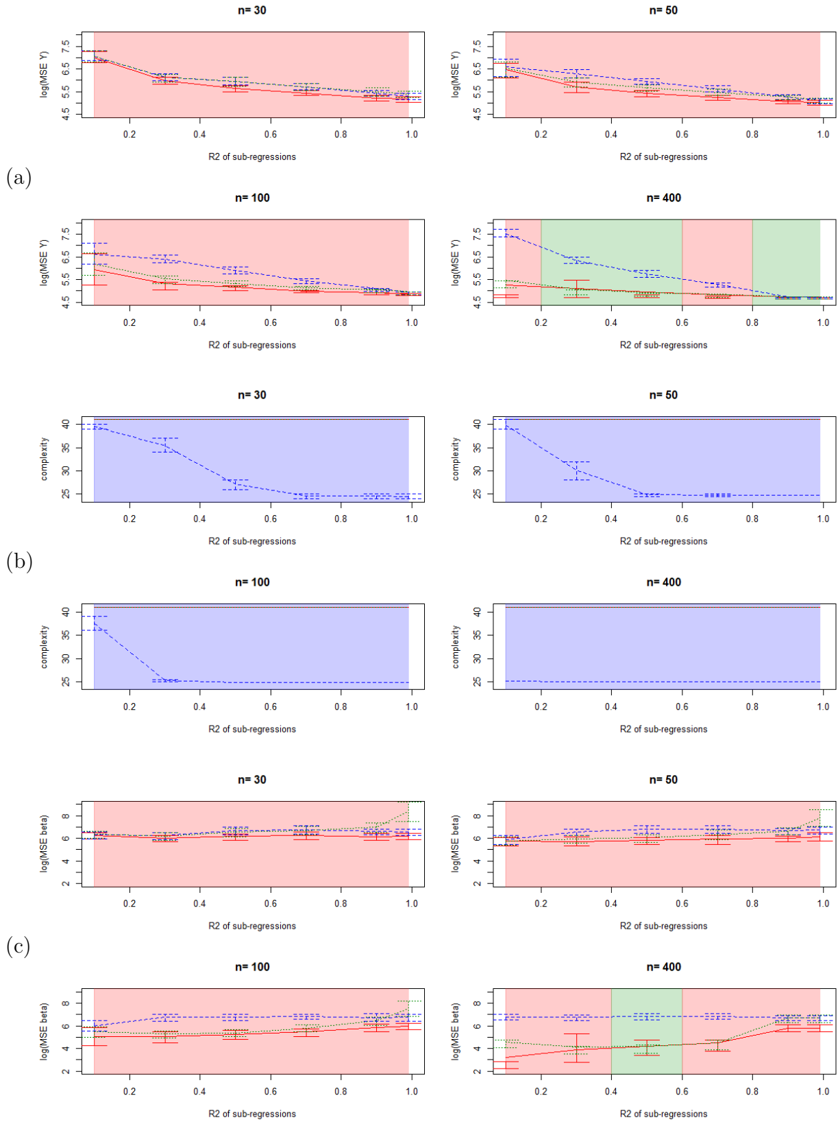
Figure 8.16: Comparison of the MSE on \hat{Y} (a), complexities (b) and MSE on \hat{\beta} (c), plain red=classical (complete) model, dashed blue=marginal model, dotted green=plug-in model.
