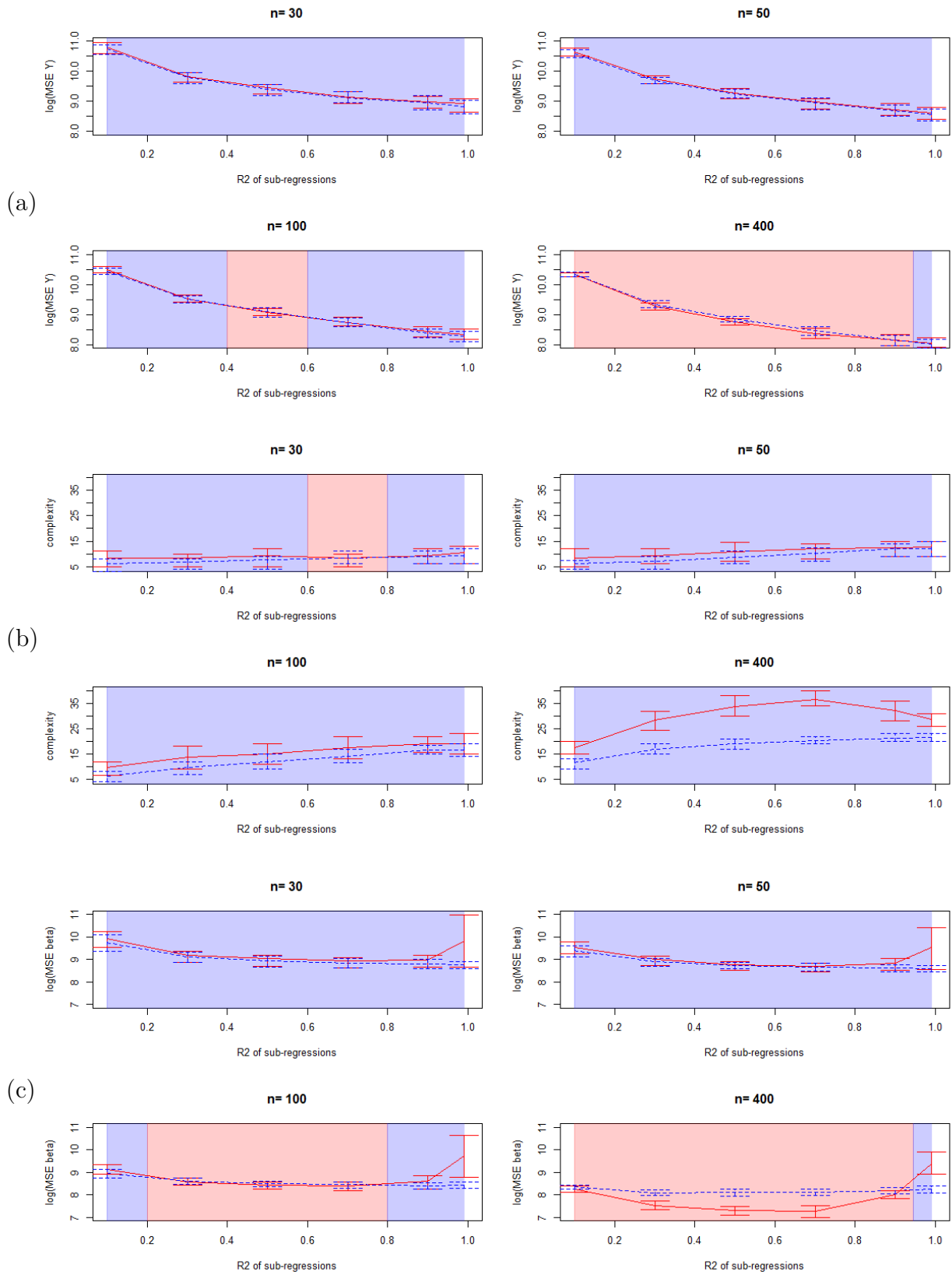
Figure 4.14: Comparison of the MSE on \hat{Y} (a), complexities (b) and MSE on \hat{\beta} (c), plain red=classical (complete) model, dashed blue=marginal model
