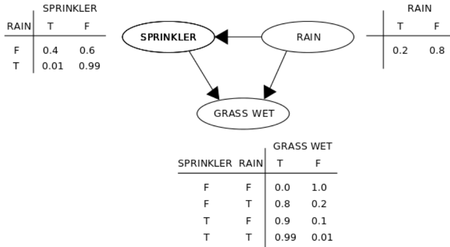
Figure 3.1: Simple Bayesian network and its probability tables. Public domain image.
