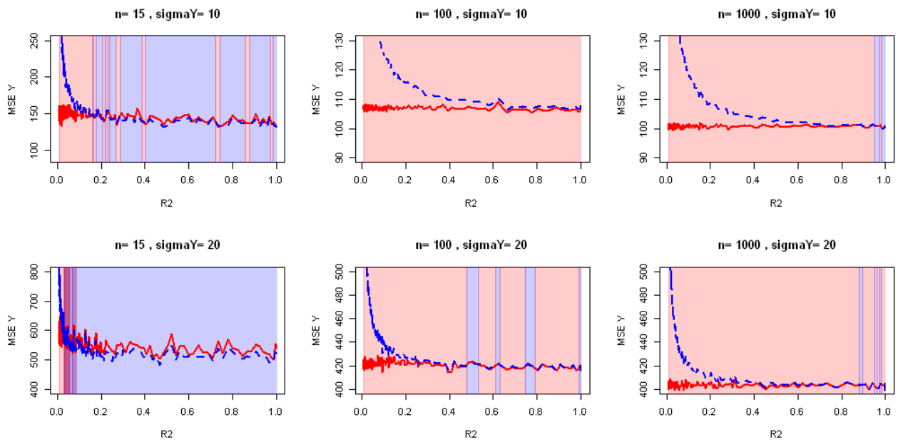
Figure 4.5: Evolution of observed Mean Squared error on \hat{Y}_{LASSO} with the strength of the correlations for various sample sizes and strength of regression. d = 5 covariates.
