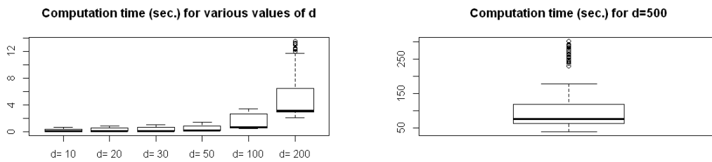
Figure 6.4: Evolution of the mean time for 10 times 1 000 steps of the MCMC, 40 candidates each time (without constraint relaxation). d_r = 0.4 \times d sub-regressions, n = 30 .
