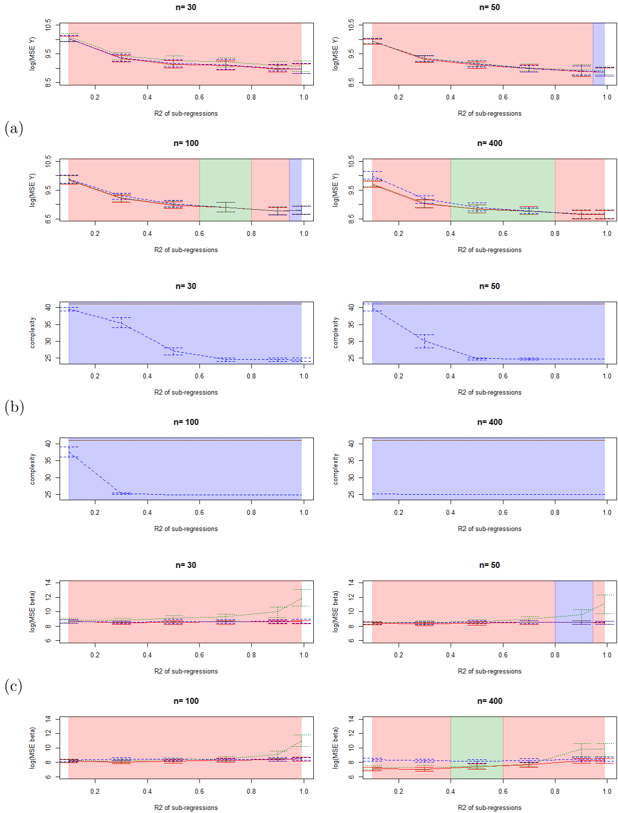
Figure 8.6: Comparison of the MSE on \hat{Y} (a), complexities (b) and MSE on \hat{\beta} (c), plain red=classical (complete) model, dashed blue=marginal model, dotted green=plug-in model.
