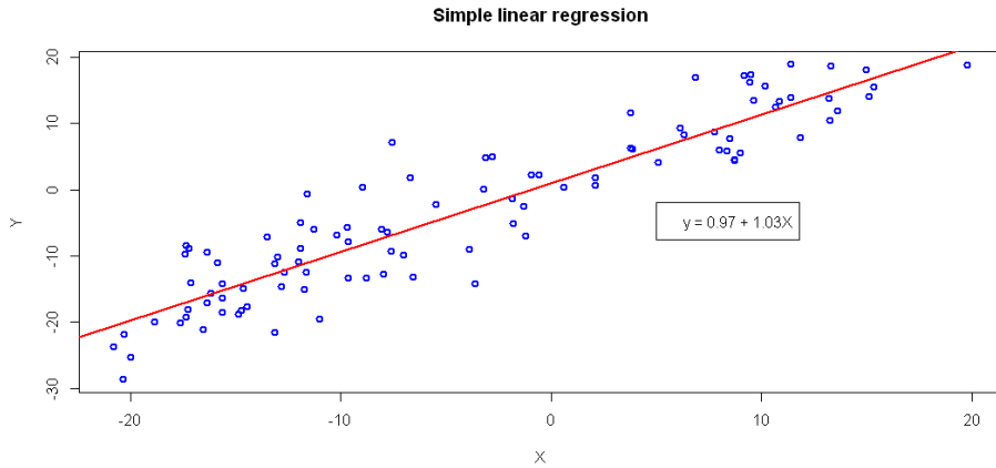
Figure 1.3: An example of simple linear regression
