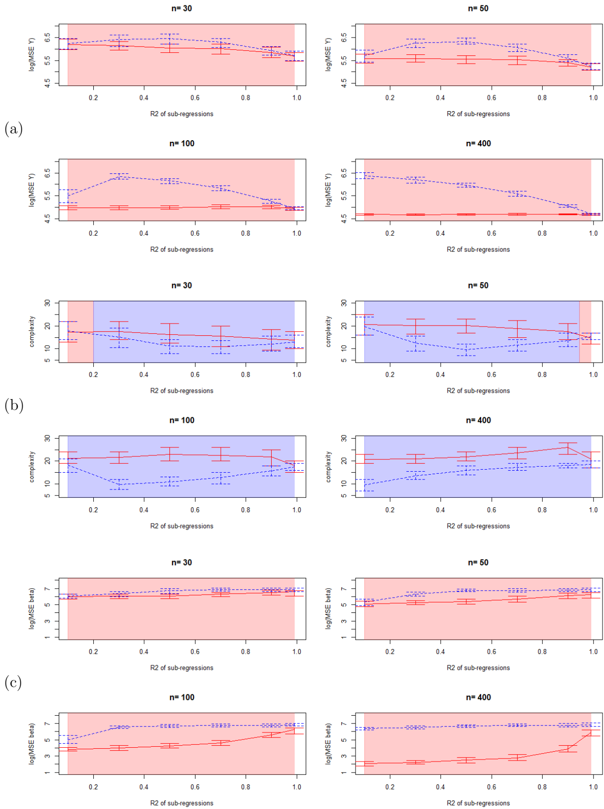
Figure 6.16: Comparison of the MSE on \hat{Y} (a), complexities (b) and MSE on \hat{\beta} (c), red=classical (complete) model, blue=marginal model
