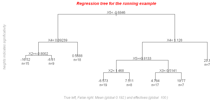
Figure 3.2: Regression tree obtain with the package CorReg (graphical layer on top of the rpart package) on the running example.
