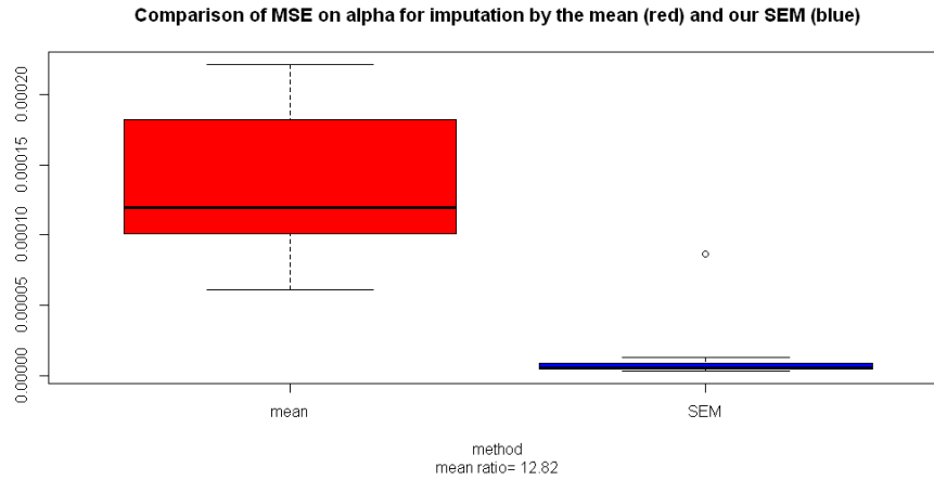
Figure 9.2: MSE on \alpha is significantly lower and with smaller variance with our Stochastic EM than with imputation by the mean.
