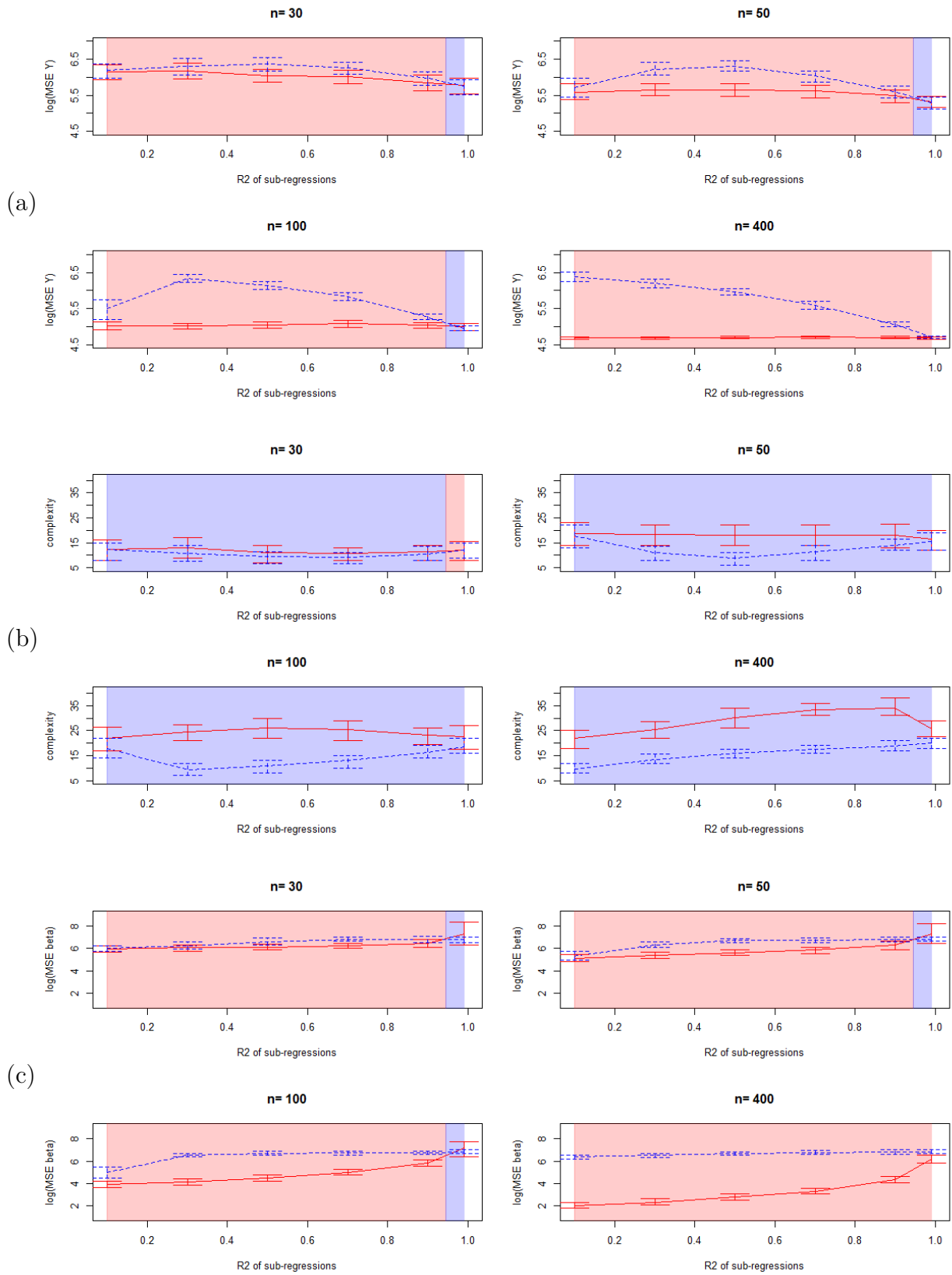
Figure 6.17: Comparison of the MSE on \hat{Y} (a), complexities (b) and MSE on \hat{\beta} (c), red=classical (complete) model, blue=marginal model
