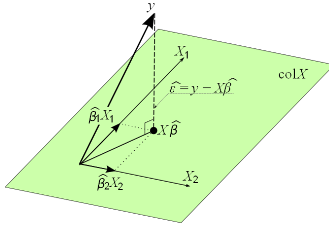
Figure 3.4: Multiple linear regression with Ordinary Least Squares seen as a projection on the d -dimensional hyperplane spanned by the regressors \mathbf{X} . Public domain image.
