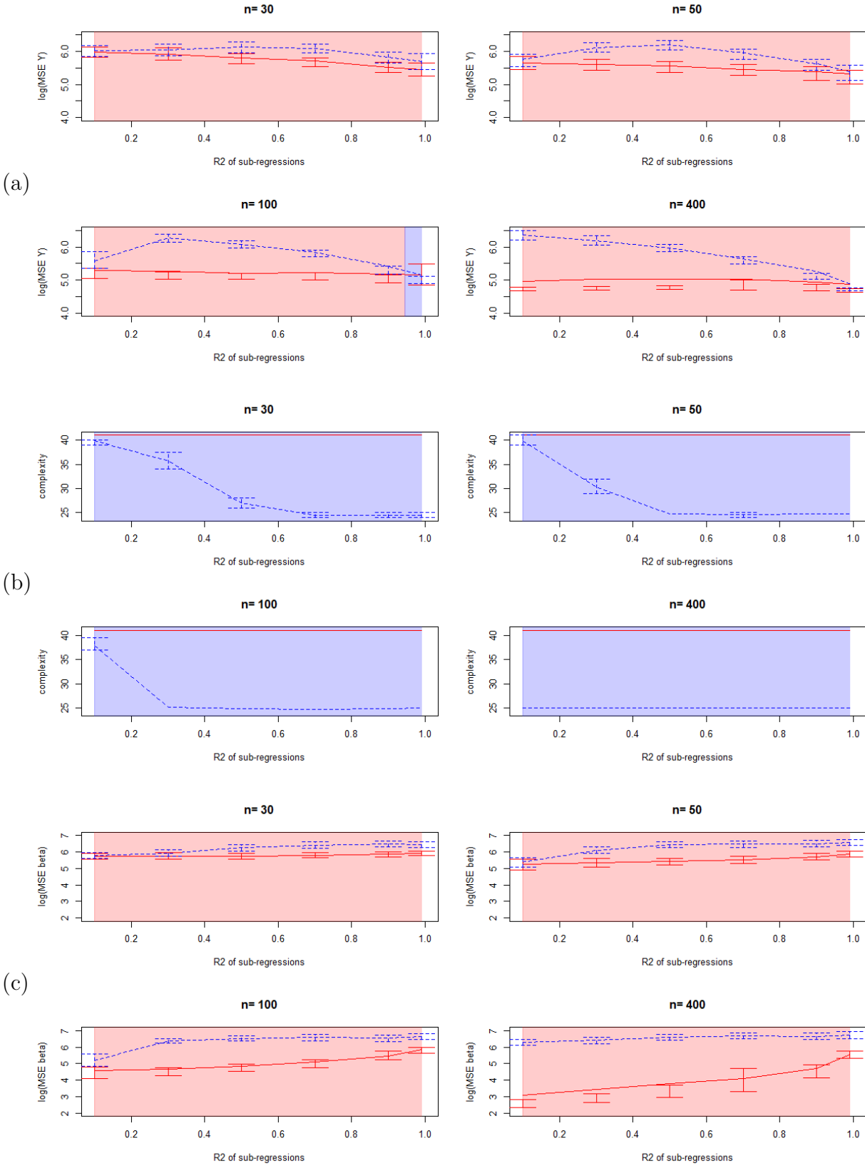
Figure 6.19: Comparison of the MSE on \hat{Y} (a), complexities (b) and MSE on \hat{\beta} (c), red=classical (complete) model, blue=marginal model
