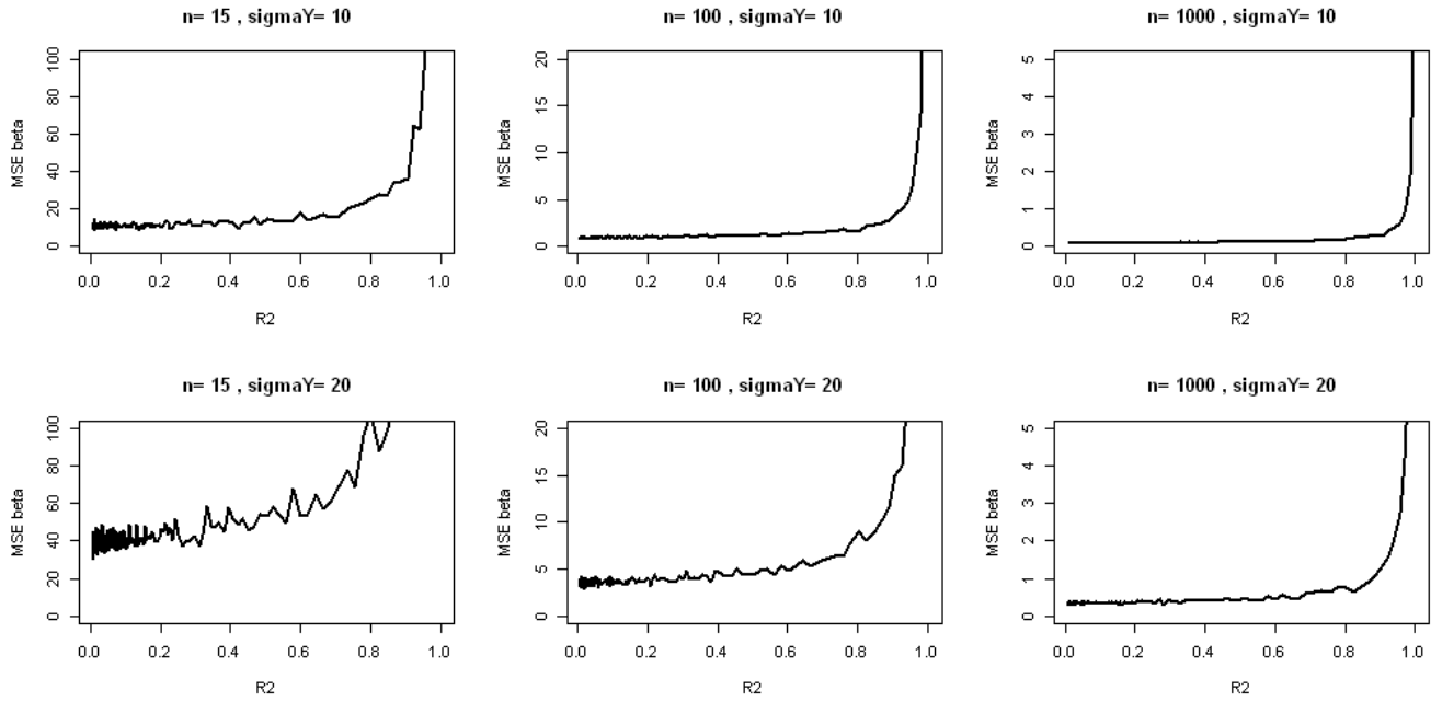
Figure 3.5: Evolution of observed Mean Squared error on \hat{\beta}_{OLS} with the strength of the correlations for various sample sizes and strength of regression. d = 5 covariates (running example).
