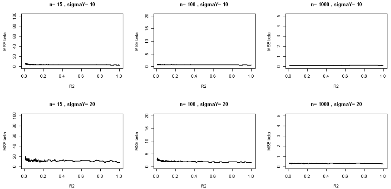
Figure 3.6: Evolution of observed Mean Squared error on \hat{\beta}_{ridge} with the strength of the correlations for various sample sizes and strength of regression. d = 5 covariates.
