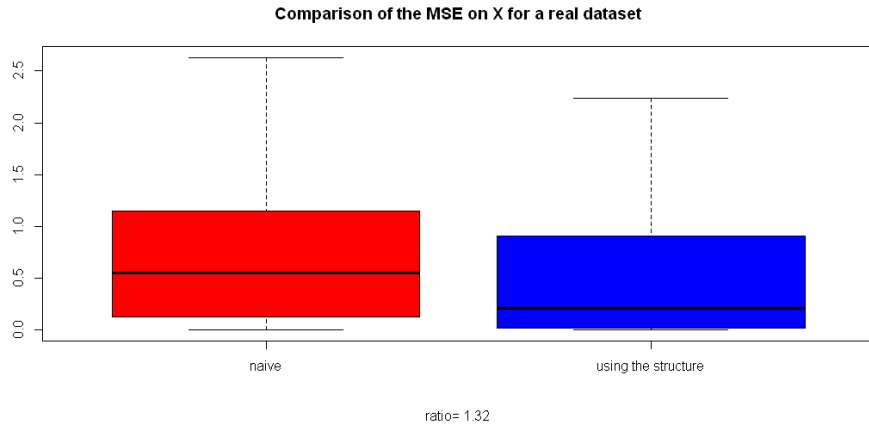
Figure 9.7: MSE on \hat{\mathbf{X}} is 1.32 times lower in mean when using our method (blue) than with imputation by the mean (red).
