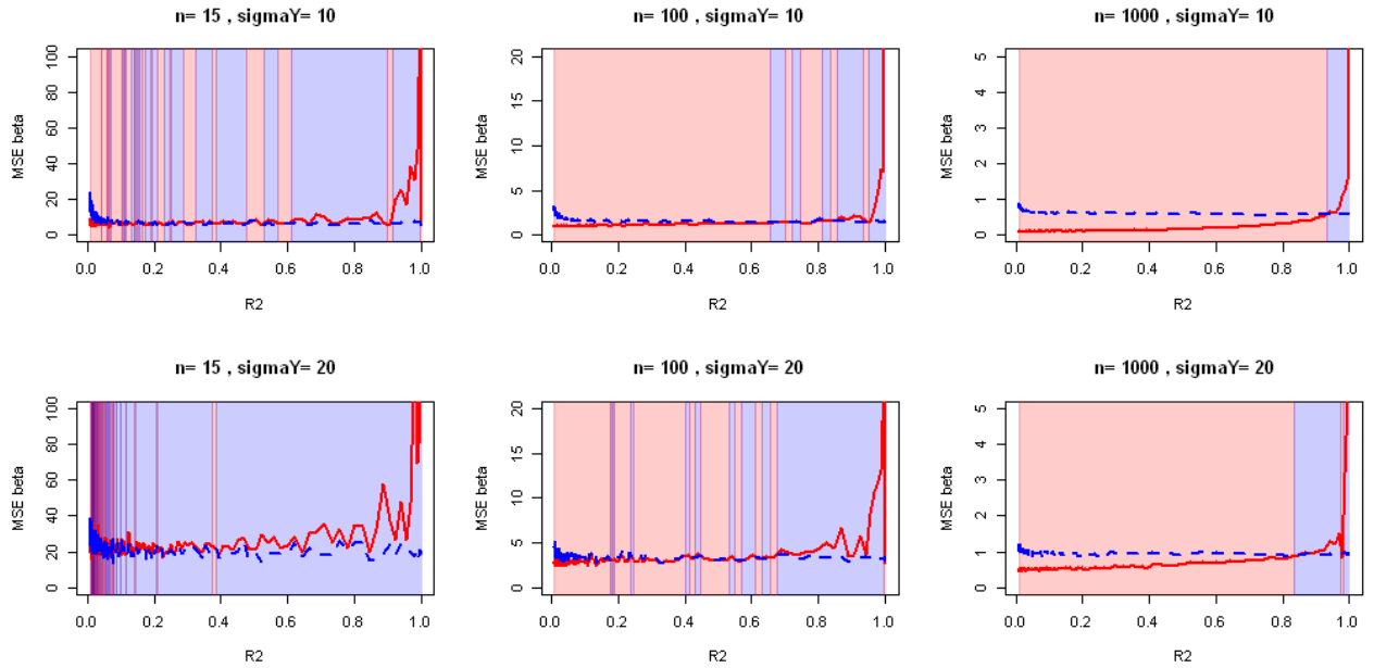
Figure 4.8: Observed MSE on \hat{\beta}_{stepwise} on both \mathbf{X} (red) and CorReg's marginal \mathbf{X}_f (blue) for varying R^2 of the sub-regression, n and \sigma_Y . d = 5 covariates.
