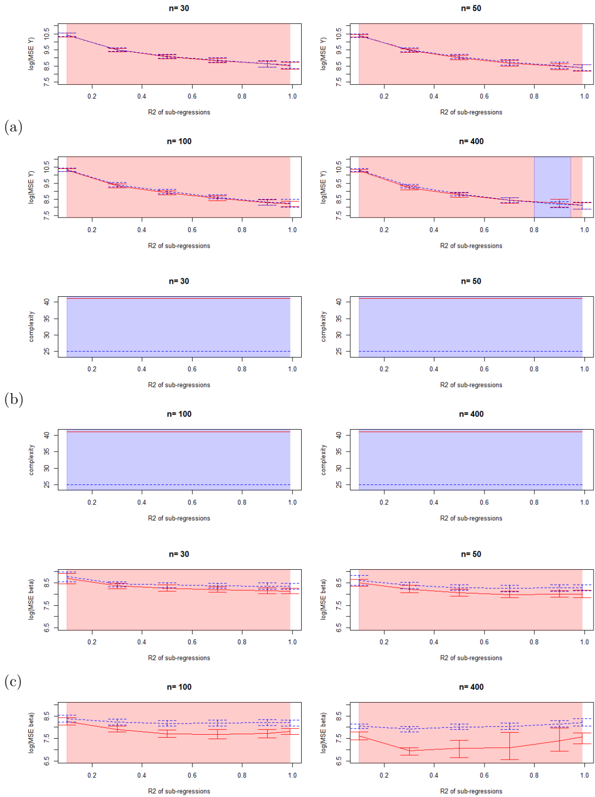
Figure 4.16: Comparison of the MSE on \hat{Y} (a), complexities (b) and MSE on \hat{\beta} (c), plain red=classical (complete) model, dashed blue=marginal model
