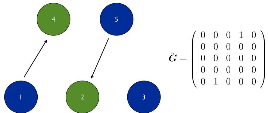
Figure 5.5: We get a feasible candidate \tilde{\mathbf{S}} = ((2, 4), (\{5\}, \{1\})) that does differ from \mathbf{S} in many points.
