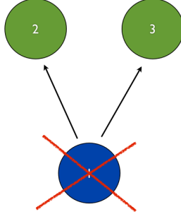
Figure 9.1: Pattern of missing values that does not allow to use equation (9.2): one missing value for a covariate that is common to 2 observed response covariates.
