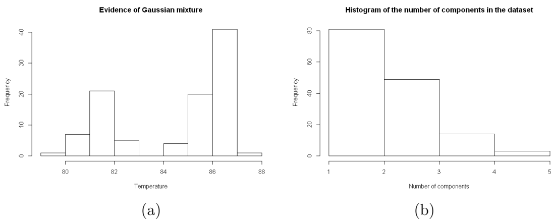
Figure 7.4: Production case study: (a) Example of a non-Gaussian real variable easily modeled by a Gaussian mixture, (b) distribution of the number of components found for each covariate.
