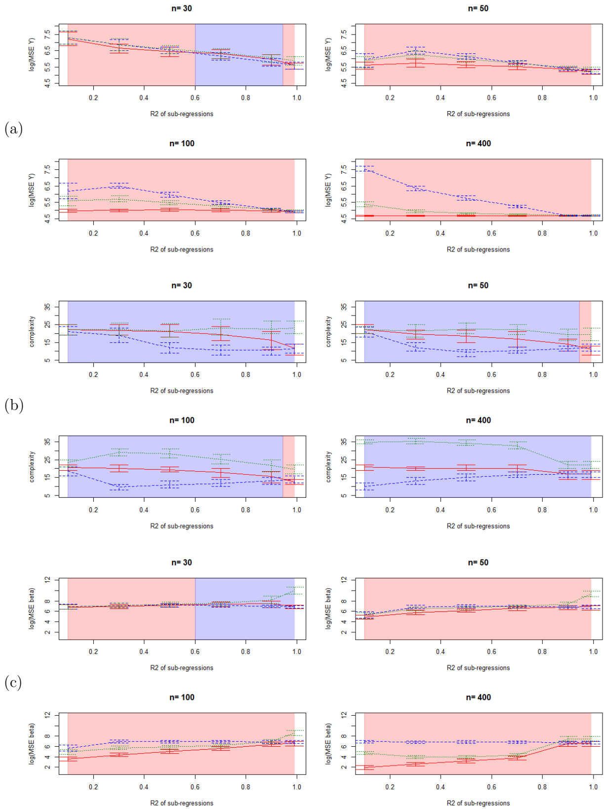
Figure 8.15: Comparison of the MSE on \hat{Y} (a), complexities (b) and MSE on \hat{\beta} (c), plain red=classical (complete) model, dashed blue=marginal model, dotted green=plug-in model.
