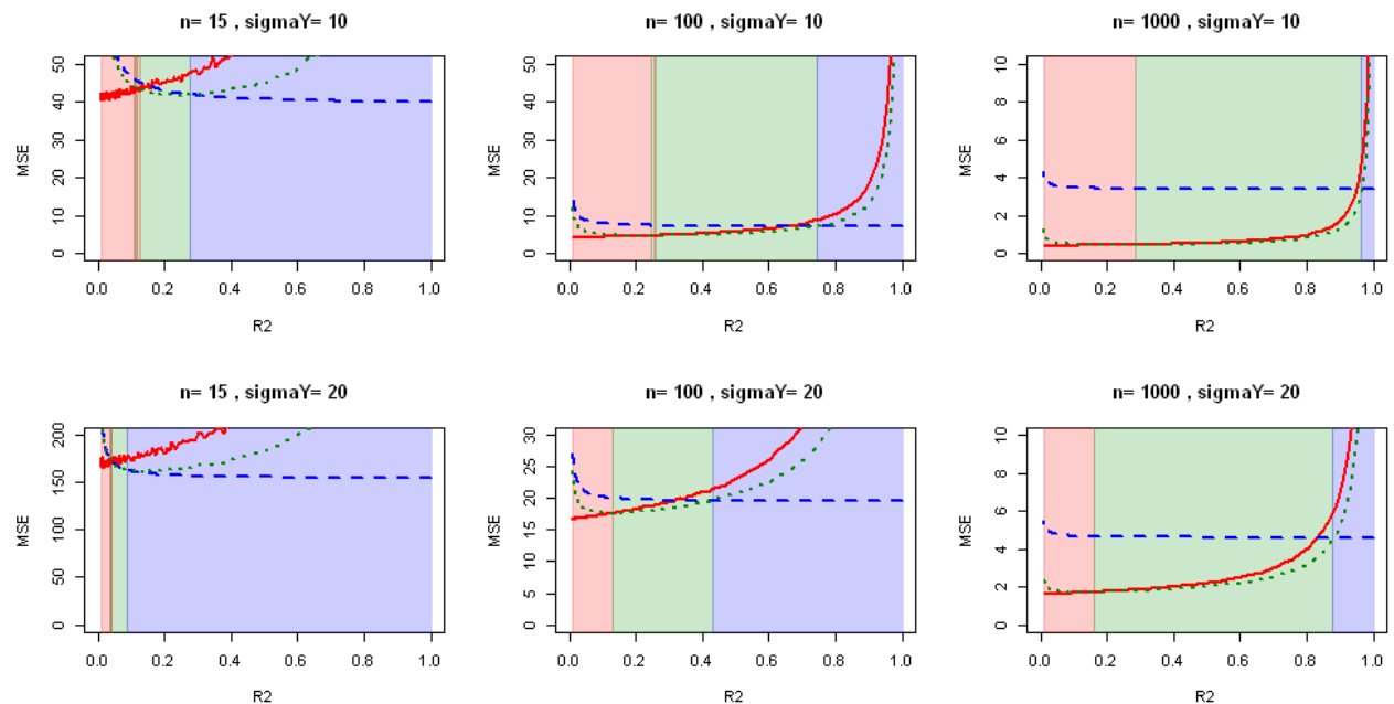
Figure 8.1: MSE on \hat{\boldsymbol{\beta}} of OLS (plain red) and CorReg marginal (blue dashed) and CorReg plug-in (green dotted) estimators for varying R^2 of the sub-regression, n and \sigma_Y . Results obtained on the running example with d = 5 covariates.
