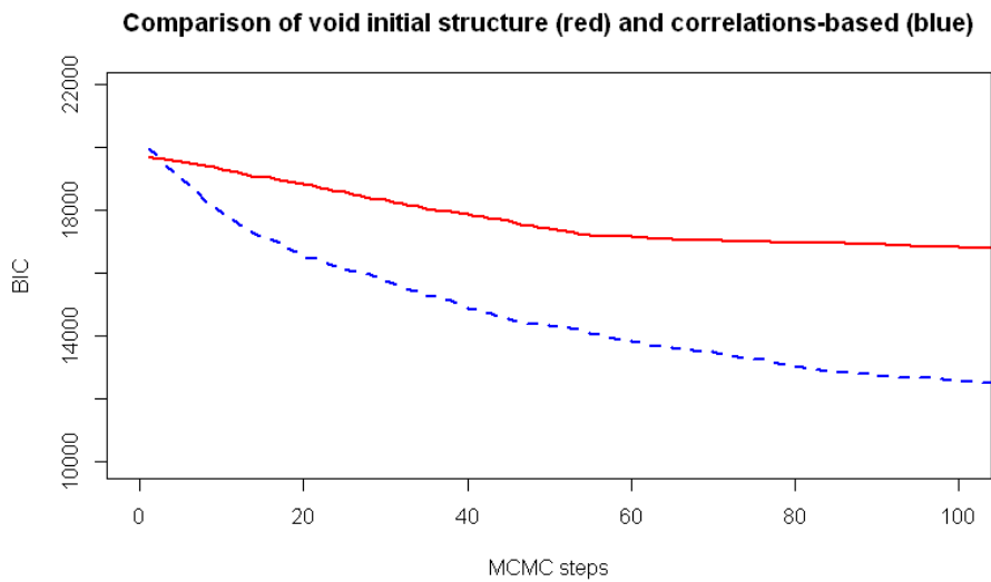
Figure 5.8: Evolution of the BIC (criterion to minimize in the MCMC) for each method.
