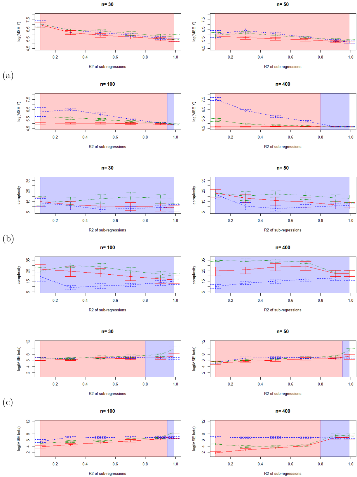
Figure 8.14: Comparison of the MSE on \hat{Y} (a), complexities (b) and MSE on \hat{\beta} (c), plain red=classical (complete) model, dashed blue=marginal model, dotted green=plug-in model.
