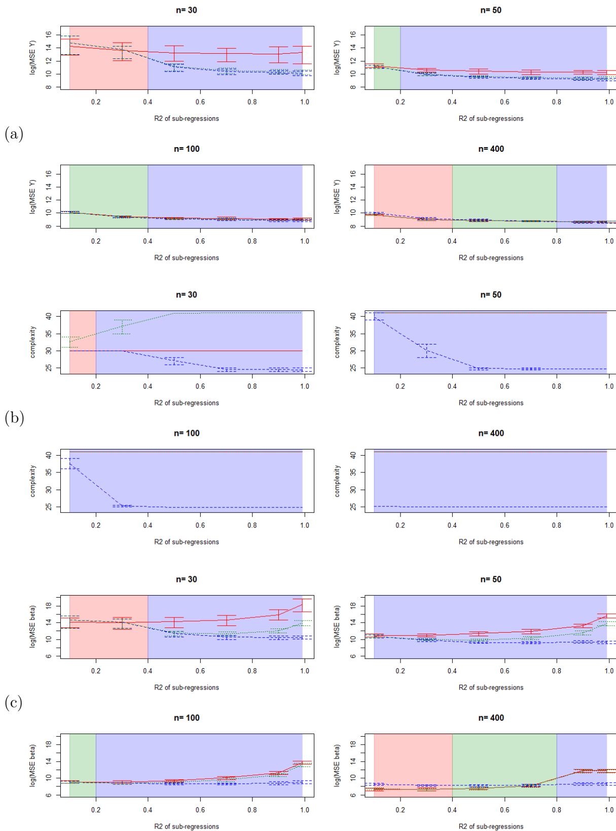
Figure 8.2: Comparison of the MSE on \hat{Y} (a), complexities (b) and MSE on \hat{\beta} (c), plain red=classical (complete) model, dashed blue=marginal model, dotted green=plug-in model.
