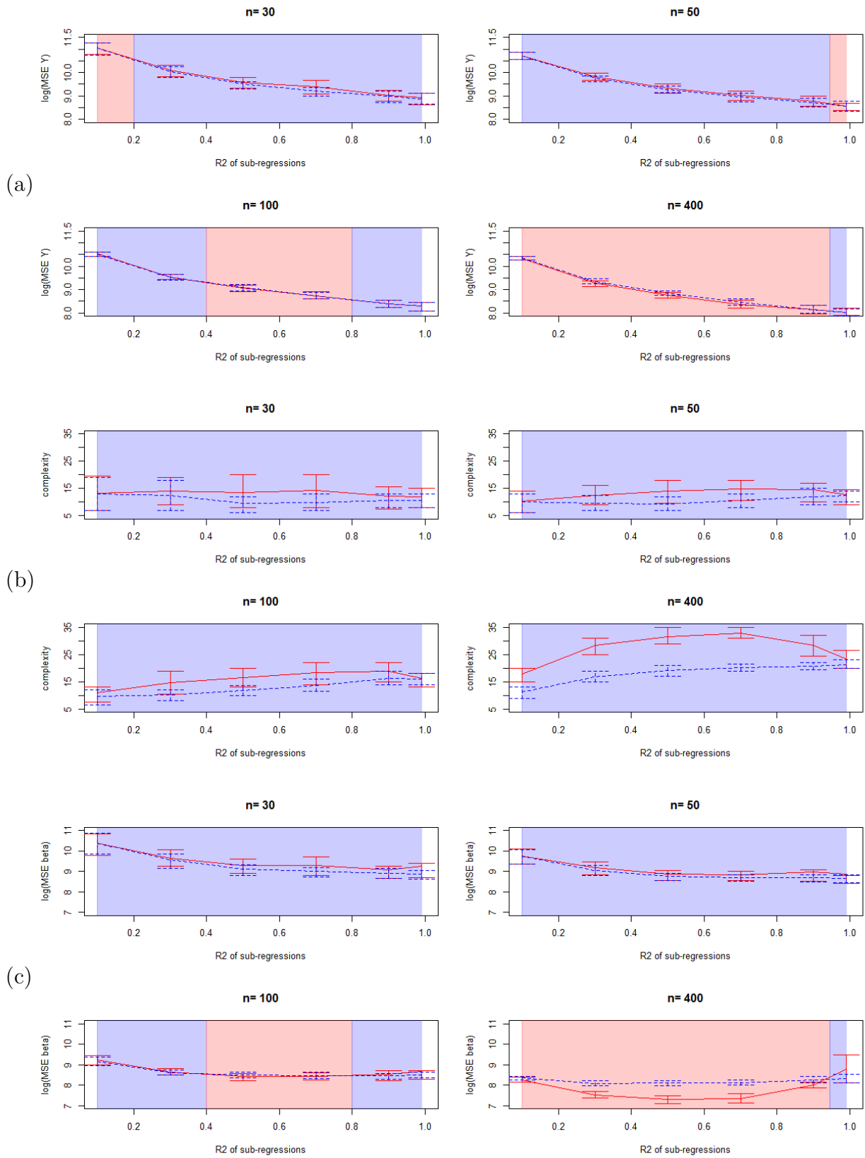
Figure 6.6: Comparison of the MSE on \hat{Y} (a), complexities (b) and MSE on \hat{\beta} (c), red=classical (complete) model, blue=marginal model
