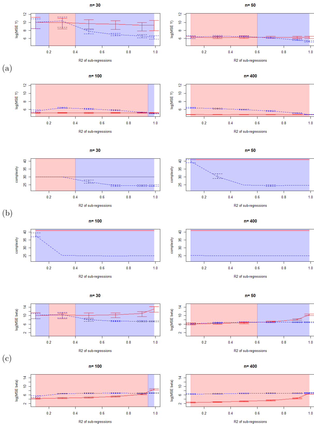
Figure 6.15: Comparison of the MSE on \hat{Y} (a), complexities (b) and MSE on \hat{\beta} (c), red=classical (complete) model, blue=marginal model
