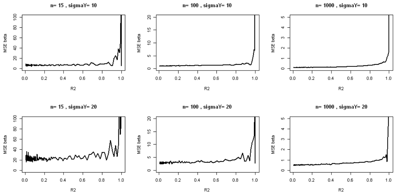
Figure 3.7: Evolution of observed Mean Squared error on \hat{\beta}_{stepwise} with the strength of the correlations for various sample sizes and strength of regression. d = 5 covariates.
