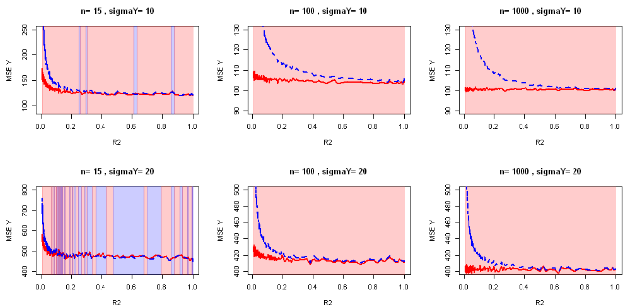
Figure 4.11: Evolution of observed Mean Squared error on \hat{Y}_{ridge} with the strength of the correlations for various sample sizes and strength of regression. d = 5 covariates.
