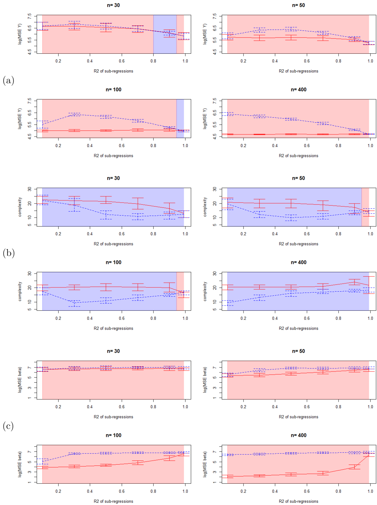
Figure 6.18: Comparison of the MSE on \hat{Y} (a), complexities (b) and MSE on \hat{\beta} (c), red=classical (complete) model, blue=marginal model
