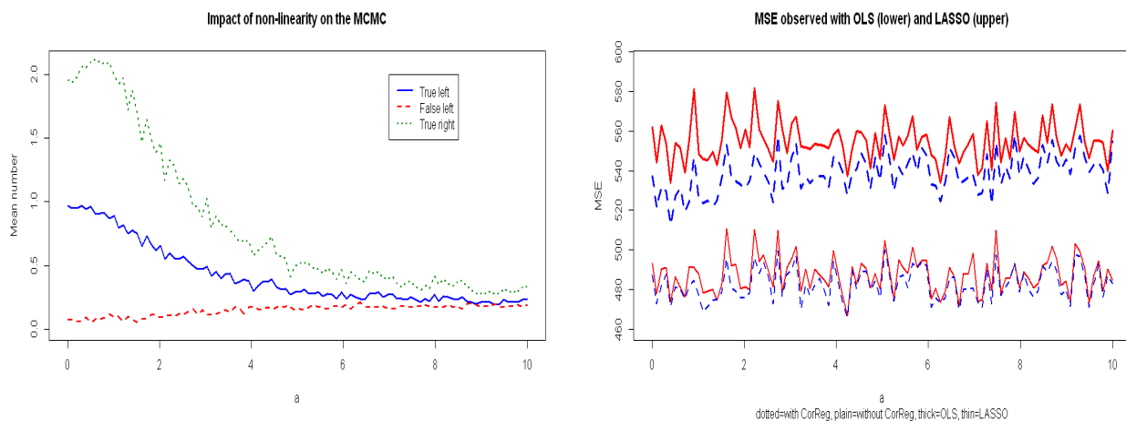
(a) Evolution of the quality of \hat{\mathbf{S}} when the paramater a increases (b) MSE on the main regression for OLS(thick) and LASSO (thin) used both with (plain) or without CorReg (dotted).
