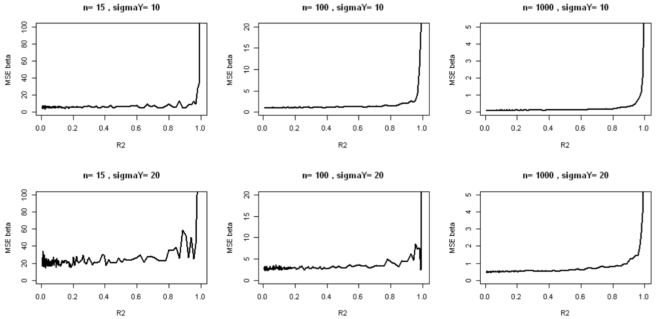
Figure 3.13: Evolution of observed Mean Squared error on \hat{\beta}_{elasticnet} with the strength of the correlations for various sample sizes and strength of regression. d = 5 covariates.
