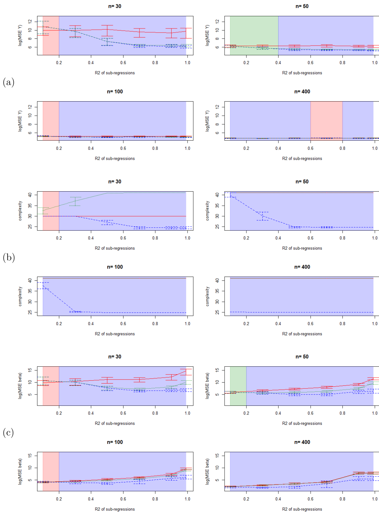
Figure 8.7: Comparison of the MSE on \hat{Y} (a), complexities (b) and MSE on \hat{\beta} (c), plain red=classical (complete) model, dashed blue=marginal model, dotted green=plug-in model.
