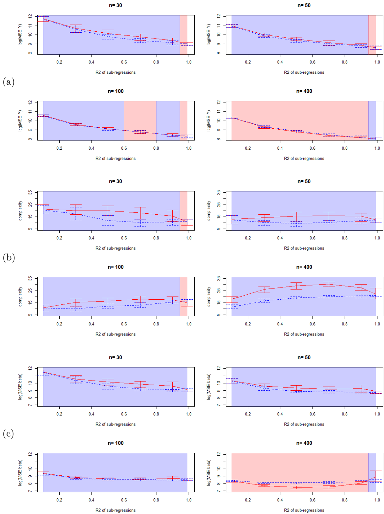
Figure 6.8: Comparison of the MSE on \hat{Y} (a), complexities (b) and MSE on \hat{\beta} (c), red=classical (complete) model, blue=marginal model
