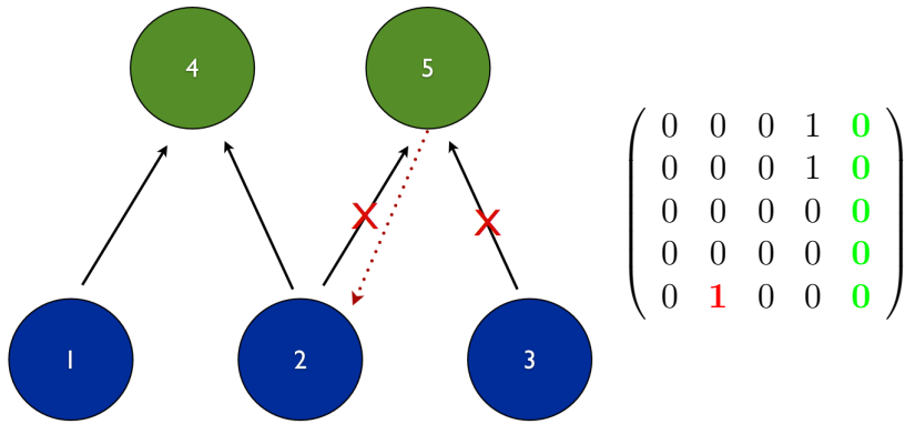
Figure 5.3: Column-wise relaxation: newly predictive covariate cannot be regressed anymore.
