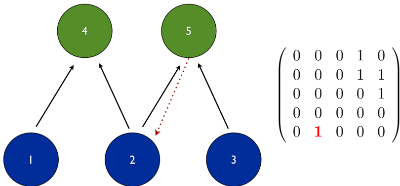
Figure 5.2: We want to define the candidate \tilde{\mathbf{S}} = \mathbf{S}^{(5,2)} and its associated matrix but the structure obtained would not be feasible (breaking the uncrossing rule).
