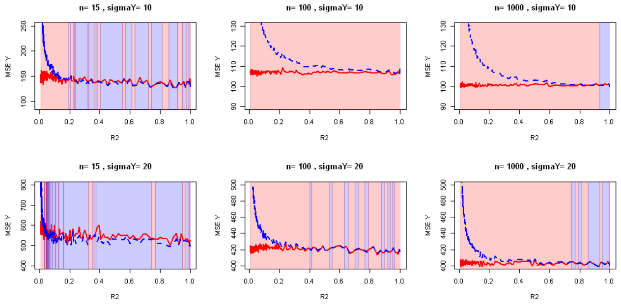
Figure 4.7: Evolution of observed Mean Squared error on \hat{Y}_{elasticnet} with the strength of the correlations for various sample sizes and strength of regression. d = 5 covariates.
