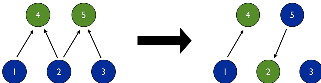
Figure 5.6: All this modifications are made in only one step in the MCMC, meaning an increased scope for the neighbourhoods.
