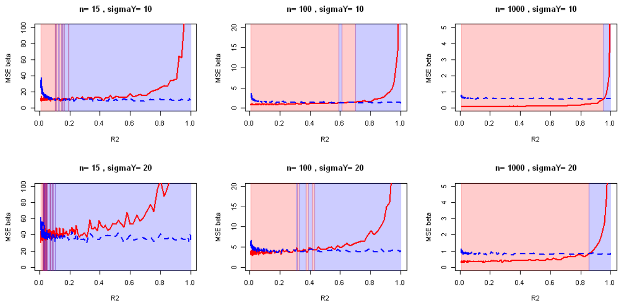
Figure 4.2: Observed MSE on \hat{\beta} of OLS (plain red) and CorReg's marginal model (dashed blue) estimators for varying R^2 of the sub-regression, n and \sigma_Y . d = 5 covariates.
