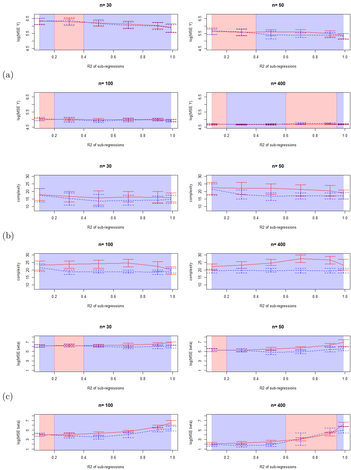
Figure 6.11: Comparison of the MSE on \hat{Y} (a), complexities (b) and MSE on \hat{\beta} (c), red=classical (complete) model, blue=marginal model
