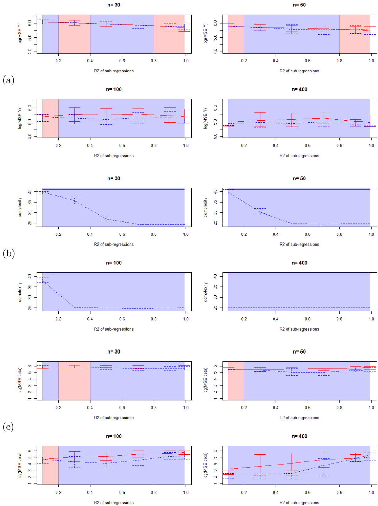
Figure 6.14: Comparison of the MSE on \hat{Y} (a), complexities (b) and MSE on \hat{\beta} (c), red=classical (complete) model, blue=marginal model
