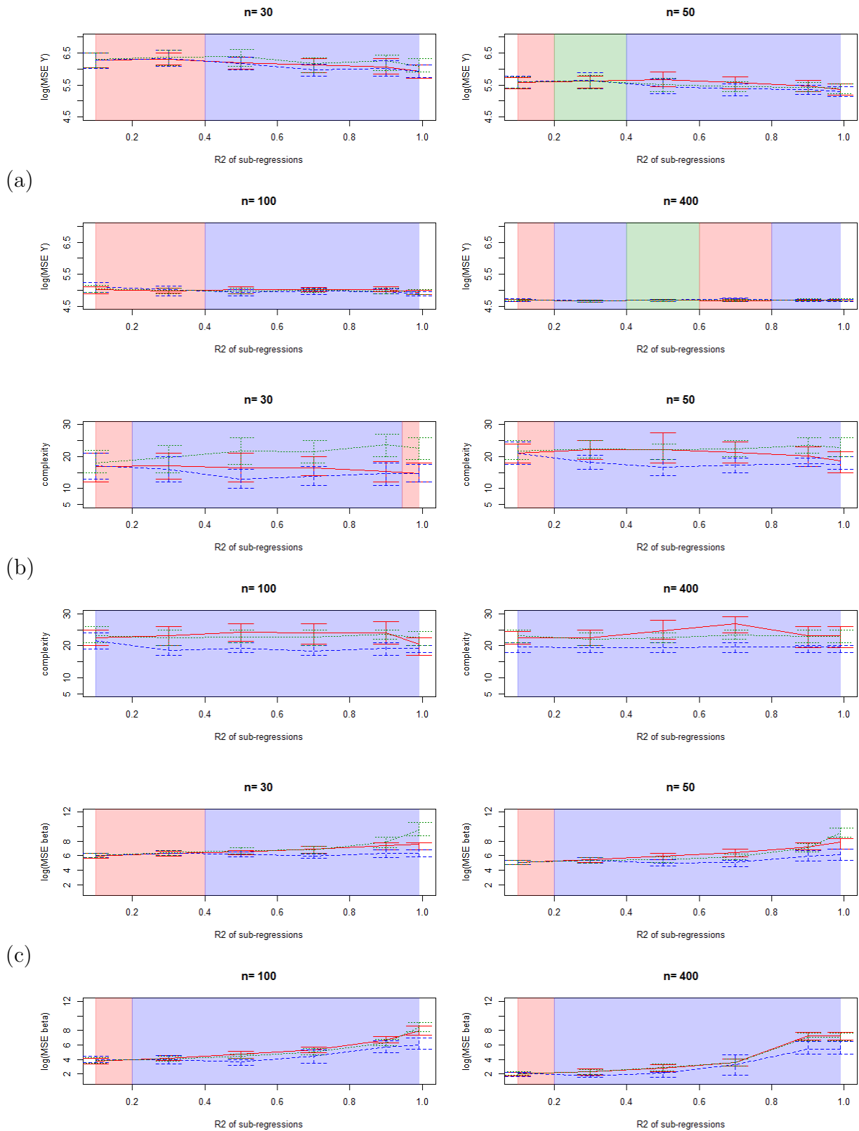
Figure 8.8: Comparison of the MSE on \hat{Y} (a), complexities (b) and MSE on \hat{\beta} (c), plain red=classical (complete) model, dashed blue=marginal model, dotted green=plug-in model.
