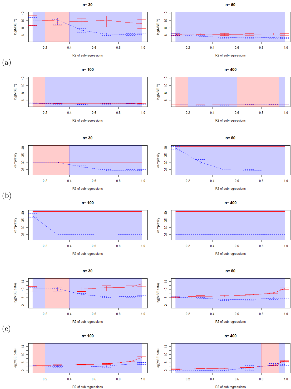
Figure 6.10: Comparison of the MSE on \hat{Y} (a), complexities (b) and MSE on \hat{\beta} (c), red=classical (complete) model, blue=marginal model
