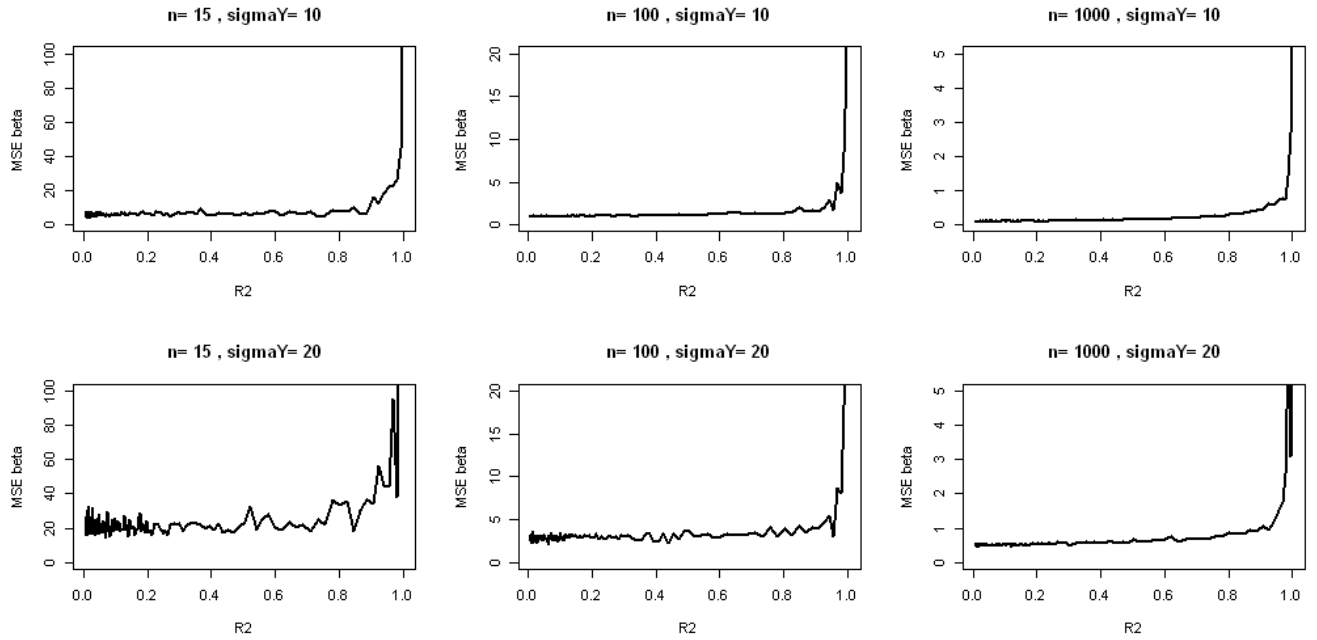
Figure 3.11: Evolution of observed Mean Squared error on \hat{\beta}_{lar} with the strength of the correlations for various sample sizes and strength of regression. d = 5 covariates.
