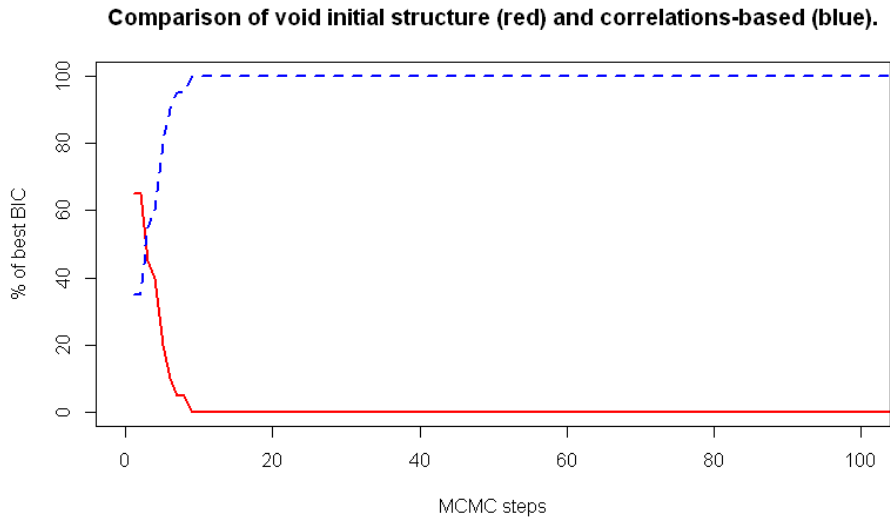
Figure 5.7: Amount of time each method is better for the 100 first steps of the MCMC.
