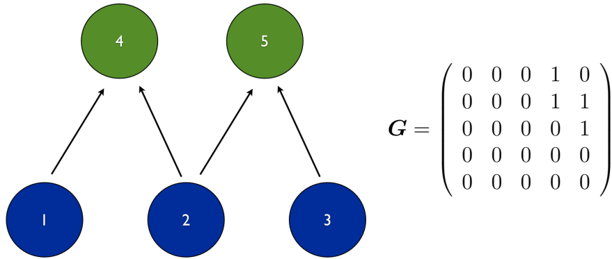
Figure 5.1: We start from a structure \mathbf{S} = ((4, 5), (\{1, 2\}, \{2, 3\})) and its associated matrix G
