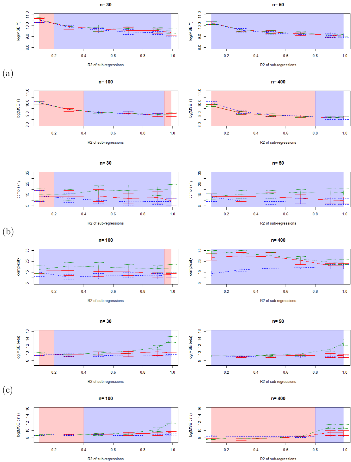
Figure 8.3: Comparison of the MSE on \hat{Y} (a), complexities (b) and MSE on \hat{\beta} (c), plain red=classical (complete) model, dashed blue=marginal model, dotted green=plug-in model.
