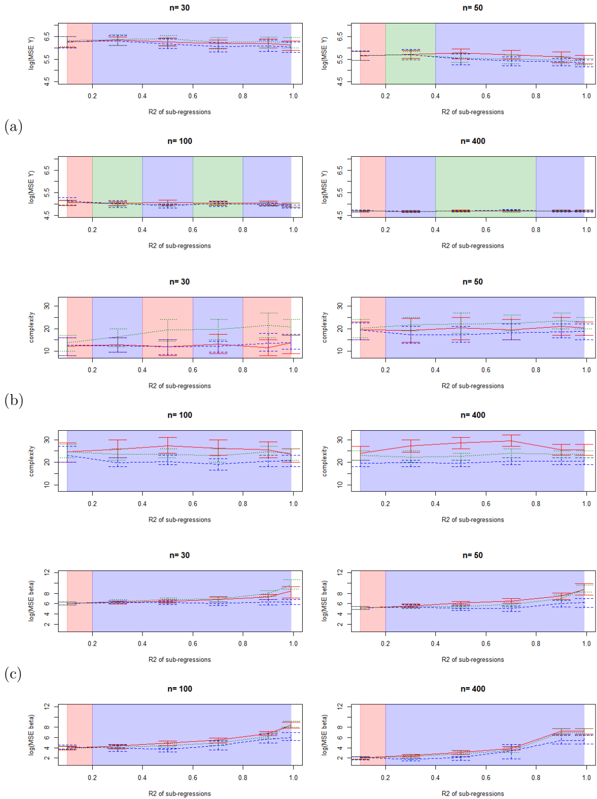
Figure 8.9: Comparison of the MSE on \hat{Y} (a), complexities (b) and MSE on \hat{\beta} (c), plain red=classical (complete) model, dashed blue=marginal model, dotted green=plug-in model.
