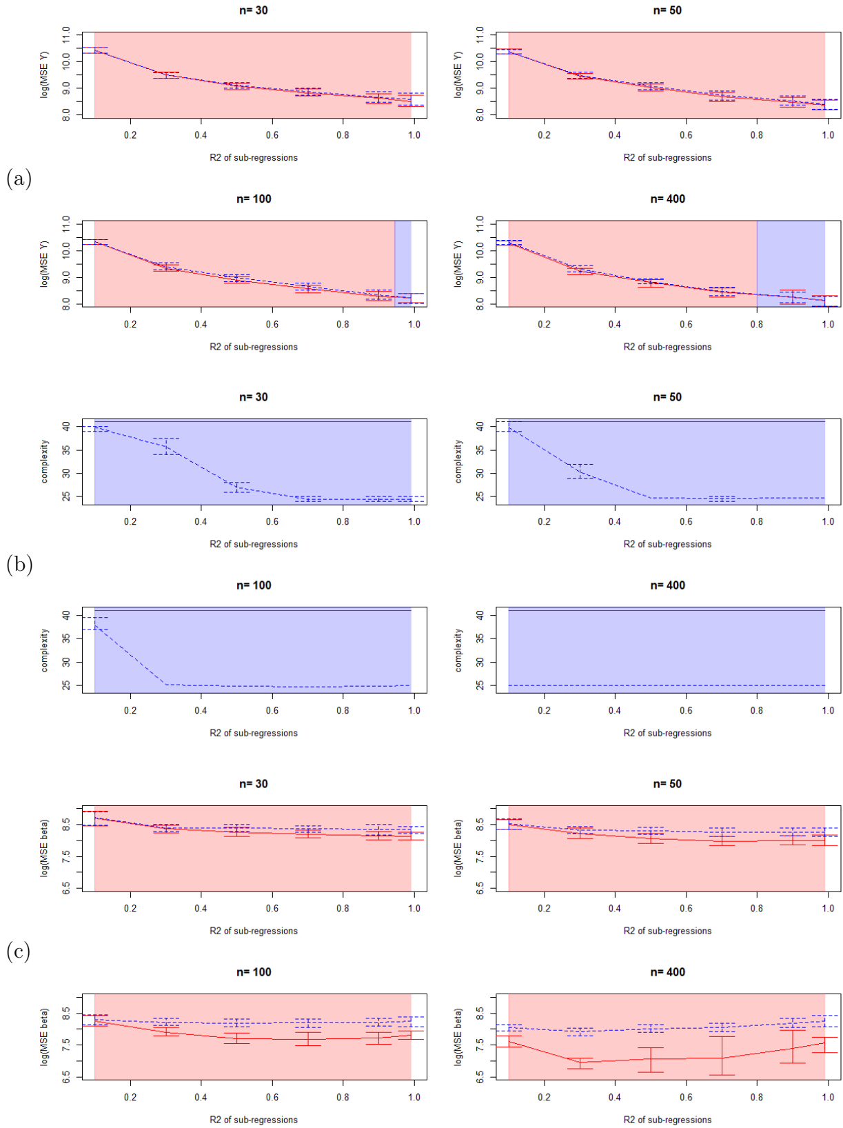
Figure 6.9: Comparison of the MSE on \hat{Y} (a), complexities (b) and MSE on \hat{\beta} (c), red=classical (complete) model, blue=marginal model
