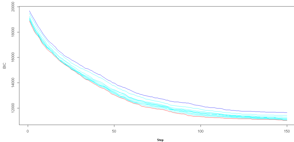
Figure 5.9: Comparison of distinct number of correlation-based initializations for the MCMC. Dark blue=1 initialization, red=10 initializations, the cyan curves represent all intermediate values for the number of initializations (from 2 to 9).
