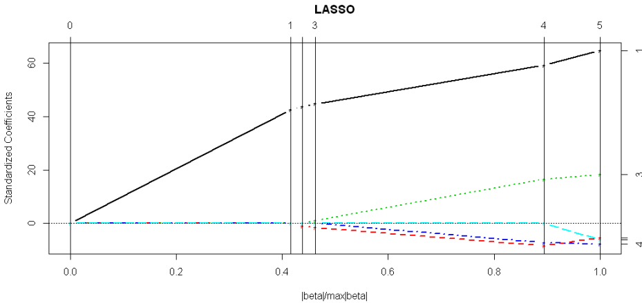
Figure 3.10: The LASSO path computed by lars
