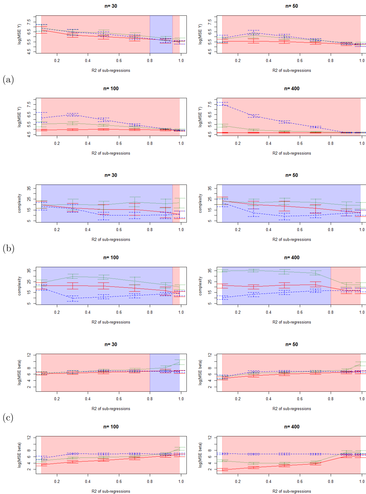
Figure 8.13: Comparison of the MSE on \hat{Y} (a), complexities (b) and MSE on \hat{\beta} (c), plain red=classical (complete) model, dashed blue=marginal model, dotted green=plug-in model.
