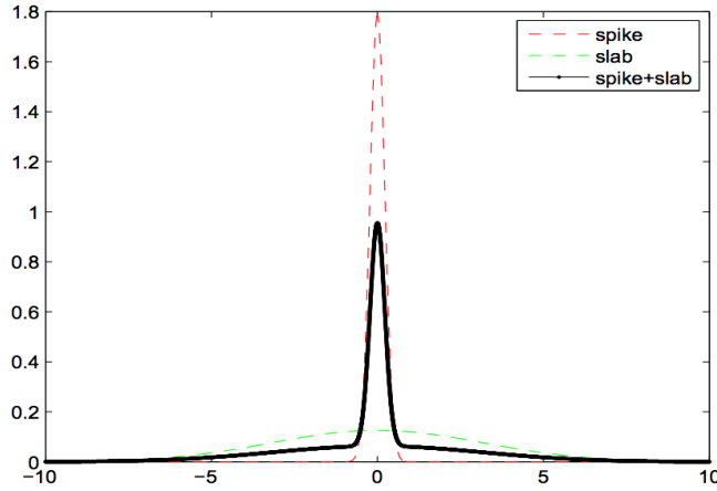
Figure 3.15: The spike and the slab
