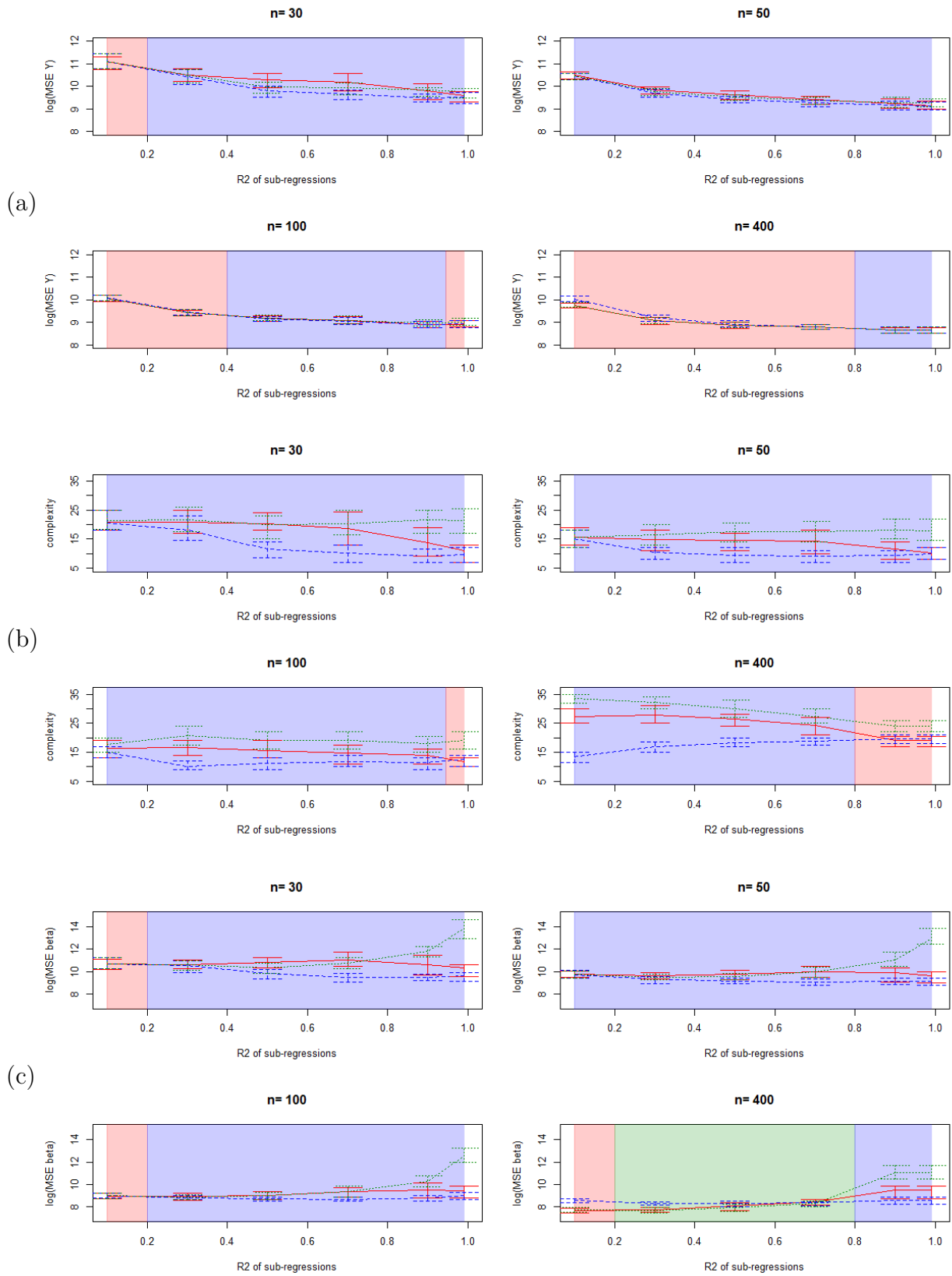
Figure 8.5: Comparison of the MSE on \hat{Y} (a), complexities (b) and MSE on \hat{\beta} (c), plain red=classical (complete) model, dashed blue=marginal model, dotted green=plug-in model.
