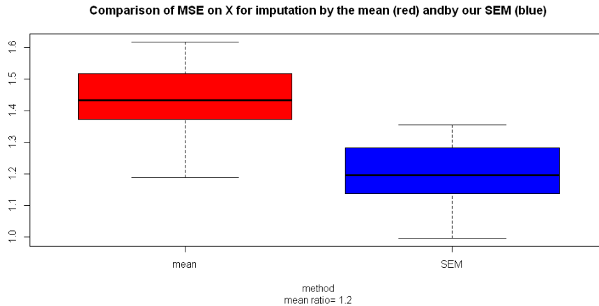
Figure 9.3: MSE on \hat{\mathbf{X}} is significantly lower when using our Stochastic EM than with imputation by the mean.
