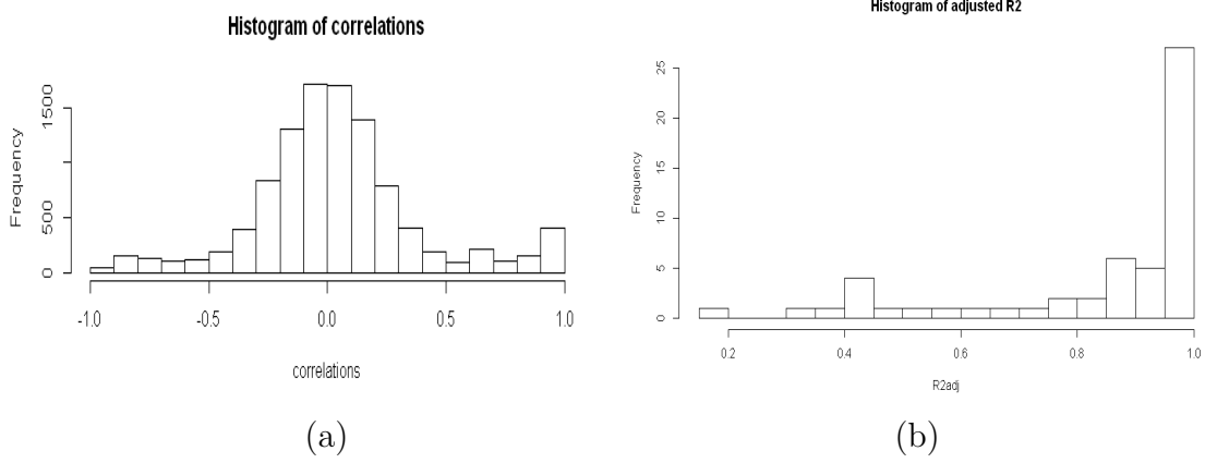
Figure 7.3: Production case study: (a) Histogram of correlations \rho in \mathbf{X} , (b) histogram of the adjusted R^2_{adj} for the d_r = 55 sub-regressions.
