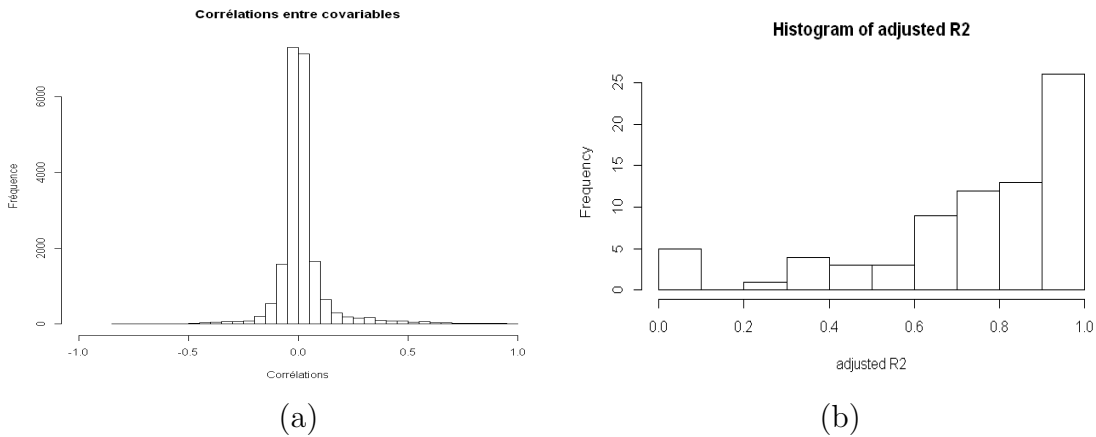
Figure 7.1: Quality case study: (a) Histogram of correlations \rho in \mathbf{X} , (b) histogram of the adjusted R_{adj}^2 for the d_r = 76 sub-regressions.
