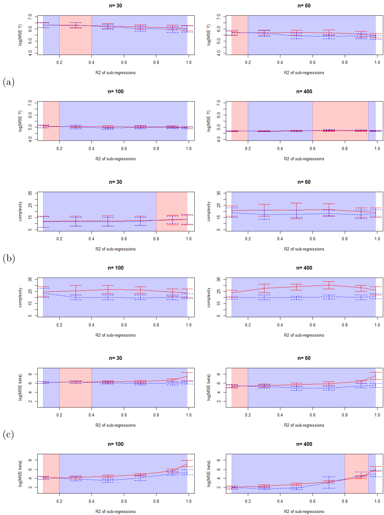
Figure 6.12: Comparison of the MSE on \hat{Y} (a), complexities (b) and MSE on \hat{\beta} (c), red=classical (complete) model, blue=marginal model
