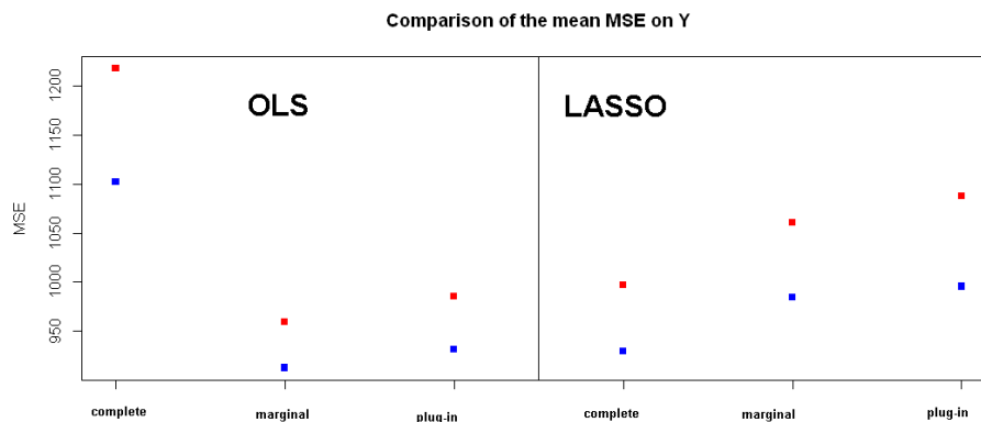
Figure 9.4: MSE on \hat{\mathbf{Y}} are lower when using our Stochastic EM (blue) than with imputation by the mean (red) for the three model (complete, marginal and plug-in) using OLS or LASSO
