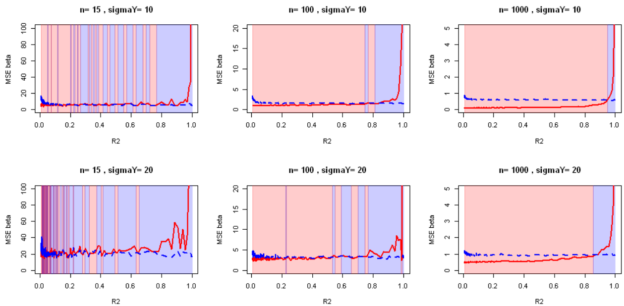
Figure 4.6: Observed MSE on \hat{\beta}_{elasticnet} on both X (red) and CorReg's marginal X_f (blue) for varying R^2 of the sub-regression, n and \sigma_Y . d = 5 covariates.
