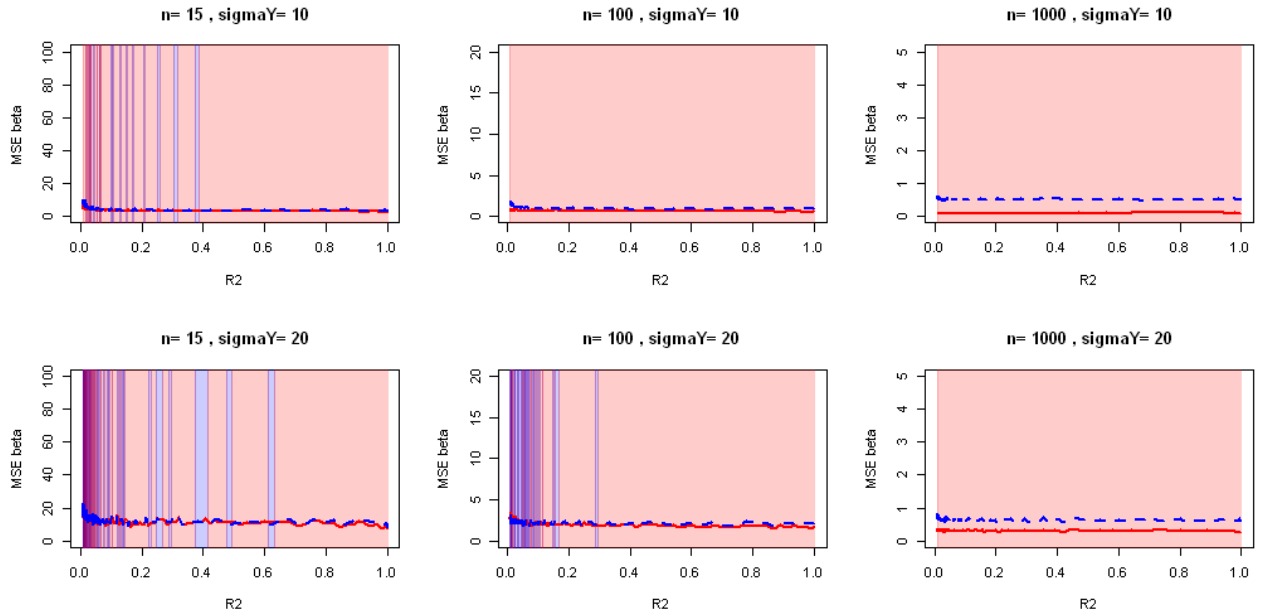
Figure 4.10: Observed MSE on \hat{\beta}_{ridge} on both \mathbf{X} (red) and \text{CorReg} 's marginal \mathbf{X}_f (blue) for varying R^2 of the sub-regression, n and \sigma_Y . d = 5 covariates.
