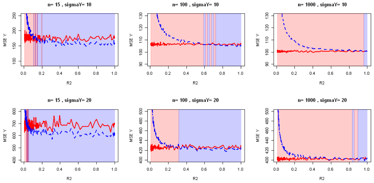
Figure 4.3: Evolution of observed Mean Squared error on \hat{Y}_{OLS} with the strength of the correlations for various sample sizes and strength of regression. d = 5 covariates.
