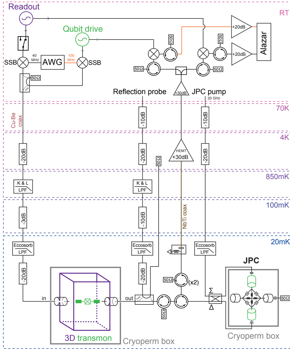
Figure 67: Full schematic of the wiring for the fluorescence trajectories experiment described in Sec. 3.4.2. The fluorescence field from the qubit on the output line is amplified by a JPC tuned at \omega_q . The same source used to generate preparation pulses of the qubit is used to down convert the resulting signal to 100 MHz (in orange) before digitization and numerical demodulation.
