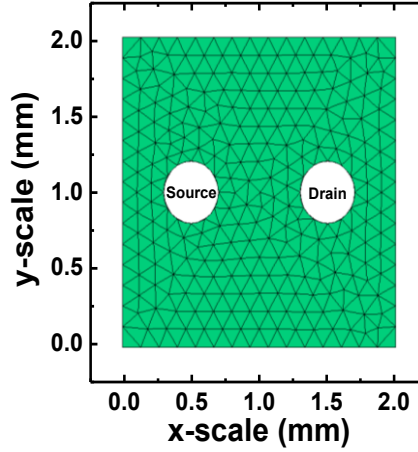
Figure V-15: Mesh of the computed structure with source and drain contacts. R_\theta = 200 \mu\text{m} and die surface equal to 2 \text{ mm} \times 2 \text{ mm} . The inter-probe distance is 1 \text{ mm} . 3000 nodes were used for meshing.
