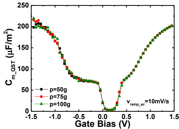
Figure IV-6: QSCV capacitance versus gate bias for different probe pressures. The SOI structure had 88 nm top silicon film thickness and 145 nm BOX thickness. Passivated top surface.
