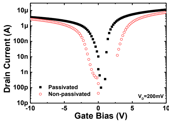
Figure II-14: Drain current as a function of gate bias for SOI structure with 88 \text{ nm} top silicon film and 145 \text{ nm} BOX. The passivated structure (plain symbols) was measured using p = 100 \text{ g} , while in non-passivated sample (empty symbols) the tip pressure was 80 \text{ g} .
