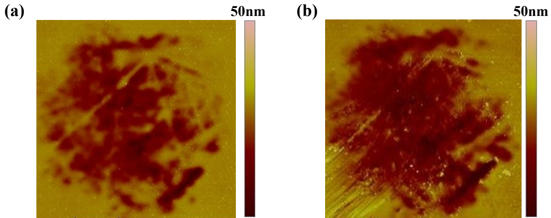
Figure II-15: 10\ \mu\text{m} \times 10\ \mu\text{m} AFM image for passivated (a) and non-passivated (b) SOI samples. The same tip was used with different pressure: 100\text{ g} in case of passivated and 80\text{ g} for the non-passivated one.
