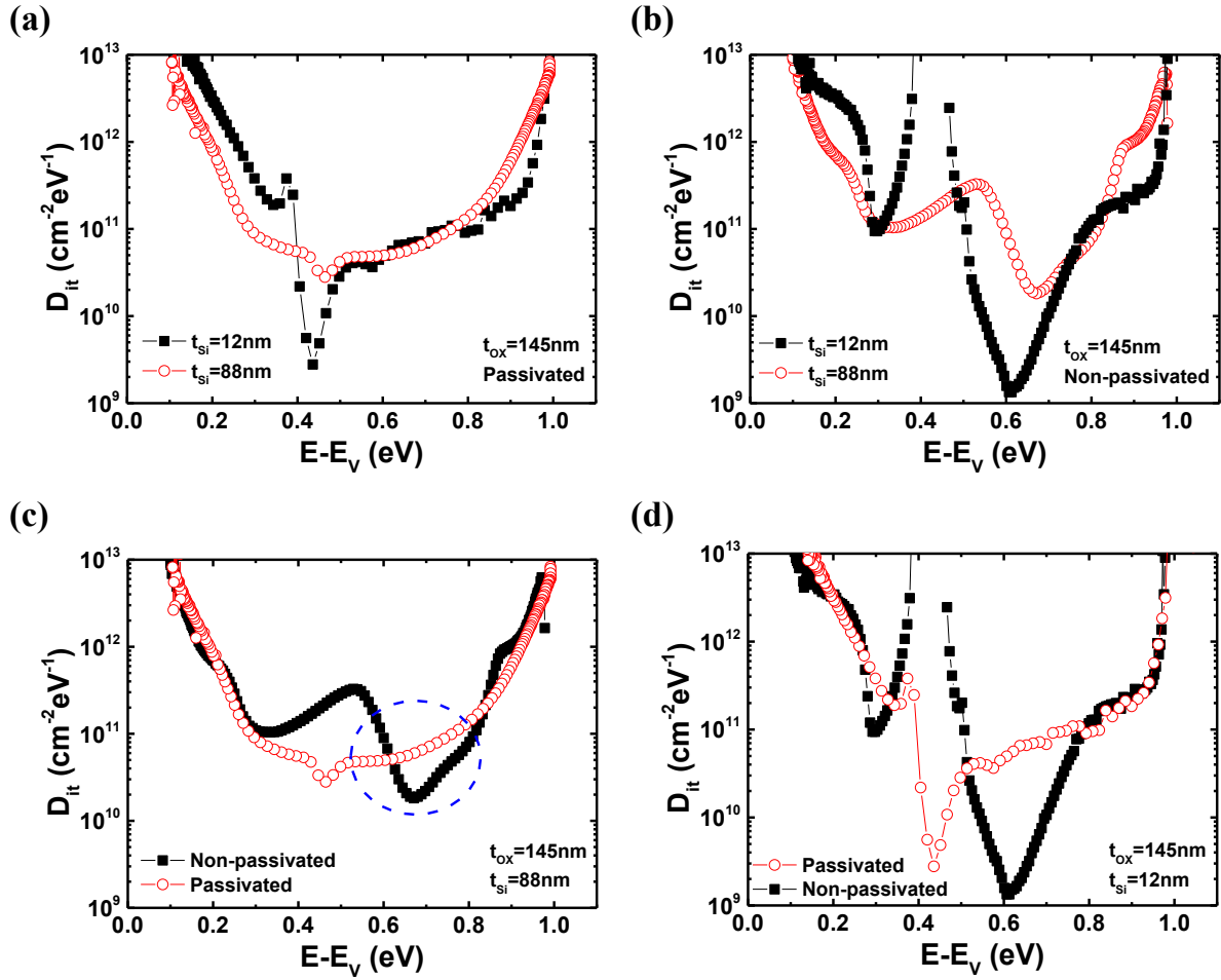
Figure IV-30: D_{it} computed versus E-E_V in case of 88\text{ nm} (empty symbols) and 12\text{ nm} (plain symbols) top silicon film thickness. The BOX thickness was 145\text{ nm} . Passivated (a) and non-passivated (b) top surface, (c) thick Si film and (d) thin silicon layer.
