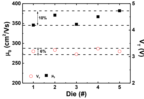
Figure II-13: Extracted \mu_0 (plain symbols) and V_T (empty symbols) from different dies present in the same SOI wafer with 88 \text{ nm} thick Si film and 145 \text{ nm} thick BOX. The top surface was non-passivated.
