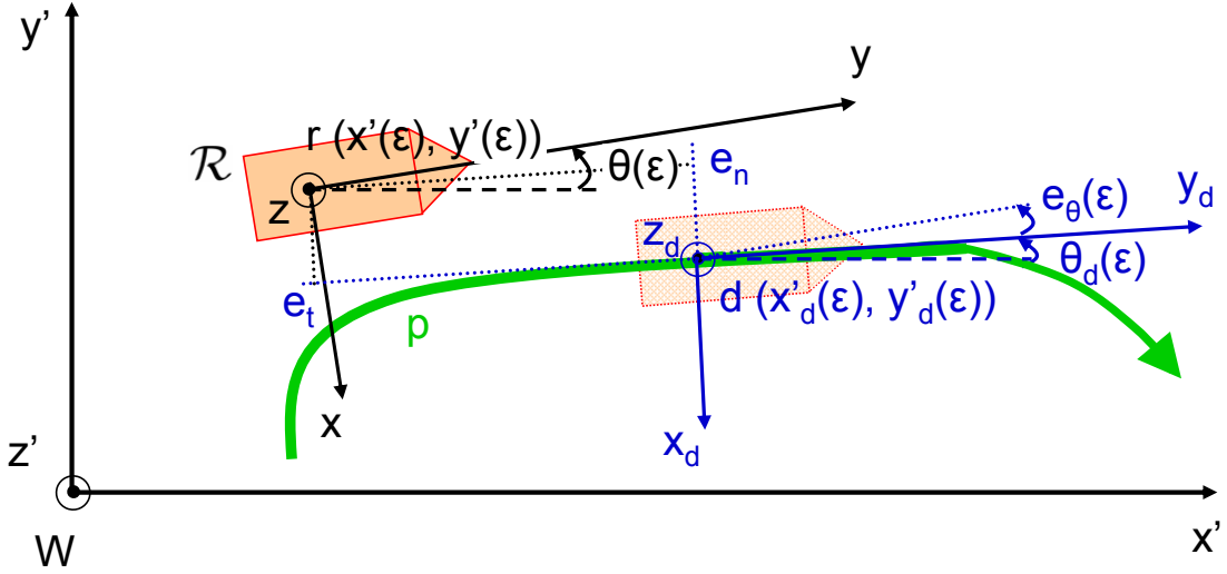
Figure 1.1: Path following relevant variables.
