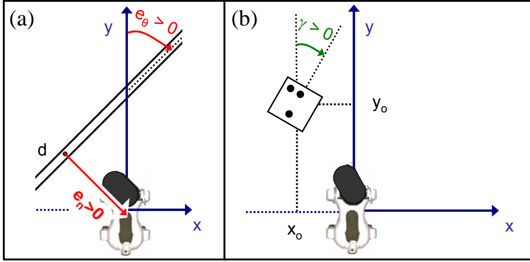
Figure 4.7: Relevant variables utilized in: (a) straight white line tracking, and (b) coded square tracking.
