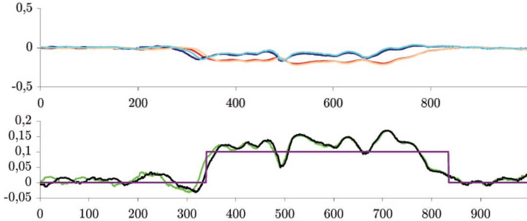
Figure 3.15: Evolution of relevant variables during the first image-based experiment. Top: errors \mathcal{E}_1^* (non-dimensional), and \mathcal{E}_2 (in rad) are plotted (red and blue: correct camera calibration, pink and cyan: coarse calibration). Bottom: c_d in \text{m}^{-1} (purple) and \phi in rad (green: correct camera calibration, black: coarse calibration).
