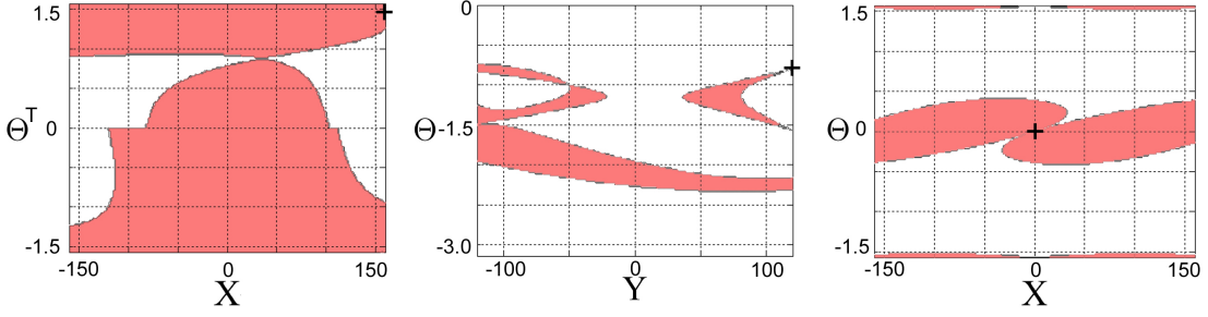
Figure 3.7: Image-based stability loci of the state variables ( X , Y in pixels, \Theta , \Theta^t in rad) that verify the Lyapunov sufficient asymptotic stability condition (pink) for: top row controller (left), right column controller (center), and bottom row controller (right). The desired states are indicated with the black cross.
