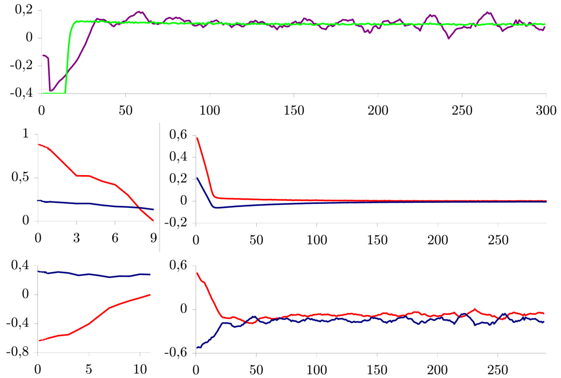
Figure 3.4: Evolution of relevant variables during simulated PF with path initially intersecting the right pixel column. Top: applied steering angle \phi in rad (purple: position-based, green: image-based). Center: state errors \mathcal{E}_1 (red, in m) and \mathcal{E}_2 (blue, in rad) for the position-based column controller (left) and row controller (right). Bottom: state errors \mathcal{E}_1^* (red, non-dimensional) and \mathcal{E}_2 (blue, in rad) for the image-based column controller (left) and row controller (right).
