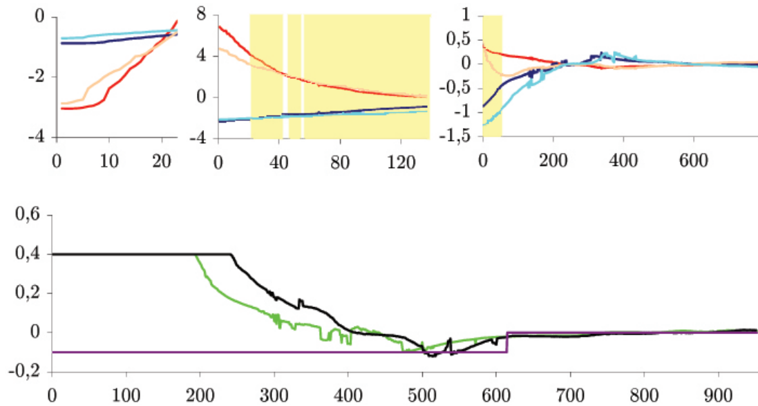
Figure 3.13: Evolution of relevant variables during the third position-based experiment. Top: errors during phases 3.1 to 3.3 (left to right). \mathcal{E}_1 (in m) and \mathcal{E}_2 (rad) are plotted (red and blue: correct camera calibration, pink and cyan: coarse calibration). The iteration steps with state variables not verifying the stability condition are highlighted in yellow. Bottom: c_d in \text{m}^{-1} (purple) and \phi in rad (green: correct camera calibration, black: coarse calibration).
