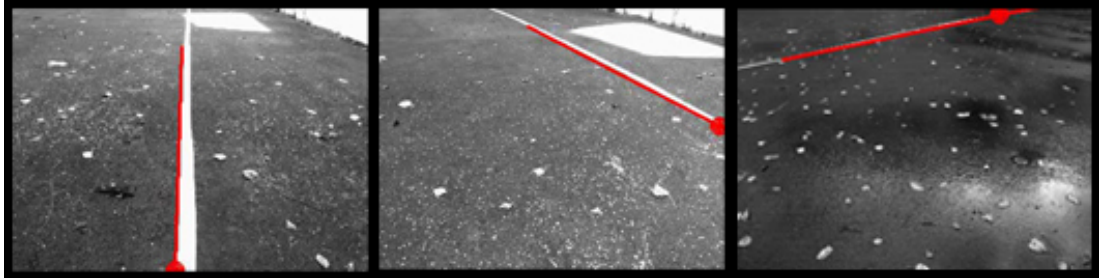
Figure 3.5: Initial conditions used in the path following experiments. The point D and tangent \Gamma derived by image processing are indicated respectively by a red circle and a red line.
