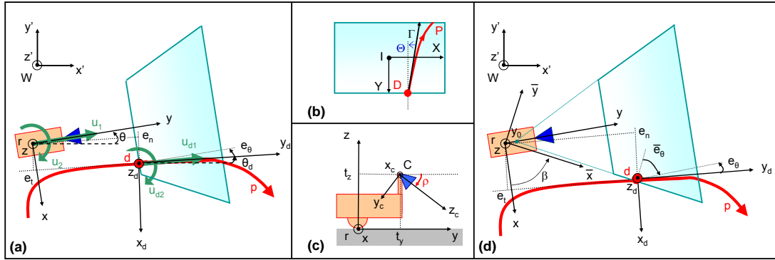
Figure 3.1: Relevant variables utilized in this work. The task for the robot (represented in orange), equipped with a fixed pinhole camera (blue) is to follow the red path, noted p . The figure represents: top view (a,d), image plane (b), and side view (c). The camera field of view and its projection on the ground are represented in cyan. The control inputs are represented in green.
