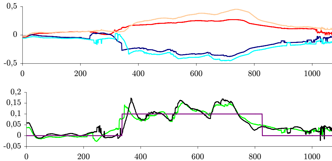
Figure 3.9: Evolution of relevant variables during the first position-based experiment. Top: errors \mathcal{E}_1 in m, and \mathcal{E}_2 , in rad (red and blue: correct camera calibration, pink and cyan: coarse calibration). Bottom: c_d in \text{m}^{-1} (purple) and \phi in rad (green: correct camera calibration, black: coarse calibration).
