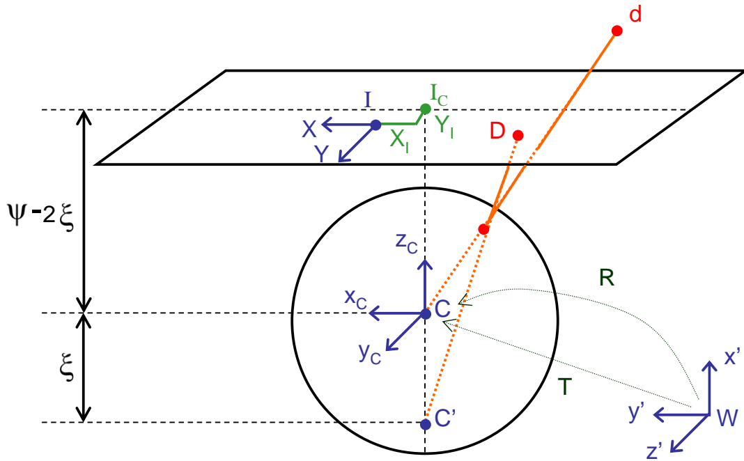
Figure 1.6: The unified central catadioptric camera model: virtual unitary sphere, image plane, and other relevant variables.
