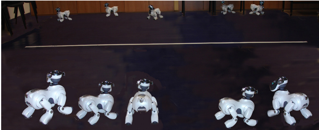
Figure 4.8: The maximum distance at which the robot can detect the roadmap is measured by positioning the robot in various configurations around a straight white line.
