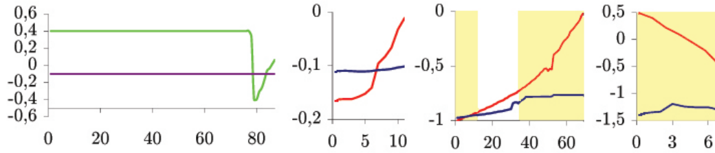
Figure 3.19: Evolution of relevant variables during the third image-based experiment with correct camera calibration. Left to right: c_d (purple, in \text{m}^{-1} ) with \phi (green, in rad), and errors \mathcal{E}_1^* (red, non-dimensional) and \mathcal{E}_2 (blue, in rad) during phases 3.1 to 3.3. The iterations steps with state variables not verifying the stability condition are highlighted in yellow.
