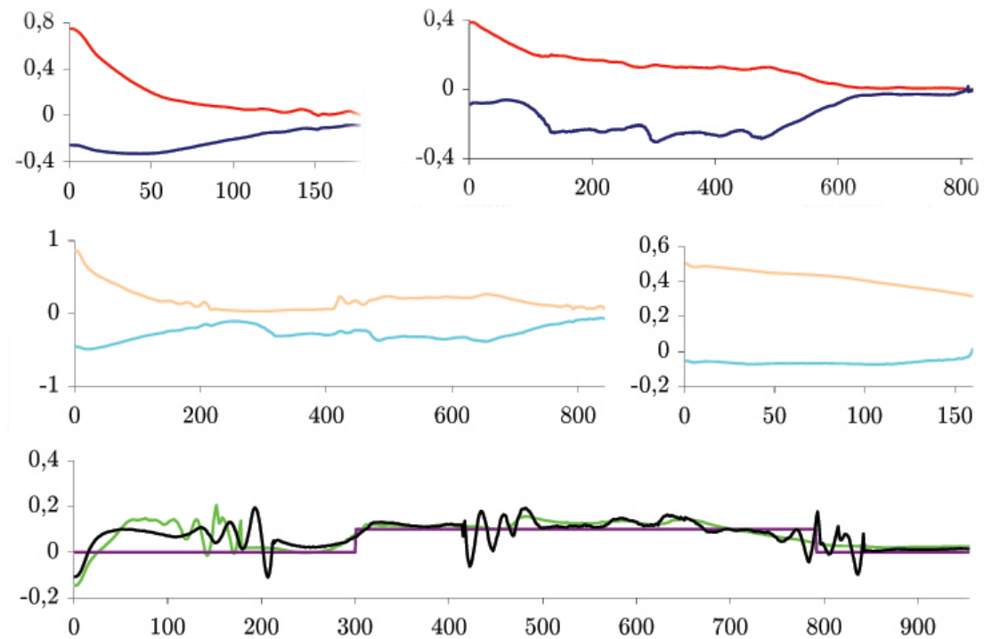
Figure 3.11: Evolution of relevant variables during the second position-based experiment. Top: errors \mathcal{E}_1 (red, in m) and \mathcal{E}_2 (blue, in rad) with correct camera calibration for phases 2.1 (left) and 2.2 (right). Center: same errors ( \mathcal{E}_1 in pink, and \mathcal{E}_2 in cyan) with coarse camera calibration. Bottom: c_d in \text{m}^{-1} (purple) and \phi in rad (green: correct camera calibration, black: coarse calibration).
