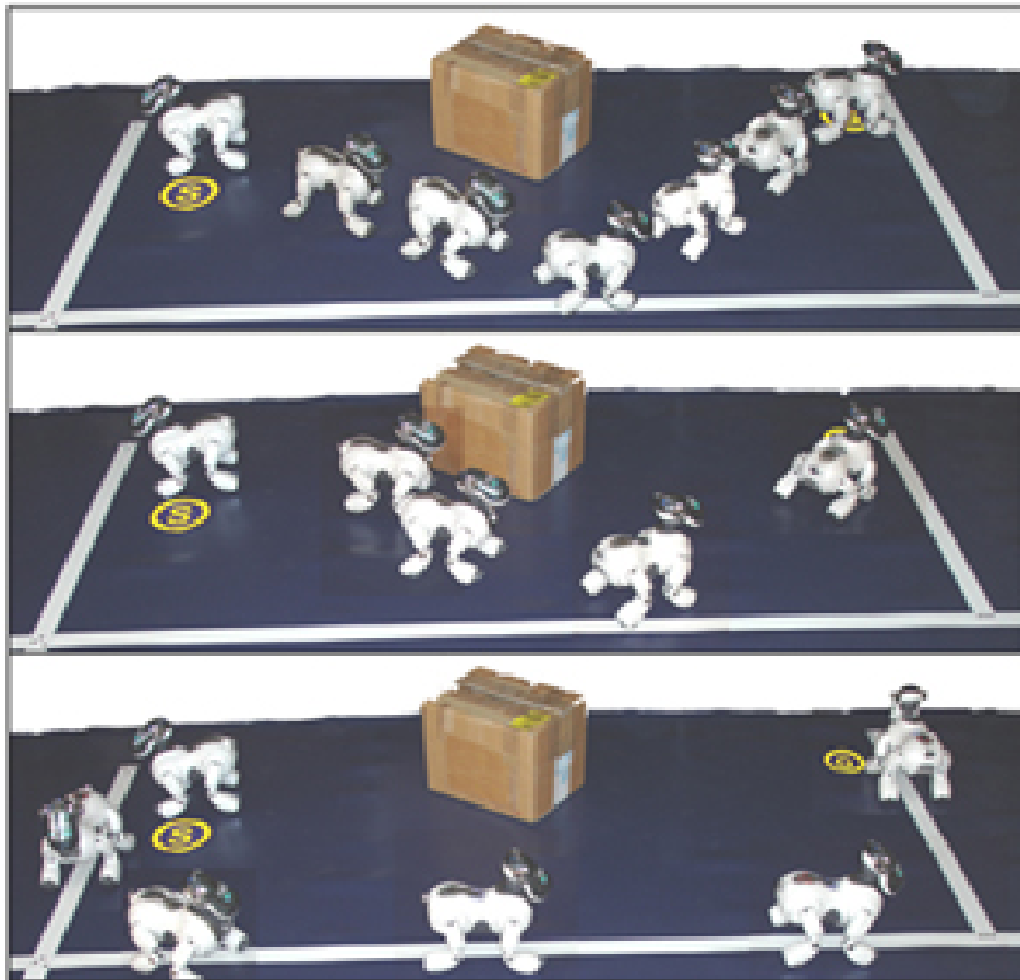
Figure 4.9: Comparison between the three ASPICE navigation modes: with the mouse as input device, the user drives the robot from point S to point G using the single step (above), semi-autonomous (center) and autonomous (below) modes.
