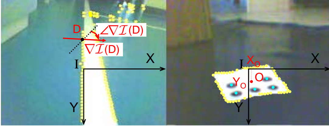
Figure 4.5: Extracting edges (in yellow) for straight white line (left) and coded square (right) detection. The detected coded square center is marked in red and the dot centers are marked in cyan.
