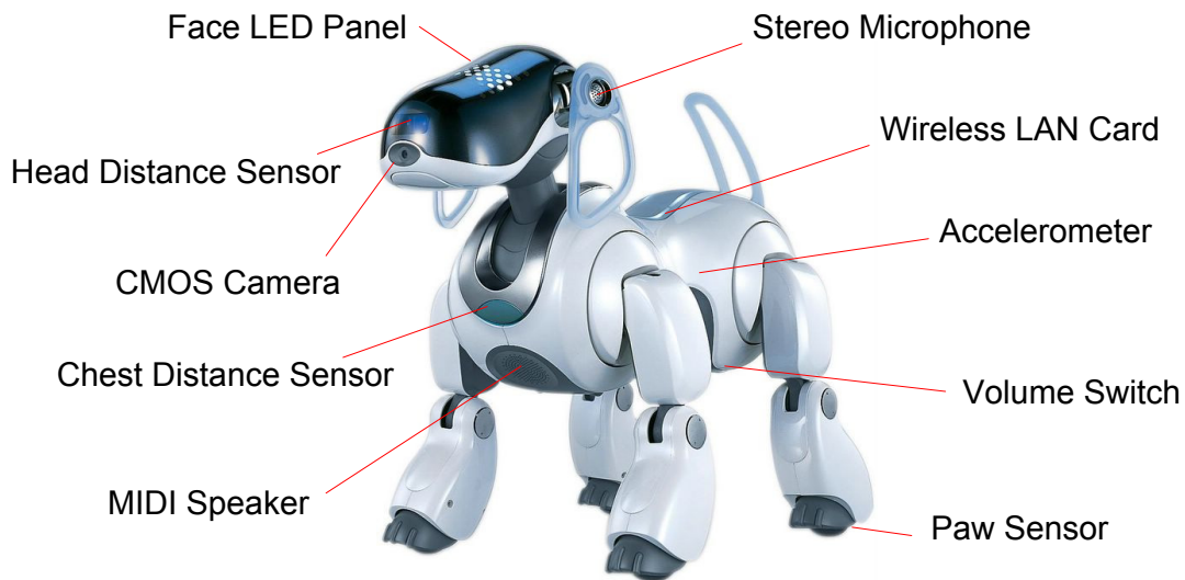
Figure 4.4: The Sony AIBO ERS-7 used in the ASPICE Project.
