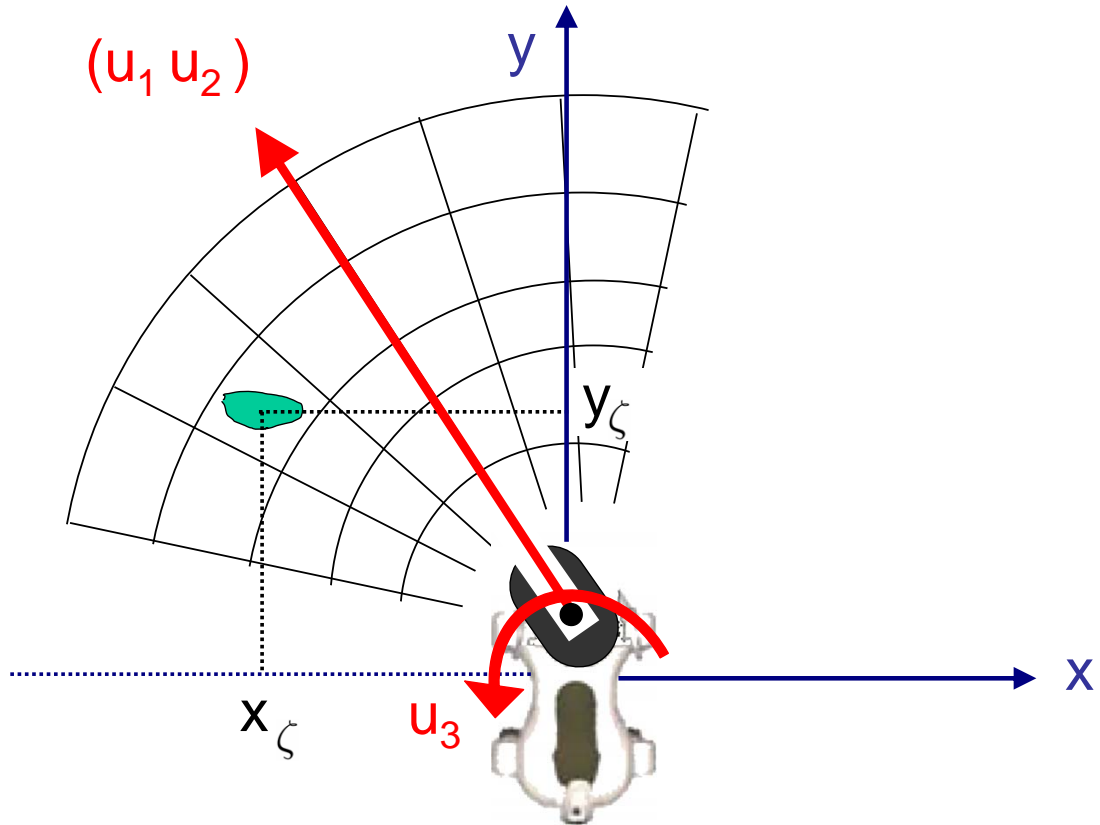
Figure 5.1: Relevant variables utilized in occupancy grid generation.
