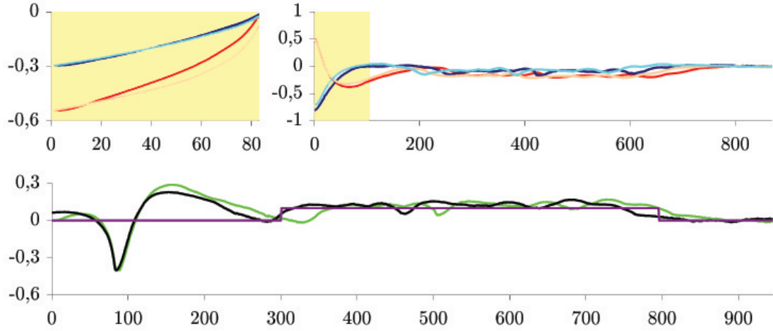
Figure 3.17: Evolution of relevant variables during the second image-based experiment. Top: errors during phases 2.1 (left) and 2.2 (right). \mathcal{E}_1^* (non-dimensional) and \mathcal{E}_2 (in rad) are plotted (red and blue: correct camera calibration, pink and cyan: coarse calibration). The iteration steps with state variables not verifying the stability condition are highlighted in yellow. Bottom: c_d in \text{m}^{-1} (purple) and \phi in rad (green: correct camera calibration, black: coarse calibration).
