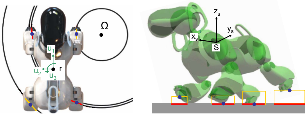
Figure 1.4: Foot loci during kinematic parameterized trot walk: the feet are indicated in blue and the loci in red during stance, and in orange during swing.
