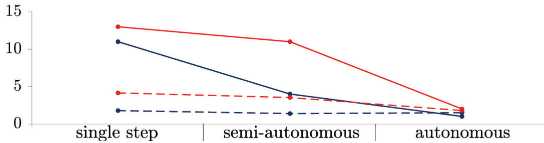
Figure 4.11: Comparison between the 3 navigation modes using 2 input devices: mouse (blue) and BCI (red). Execution time (in minutes): dashed, user intervention (number of commands): solid.
