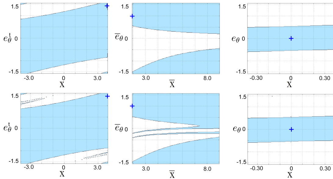
Figure 3.6: Position-based stability loci of the state variables ( x , \bar{x} in m, e_\theta^t , e_\theta , \bar{e}_\theta in rad) that verify the Lyapunov sufficient asymptotic stability condition (cyan) for c_d = 0 (above) and c_d = \pm 0.1 \text{ m}^{-1} (below), and for: top row controller (left), right column controller (center), and bottom row controller (right). The desired states are indicated with the blue cross.
