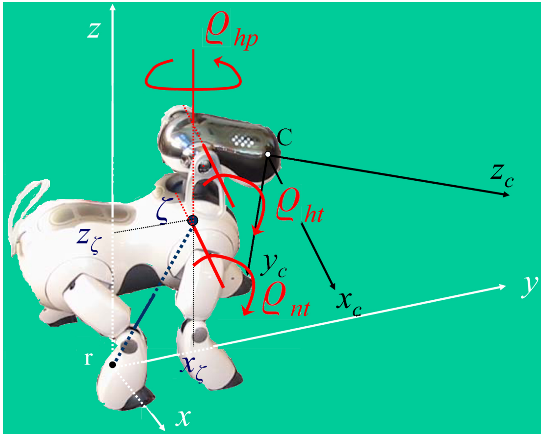
Figure 4.6: The camera frame and head joint positions.
