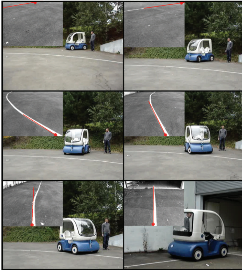
Figure 3.12: Third position-based experiment: the initial error is large ( D is on the top pixel row of the image plane).
