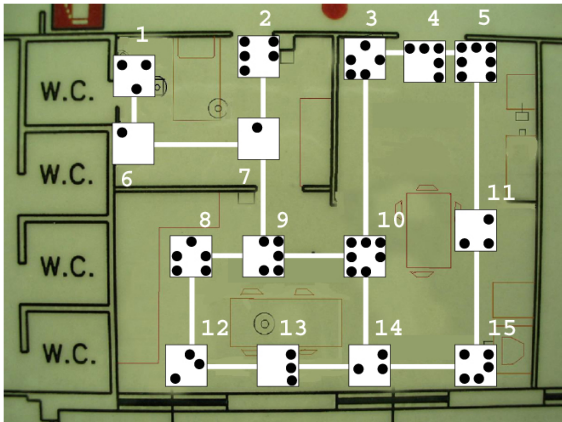
Figure 4.2: The roadmap used in autonomous navigation mode. The ID labels of each coded square are indicated. Note that crossings appear larger than they are.
