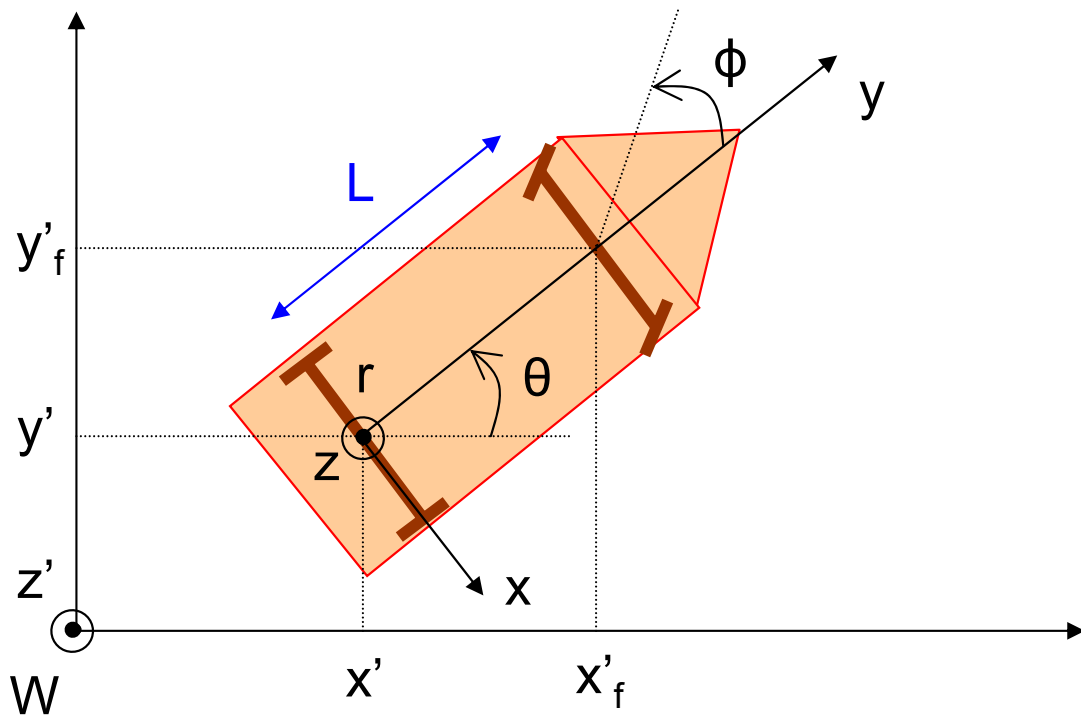
Figure 1.3: Car-like model relevant variables.
