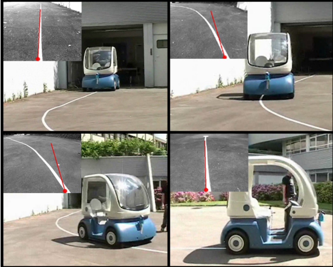
Figure 3.8: First position-based experiment: Cycab is initially positioned on the path with small initial error. The robot positions and corresponding processed images at consecutive time frames are shown during PF.
