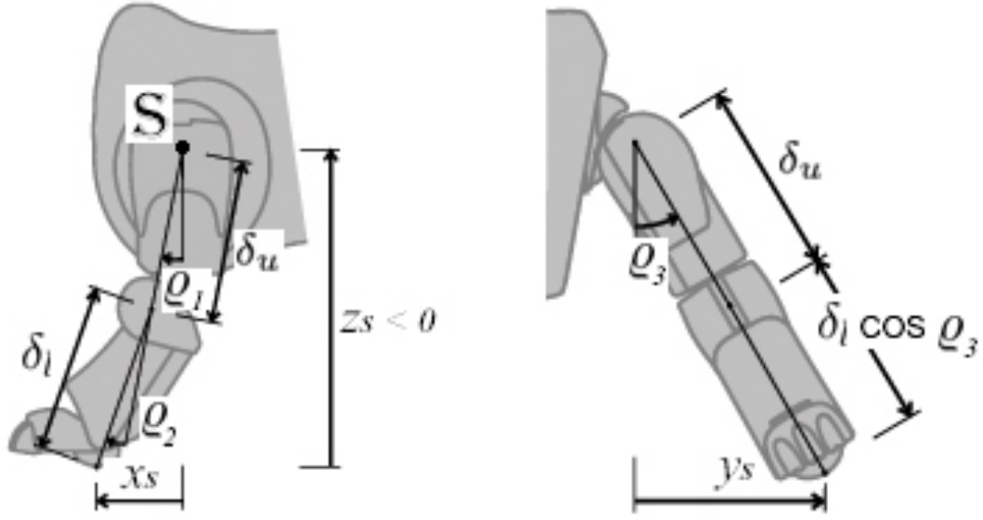
Figure 1.5: Fore left leg design: side view (left), and front view (right).
