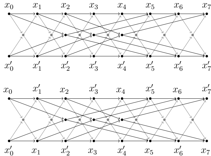
Figure 6.9: The two databases above are a proof that \mathbf{V} \not\rightarrow \mathbf{Q} = \langle n \rangle for any odd n that is not greater than 7. Indeed, we can check that both databases agree on \mathbf{V} . However, there is no path of length 1 (respectively 3, 5 and 7) from x_0 to x_1 (respectively x_3, x_5 and x_7 ) in the bottom database.
