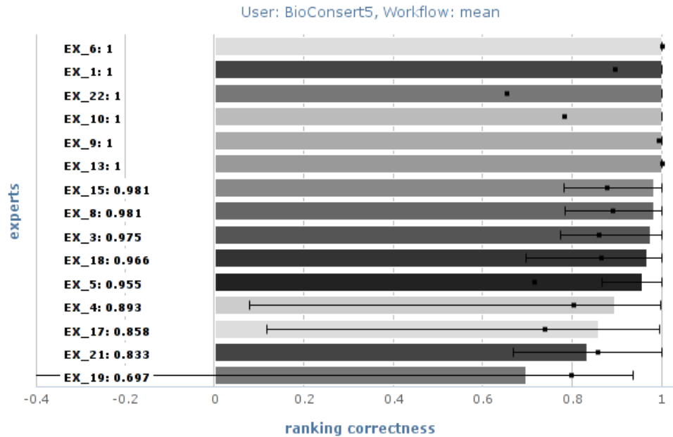
FIGURE 3.7 : Mean ranking correctness (bars) with upper and lower stddev (errorbars), and mean ranking completeness (black squares) for single experts' rankings compared to the ranking derived as BioConsert expert consensus.
