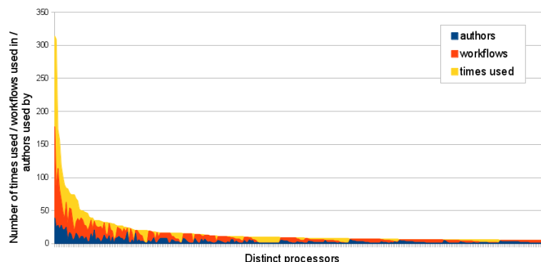
FIGURE 3.3 : Usage counts of the 300 most used processors showing a Zipf-like distribution.
