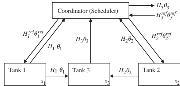
Figure 3. Physical decomposition of the heating system.
