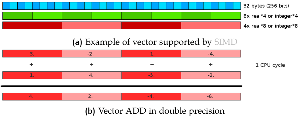
FIGURE 6 – SIMD schema
