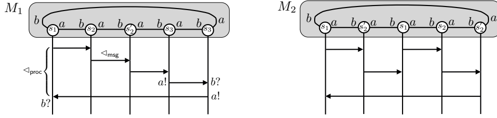
Figure 3.5: Two MSCs with a ring topology
