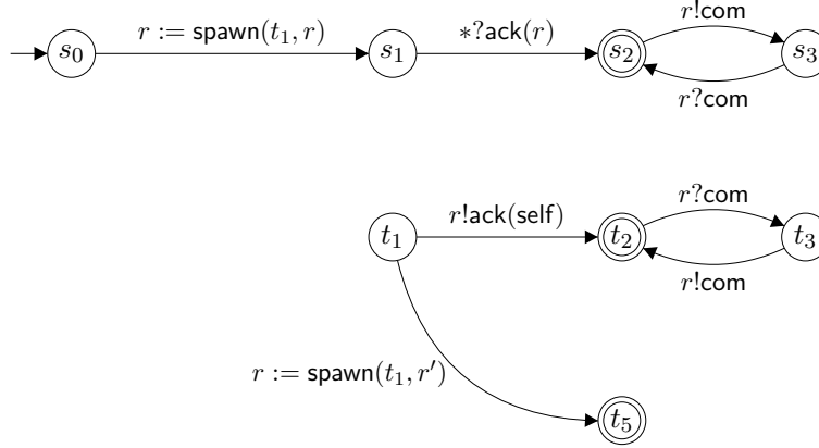
Figure 5.2: The DCA \mathcal{A}_{5.2} modeling a peer-to-peer protocol
