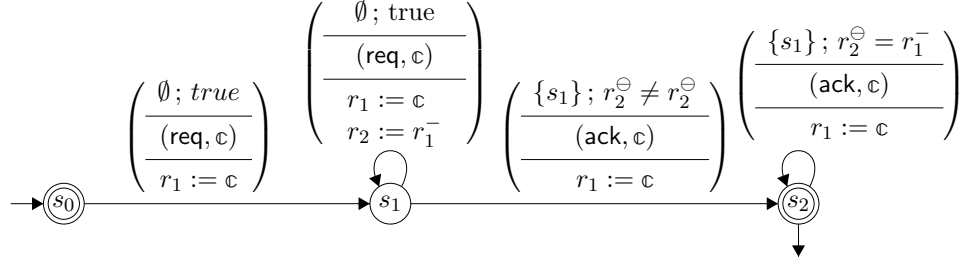
Figure 4.6: (Non-guessing) class register automaton \mathcal{A}_{4.6}
