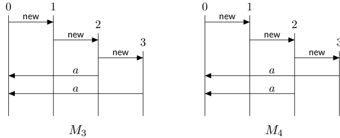
Figure 5.5: Realizability vs. Implementability
