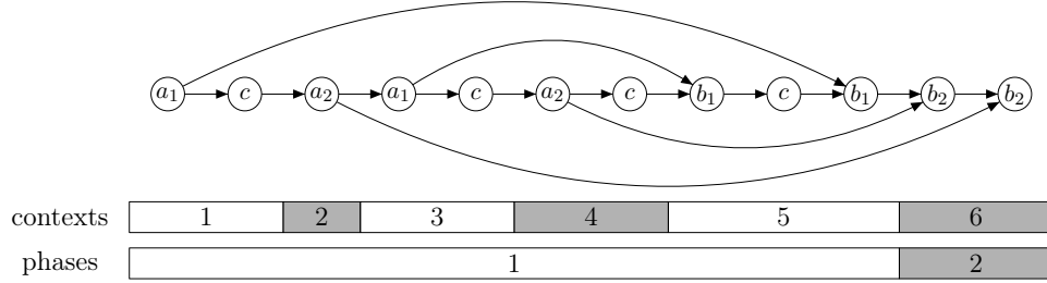
Figure 2.3: Illustration of context, phase, and scope
