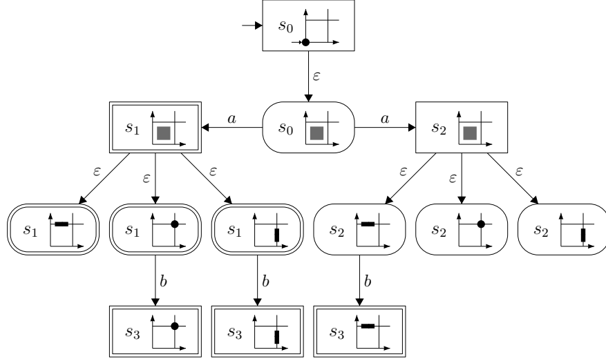
Figure 6.3: Part of the region automaton \mathcal{A}_\exists of the icTA \mathcal{A} from Figure 6.1
