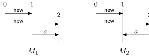
Figure 5.4: Implementability
