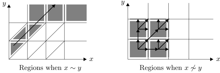
Figure 6.2: Region successors
