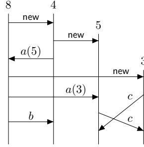
Figure 5.1: An MSC
