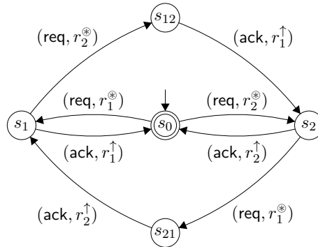
Figure 4.2: Session automaton \mathcal{A}_{4.2} for L_1 \cap \dots \cap L_5
