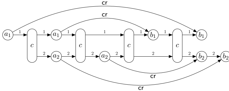
Figure 2.4: The nested trace T_{2.4}
