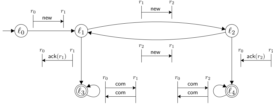
Figure 5.6: The rMSG \mathcal{H}_{5.6} modeling the peer-to-peer protocol
