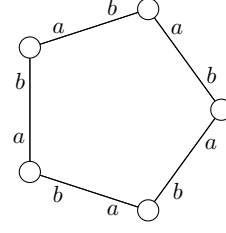
Figure 3.2: Ring
