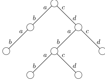
Figure 3.3: Tree topology
