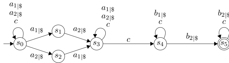
Figure 2.2: Nested-word automaton \mathcal{A}_{2.2}
