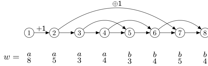
Figure 4.5: The relations \triangleleft_{+1} and \triangleleft_{\oplus 1}
