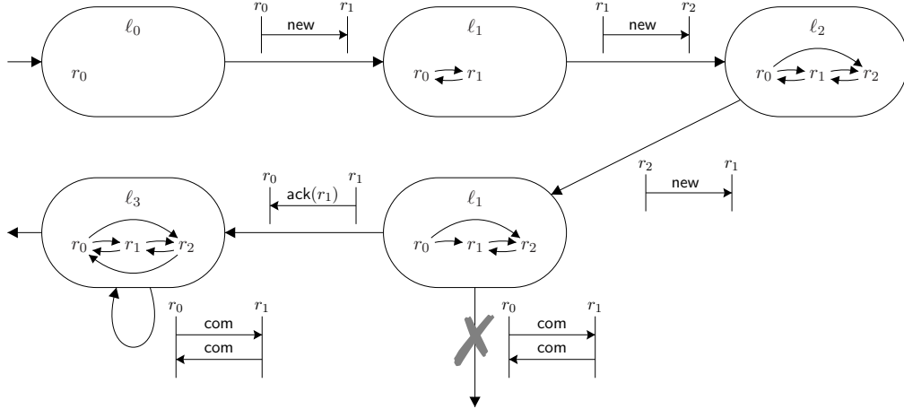
Figure 5.7: Part of the finite symbolic transition system associated with \mathcal{H}_{5.6}
