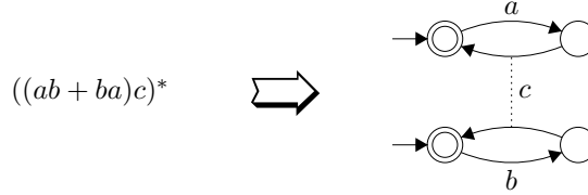
Figure 1.6: Realizability of concurrent finite-state systems
