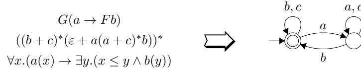
Figure 1.4: Realizability of sequential finite-state systems
