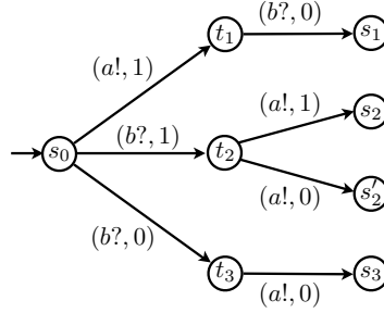
Figure 3.6: The PCA \mathcal{A}_{\text{token}}
