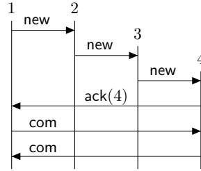
Figure 5.3: An MSC accepted by the DCA \mathcal{A}_{5.2}
