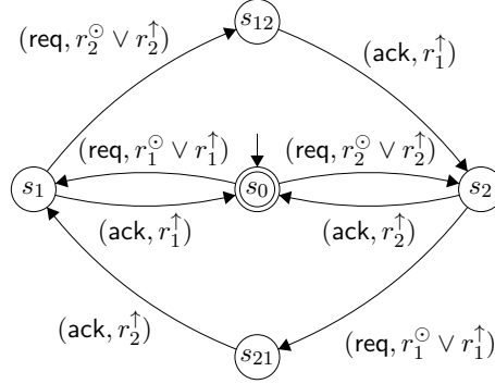
Figure 4.1: Register automaton \mathcal{A}_{4.1} for L_1 \cap \dots \cap L_4
