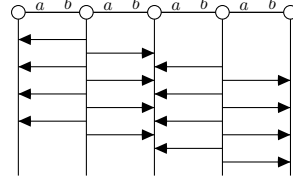
Figure 3.9: Grid encoding for \mathbf{s}\oplus\mathbf{r}
