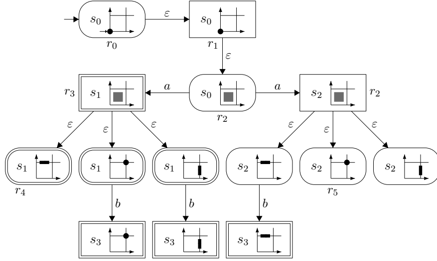
Figure 6.5: Part of the game \mathcal{G}(\mathcal{A}) of the icTA \mathcal{A} from Figure 6.1
