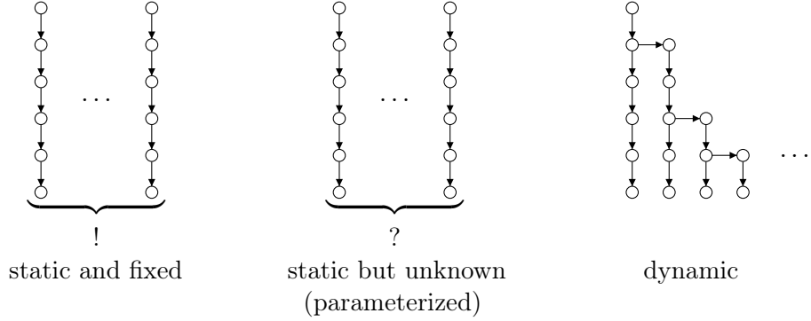
Figure 1.2: System architectures
