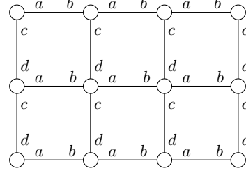
Figure 3.4: Grid
