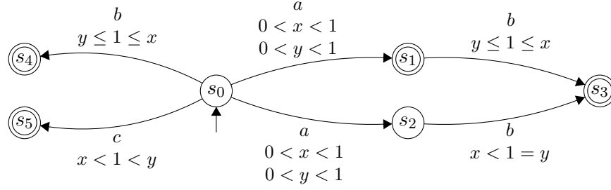
Figure 6.1: The icTA \mathcal{A} with independent clocks x and y
