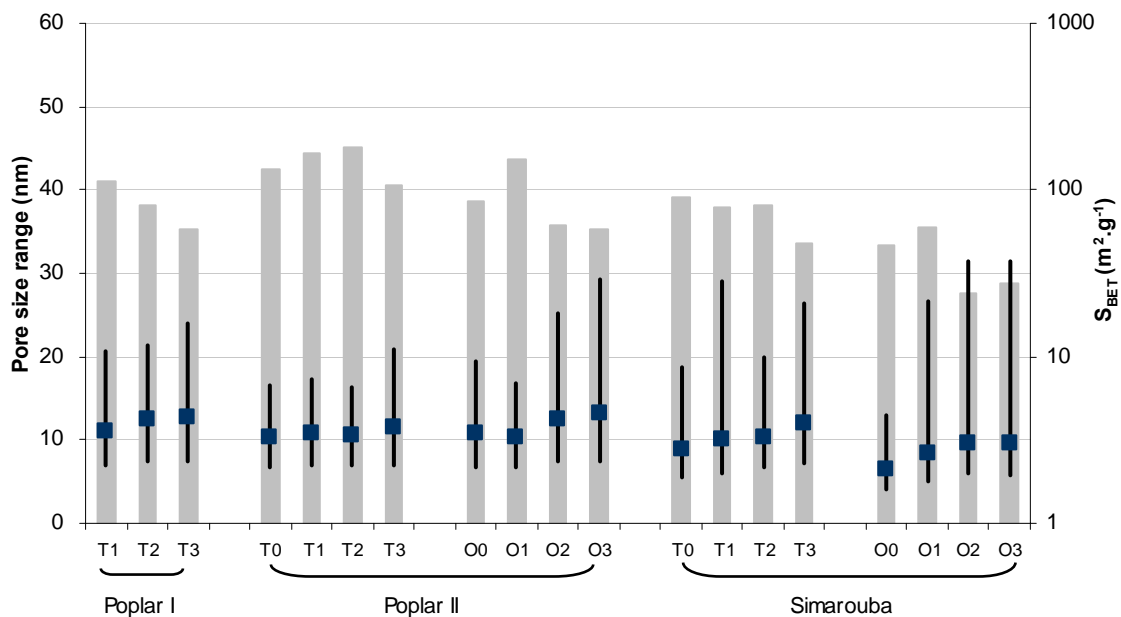
Figure 5.3 The median pore size (filled square), pore size range distribution (straight lines) and specific surface area, S_{\text{BET}} (grey histogram) of poplar and simarouba near cambium zone. (Poplar I and poplar II denote sample taken from tree I and II. The S_{\text{BET}} is shown in logarithmic scale. T0-T3: tension wood samples; O1-O3: opposite wood samples.)
