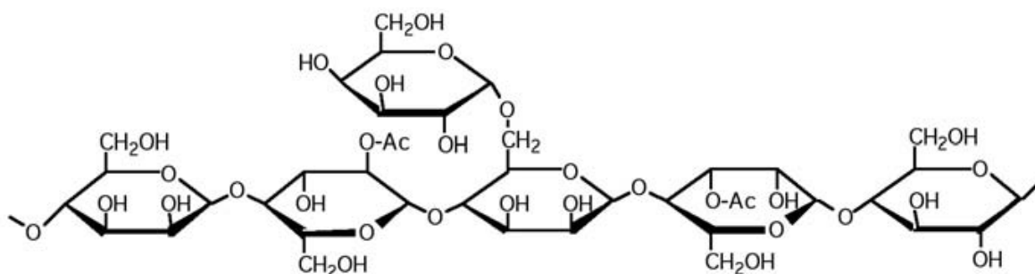
Figure 1.8 Partial chemical structure of O-acetyl-galactoglucomannan of softwood (from Navi and Sandberg 2012)
