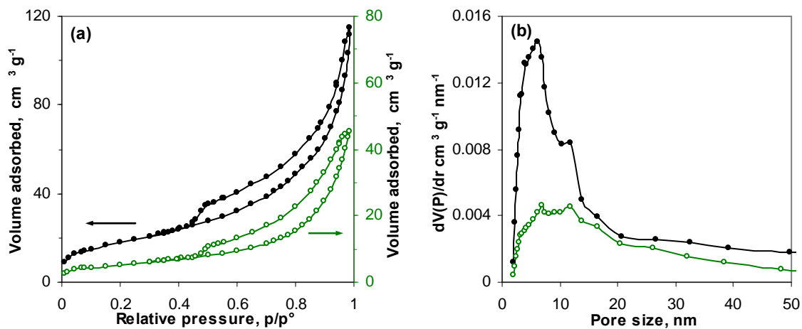
Figure 3 (a) N 2 adsorption-desorption isotherms at 77 K and (b) pore size distributions for poplar tension wood (green curves with open symbols), G-layers extracted from the same tension wood sample with 15min sonication (G15, black curves with solid symbols)
