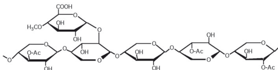
Figure 1.7 Partial chemical structure of O-acetyl-4-O-methylglucuronoxylan of hardwood (from Navi and Sandberg 2012)
