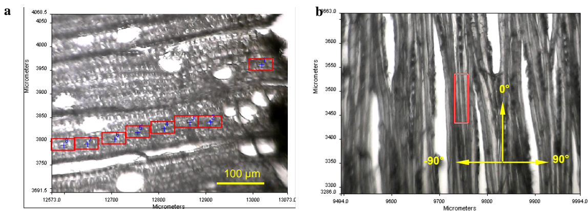
Figure 2 Visible images of transverse (a) and tangential (b) sections of poplar tension wood showing the measuring area (a: 50×25 µm, R×T; b: 25×100 µm, T×L) and the polarization directions of the measurement
