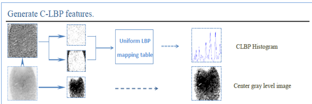
Figure 4.6 – Procedure of calculating CLBP feature.
