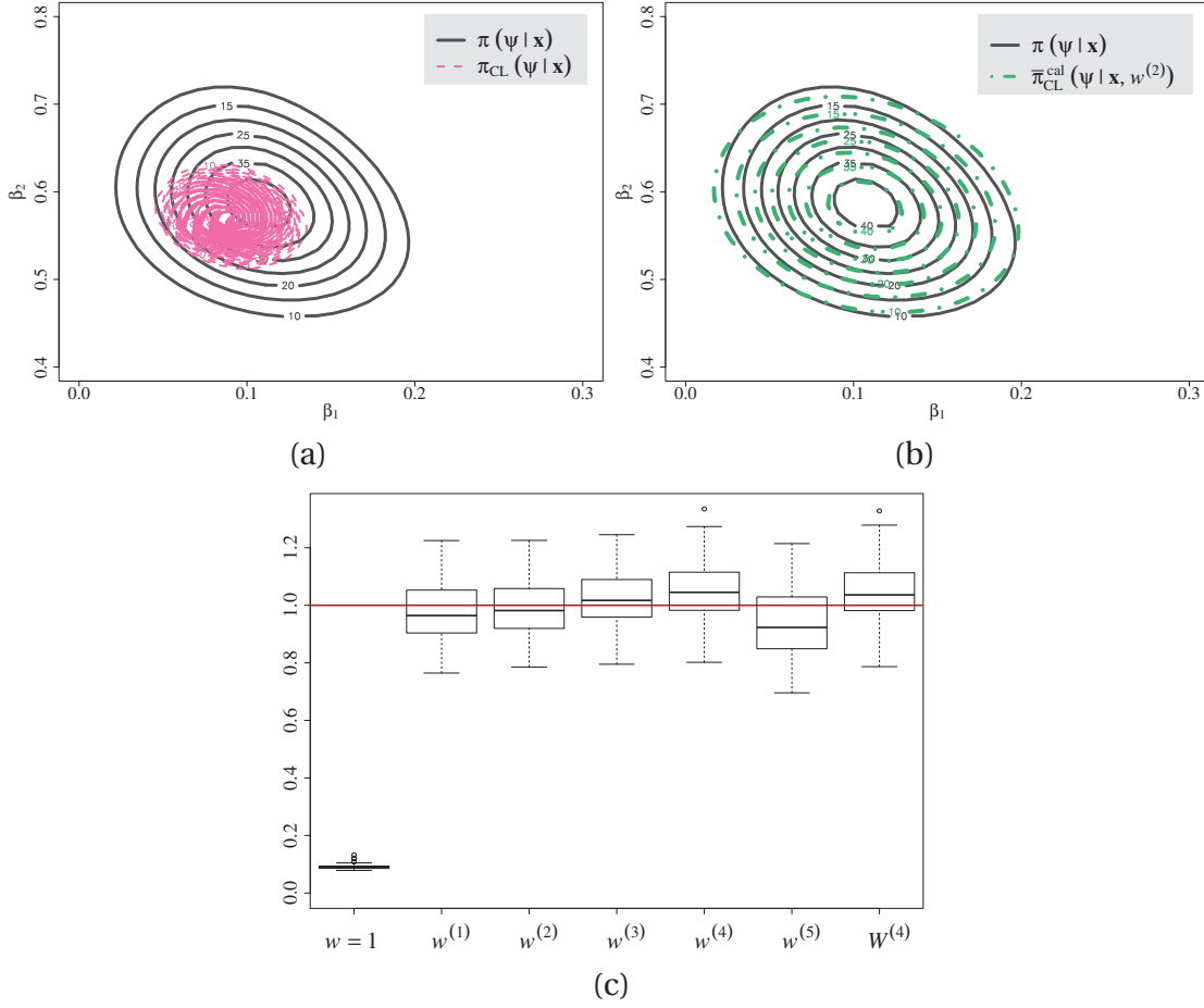
Figure 2.3: Second experiment results. (a) Posterior parameter distribution (grey) and non-calibrated composite posterior parameter distribution (pink) for a first-order anisotropic Ising model. (b) Posterior parameter distribution (grey) and composite posterior parameter distribution (green) with mode and magnitude adjustments ( w = w^{(2)} ). (c) Boxplots displaying \frac{1}{\sqrt{2}} \|\text{Var}_{\text{CL}}(\theta) \text{Var}^{-1}(\theta)\|_F for 100 realisations of an anisotropic first-order Ising model.
