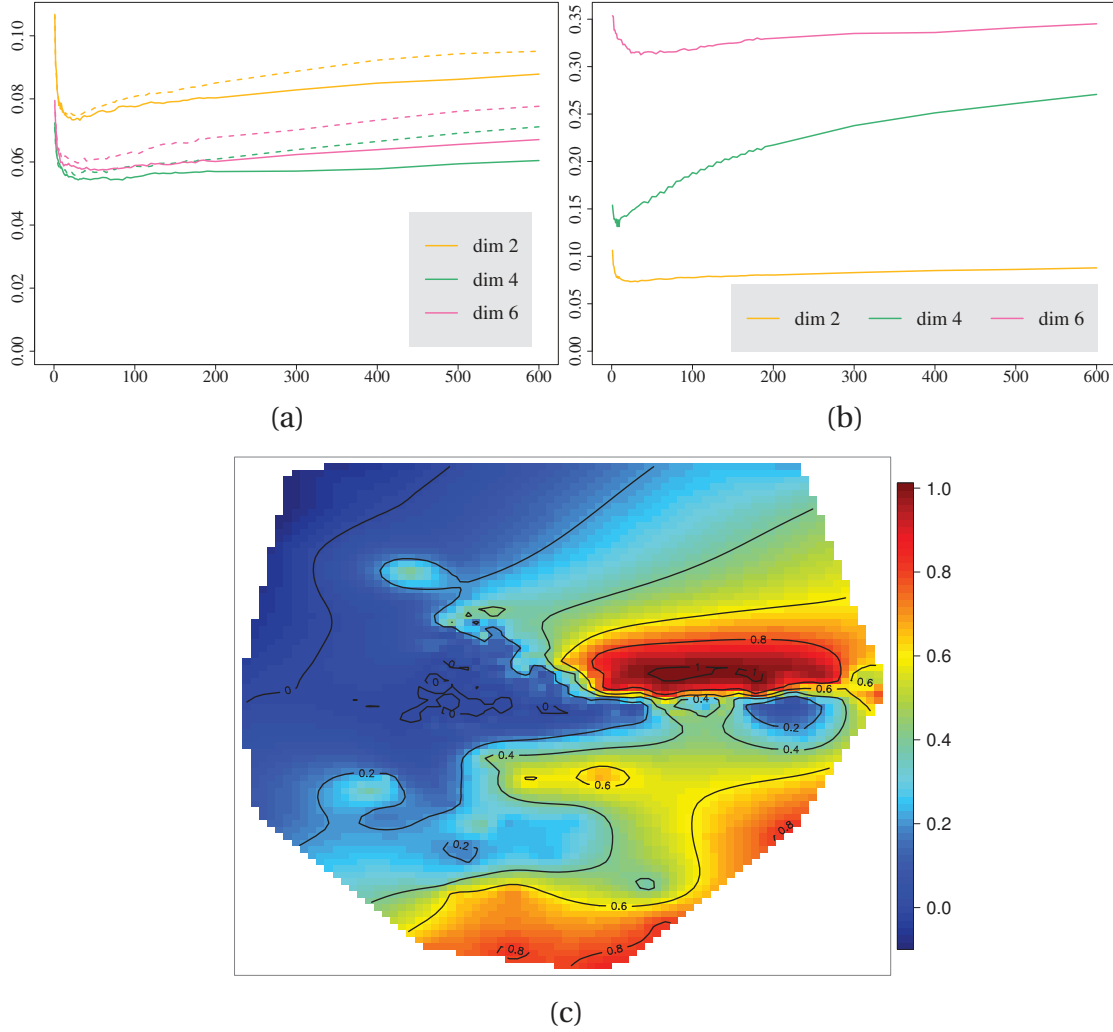
Figure 3.2: First experiment results. (a) Prior error rates (vertical axis) of ABC with respect to the number of nearest neighbors (horizontal axis) trained on a reference table of size 100,000 (solid lines) or 50,000 (dashed lines), based on the 2D, 4D and 6D summary statistics. (b) Prior error rates of ABC based on the 2D summary statistic compared with 4D and 6D summary statistics including additional ancillary statistics. (c) Evaluation of the local error on a 2D surface.
