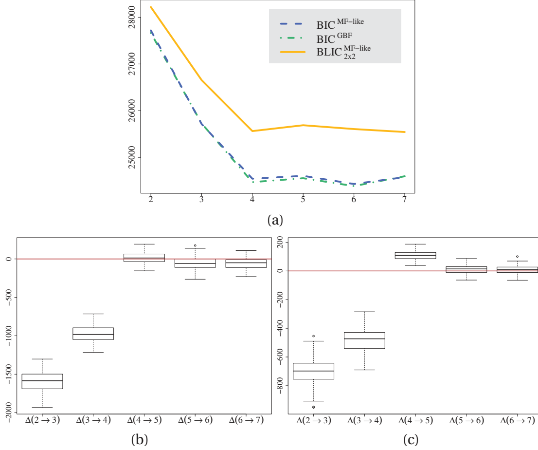
Figure 4.1: First experiment results. (a) \text{BIC}^{\text{MF-like}} , \text{BIC}^{\text{GBF}} and \text{BLIC}_{2 \times 2}^{\text{MF-like}} values for one realization of a first order hidden Potts model \text{HPM}(\mathcal{G}, \theta, 4) . (b) Difference between \text{BLIC}_{2 \times 2}^{\text{MF-like}} values for 100 realization of a first order hidden Potts model \text{HPM}(\mathcal{G}_4, \theta, 4) as K is increasing. (c) Difference between \text{BLIC}_{2 \times 2} values for 100 realization of a first order hidden Potts model \text{HPM}(\mathcal{G}_4, \theta, 4) as K is increasing
