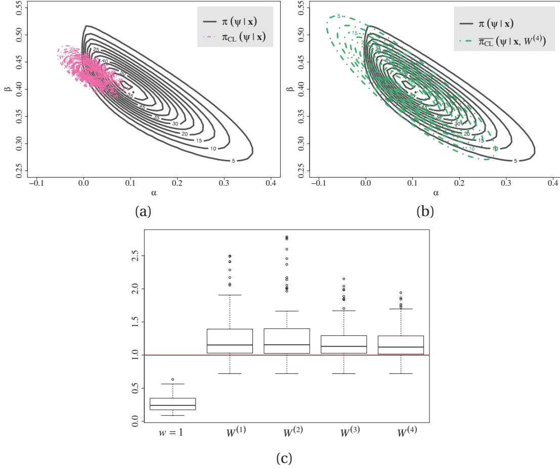
Figure 2.4: Third experiment results. (a) Posterior parameter distribution (grey) and non-calibrated composite posterior parameter distribution (pink) for a first-order autologistic model. (b) Posterior parameter distribution (grey) and composite posterior parameter distribution (green) with mode and curvature adjustments ( W = W^{(4)} ). (c) Boxplots displaying \frac{1}{\sqrt{2}} \|\text{Var}_{\text{CL}}(\psi) \text{Var}^{-1}(\psi)\|_{\text{F}} for 100 realisations of a first-order autologistic model.
