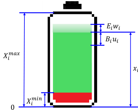
Figure 2.3: Definitions related to the battery energy at time t , where X_i^{max} is the maximum energy in the battery; X_i^{min} is the minimum energy in the battery; x_i is the remaining energy in the battery; E_i w_i is the energy possibly harvested during [kT_c, (k+1)T_c] ; and B_i u_i is the energy consumed during [kT_c, (k+1)T_c]
