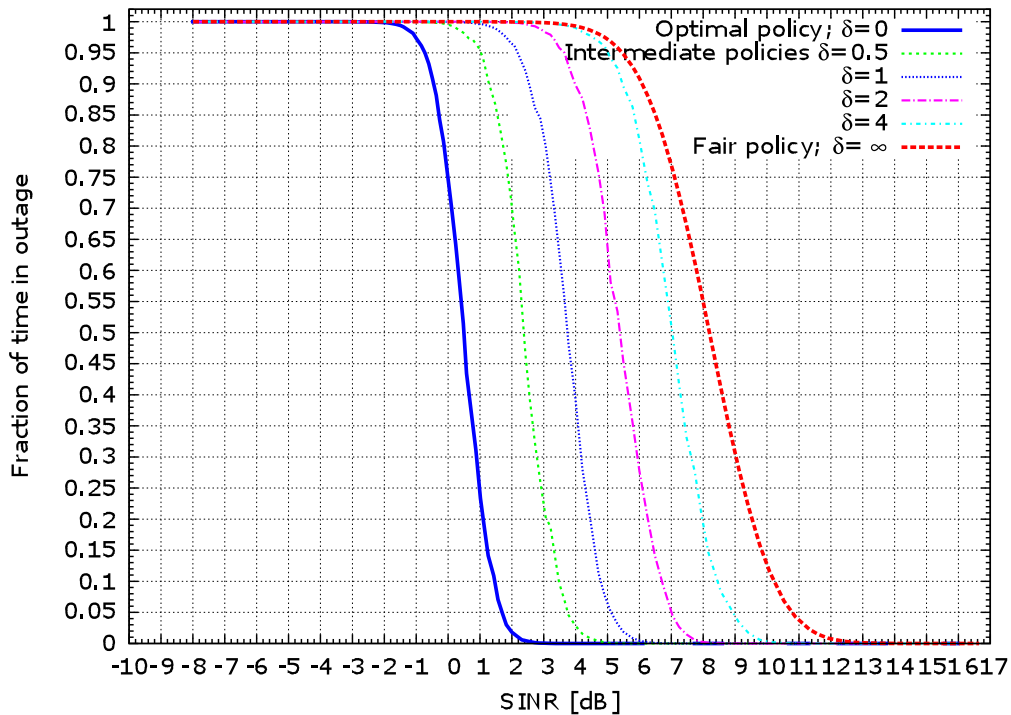
Figure 4.2: Mean fraction of the requested streaming time in outage, as function of the user SINR for different policies \text{LESF}(\delta) ; traffic 900 Erlang/km 2 .
