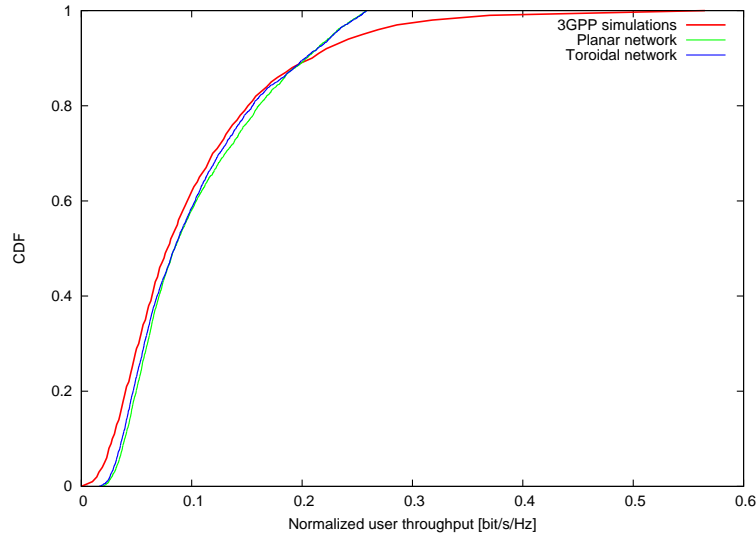
Figure 2.8: CDF of normalized user throughput
