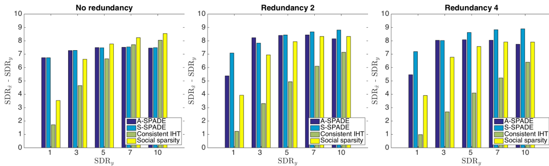
Figure 2.3 – SDR improvement \nu s redundancy for all algorithms.
