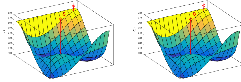
Figure 5.2 – The original sound speed (left) c and the estimate (right) \hat{c} (the diamond markers indicate the source spatial positions).
