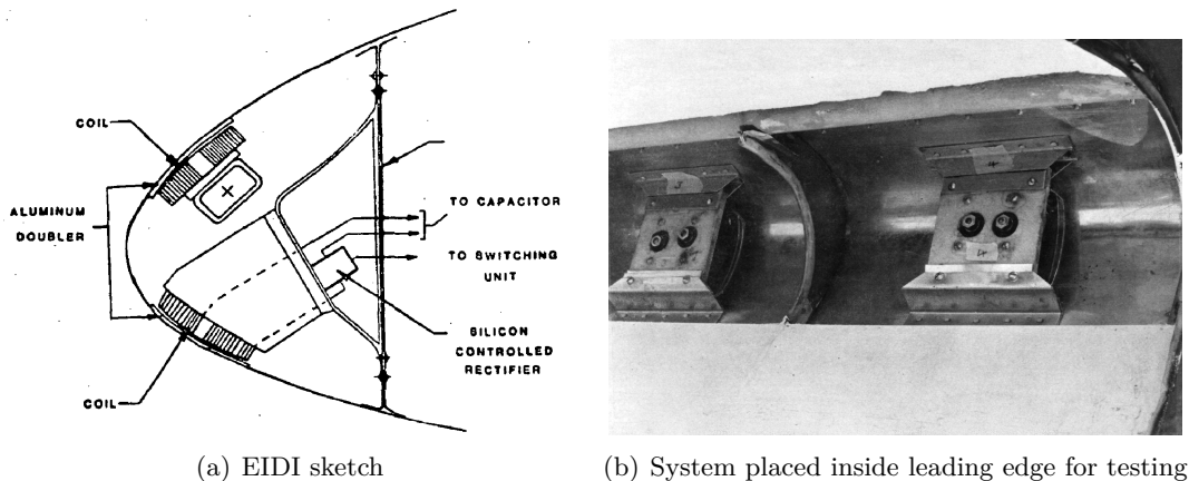
Figure 1.21: Electro-Impulse De-Icing mechanical system [45]
