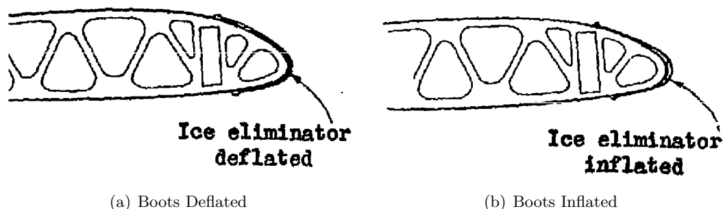
Figure 1.18: De-Icing Boots [151]
