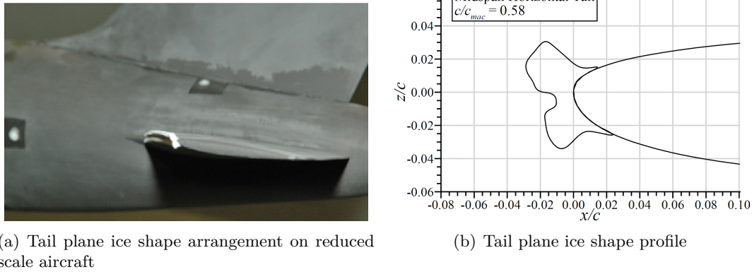
Figure 1.10: Tail plane ice shape for aerodynamic study on reduced scale aircraft [6]
