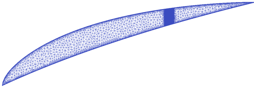
Figure 5.14: Airfoil mesh
