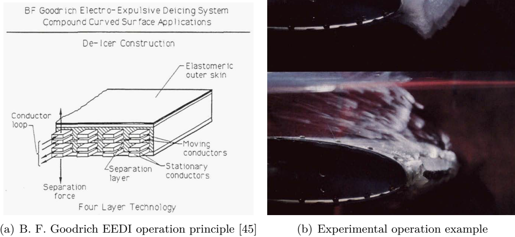
Figure 1.20: Electro-Expulse De-Icing mechanical system
