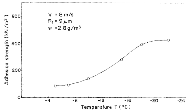
Figure 4.17: Temperature effect [59]
