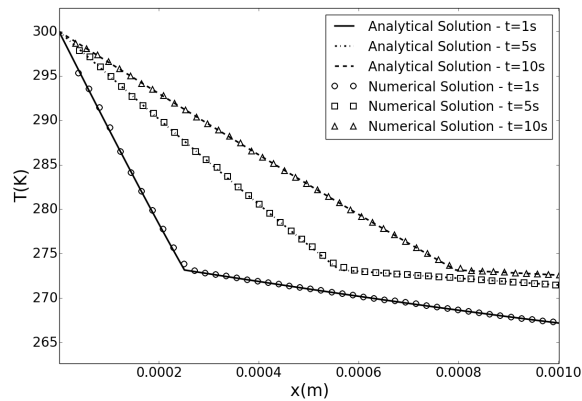
Figure 2.24: Comparison of analytical and numerical temperature profiles for the fine mesh
