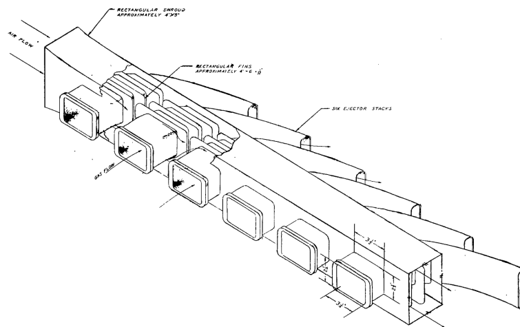
Figure 1.24: Jurgen Ju-88 Heat Exchanger [77]
