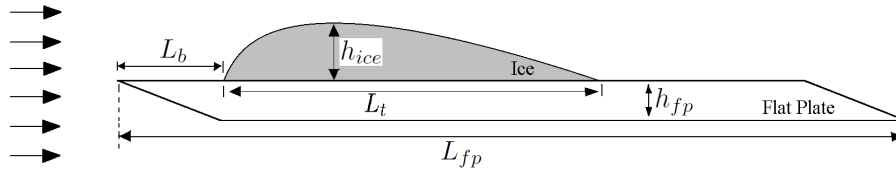
Figure 5.9: Flat Plate Test Case
