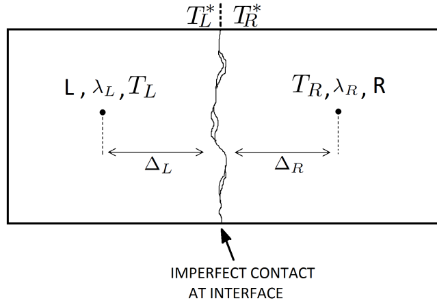
Figure 2.6: Imperfect contact
