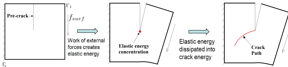
Figure 3.6: Energy transfer in crack opening mode
