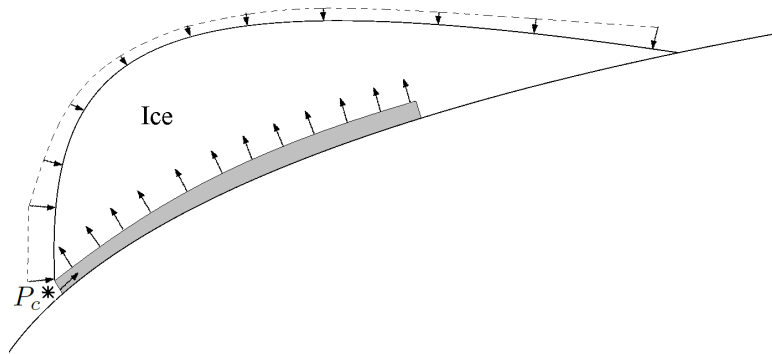
Figure 5.3: Schematic Pressure Distribution
