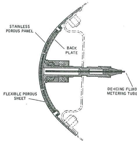
Figure 1.33: Illustration of a chemical injection ice protection system
