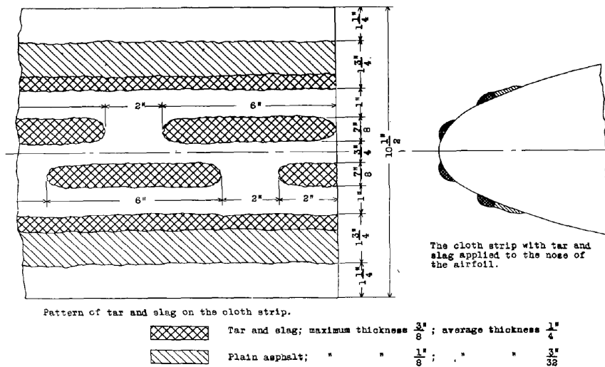
Figure 1.8: Simulated ice shape arrangement [16]
