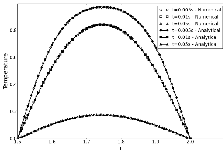
Figure 2.12: Analytical and numerical solution on mesh no 3 for the different time steps
