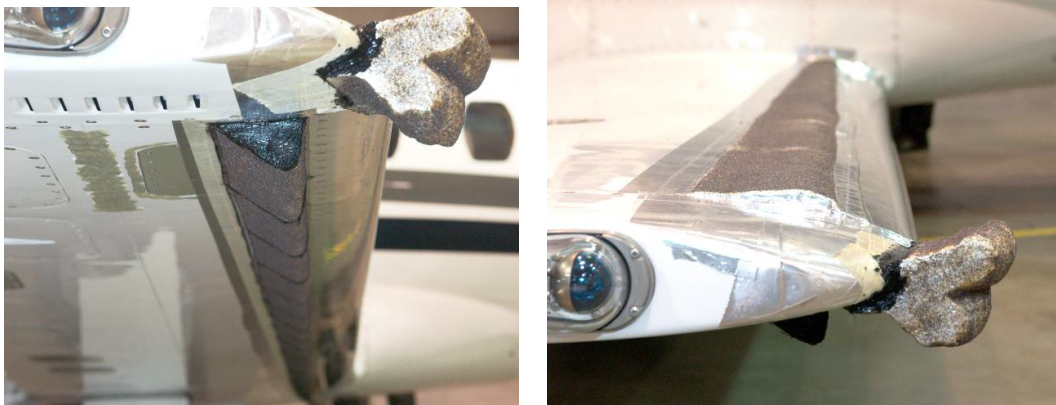
(a) Lower runback ice shapes and horns
