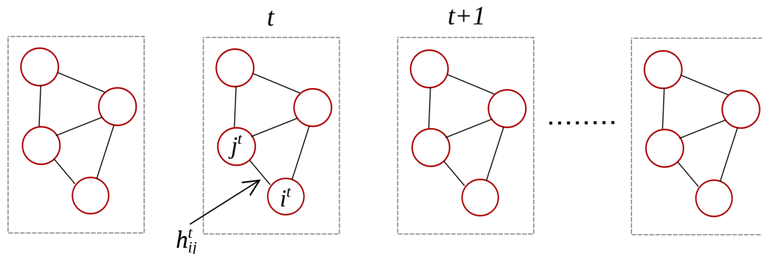
FIGURE 7.2: Static graph representation.
