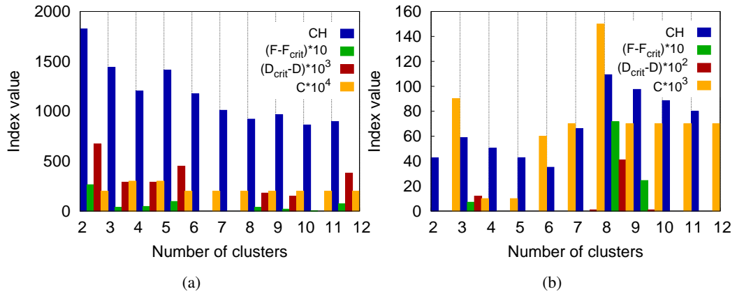
FIGURE 4.7: Clustering indices versus the number of clusters for a training set of two weeks according to: (a) the traffic volume distance measure \mathcal{V} , (b) the traffic distribution distance measure \mathcal{D} .
