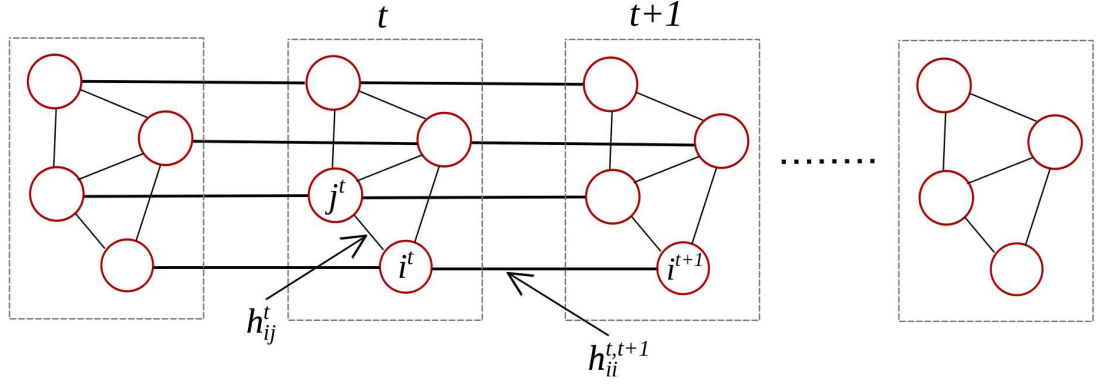
FIGURE 7.4: Time-varying graph representation.
