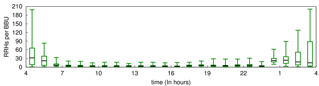
FIGURE 7.9: Distribution of the number of RRHs per BBU, over the day. The candlesticks show the median, minimum and maximum values, together with the first and third quartile for values obtained over each six hourly frames.
