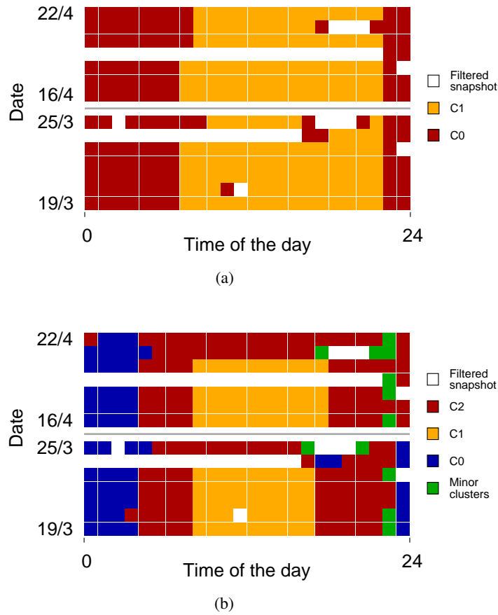
FIGURE 4.8: Content of mobile traffic profile categories defined on the training set \mathcal{S}' composed of the two weeks March 19th–25th and April 16th–22nd, 2012, according to: (a) the traffic volume distance measure \mathcal{V} and (b) the traffic distribution distance \mathcal{D} . Each square represents one snapshot, whose category maps to a color. White squares refer to snapshots that were filtered out from the dataset as discussed in Chapter 2.
