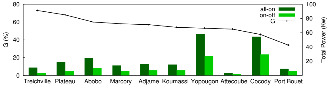
FIGURE 6.3: The obtained gain ( G ) when switch-on/off strategy is applied to define geographical coverage BS configuration, with respect to the all-on strategy. The figure also portrays the total power consumption per commune, for each case.
