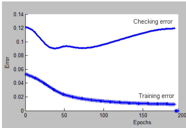
Figure 29: Error evolution during the training process. The error on the training dataset constantly decreases (bottom curve), while the error on the checking dataset begins to increase after the 38th epoch.
