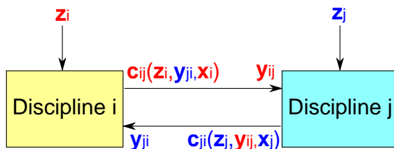
Figure 1.4: Couplings between the discipline i and the discipline j
