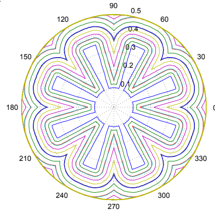
Figure 8.32: Curves of iso-combustion depth for the star grain
