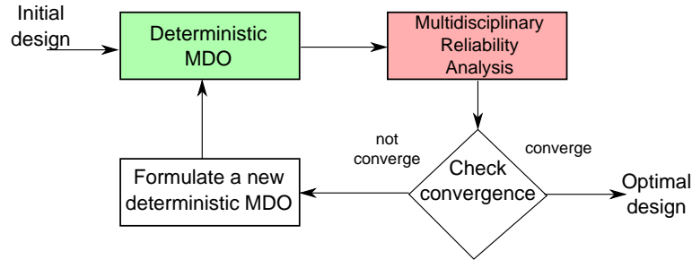
Figure 3.5: SORA procedure for UMDO [Du et al., 2008]
