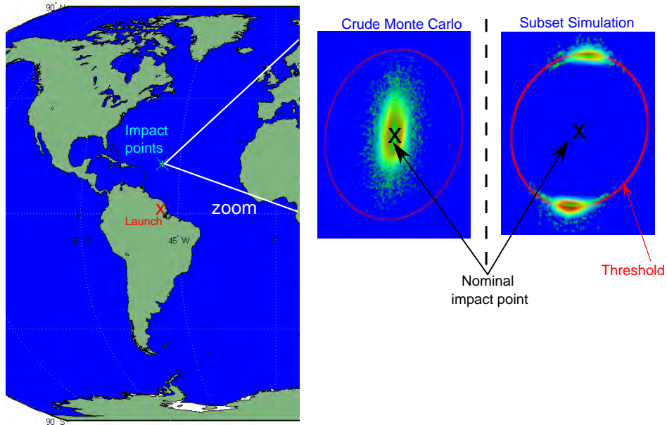
Figure 11.16: Impact points of the launch vehicle 2 nd stage
