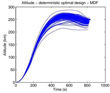
Figure 8.9: Uncertainty propagation - trajectory altitude - deterministic optimal launch vehicle
