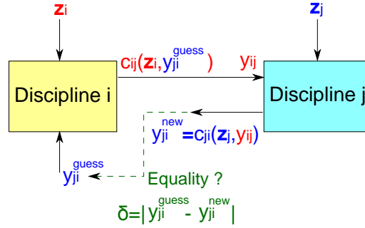
Figure 1.8: FPI between the discipline i and the discipline j
