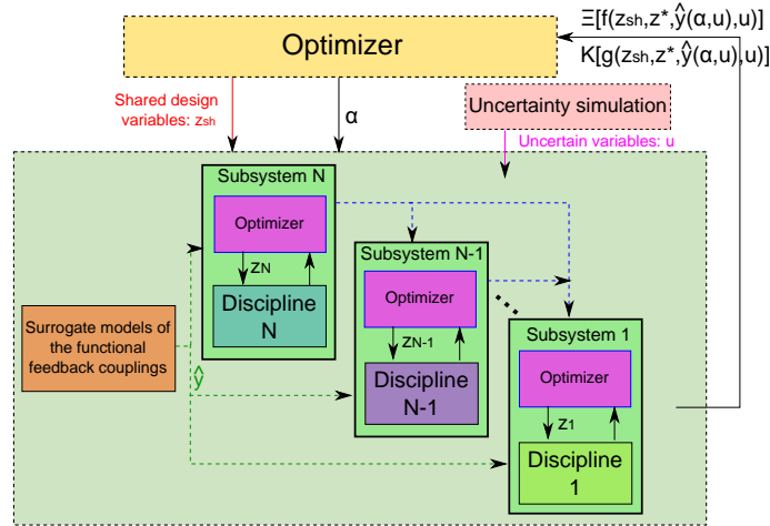
Figure 18.12: Multi-level Hierarchical Optimization under Uncertainty (MHOU)
