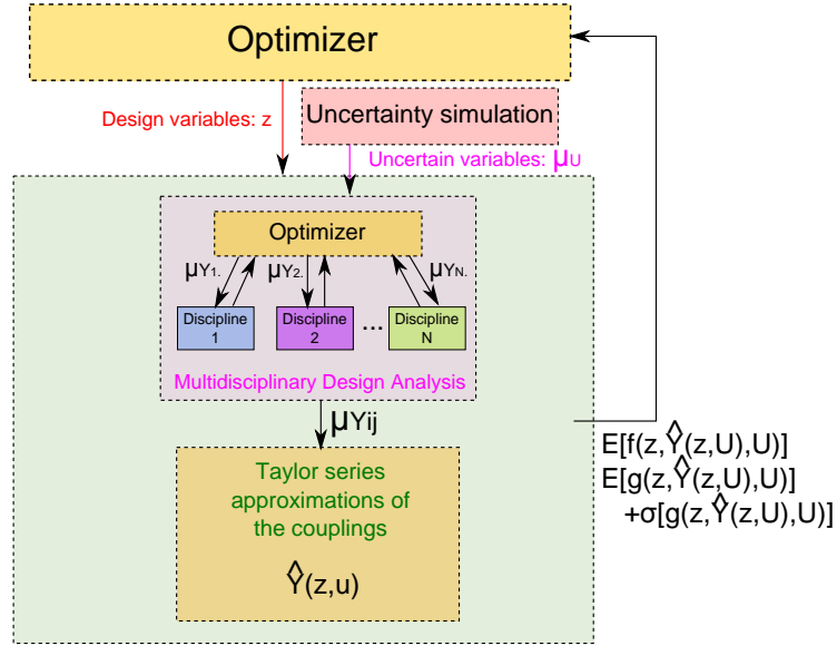
Figure 3.3: Concurrent SubSystem Uncertainty Analysis (CSSUA)
