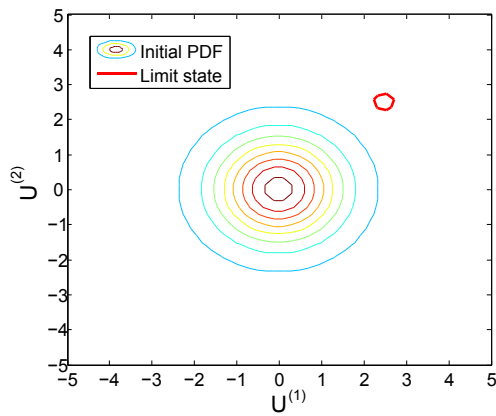
Figure 9.3: Initial PDF and limit state function
