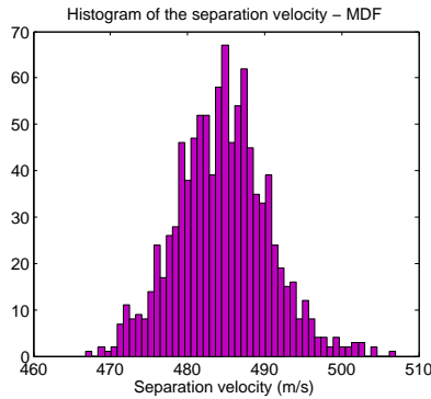
Figure 8.40: Distribution of the separation velocity for the optimal MDA solution - by
