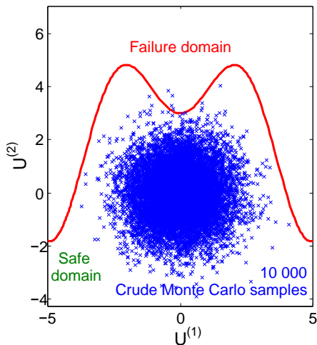
Figure 2.17: Exemple of CMC probability estimation
