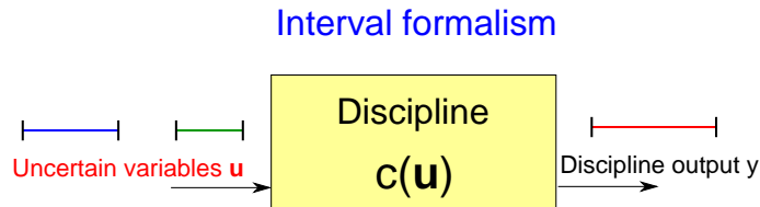
Figure 2.14: Uncertainty propagation with interval formalism
