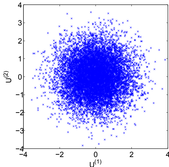
Figure 2.9: CMC samples input space
