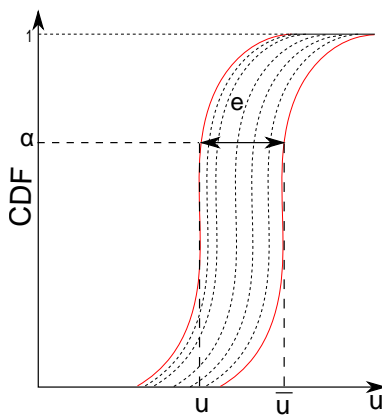
Figure 4.3: Probability boxes
