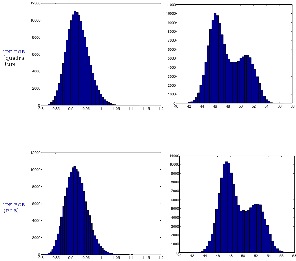
Figure 6.9: Distribution of the performance f(\cdot) (left column) and the coupling variable Y_{12} (right column) estimated from 150000 \mathbf{U} samples with IDF-PCE (quadrature) and IDF-PCE (PCE)
