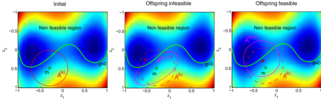
Figure 5.3: The green dot is the parent, the red dot is the generated offspring. On the left, the solid line circle is characterized by \mathbf{A}^{[k]} defining the ellipsoid delimiting an iso-probability search hypervolume. At the center, the pink ellipsoid represents the update of \mathbf{A}^{[k+1]} in order to take into account the constraint violation by the offspring. On the right figure, the offspring does not violate the constraint resulting in a standard covariance matrix update.
