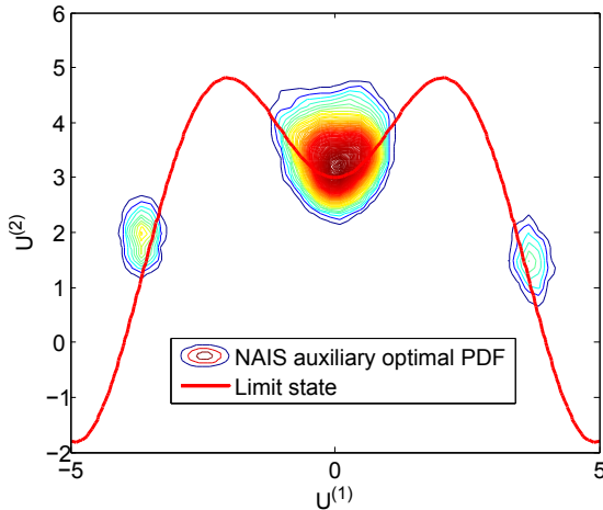
Figure 2.22: NAIS optimal auxiliary PDF isocountour
