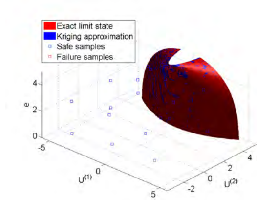
Figure 10.10: Final training set, exact limit state and kriging approximation
