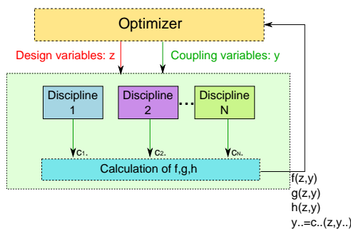
Figure 1.7: Multidisciplinary Design Optimization, decoupled approach
