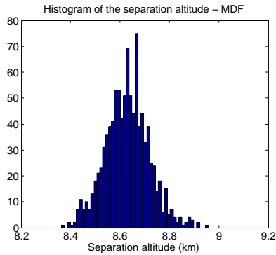
Figure 8.38: Distribution of the separation altitude for the optimal MDA solution - by
