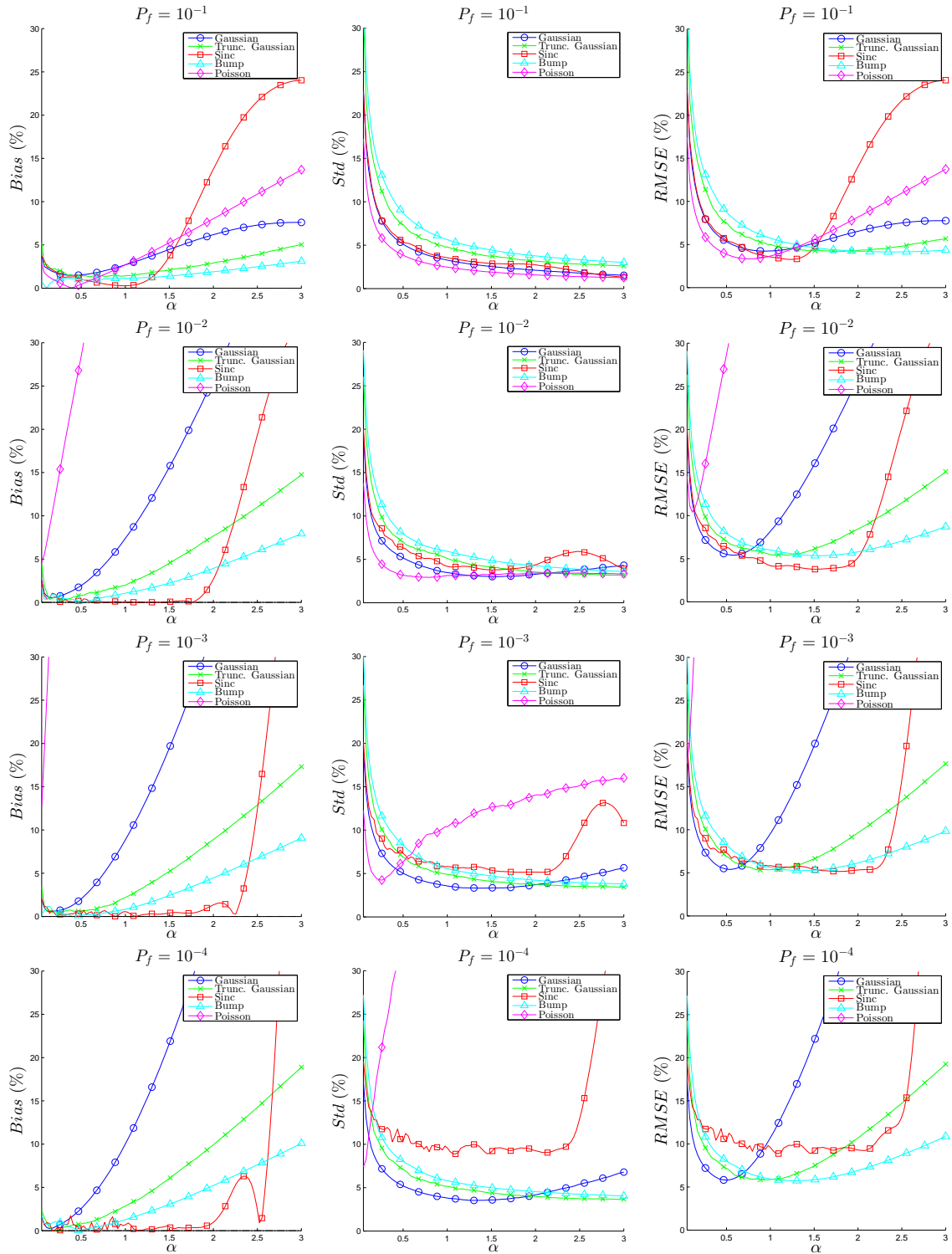
Figure 10.2: Normalized bias ( Bias ), standard error ( Std ) and root mean square error ( RMSE ) for 4 level of probability of failure.
