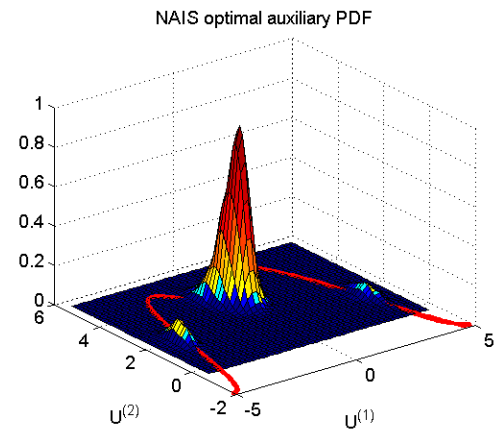
Figure 2.23: NAIS optimal auxiliary PDF
