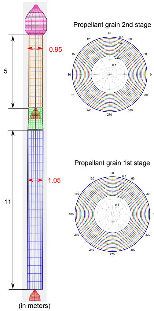
Figure 13.6: Optimal two stage booster design with modified CMA-ES(\lambda, \mu) and solid grain propellant configuration.
