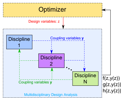
Figure 18.1: Multidisciplinary Design Optimization, approche couplée
