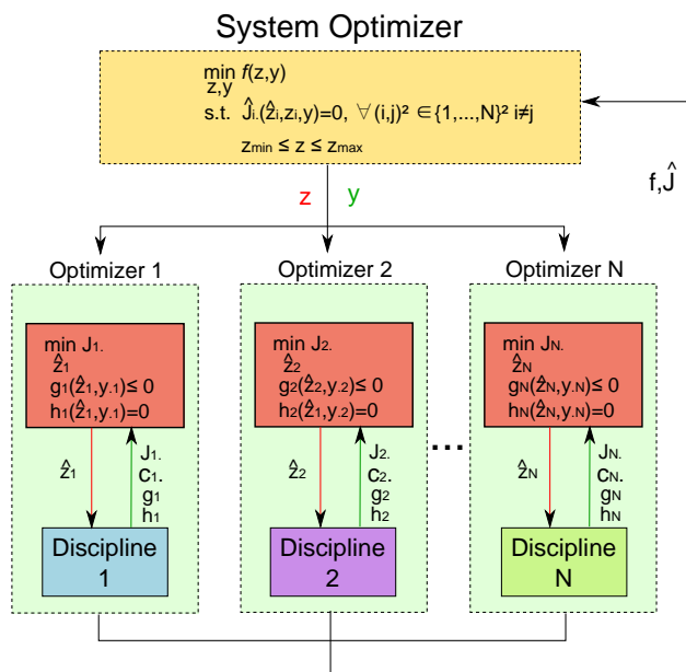
Figure 1.14: CO method
