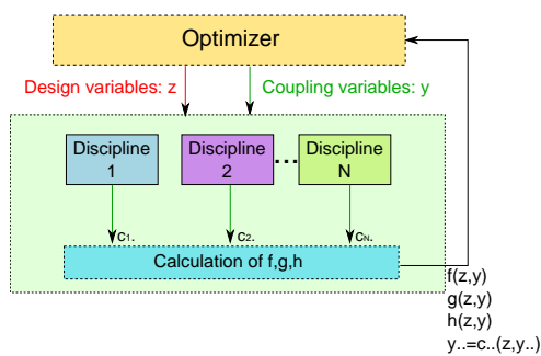
Figure 1.7: Multidisciplinary Design Optimization, decoupled approach
