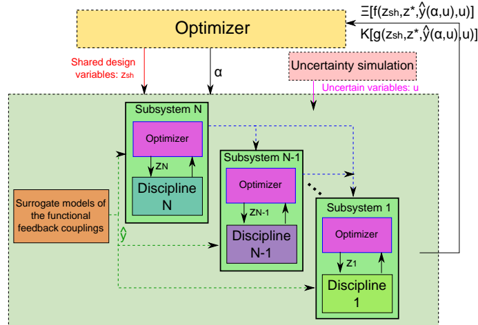
Figure 18.12: Multi-level Hierarchical Optimization under Uncertainty (MHOU)
