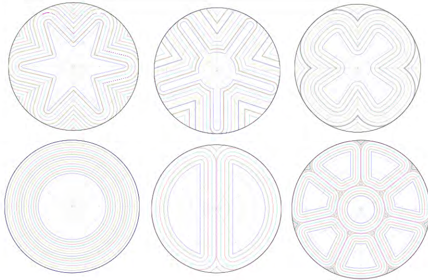
Figure 15.2: Curves of iso-combustion depth for different grain configurations
