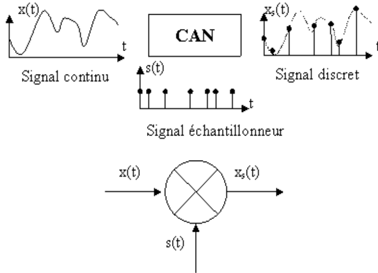
Figure II.1: Echantillonneur idéal
