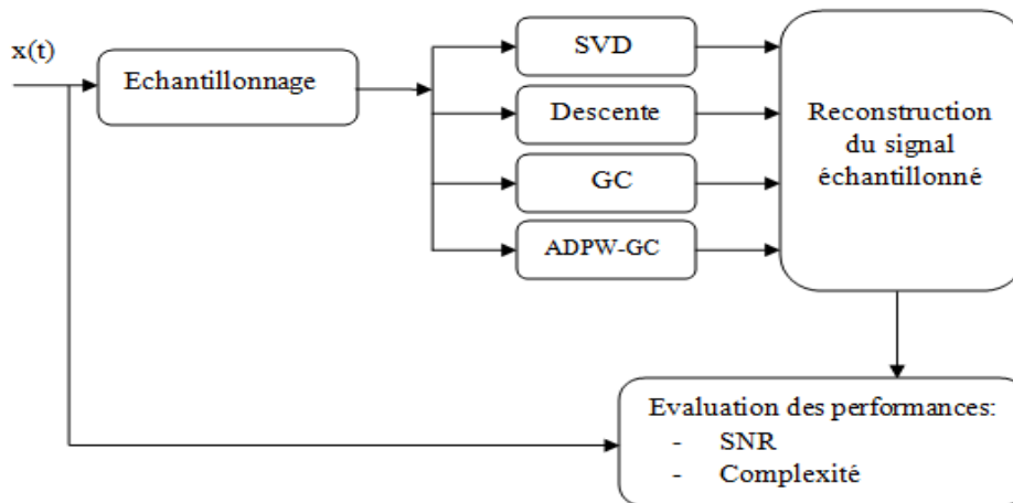
Figure II.12: Schéma bloc de simulation
