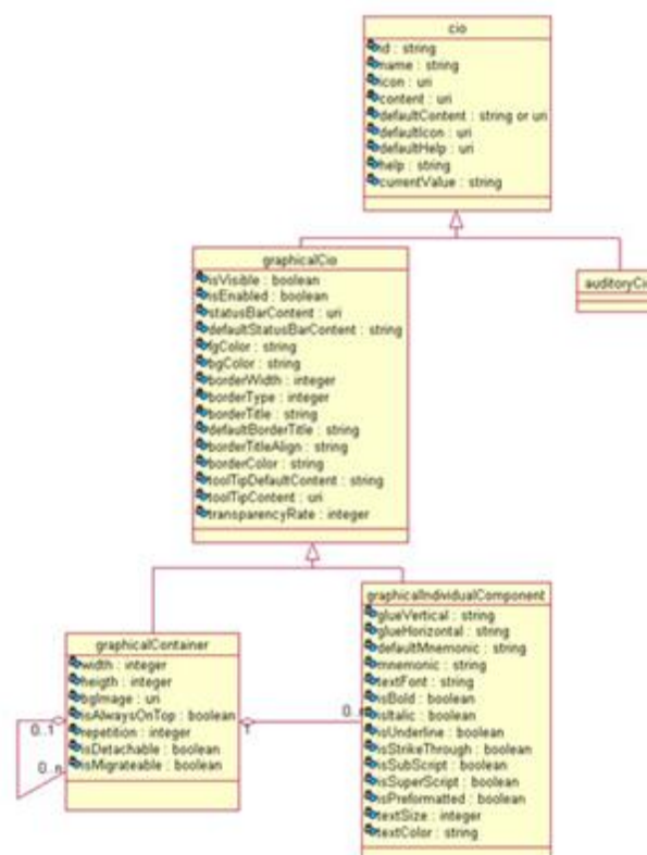
Figure 22. Concrete Interaction Objects in UsiXML: upper part of the hierarchy.
