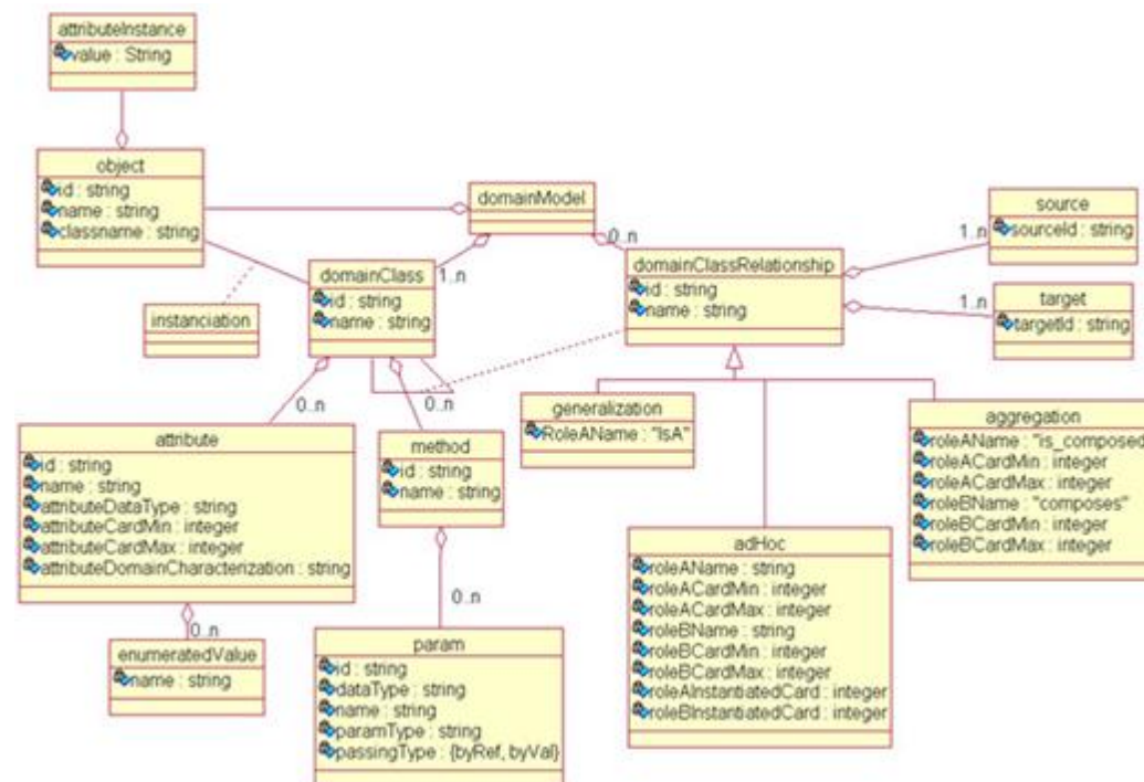
Figure 20. Meta-model of the UsiXML domain model.
