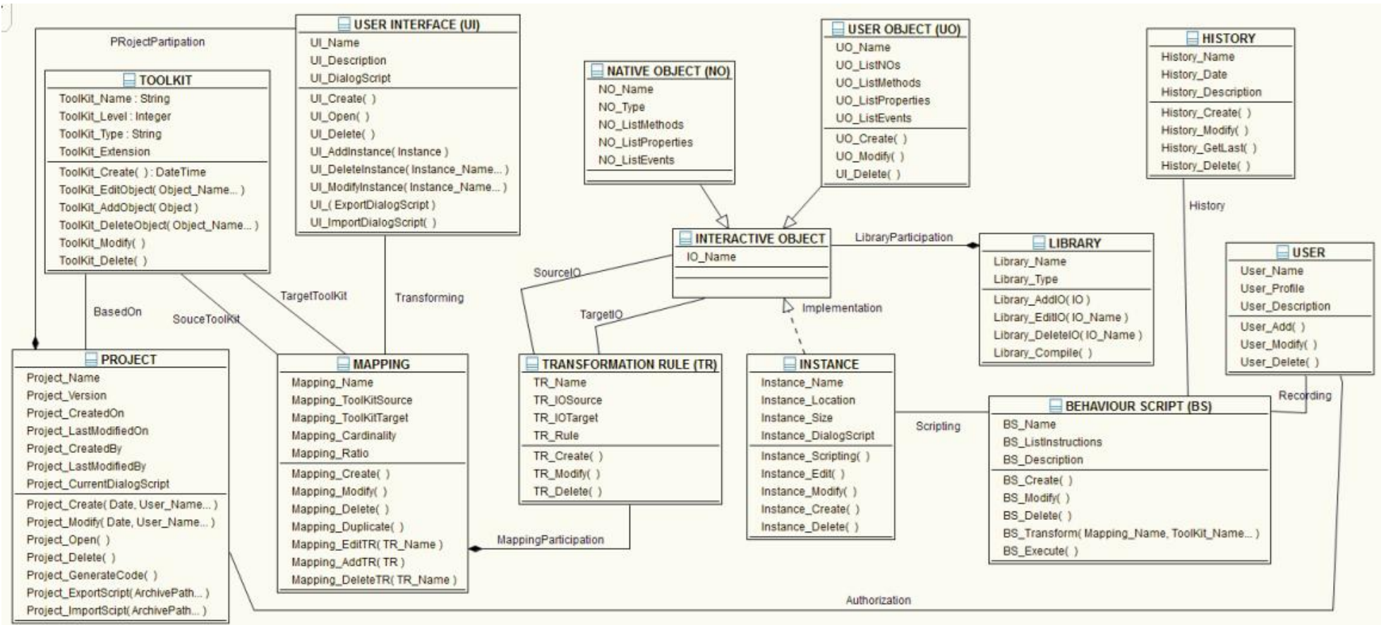
Figure 34. Conceptual modelling of behaviours for model-driven engineering.
