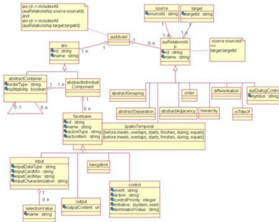
Figure 21. Meta-model of the UsiXML Abstract User Interface.
