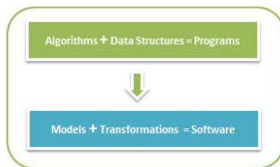
Figure 15. MDE Equation.
