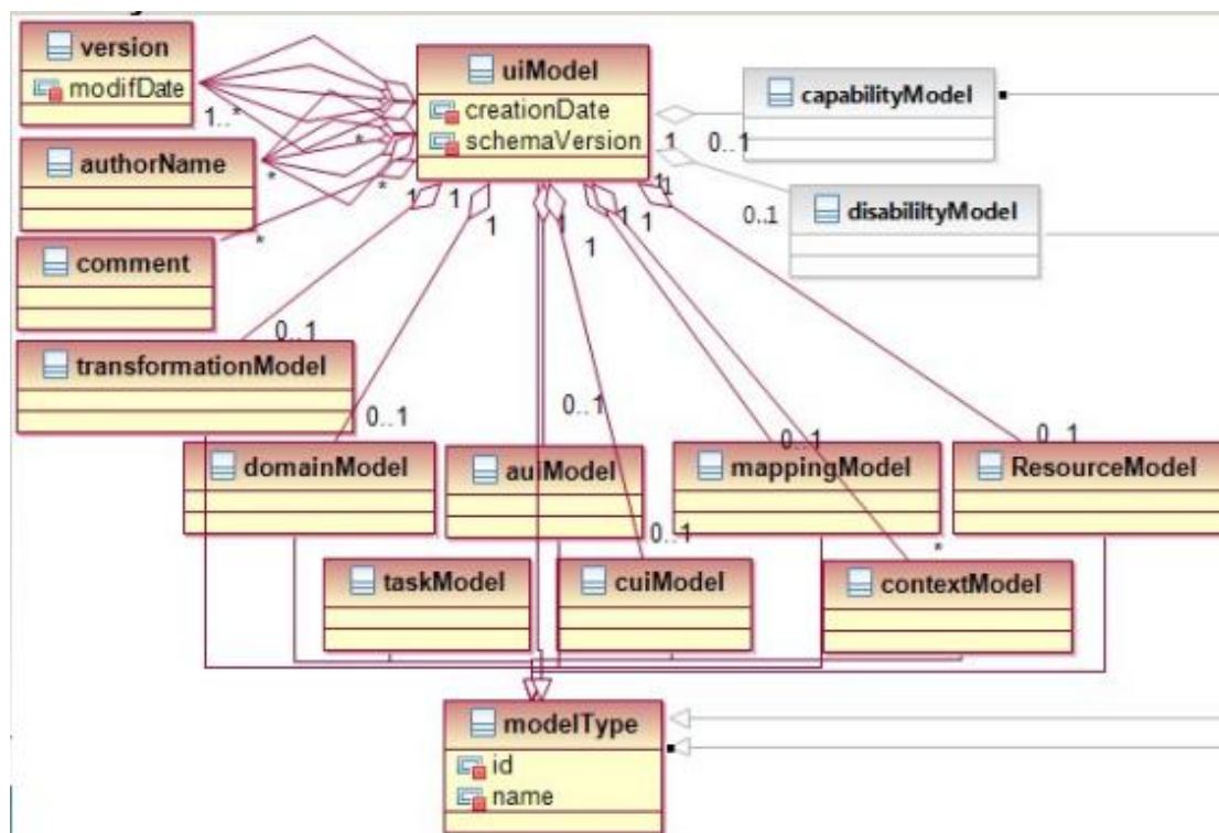
Figure 17. Constituent models in UsiXML.
