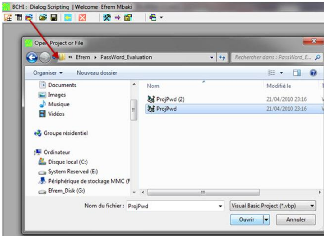
Figure 85. Opening Project.
