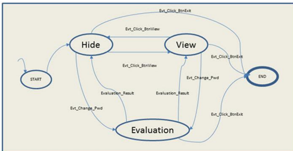
Figure 72. Dialogue Automata.
