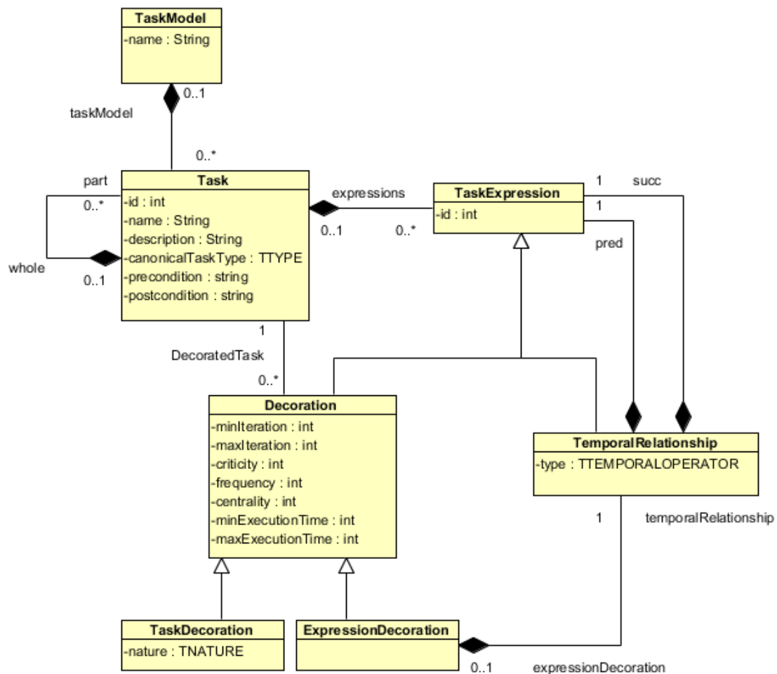
Figure 19. UsiXML Task Model.
