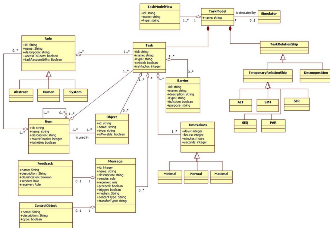
Figure 18. Meta-model of the UsiXML task model.
