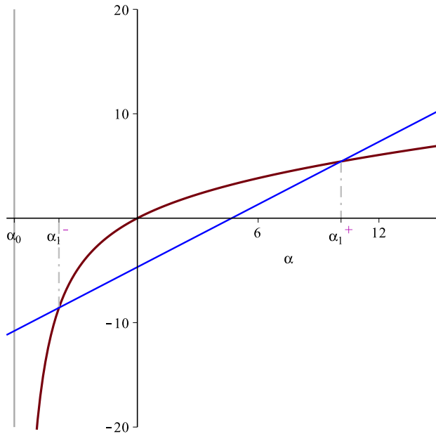
Fig. 5. The plot of \alpha \mapsto I(\alpha, \frac{\varepsilon+1}{\varepsilon-1}) (see Eq. (4.9)) and of the straight line \alpha \mapsto \alpha - (\frac{\varepsilon+1}{\varepsilon-1})^2 , intersecting the curve at \alpha_1^- and \alpha_1^+ .
