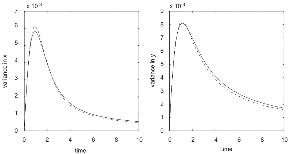
Fig. 14. Experiment 3. Variance in x , \sigma_{x,PDE}^2(t) for the PDE model and \sigma_{x,IBM}^2(t) for the IBM (left) and variance in y , \sigma_{y,PDE}^2(t) for the PDE and \sigma_{y,IBM}^2(t) for the IBM (right).
