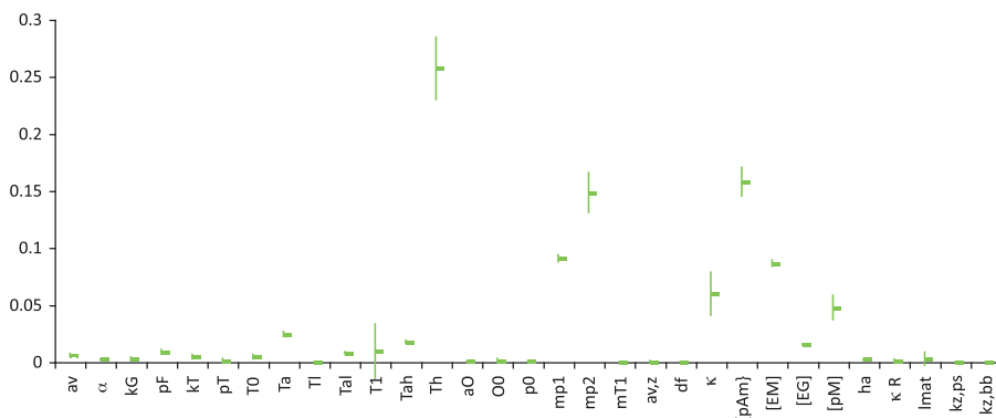
Fig. 3. Mean and standard deviation local sensitivity coefficients.
