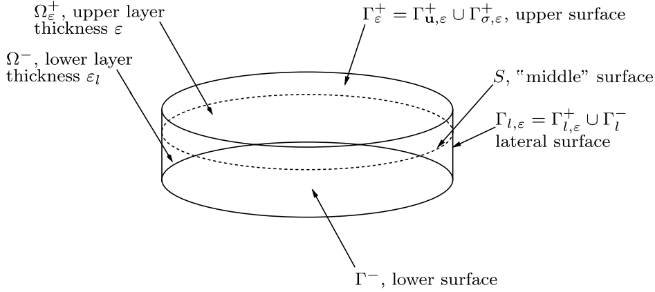
Fig. 3. The domain \Omega_\varepsilon = \Omega_\varepsilon^+ \cup \Omega^- .
