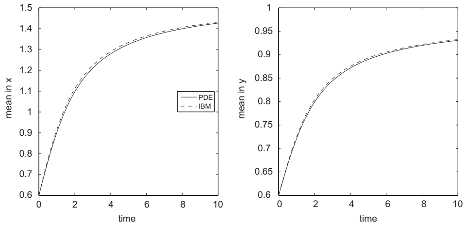
Fig. 13. Experiment 3. Mean position in x , m_{x,PDE}(t) for the PDE model and m_{x,IBM}(t) for the IBM (left) and mean position in y , m_{y,PDE}(t) for the PDE and m_{y,IBM}(t) for the IBM (right).
