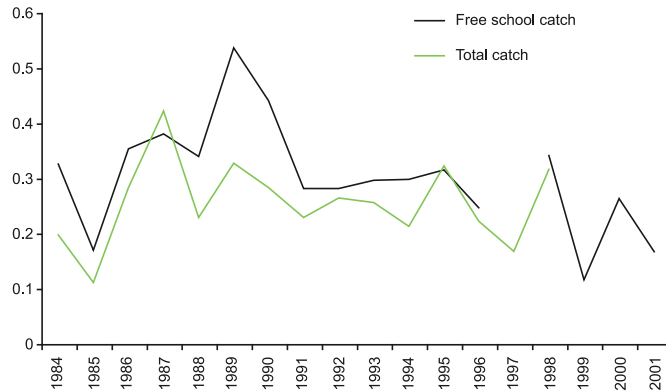
Fig. 5. Spearman's correlation coefficient for observed and computed catches (only years with significant correlations are represented).
