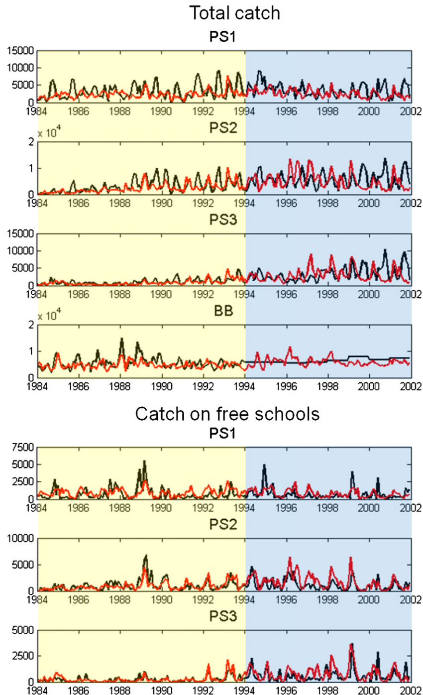
Fig. 4. Comparison between simulated (red) and observed (black) monthly aggregated catches of skipjack tuna for the different fleets: Results for total catches (top) and catches on free schools (bottom). Optimisation is performed on total catches from 1984 to 1993 and the model is running freely from 1994 to 2001. (For interpretation of the references to color in this figure legend, the reader is referred to the web version of the article.)
