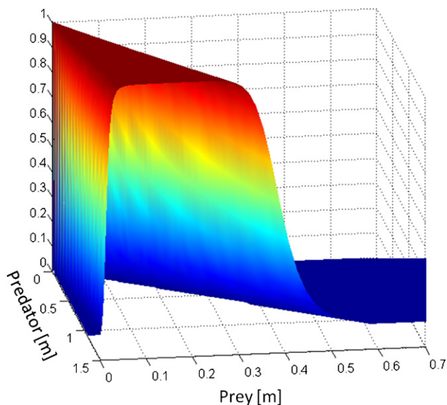
Fig. 2. Size selectivity function of predators on preys.
