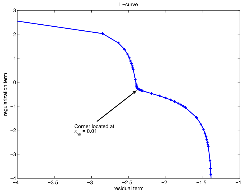
Fig. 10. Typical L-curve for the determination of \varepsilon_{ne} . It is a plot of the parametric curve x(\varepsilon_{ne}) = \log\left(\frac{1}{2}\|D^{1/2}(Bv^*(\varepsilon_{ne}) - \gamma)\|^2\right) , y(\varepsilon_{ne}) = \log\left(\frac{1}{2}(v^*(\varepsilon_{ne}))^T A v^*(\varepsilon_{ne})\right) where v^*(\varepsilon_{ne}) is the solution to Eq. (13). Hansen's algorithm [33] locates a corner at \varepsilon_{ne} = 0.01 .
