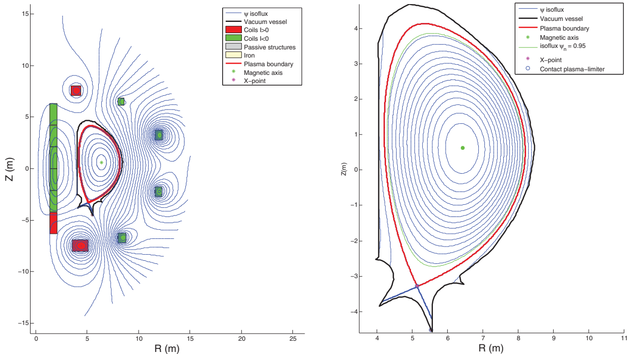
FIGURE 3. The reference solution for the ITER test problem.
