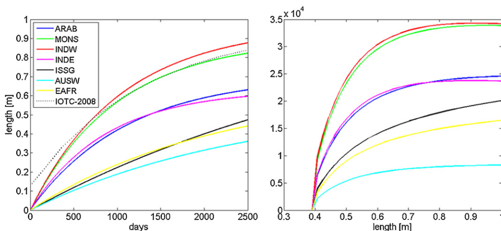
Fig. 6. Yearly average of Von Bertalanffy growth function (left) and daily fecundity [oocytes per kg biomass and day] (right) for the Longhurst provinces of the Indian Ocean.
