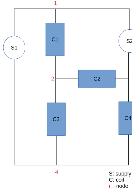
FIGURE A.1. Example of PF-circuit.
