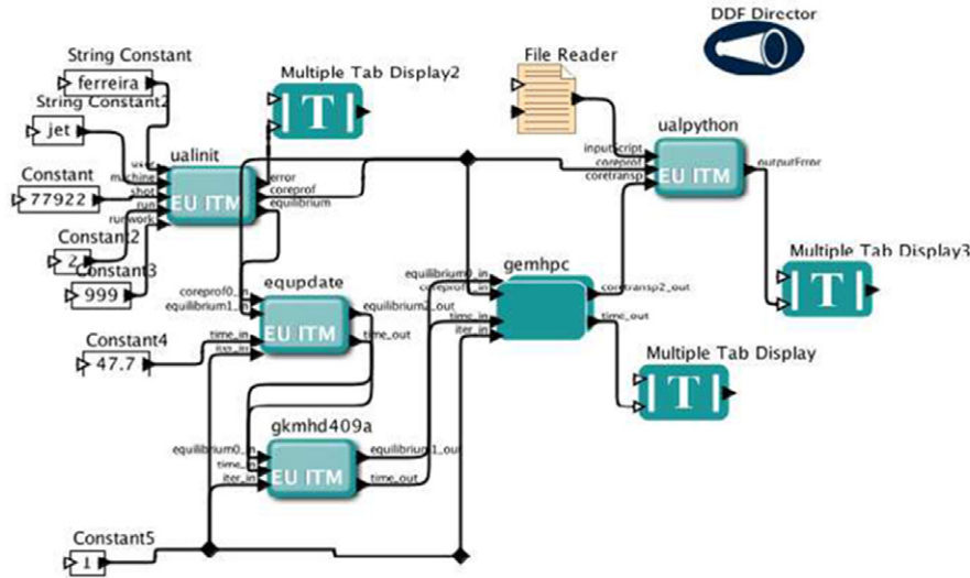
Figure 6. Turbulence workflow: JET shot data are read from the ITM database, the actor EQUPDATE provides equilibrium profile data and the equilibrium boundary, i.e. the separatrix, to actor GKMHD which adds the metrics information; both equilibrium_CPO and coreprof_CPO are input to the turbulence actor GEMHPC which runs in batch GEM gyrofluid flux-tube code in parallel on the HPC-FF.
