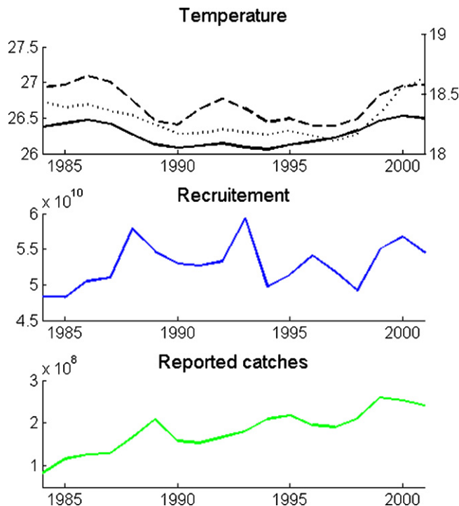
Fig. 8. Annual trends in mean temperature in the MONS (solid line), ARAB (dashed line) and INDW (dotted line) provinces (top); computed recruitment of skipjack in number of fishes reaching a size of 30 cm (center) and reported total catches (bottom).
