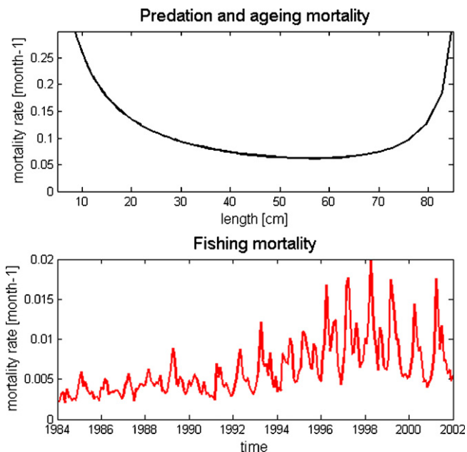
Fig. 7. Size dependent natural fish mortality (predation and ageing) compared to fishing mortality (simulated) as a function of time (1984–2001).
