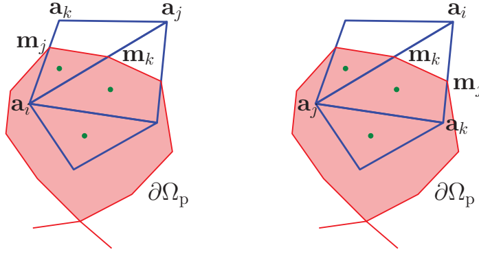
FIGURE 2. Integration over T \cap \Omega_p(\psi_h) . The green dots indicate the location of the quadrature point. The integration domain T \cap \Omega_p(\psi_h) is either (a) empty, (b) the whole element T , c) a triangular domain or quadrilateral domain.
