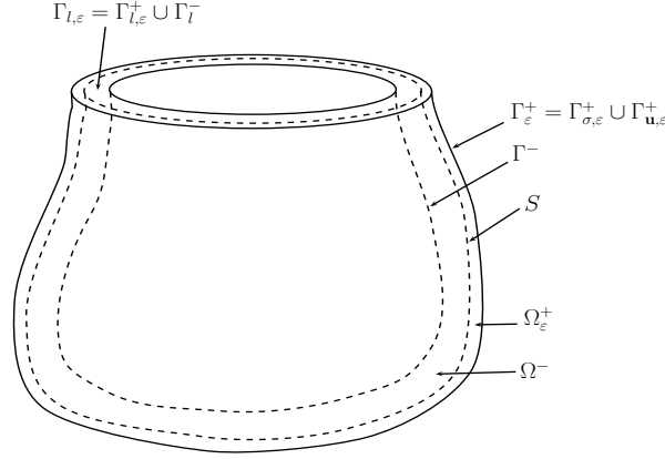
FIGURE 2.8 – Le domaine \Omega_\varepsilon = \Omega^- \cup \Omega_\varepsilon^+ .
