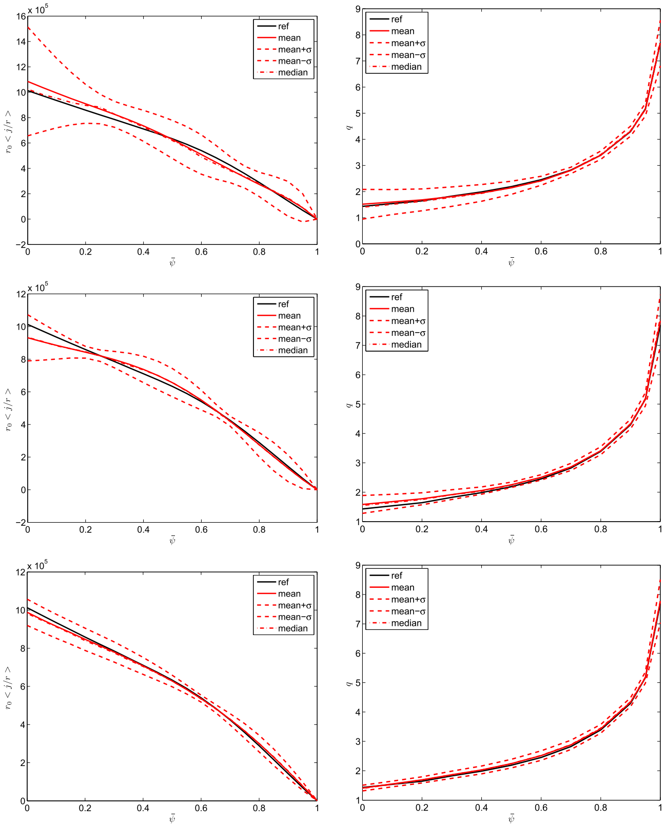
Fig. 6. Statistical results of the identification experiments with noisy magnetic measurements. Row 1: \epsilon = 10^{-2} , row 2: \epsilon = 10^{-1} , row 3: \epsilon = 1 . Column 1: R_0 \langle \frac{j(r, \bar{\psi})}{r} \rangle , and column 2: safety factor q . For each function the reference value is given in black and the mean identified function in red. The mean \pm standard deviation functions are shown in dashed red. (For interpretation of the references in colour in this figure legend, the reader is referred to the web version of this article.)
