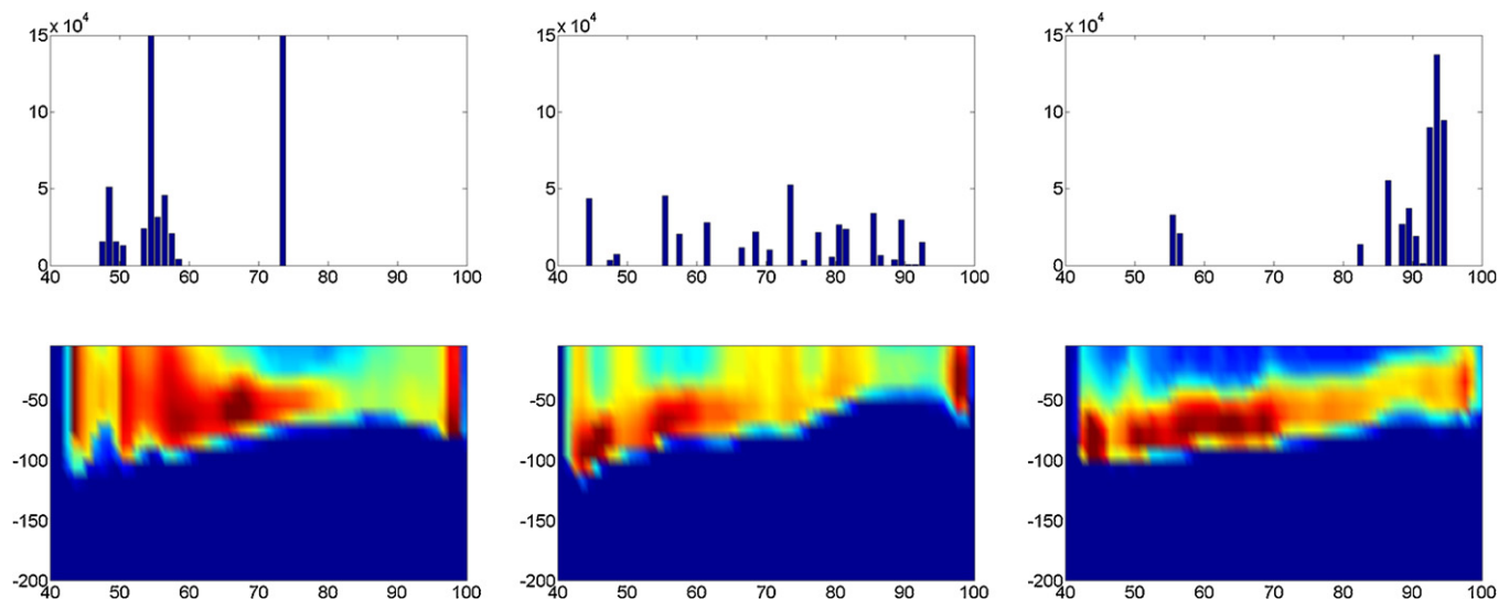
Fig. 11. Observed catches in the West-East transect on the Equator in April 1993 (top left), February 1998 (top center), April 1998 (top right) and corresponding computed vertical distribution of skipjack biomass on the same transect in April 1993 (bottom left), February 1998 (bottom center), April 1998 (bottom right).
