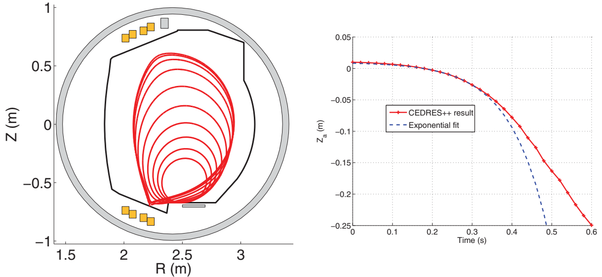
FIGURE 7. Left: plasma boundary at intervals of 100 ms in a vertical instability simulation for WEST. Right: time evolution of the vertical position of the magnetic axis z_{ax} in a vertical instability simulation for WEST.
