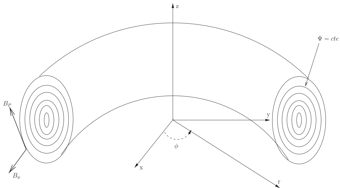
Fig. 1. Toroidal geometry.
