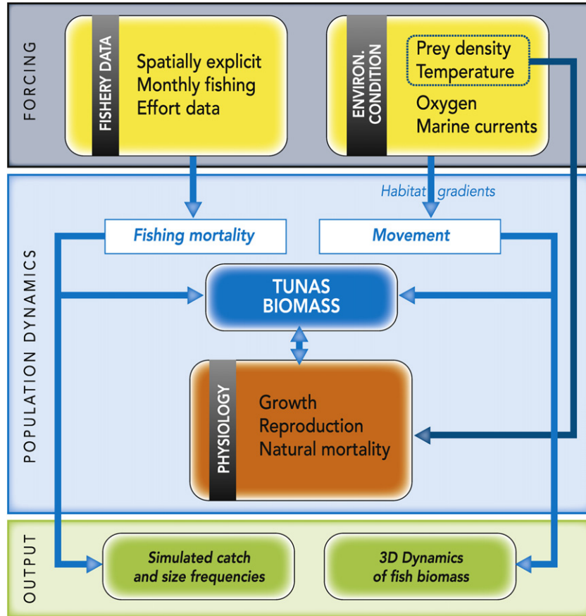
Fig. 1. Diagram showing the forcing, the processes affecting the population dynamics and the outputs of the APECOSM-E model.
