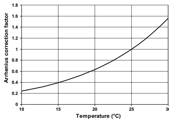
Fig. 5. Arrhenius correction factor for temperatures ranging from 10 °C to 30 °C ( T_A = 8000 and T_{ref} = 298.15K = 25\text{ °C} ). Each biological rate in the model is multiplied by the Arrhenius correction factor.
