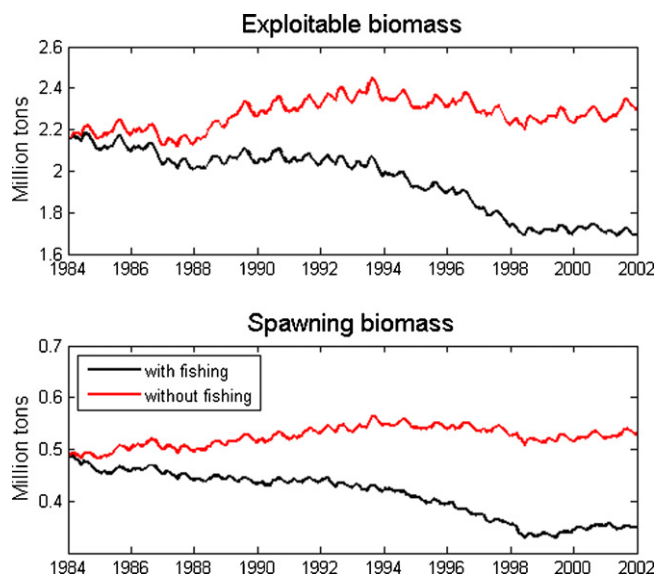
Fig. 9. Simulated exploitable and spawning skipjack biomass, with and without the effect of fishing mortality.
