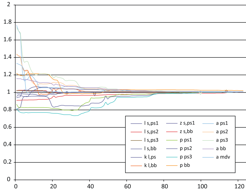
Fig. 2. Variation of the parameters as a function of the iteration number during the minimization process. Values are normalized relatively to the optimized values.
