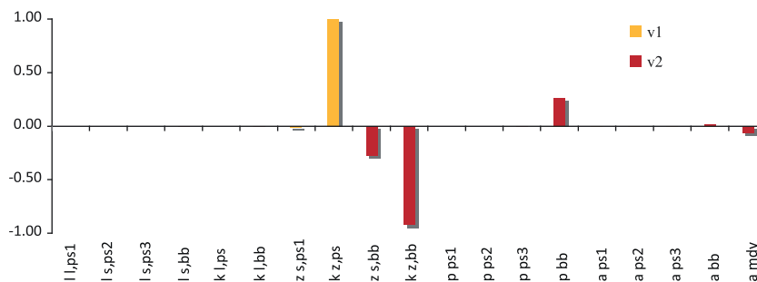
Fig. 1. Values of the elements that compose eigenvectors v_1 and v_2 , corresponding to the two smallest eigenvalues of the Hessian.
