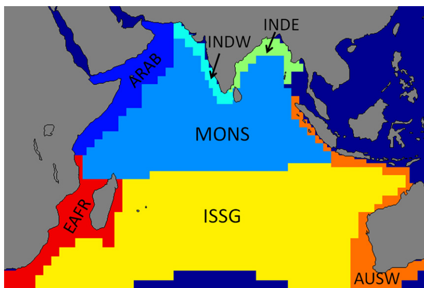
Fig. 5. Longhurst provinces in the Indian Ocean.
