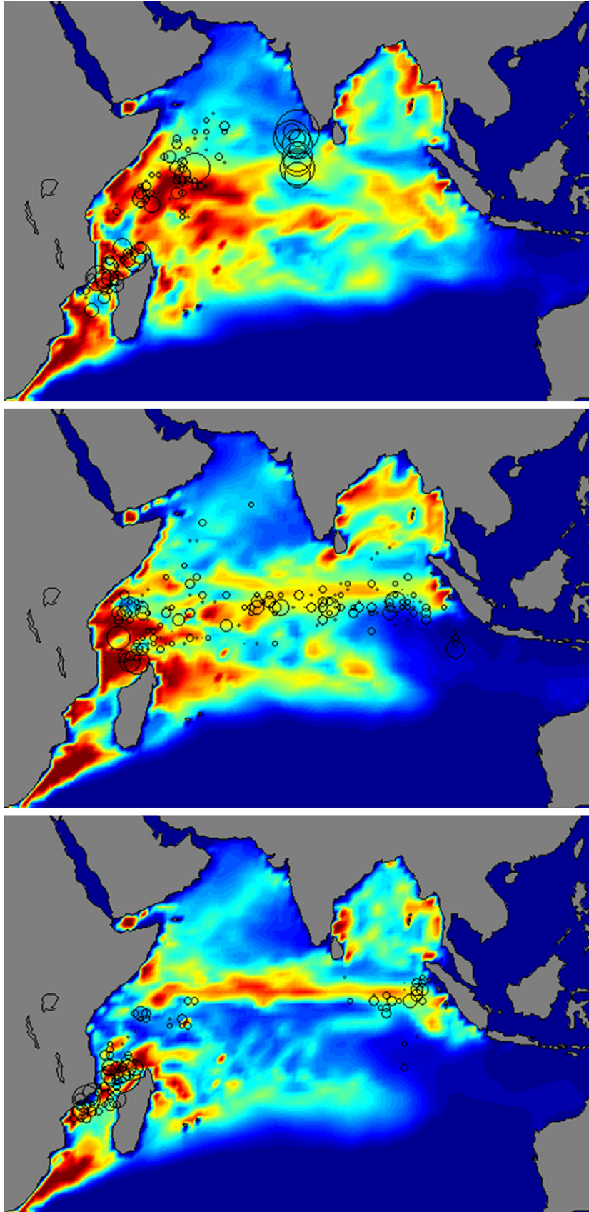
Fig. 10. Computed vertically integrated exploitable skipjack population vs observed catches (circles) in the Indian Ocean: April 1993 (top), February 1998 (center), April 1998 (bottom).
