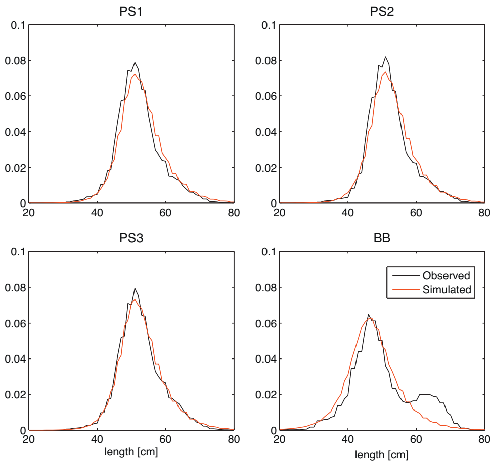
Fig. 6. Comparison between observed and simulated length frequency for the four different fleets (1984–1993).
