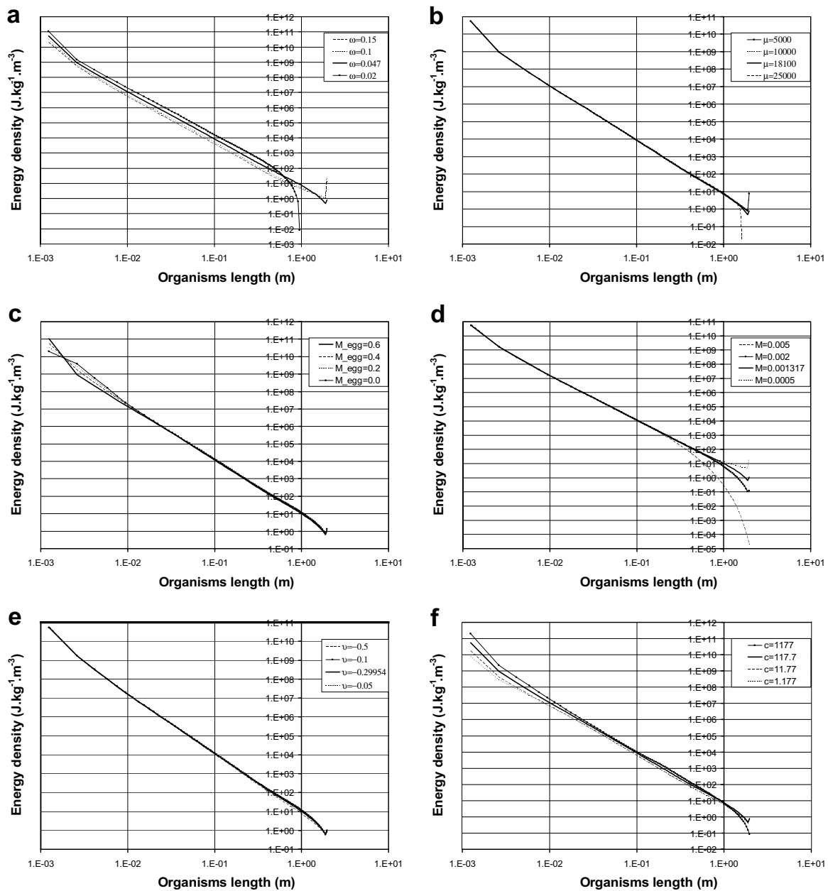
Fig. 9. Systematic sensitivity analysis of the steady state to the parameters. Different values of \omega , \mu , M_{\text{egg}} , M , v , c , \kappa , \rho_2 , \rho_1 , e_A and E_g varying in a large range around their reference values are considered respectively in (a)–(l). The sensitivity of the steady state to the parameter \kappa is considered in the case where M_{\text{egg}} = 0.4 (g) and M_{\text{egg}} = 0 (h).
