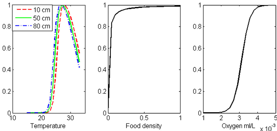
Fig. 4. Functional responses for temperature, food density and oxygen conditions.
