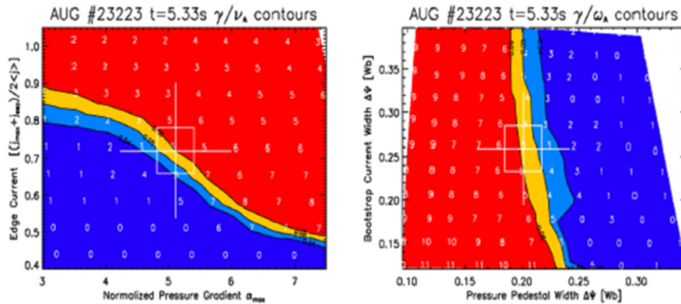
Figure 2. Pedestal height (left) and width (right) study for ASDEX Upgrade obtained with the J-alpha stability workflow [8] with kind permission of the European Physical Journal (EPJ). The plot shows the contours of the linear ideal MHD growth rates \gamma (normalized to the Alfvén frequency v_A ) of the fastest growing edge modes (toroidal mode numbers are indicated by the white integers) in the plane defined by the maximum normalized edge pressure gradient \alpha_{\max} and the normalized edge current density. Contours indicate the level of the diamagnetic drift frequency separating the stable (blue) from the unstable (red) region. The crosshair indicates the experimental equilibrium including error bars.
