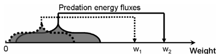
Fig. 2. Schematic representation of weight (size) structured energy flow through the ecosystem.
