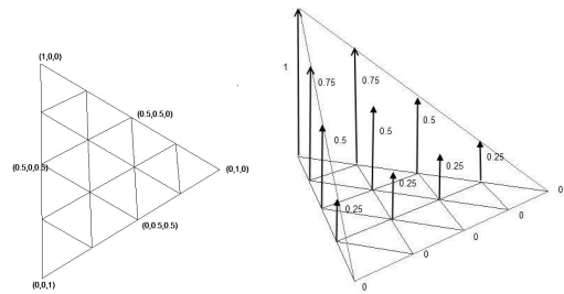
Fig. 2. The shape functions. The shape function of a point inside of a face is determined from barycentric coordinates of the respective point.
