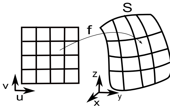
Figure 2.4: Example of mapping from \mathbb{R}^2 to \mathbb{R}^3 .
