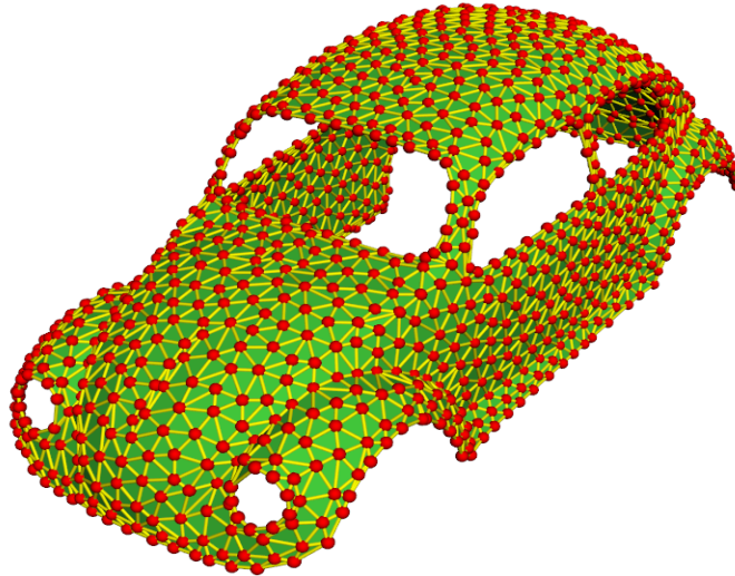
Figure 2.6: The structure of a mesh representing a car body. The red points are the vertices, the yellow lines are the edges and green represents the faces (triangles in this example). The Beetle model is provided courtesy of L. Kobbelt.
