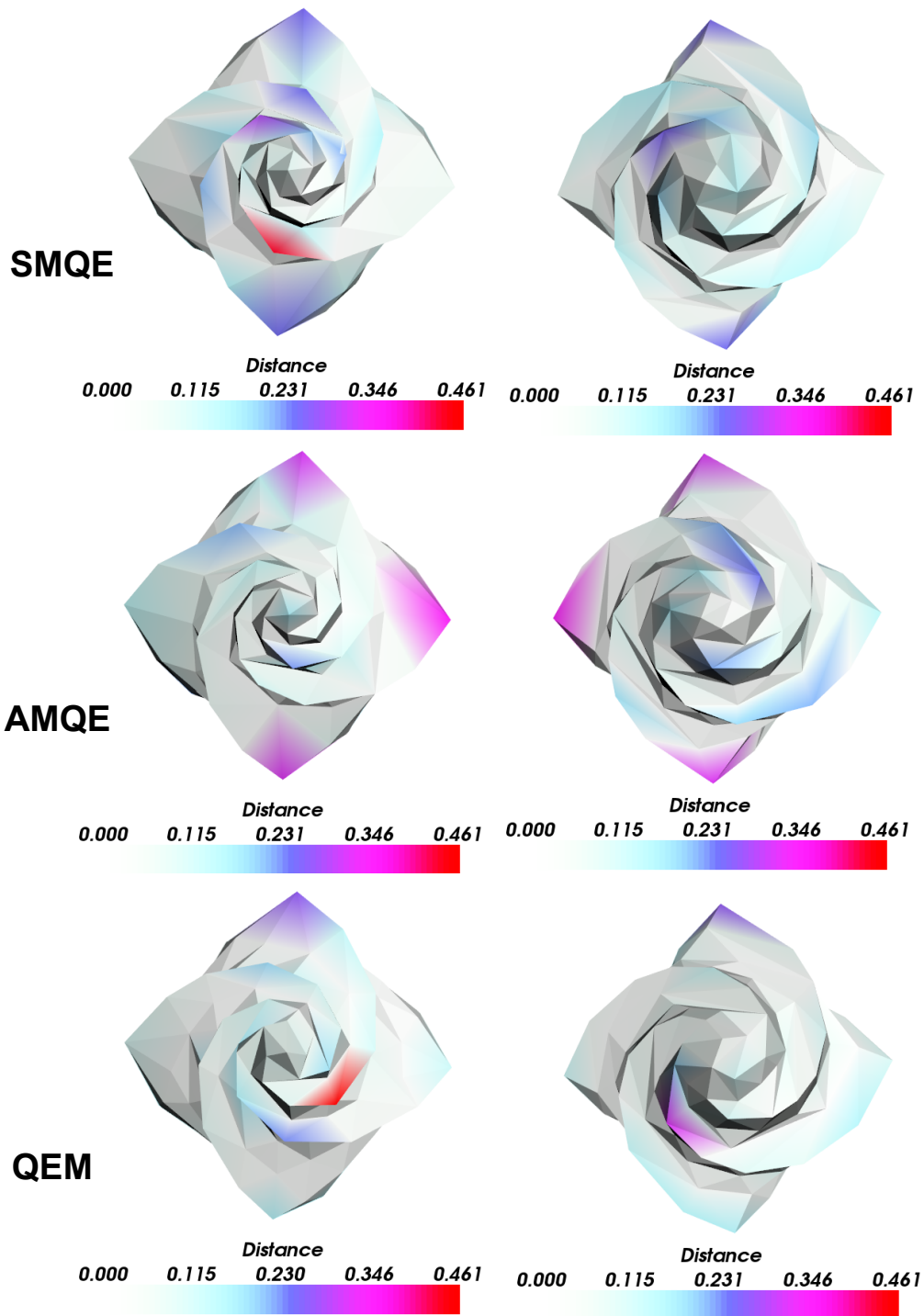
octa-flower 169 vertices
