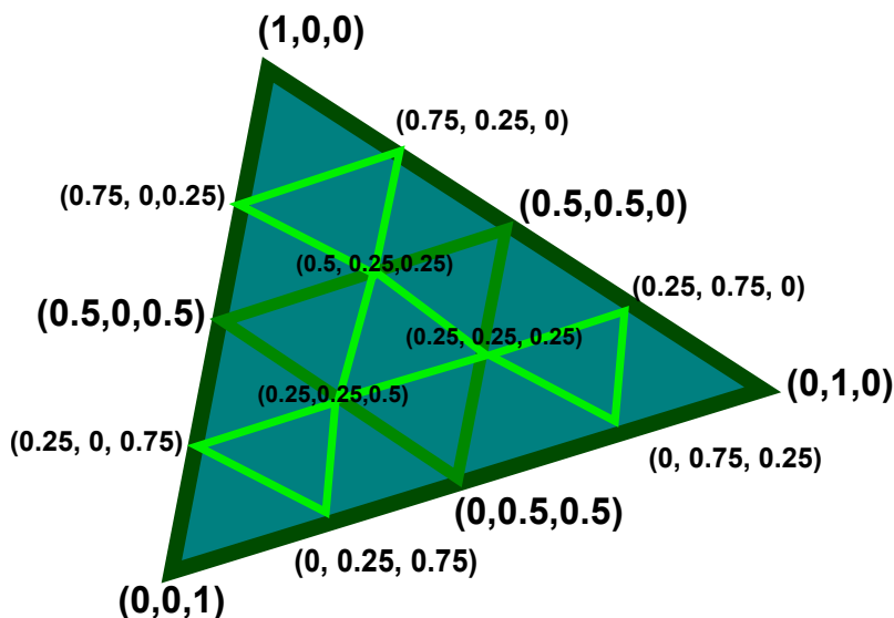
Figure 4.9: Two 1:4 subdivisions of a triangle and its barycentric coordinates.
