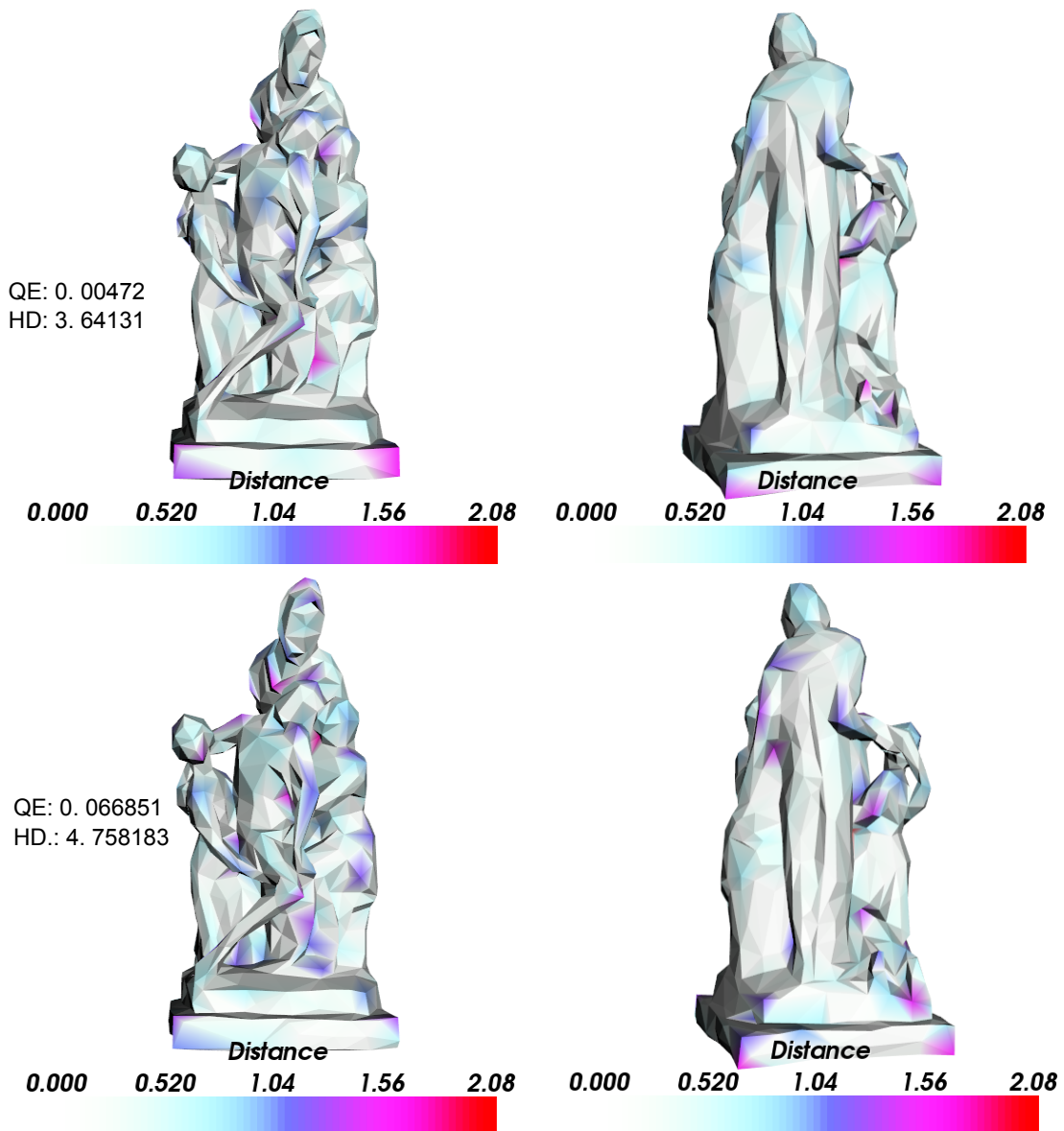
Figure 5.6: The distance between the Pieta model with 13 940 vertices and its simplified version with 900 vertices. The distance is computed between each vertex of the original model to the simplified model by using the PQP library.
