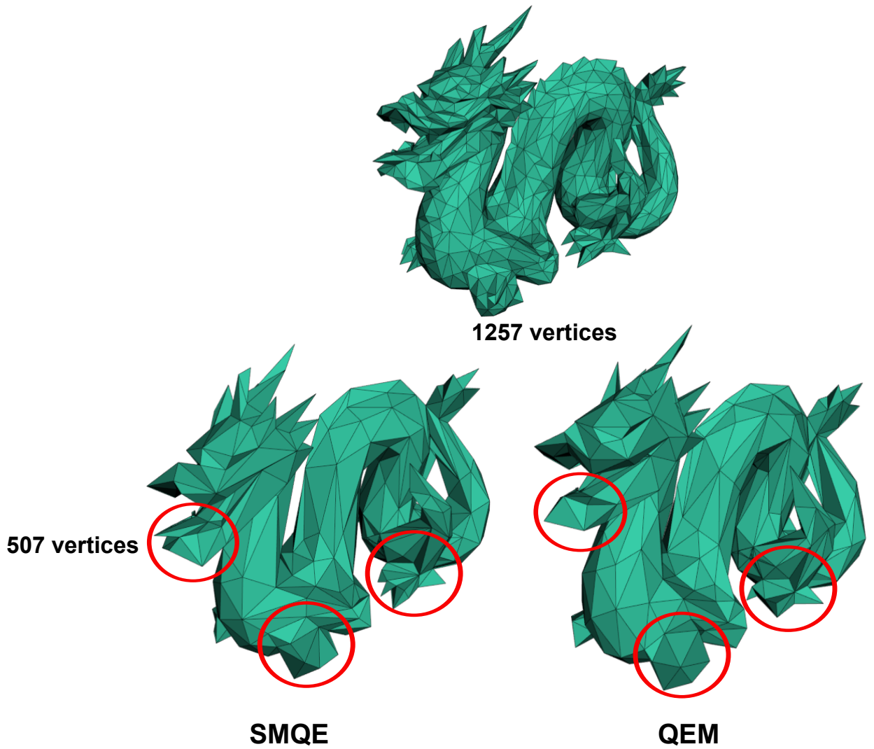
Figure 5.16: The simplified versions of the Dragon (1257 vertices) with 507 vertices using the SMQE and QEM methods.
