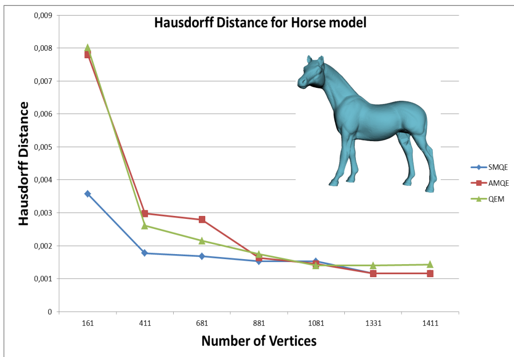
Figure 5.14: The Hausdorff distances introduced in the simplification of Horse. The Hausdorff distances are measured using the Metrol tool.
