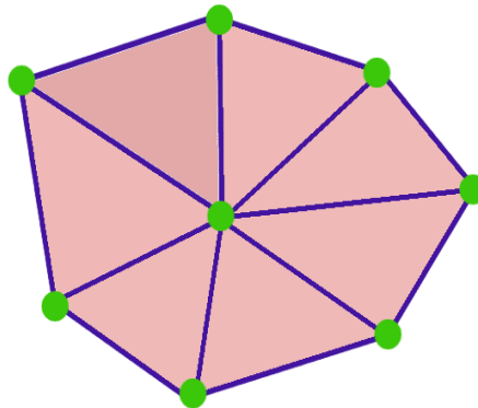
Figure 2.7: The geometry of a mesh.
