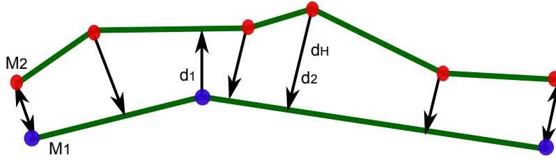
Figure 3.1: Surface to Surface Distance
