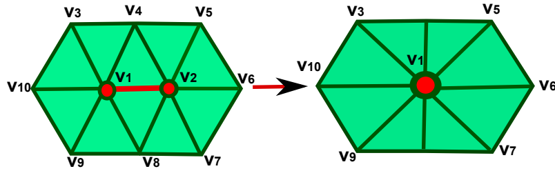
Figure 4.4: Interior Edge Collapse. One edge is collapse to a single vertex. Triangles which share the deleted edge are deleted. The number of vertices is reduced by one, the number of faces by two and the number of edges by three.
