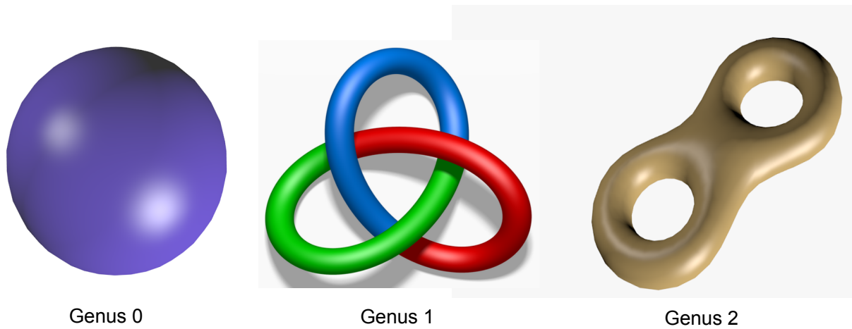
Figure 2.11: Objects of different genus. From left to right: a sphere of genus 0, a torus of genus 1 and a double torus of genus 2.
