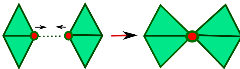
Figure 3.10: Vertex Pair Contraction . A pair of unconnected vertices are collapsed. The number of vertices is reduced by one, the number of edges and faces remaining constant.
