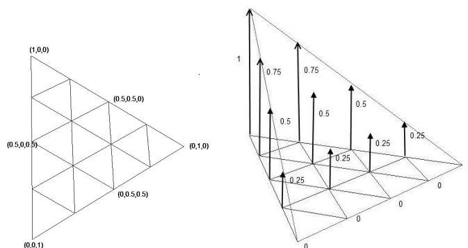
Figure 4.22: The shape functions. The shape function of a point inside a face is determined from the barycentric coordinates of the respective point.
