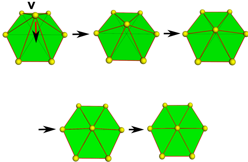
Figure 4.23: Volume minimization between two meshes.
