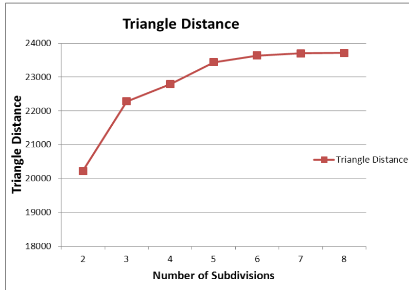
Figure 4.12: The distance for one triangle accordingly to the number of subdivisions of the triangle.
