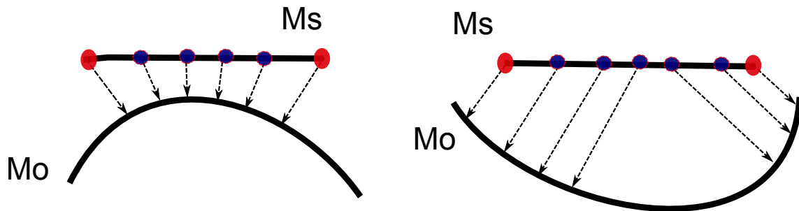
Figure 4.7: Improvement of the approximated distance between two curves by adding sample points.
