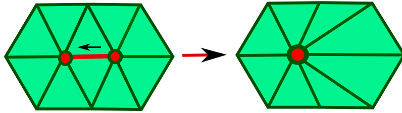
Figure 3.9: Half-Edge Collapse . The edge is collapsed to one of its endpoints. The number of vertices is reduced by one, the number of faces is reduced by two and the number of edges is reduced by three.
