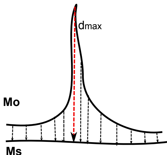
Figure 4.1: The representation of the maximum distance between two surfaces.
