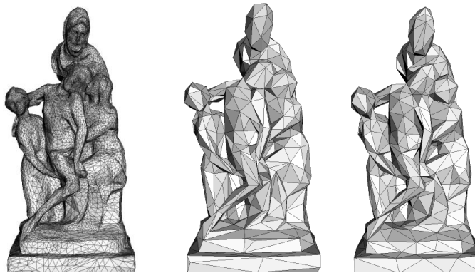
Fig. 1: Approximations of Pieta. From left to right: Original model with 13940 vertices (27904 triangles), simplified models with 450 vertices using our simplification algorithm and QEM.
