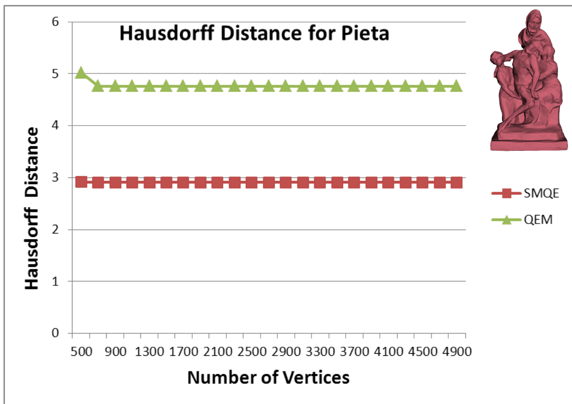
Figure 5.5: The Hausdorff distance introduced in simplification of Pieta model.
