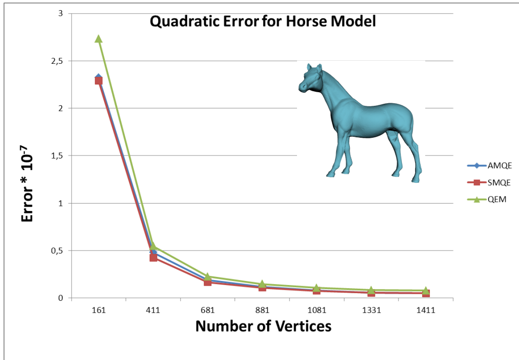
Figure 5.13: The quadratic error introduced in the simplification of Horse.
