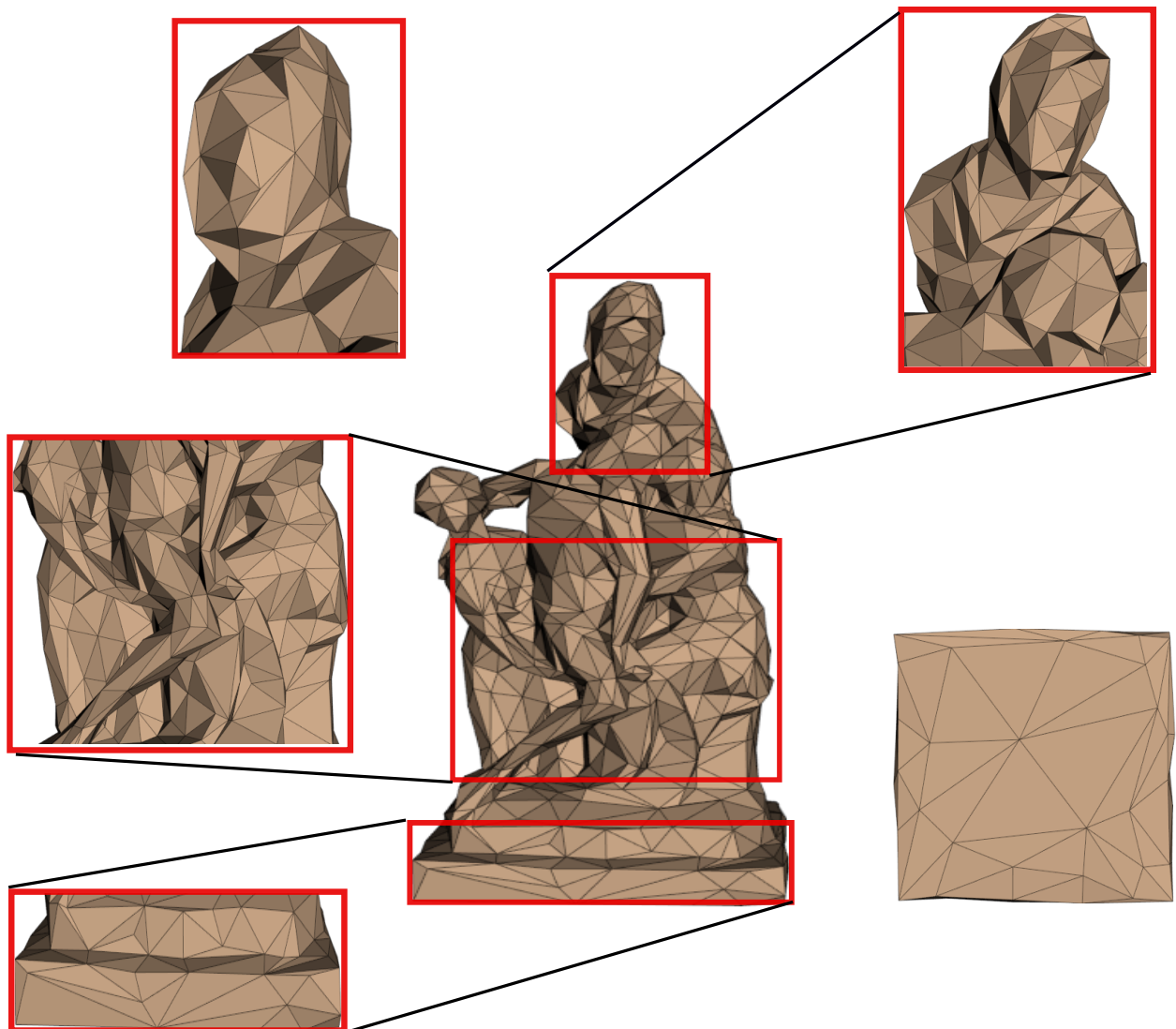
Figure 5.1: The simplified Pieta model with 900 vertices using SMQE.
