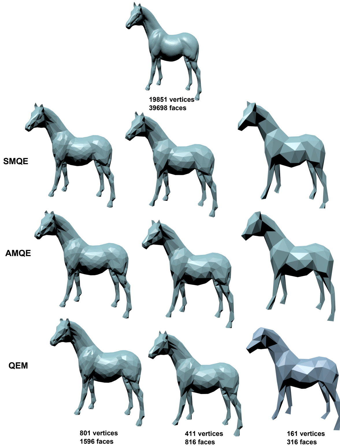
Figure 5.11: Sequence of simplifications for the Horse model (19 851 vertices) with 801, 411 and 161 vertices, respectively. The simplifications are realized using the SMEQ, AMQE and QEM methods.
