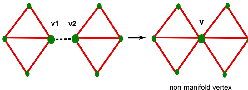
Figure 3.11: Vertex Pair Contraction . If two vertices such as v_1 and v_2 are collapsed, their collapsed can generate non-manifold vertices, such as vertex v .
