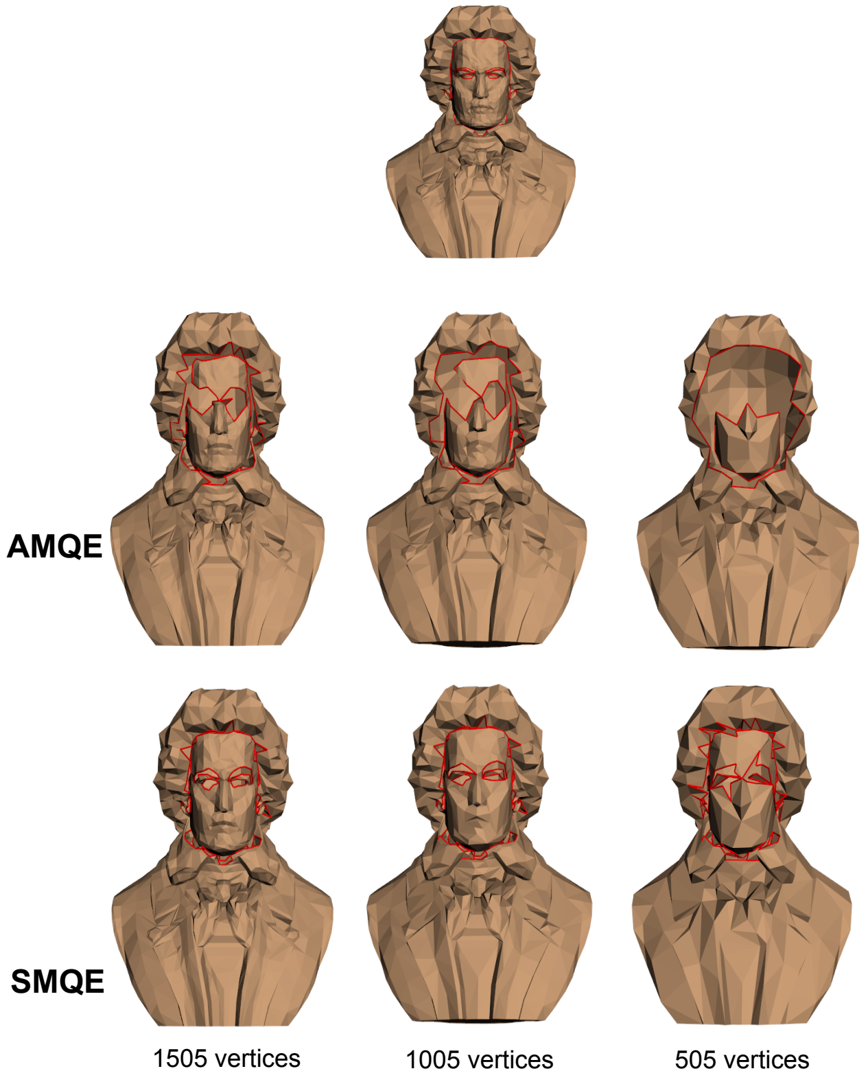
Figure 5.23: A sequence of simplifications for the Beethoven (2655 vertices) model with 1505, 1005 and 505 vertices. The boundaries (red lines) are better preserved for the simplifications realized with the SMQE method than with AMQE.
