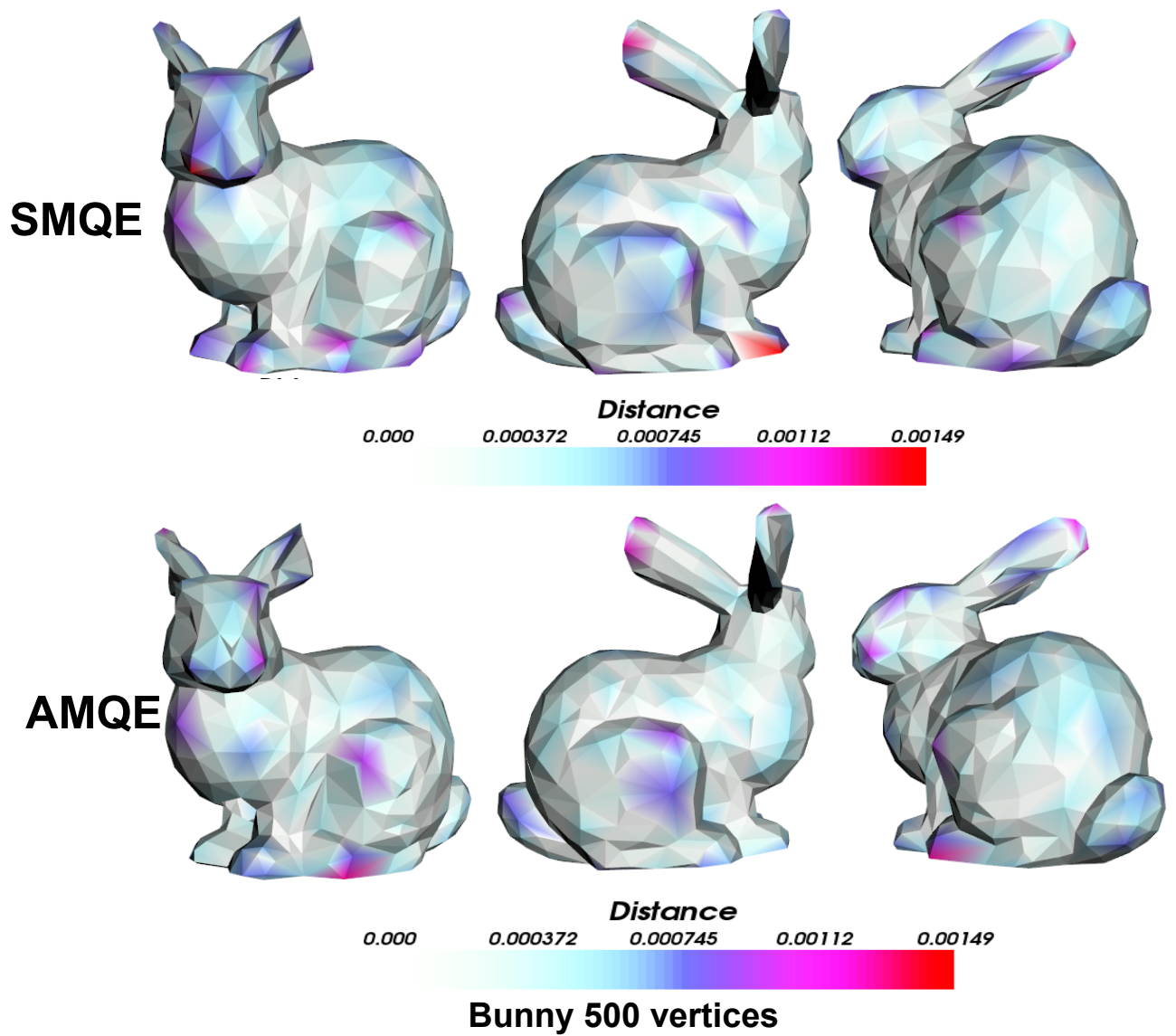
Figure 5.22: The distances between the original Bunny (35 947 vertices) and its simplified version with 500 vertices. The distances are computed between each vertex of the original model to the simplified model by using the PQP library.
