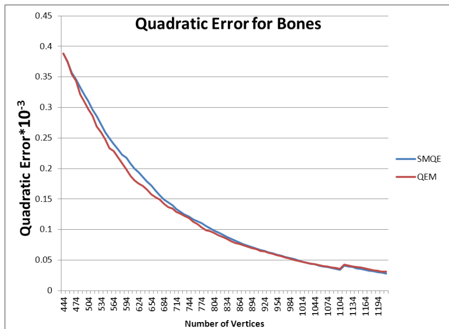
Figure 5.33: Quadratic Error for the Bones model vs. Number of Vertices
