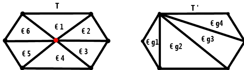
Figure 3.5: Representation of a triangulation and its corresponding simplified version.
