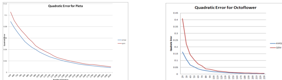
Fig 3: Geometric error vs. number of vertices for Pietà and Octoflower. The quadratic error is computed between approximated mesh and original one for each step of simplification. Simplifications are made using OEM (red line) and our algorithm (blue line).
