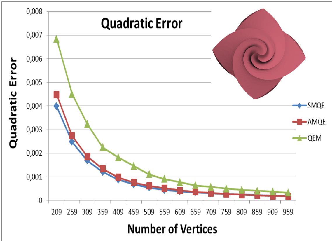
Figure 5.8: The quadratic error introduced in the simplification of the Octa-flower.
