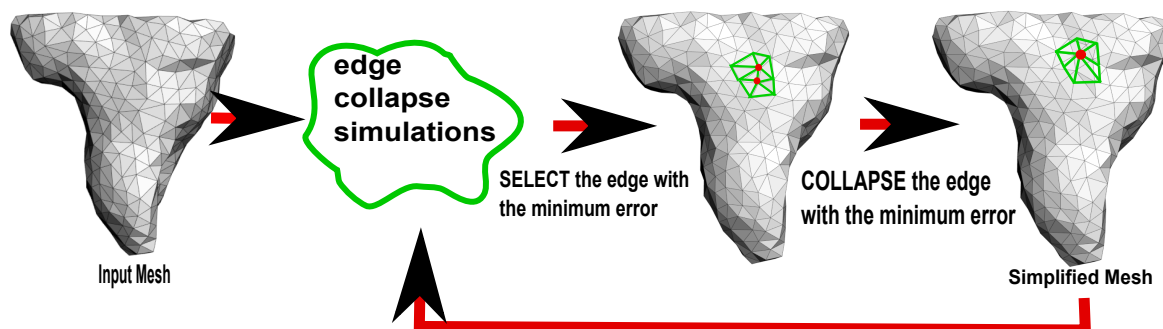
Figure 4.3: Overview of the simplification algorithm.
