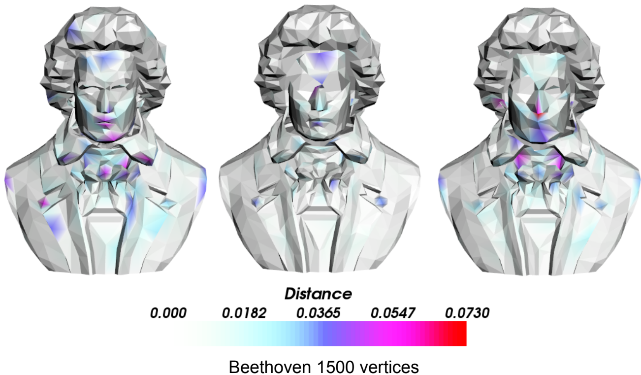
Figure 5.26: The distances between the original Beethoven (2655 vertices) and its simplified version with 1500 vertices. The distances are computed between each vertex of the original model to the simplified model by using the PQP library.
