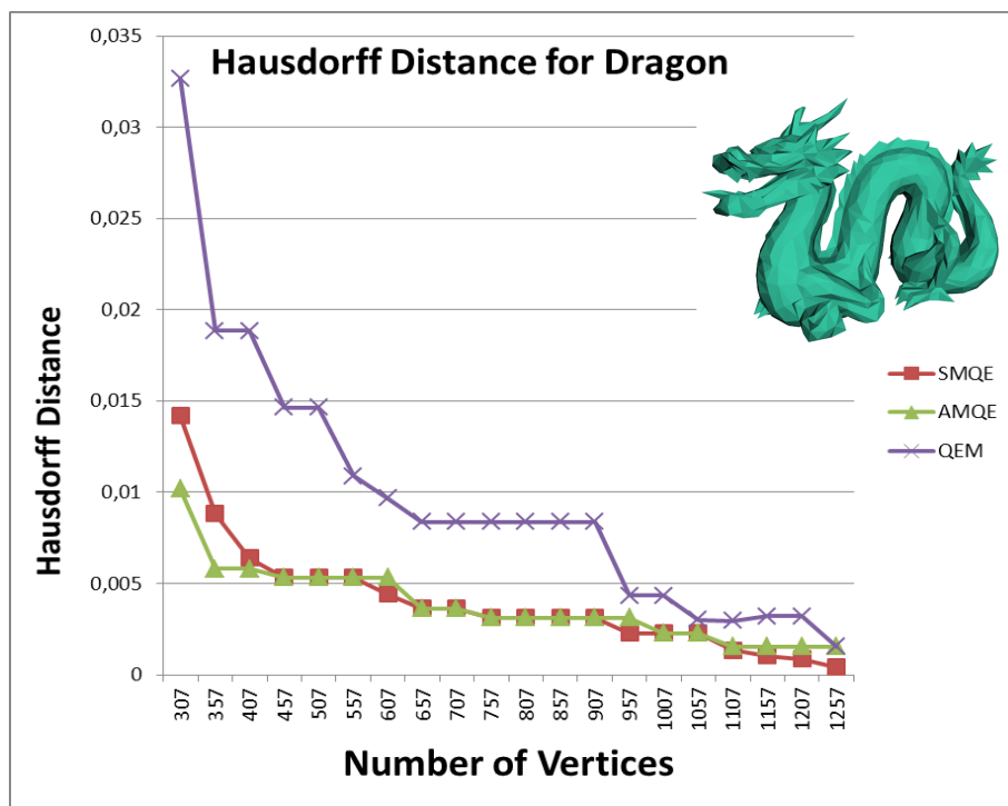
Figure 5.18: The Hausdorff errors introduced in the simplification of the Dragon.
