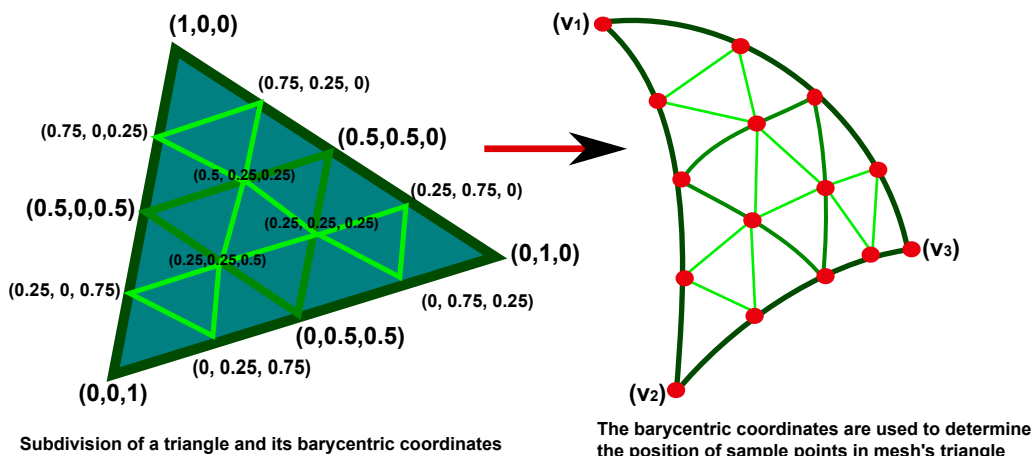
Figure 4.10: Two 1:4 subdivisions of a triangle and its barycentric coordinates.
