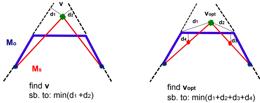
Figure 4.21: The 2D representation of the vertex placement. In the left image, the new vertex is placed to minimize the sum of quadratic errors to the planes. In the right image, the vertex minimizes the sum of squared distances to its adjacent faces.
