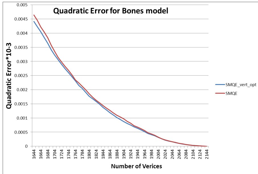
Figure 5.35: Quadratic Error for Bones model vs. Number of Vertices. SMQE_{vert-opt} represents the error for the model simplified with SMQE and using Volume-based vertex optimization to locate the resulting vertex.
