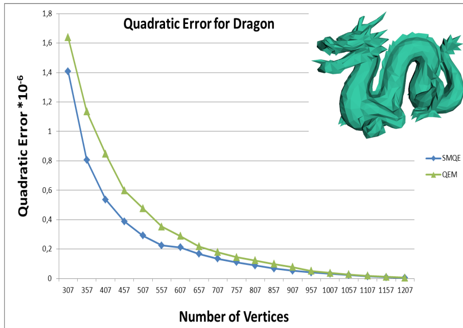
Figure 5.17: The quadratic errors introduced in the simplification of the Dragon.
