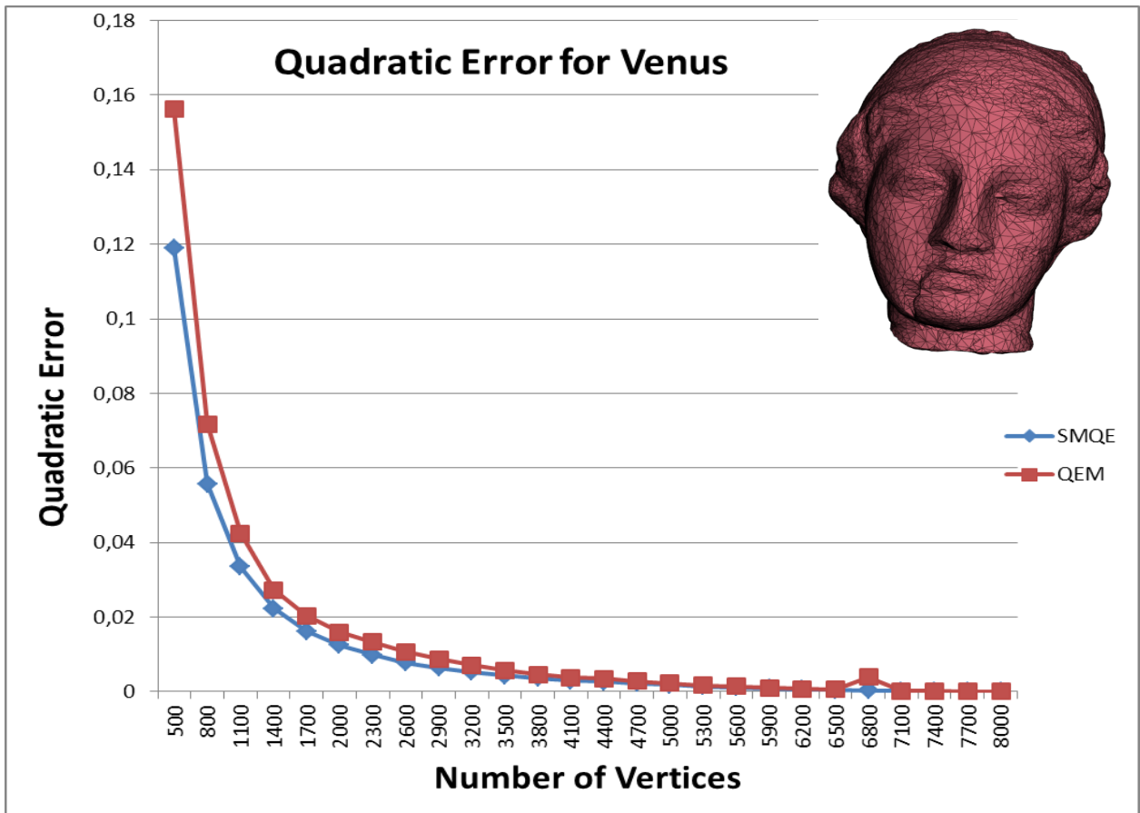
Figure 5.29: The quadratic errors introduced in the simplification of the Venus model.
