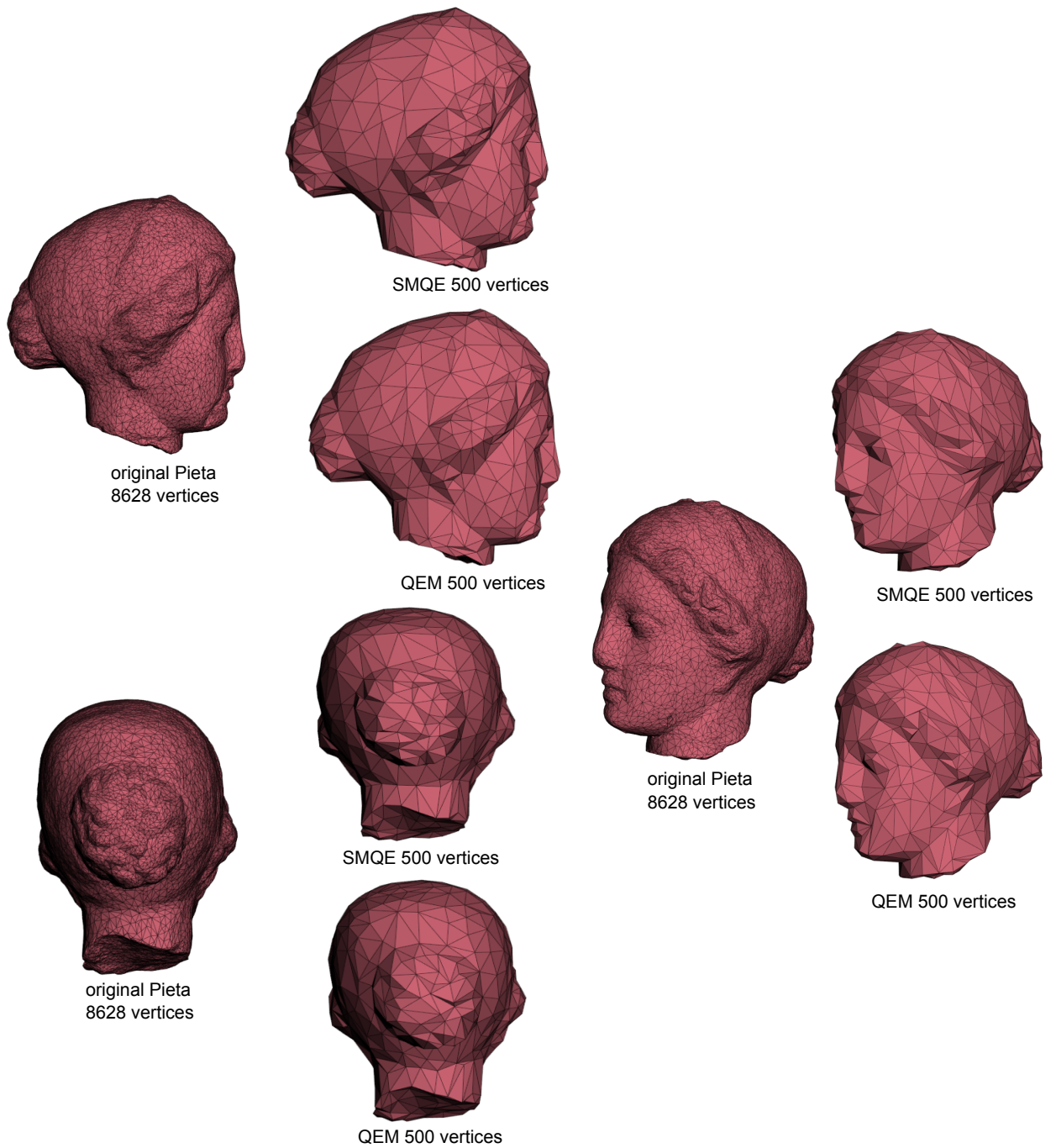
Figure 5.28: Simplified versions for the Venus model; multiple viewpoints.
