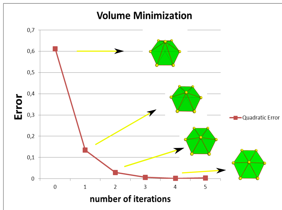
Figure 4.24: The variation of the volume embedded between two meshes with the number of iterations.
