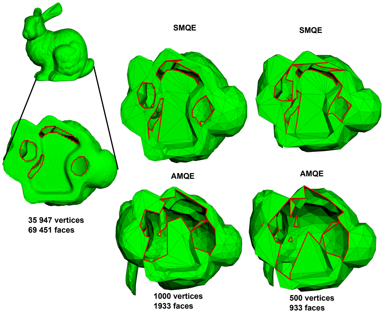
Figure 5.21: The base for the Bunny model (first column) and its simplified versions with 1000 vertices, respectively 500 vertices. The boundaries (red) are better preserved for the model simplified with SMQE (top) than for the model simplified with AMQE (bottom).
