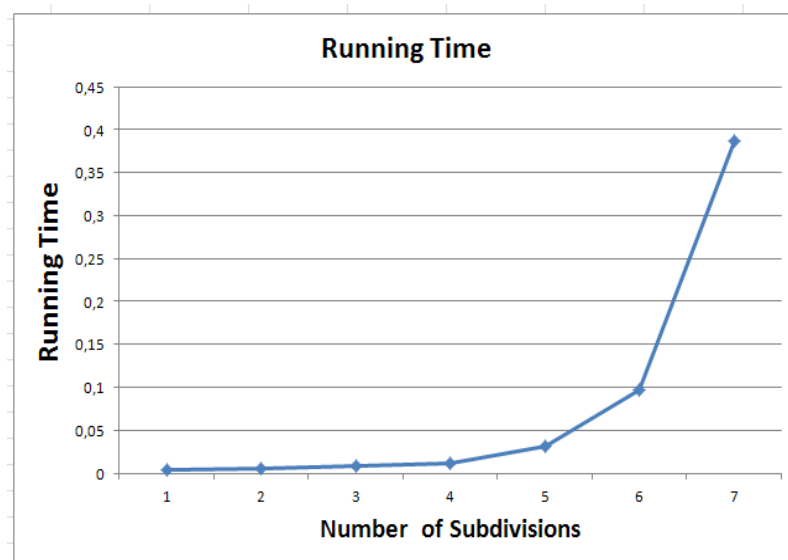
Figure 4.13: The running time to compute the distance for one triangle accordingly to the number of subdivisions of the triangle.
