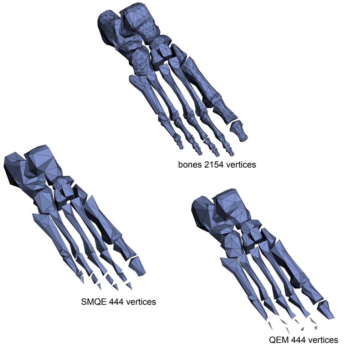
Figure 5.32: Simplifications for the Bones model.
