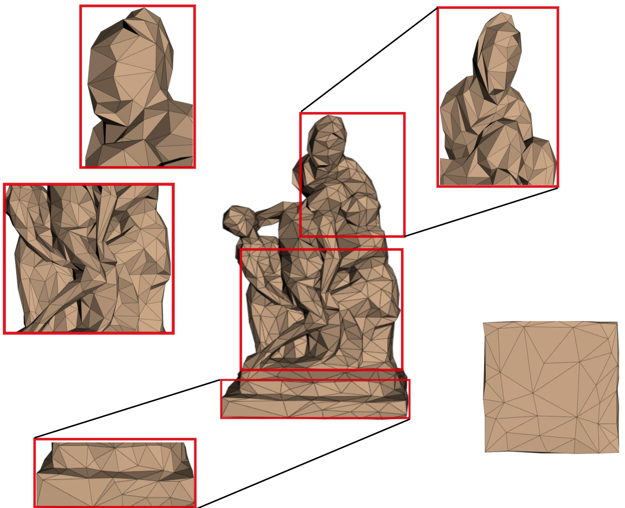
Figure 5.2: The simplified Pietà model with 900 vertices using QEM.
