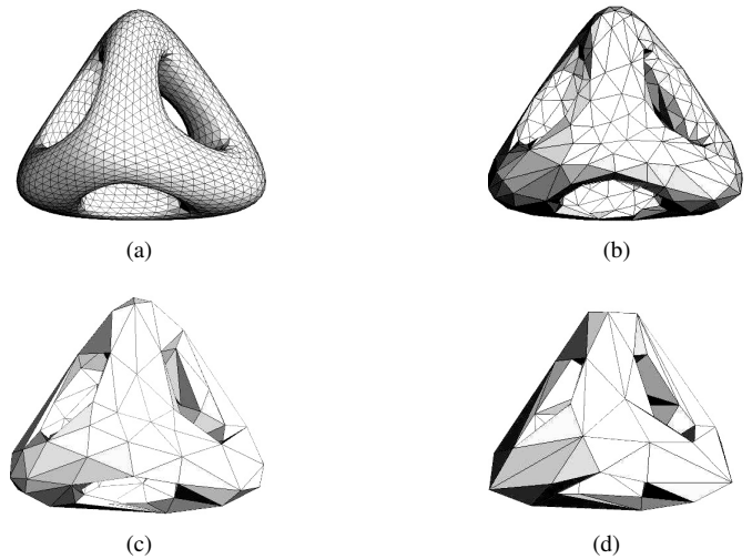
Fig. 7. Approximations of a genus 3. Original model with 2000 vertices. Approximation models using 500, 100 and 50 vertices.
