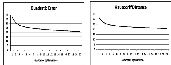
Fig. 3. Quadratic Error and Hausdorff distance vs. number of optimizations. The Heart model is approximated with 30 vertices. The position of each vertex in the approximation is optimized using 20 optimization steps
