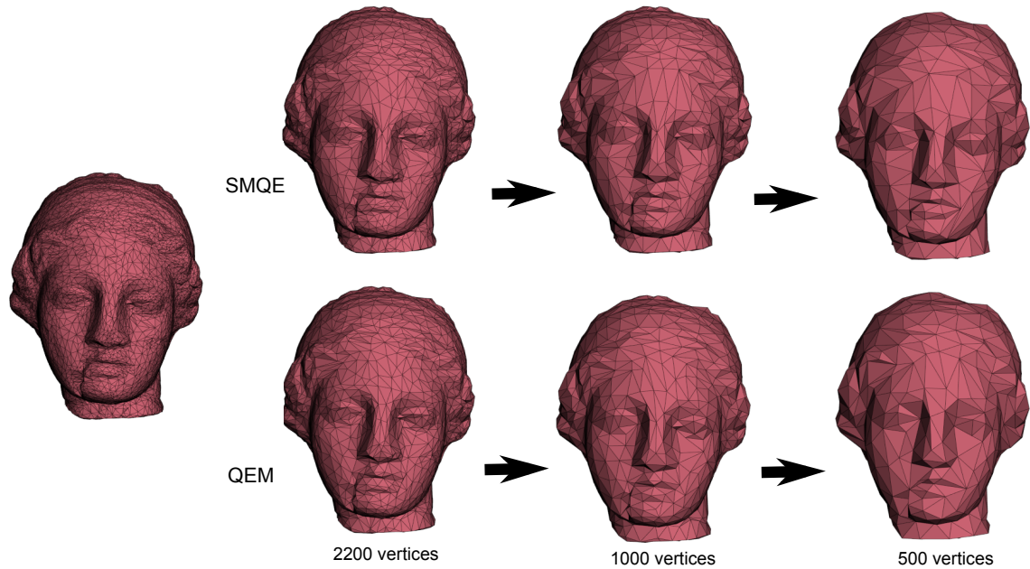
Figure 5.27: The sequence of the simplifications for the Venus model (8268) with 2200, 1000 and 500 vertices using the SMQE and QEM methods.
