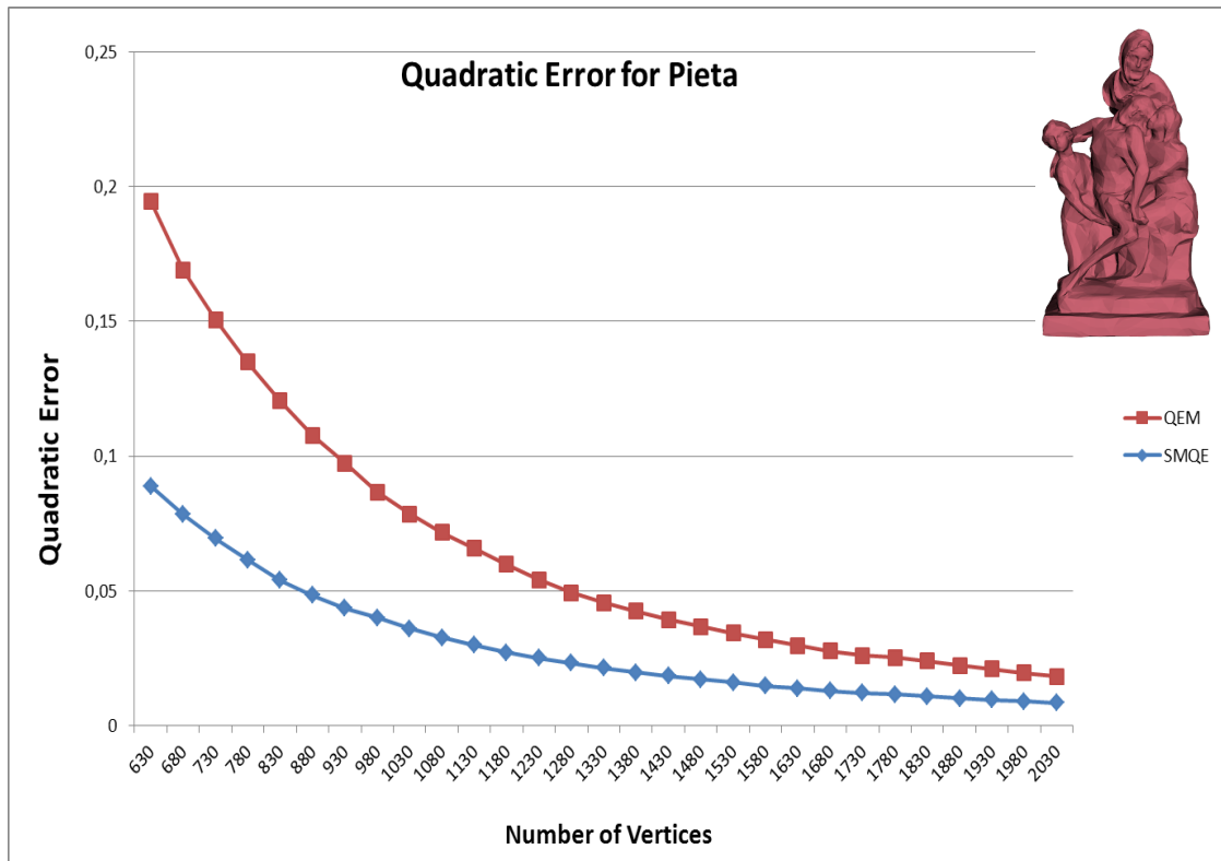
Figure 5.4: The quadratic error introduced in simplification of Pieta model.
