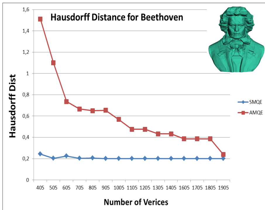
Figure 5.25: The Hausdorff distances introduced in the simplification of Beethoven measured with the Metro tool.
