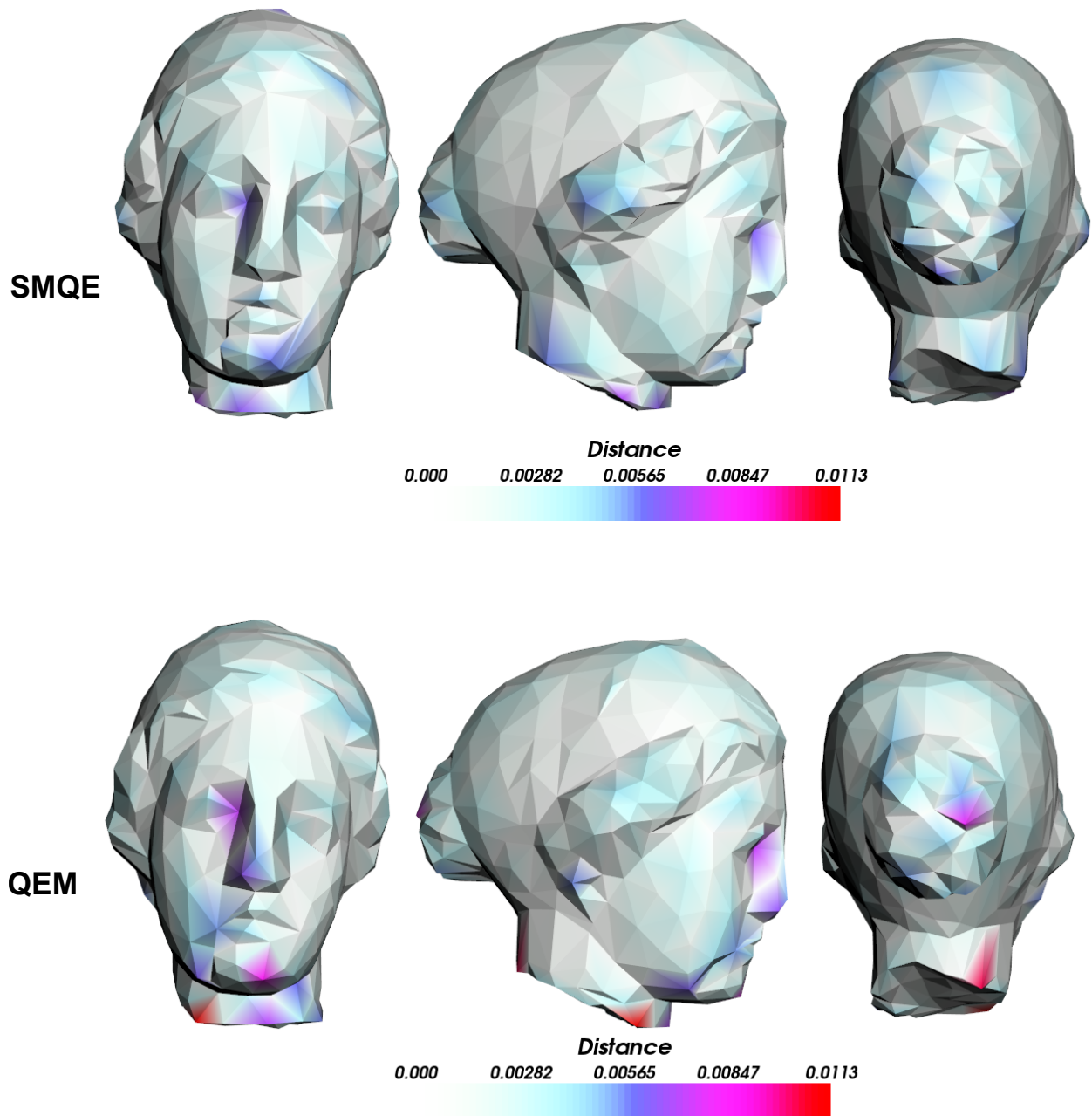
Figure 5.31: The distances between the Venus model and its simplified version with 500 vertices.
