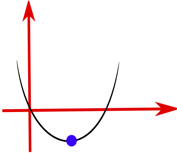
Figure 4.20: The quadratic form of the sum of squared distances from a point to its associated set of planes.
