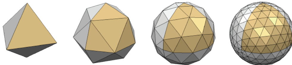
Figure 2.13: Surface subdivision . Each subdivision step increases the number of faces by 4. At each subdivision step, the edges are halved. Image taken from [Botsch et al. , 2006]
