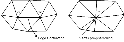
Fig. 1. Edge collapse. Vertices v_1 and v_2 are collapsed into a single vertex \bar{v} . The edge e = (v_1, v_2) and the faces which share this edge are removed after contraction.
