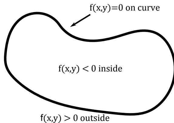
Figure 2.15: The function evaluation for an implicit representation of a surface. If the function is positive, the point (x,y) is outside the object, if it is negative, the point is inside, and the point is situated on the object surface if the function is 0.
