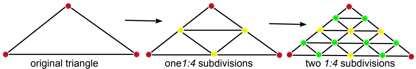
Figure 4.8: Iterative 1:4 subdivisions of a triangle.
