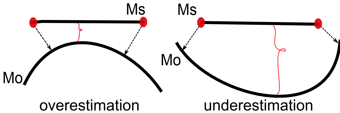
Figure 4.6: Approximation of the distance between two curves taking into consideration only the vertices (red points) of the simplified curve M_s
