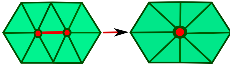
Figure 3.8: Edge Collapse. One edge is collapse to a single vertex. Triangles which share the deleted edge are deleted, too. The number of vertices is reduced by one, the number of faces by two and the number of edges by three.
