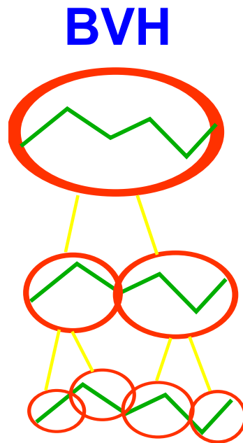
Figure 4.14: The Bounding Volume Hierarchies used by PQP to compute the distance between two objects.
