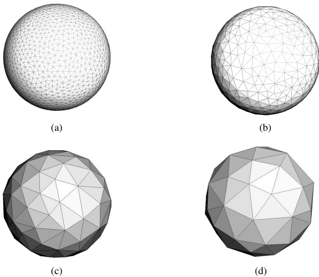
Fig. 6. Approximations of a triangulated sphere. Original model with 2000 vertices. Approximation models using 500, 100 and 50 vertices.
