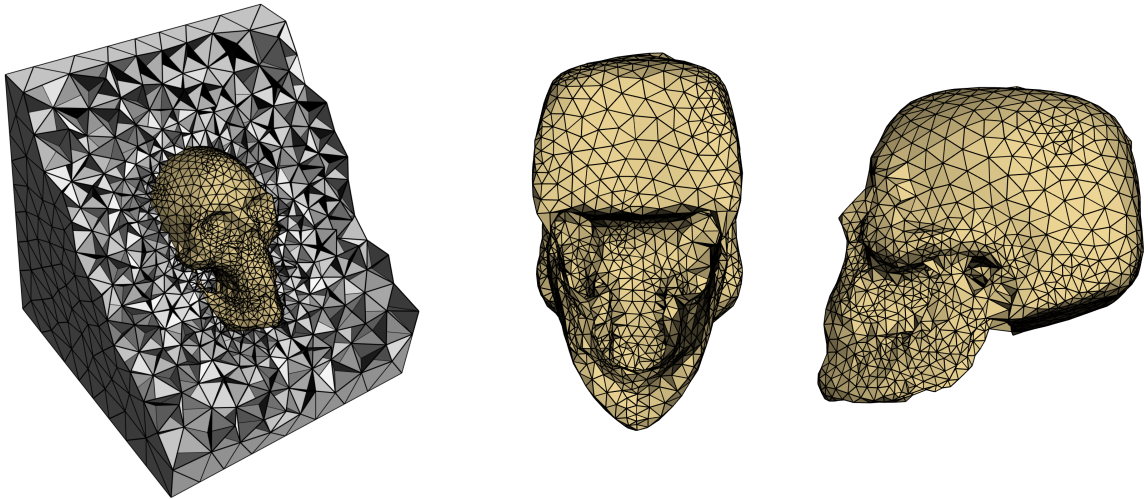
Figure 2.2: Left: Volumetric representation of a human head. Right: The surface representation. For volumetric representation more information is necessary than the surface representation. Volumetric Head model provided courtesy of Julien Dardenne.
