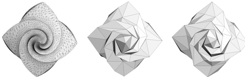
Fig.4: Approximations for Octoflower model: From left to right: Original model with 1919 vertices (15834 triangles), simplified models with 109 vertices using our simplification algorithm and QEM.
