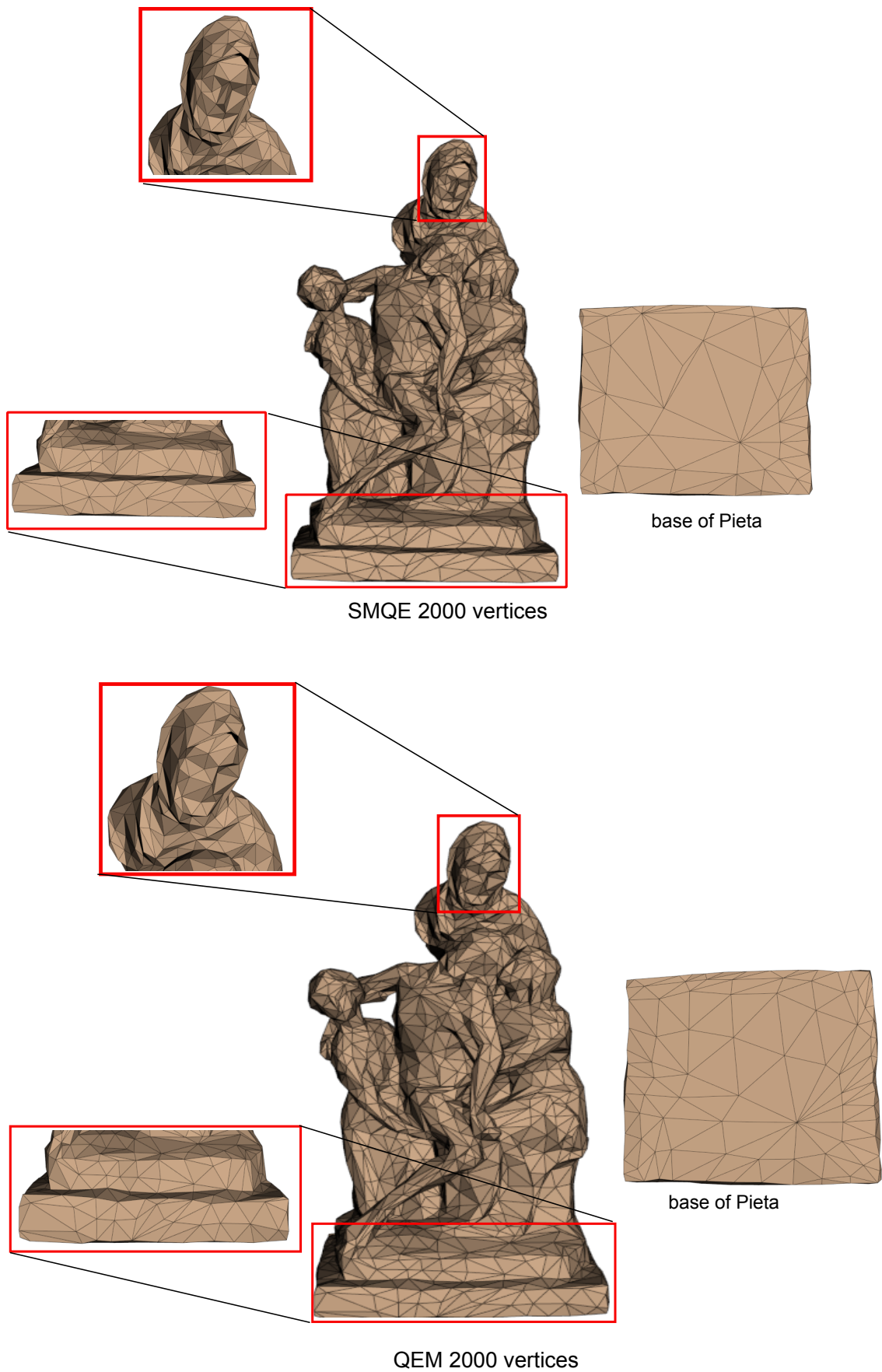
Figure 5.3: The simplified Pietà model with 2000 vertices using SMQE (top) and QEM (bottom).
