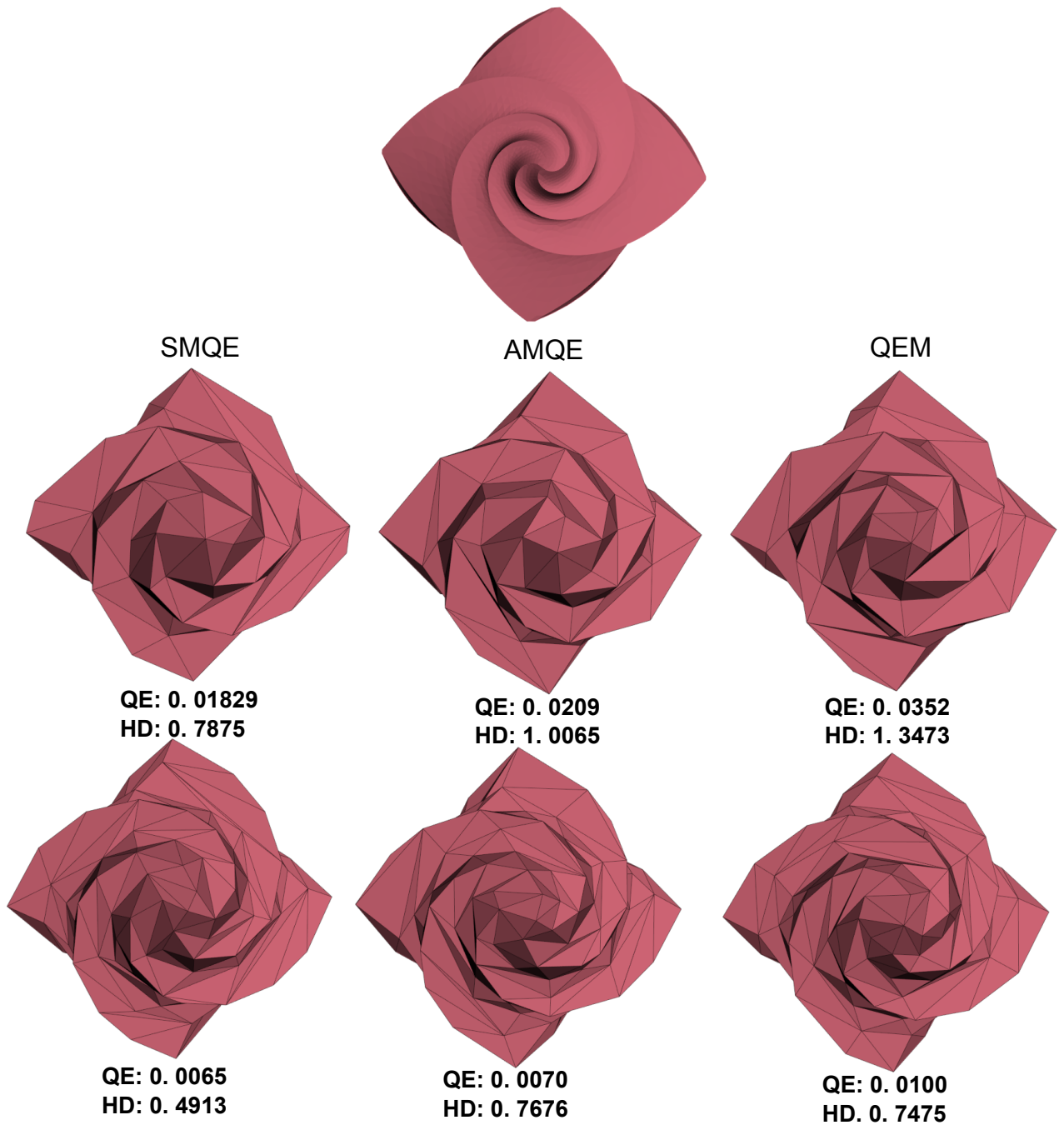
Figure 5.7: Simplifications of Octa-flower model using SMQE, AMQE and QEM. On the top, the simplified model has 99 vertices and 169 on the bottom.
