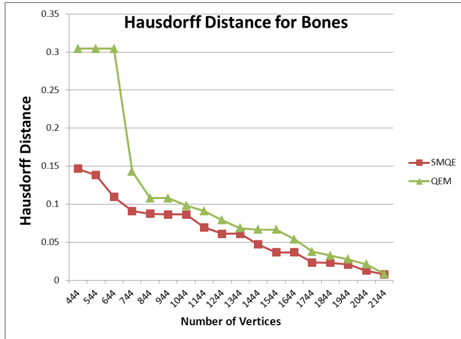
Figure 5.34: Hausdorff Distance for the Bones model vs. Number of Vertices. The Hausdorff distance is computed using the Metro tool.
