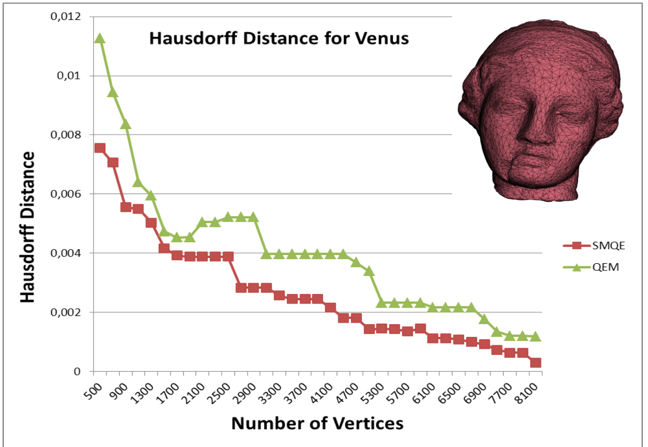
Figure 5.30: The Hausdorff distances introduced in the simplification of the Venus model, measured using the Metro tool.
