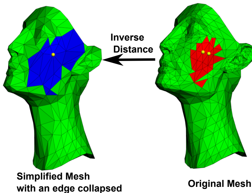
Figure 4.17: The local reverse error between two meshes. The red triangles of the Original Mesh are the triangles for which the distances to the Simplified Mesh are computed.
