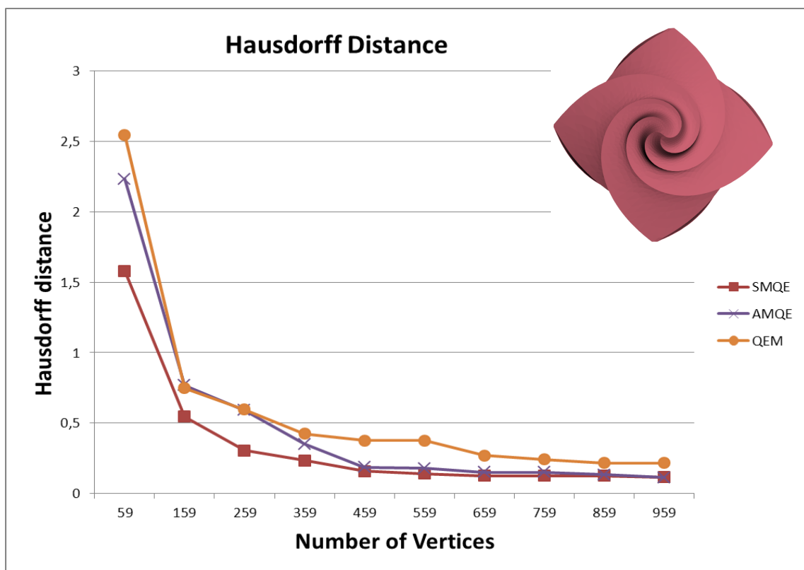
Figure 5.9: The Hausdorff distance introduced in the simplification of the Octa-flower. The Hausdorff distance is computed using the Metro tool.
