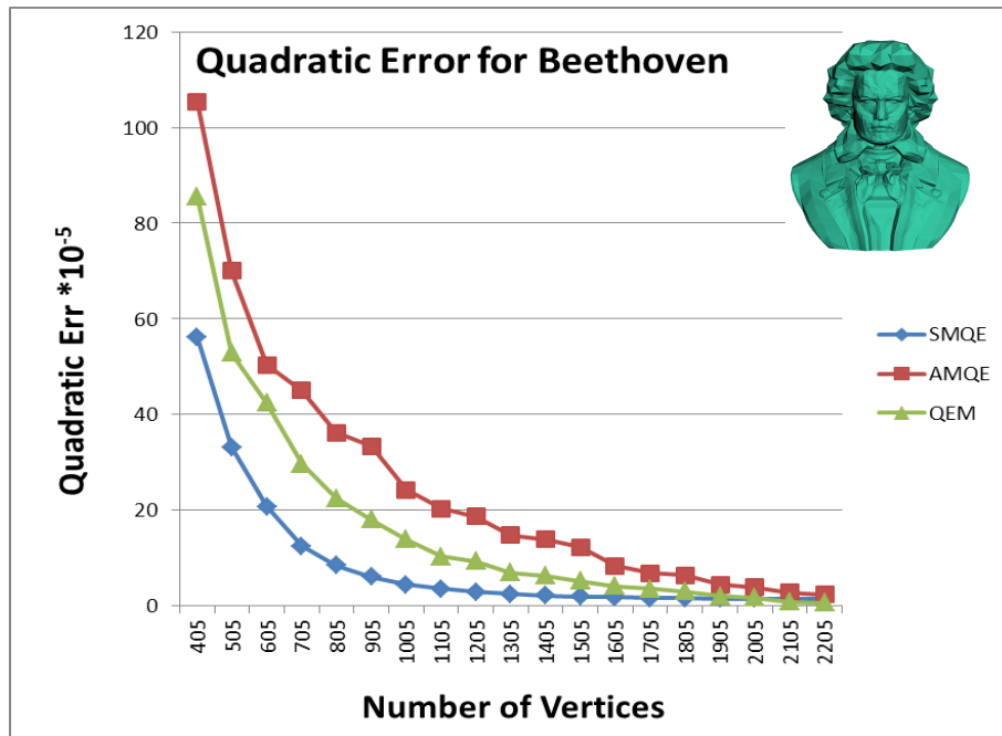
Figure 5.24: The quadratic errors introduced in the simplification of Beethoven.
