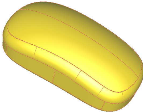
Figure 2.12: Mouse created using spline representation. The Mouse model is provided courtesy of Stephane Guillet by the AIM@SHAPE Shape Repository.
