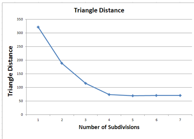
Figure 4.11: The distance for one triangle accordingly to the number of subdivisions of the triangle.
