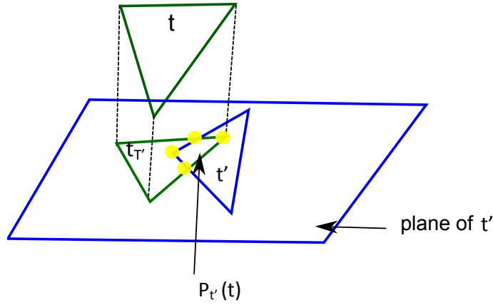
Figure 3.6: Example of the approximation of the Hausdorff distance between two triangles.
