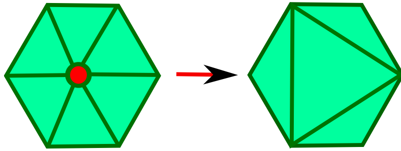
Figure 3.7: Vertex removal. One vertex and the adjacent triangles are removed. The resulting hole is triangulated with fewer triangles.
