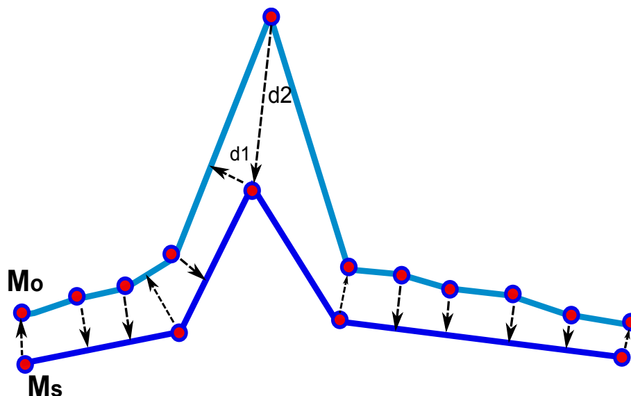
Figure 4.19: A 2D example for importance of SMQE in the preservation of the features of a mesh.
