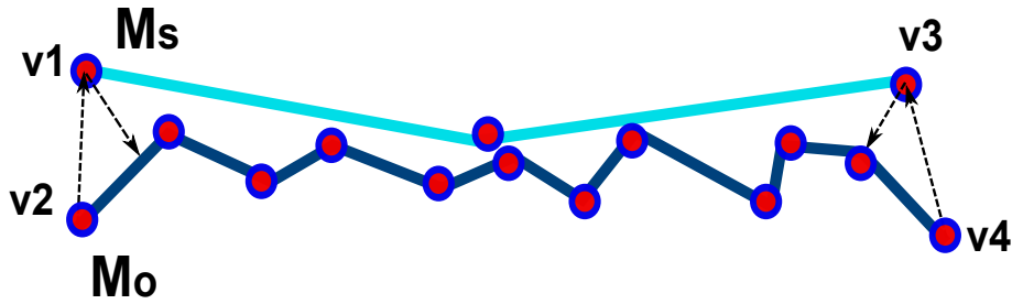
Figure 4.18: A 2D example for application of SMQE on boundaries.
