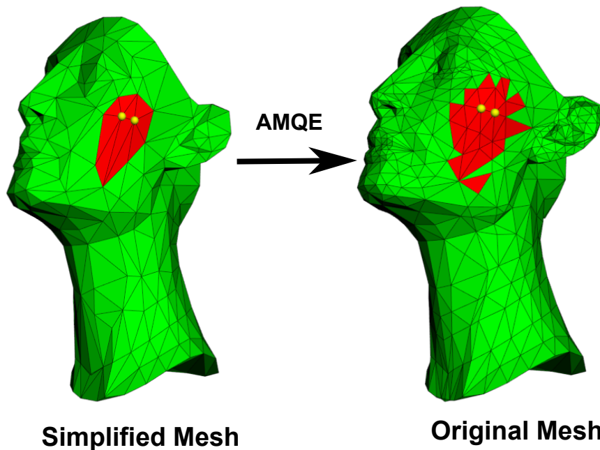
Figure 4.16: The local direct error between two meshes. In order to simulate the collapse for the edge with highlighted endpoints, the distance is computed for all the triangles which share the endpoints (the red triangles of the Simplified Mesh). The red triangles of the Original Mesh are the triangles which are the closest of the red triangles of the Simplified Mesh.
