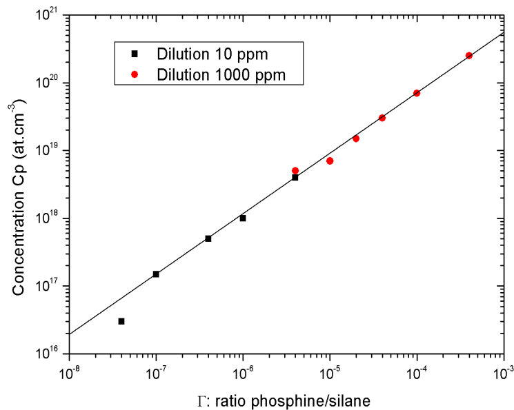
Figure 71: Variation in the concentration of phosphorus atoms versus the molecular ratio \Gamma [102].
