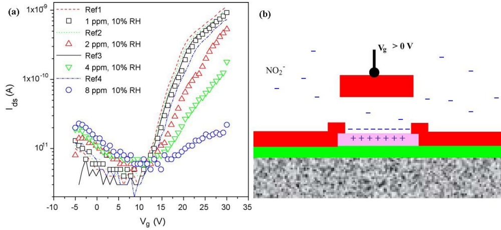
Figure 29: (a) Transfer characteristics of N-type SGFET under different \text{NO}_2 contents in parts-per-million (ppm) at 10% relative humidity (RH) synthetic air, (b) Negative charges -Q_{ss} due to \text{NO}_2 adsorption on channel surface [71].
