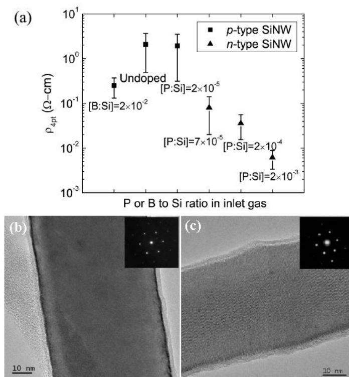
Figure 14: (a) Four-point resistivity of SiNWs grown using [B:Si]=2 \times 10^{-2} , [P:Si]=0 , 2 \times 10^{-5} , 7 \times 10^{-5} , 2 \times 10^{-4} and 2 \times 10^{-3} ; TEM images of phosphorus-doped SiNWs: (b) with [P:Si]=2 \times 10^{-5} , (c) with [P:Si]=2 \times 10^{-3} [37].
