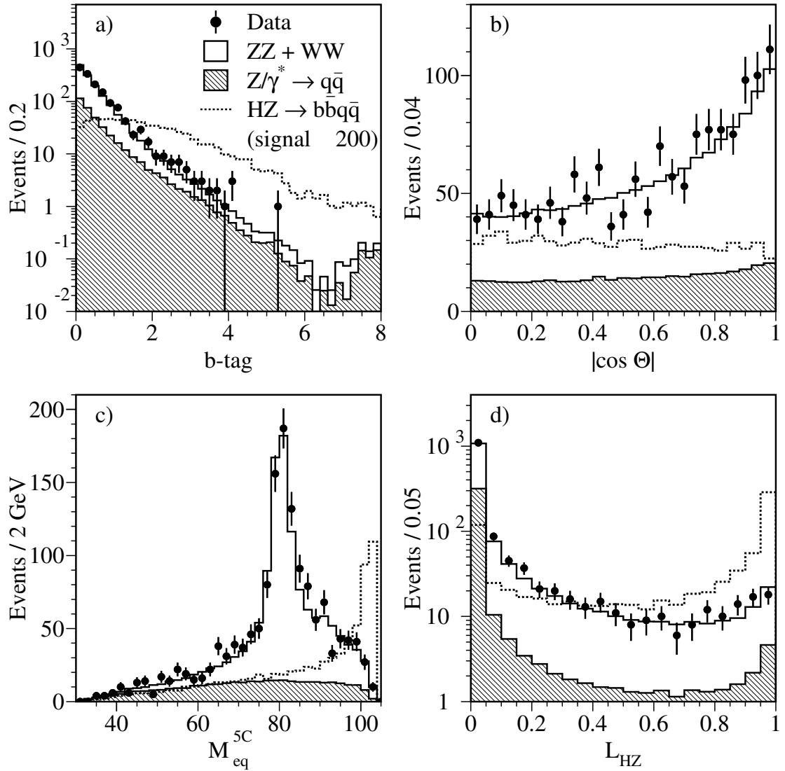
FIGURE 3.6: Distribution of a) the event b -tag, b) the cosine of the boson production angle, c) the mass from the 5C equal-mass fit and d) the likelihood for the events selected in the Hq\bar{q} search channel. The points correspond to the data collected at \sqrt{s} > 206 GeV. The open and hatched histograms are the expected backgrounds from Standard Model processes. The dashed line is the distribution expected for a 115 GeV Higgs signal, multiplied by a factor of 200.
