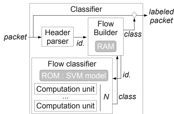
Figure 4.2: Architecture of the classifier
